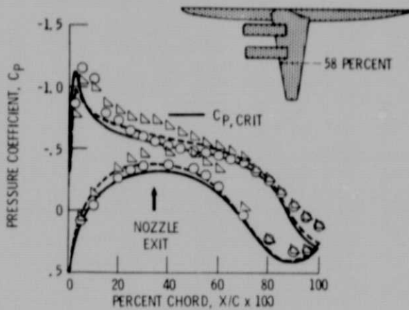
Figure 21. - Comparison of analytical and experimental wing pressures outboard of nacelles - nacelles on vs nacelles off.
