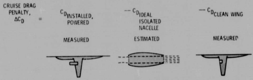
Figure 9. - Drag definition.
