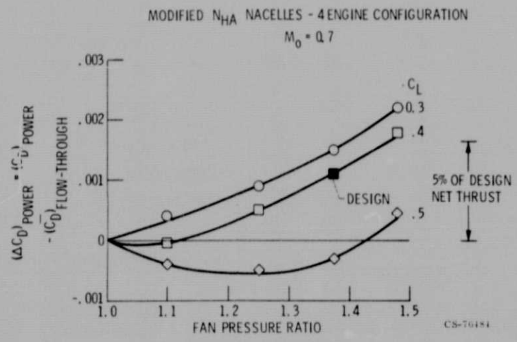
Figure 10. - Power effect.
