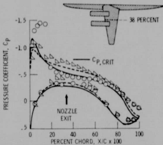
Figure 22. - Comparison of analytical and experimental wing pressures between nacelles - nacelles on vs nacelles off.
