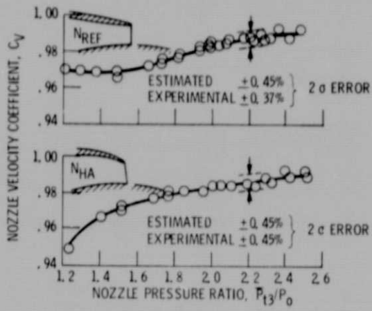
Figure 8. - Static calibration results.
