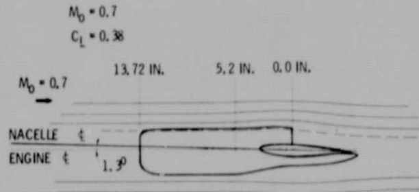
Figure 5. - Streamline contoured nacelle, profile view.
