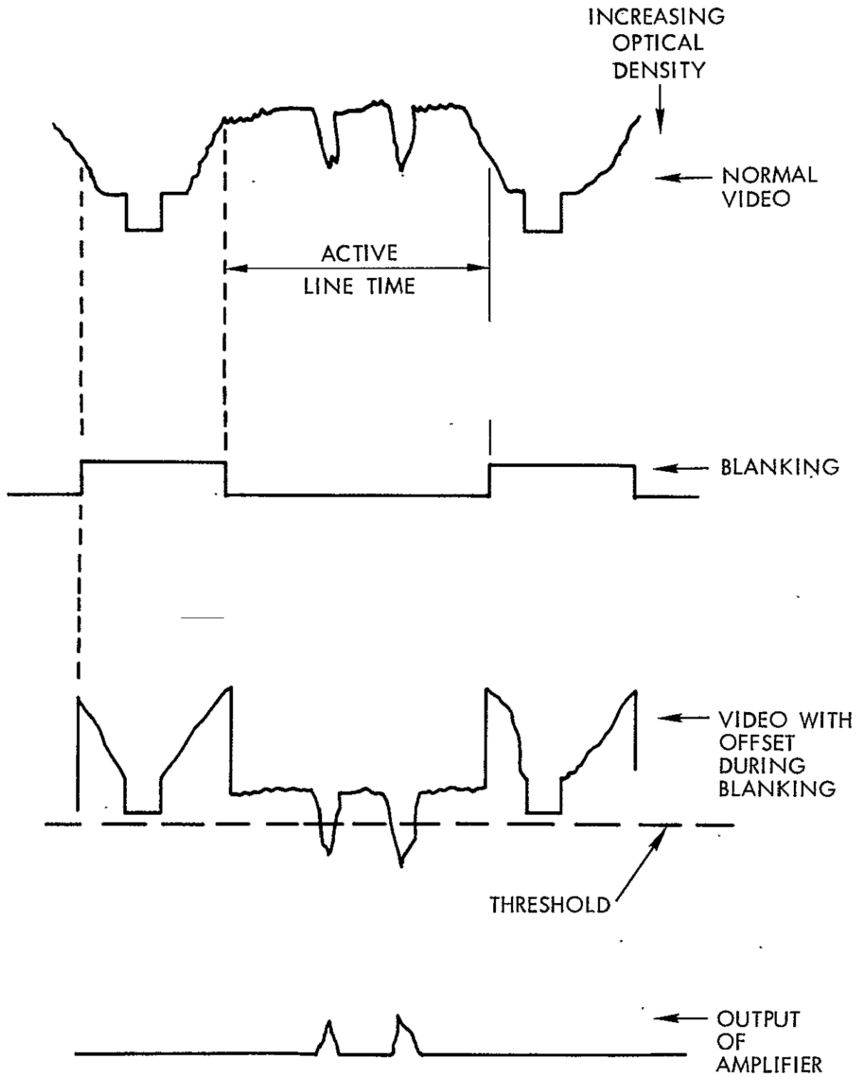
Figure 6-11. IOD waveform
