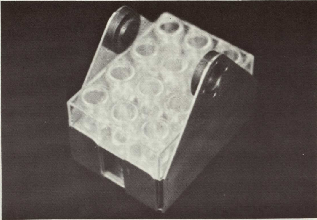
Fig. 4-5. Centrifuge carrier
