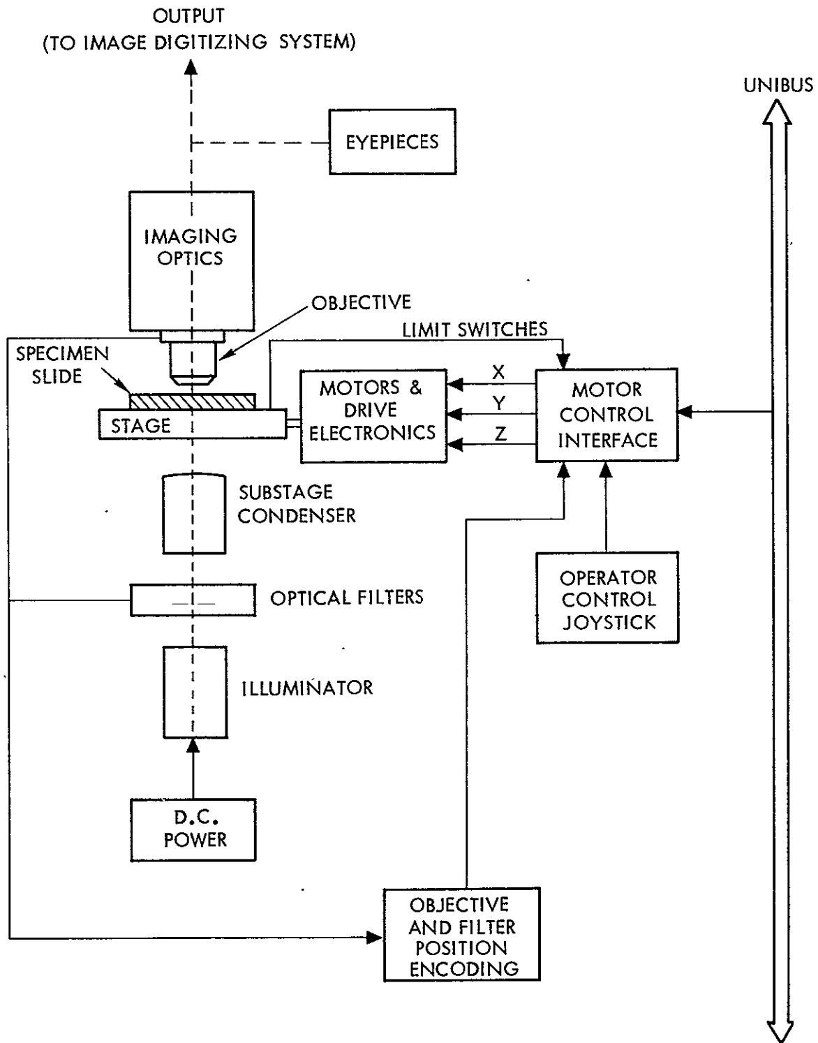
Fig. 6-2. Microscope/stage system
