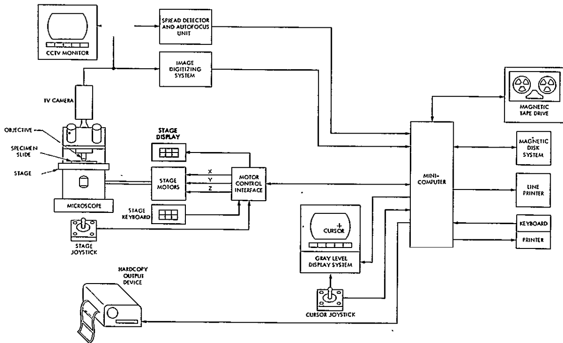
Fig. 3-3. System configuration
