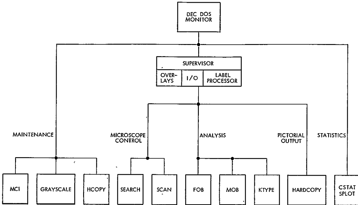
Figure 7-1. Software hierarchy
