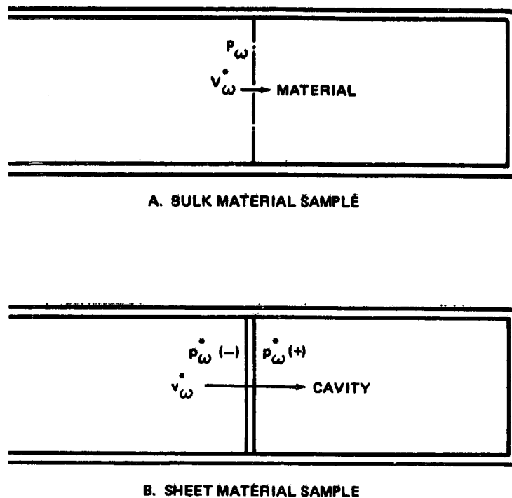
Figure 1. Impedance Concepts for Bulk and Sheet Materials
