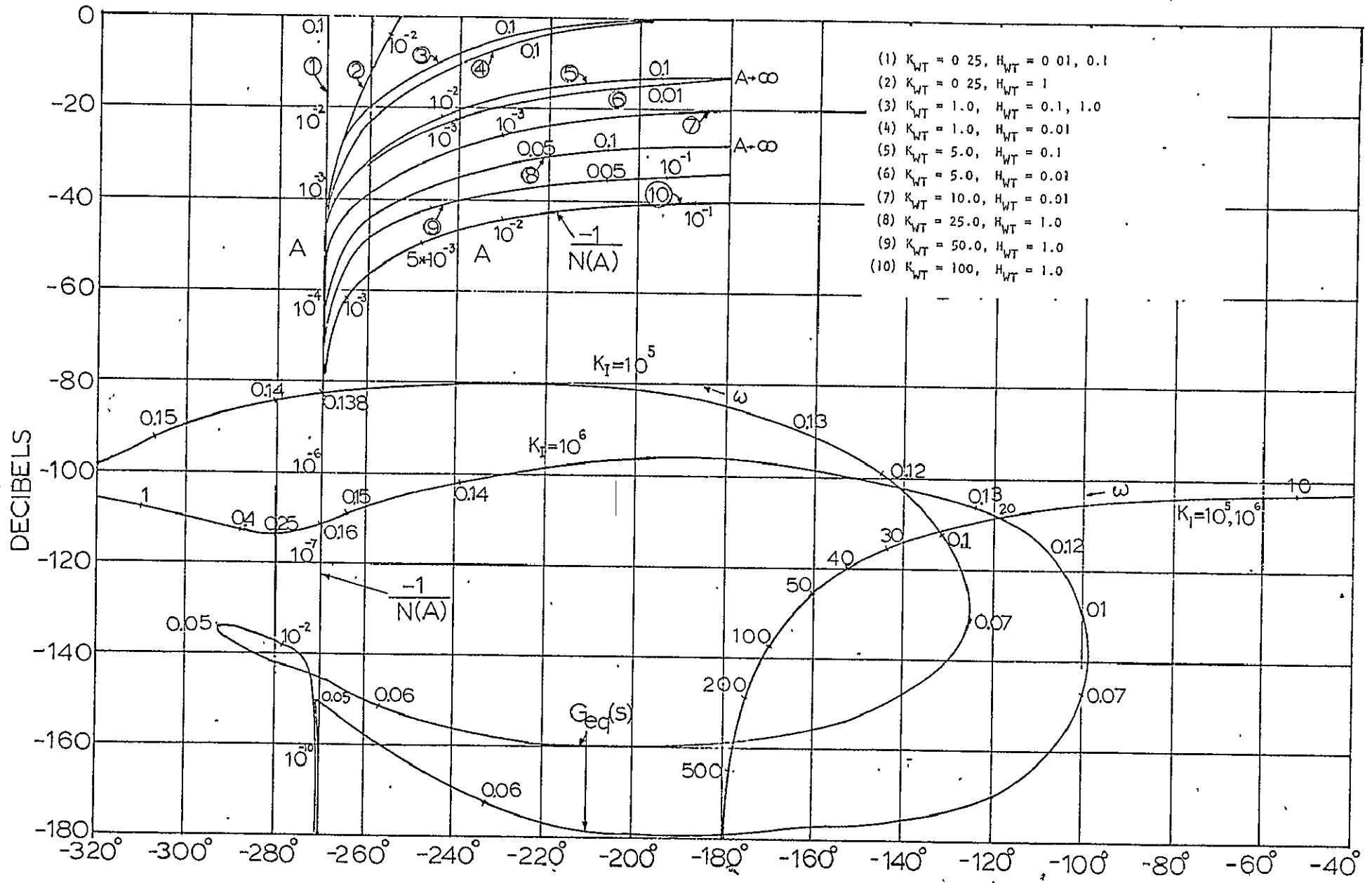
Figure 9-2. Frequency response plots and describing function loci of IPS system with flex pivot and wire cable nonlinearities (Dahl model).
