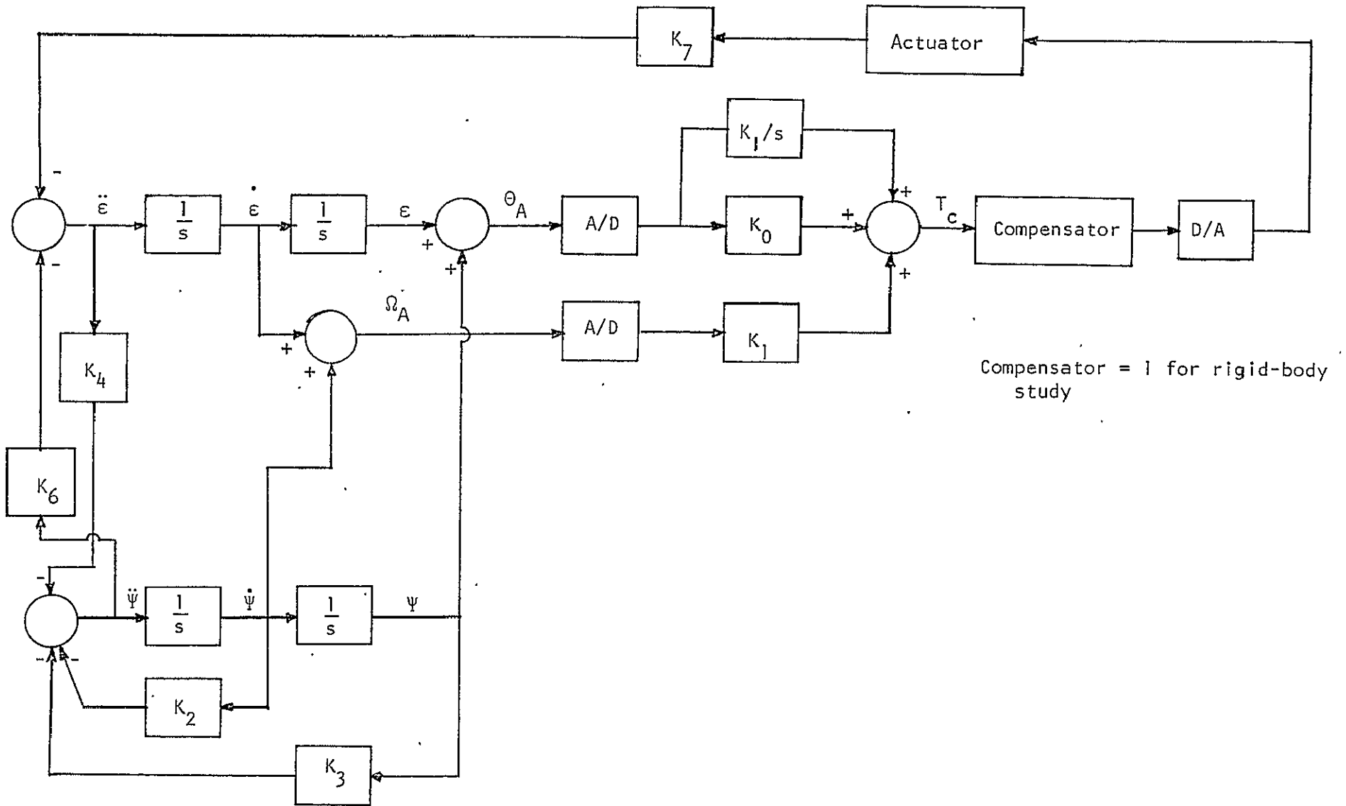
Figure 1-1. Block diagram of simplified linear IPS control system.
