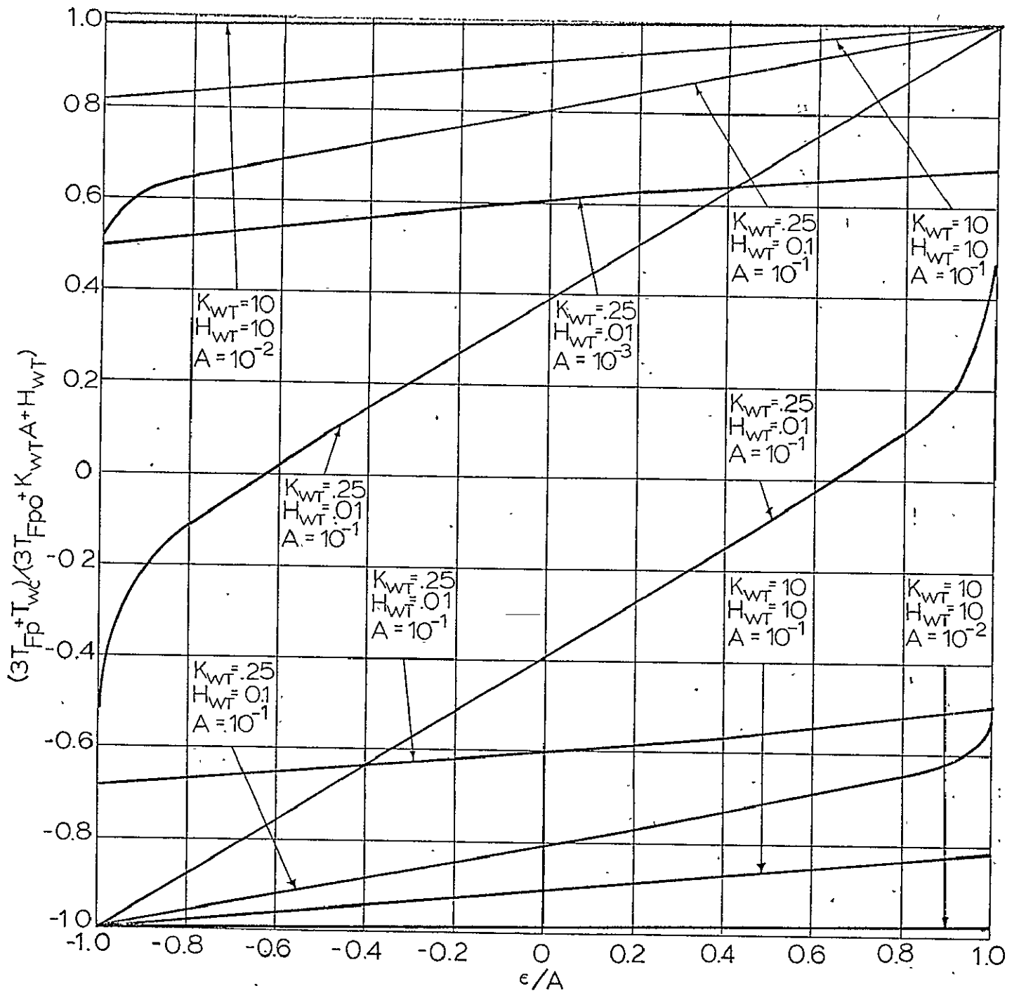
Figure 8-4. Normalized flex pivot plus wire cable torques versus \epsilon/A for IPS with cosine function input.
