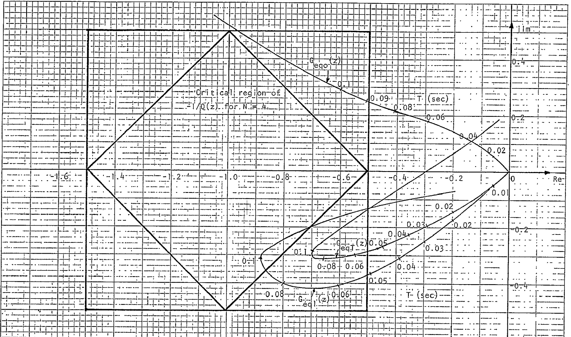
Figure 6-13. Frequency loci of G_{eqo}(z) , G_{eqI}(z) , G_{eqT}(z) , and the critical region of -1/Q(z) of quantizer for N=4 and K=10^7 .
