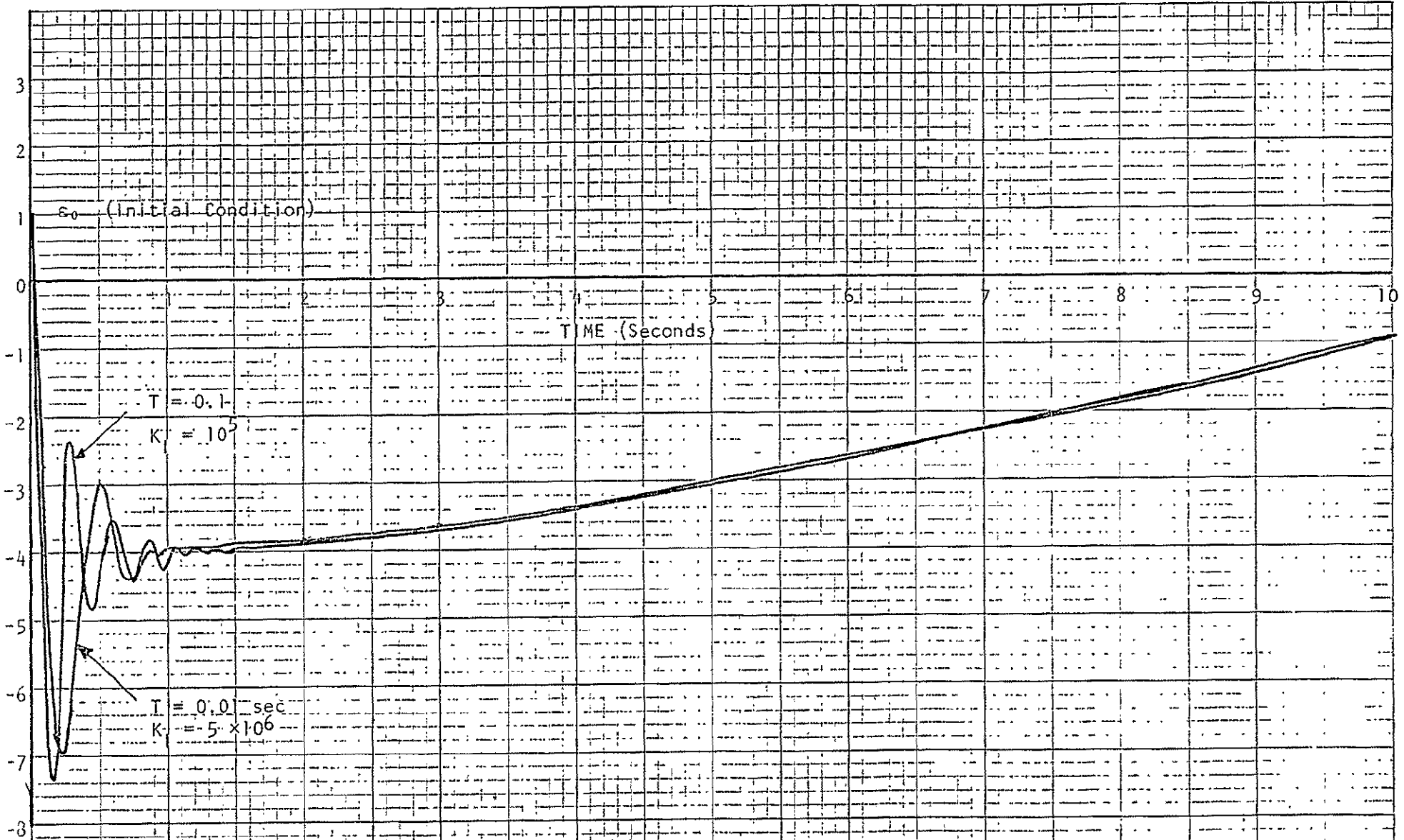
Figure 2-7. Responses of \epsilon(t) of simplified digital IPS control system.
