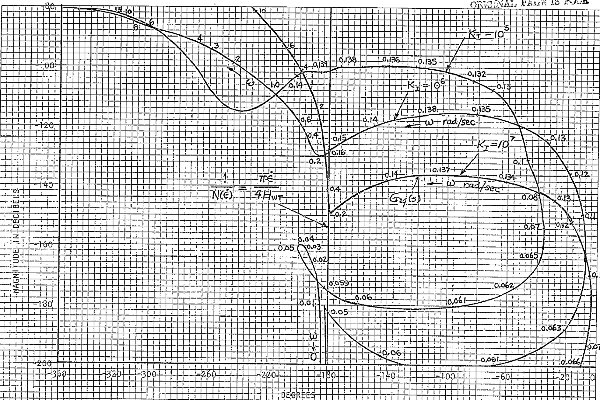
Figure 3-6. Frequency response and describing function plots for self-sustained oscillations analysis.
