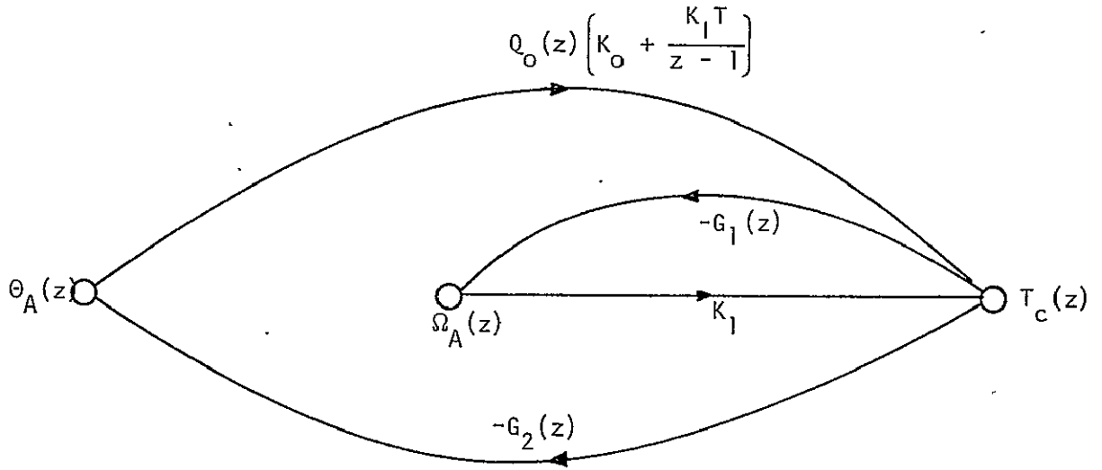
Figure 6-1. Digital signal flow graph of IPS when Q_0 is in effect.
