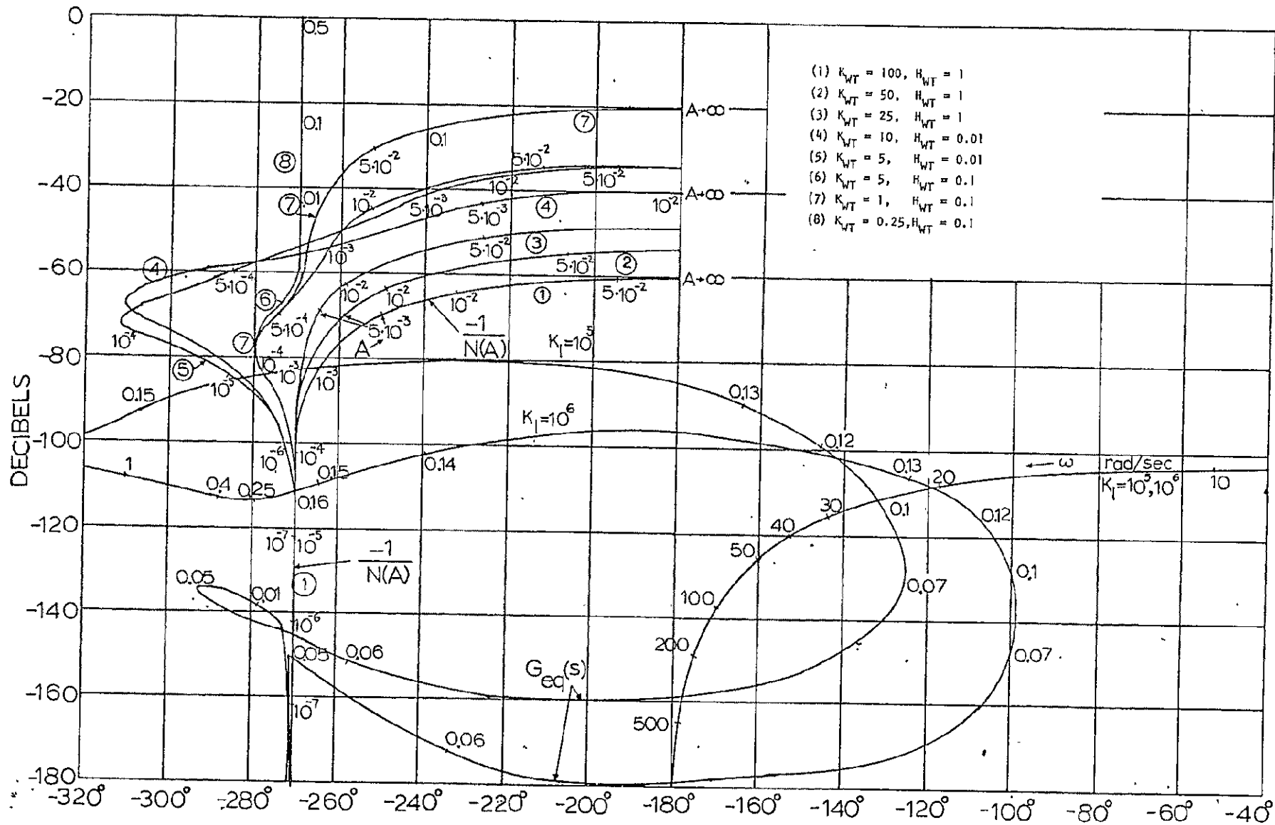
Figure 11-2. frequency response plots and describing function loci of IPS system with flex pivot and wire cable nonlinearities (Dahl model i = 1 ).
