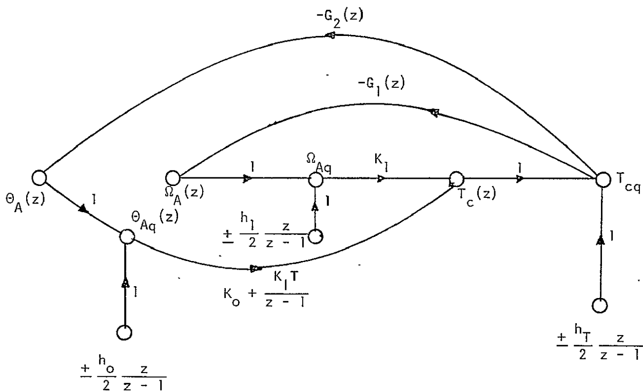
Figure 5-3. Digital signal flow graph of the simplified digital IPS with quantization.
