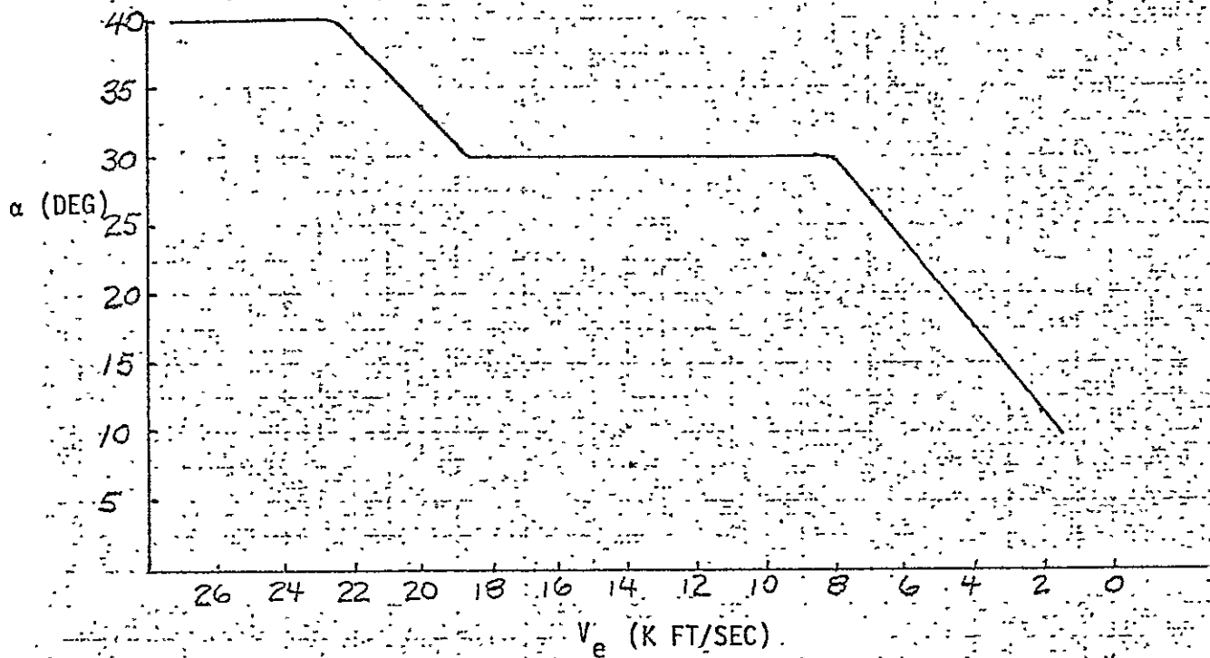
TPS DESIGN TRAJECTORY (40°/30° \alpha )
