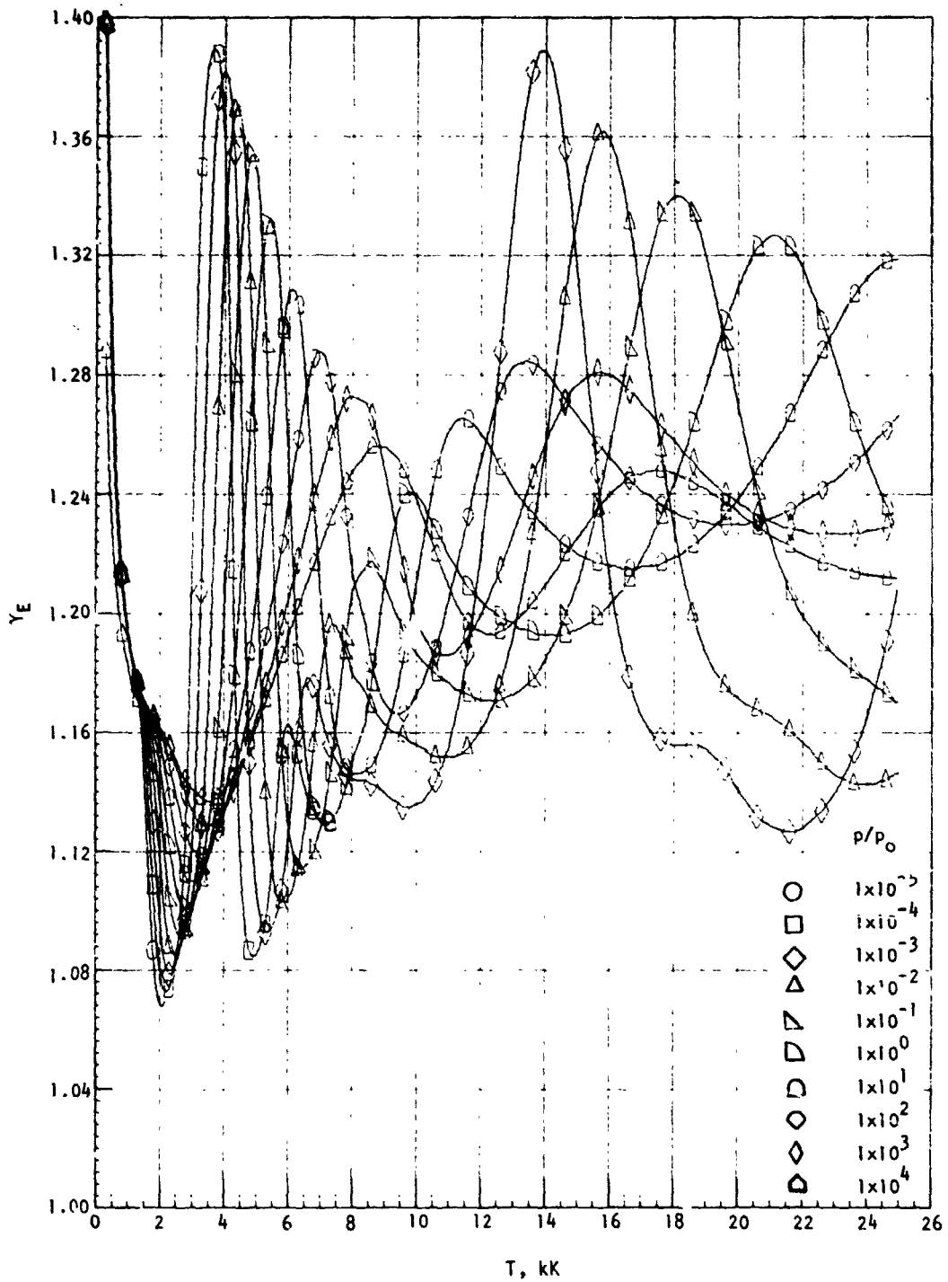
(h) Isentropic exponent, \gamma_E .
