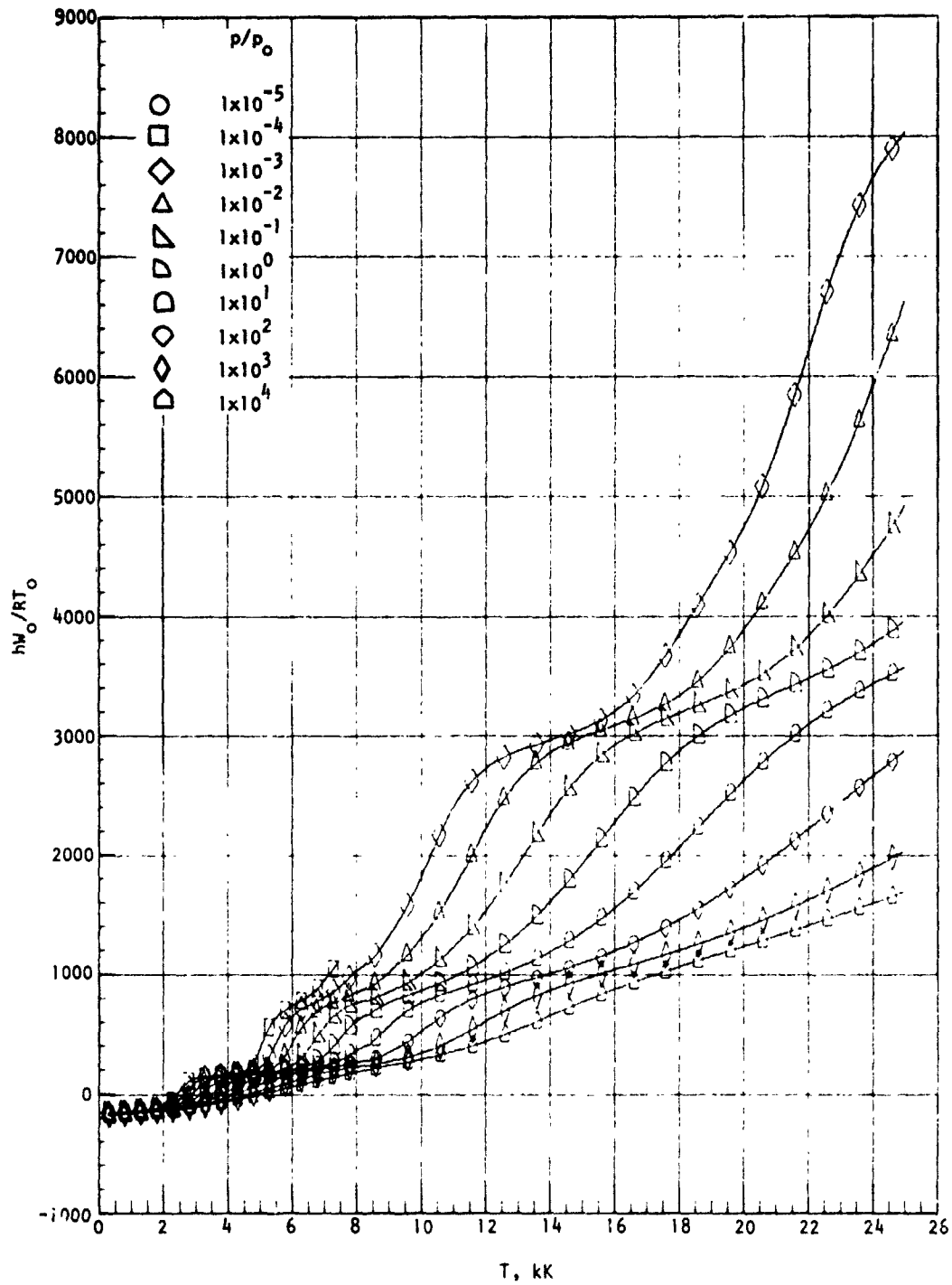
(b) Enthalpy, hW_0/RT_0 .
