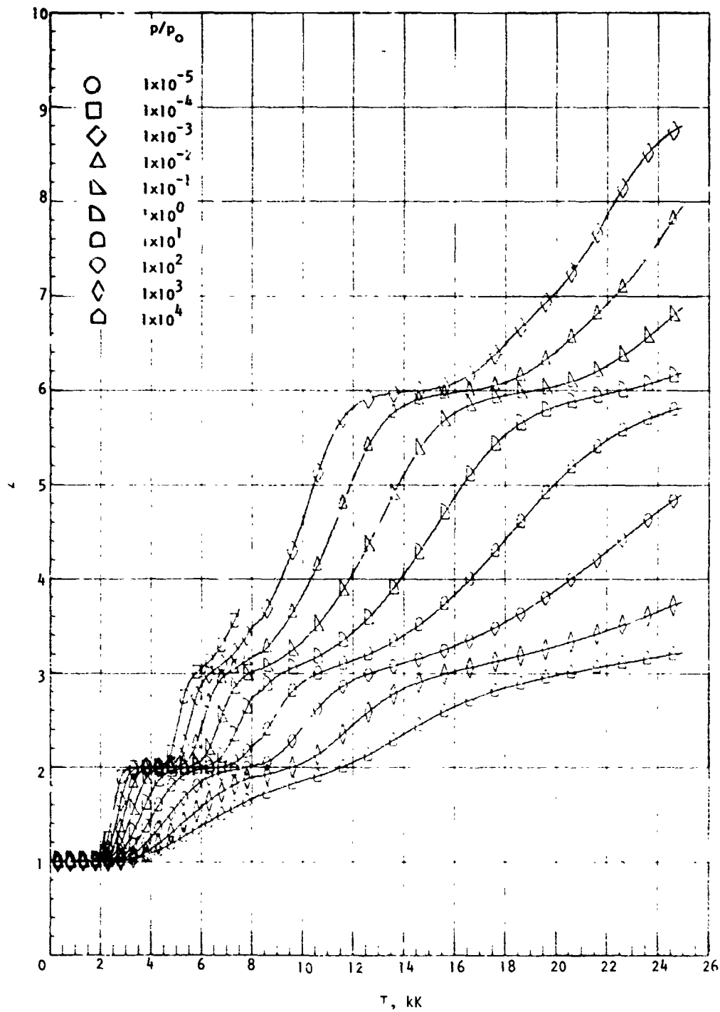
(e) Z = ratio of dissociated carbon dioxide per kmole of undissociated carbon dioxide, Z .
