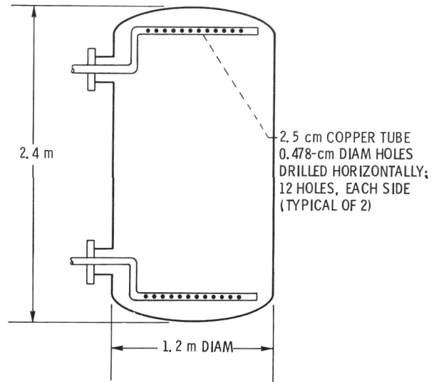
Figure 4. - Flow distribution manifold design.
