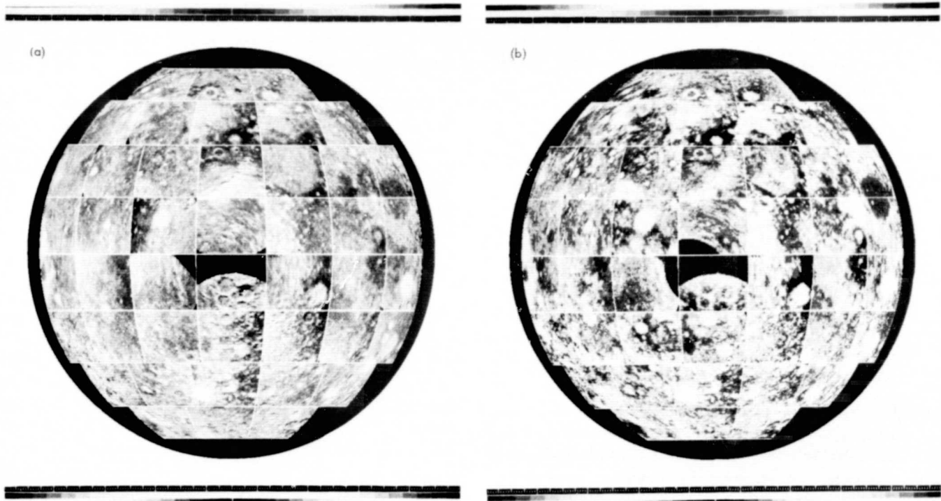
Fig. 2. Data sets for the S-217 Experiment: 70-cm polarized and depolarized radar echoes (provided by T. W. Thompson; see Ref. 15)
