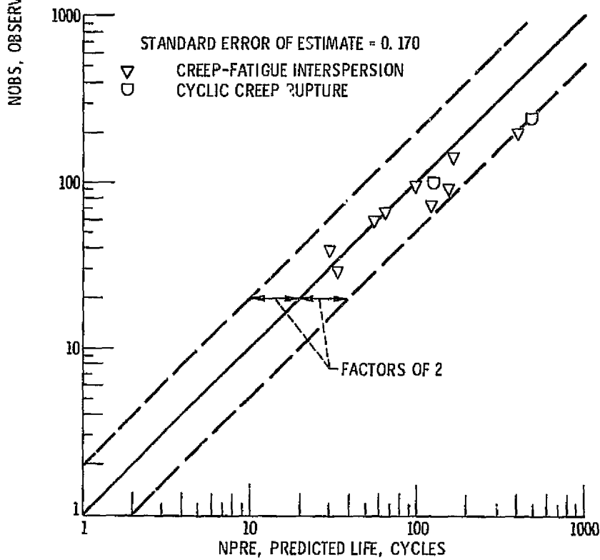
Fig. 4. - Comparison of observed MPC creep-fatigue lives of annealed \frac{1}{2}\text{Cr}-1\text{Mo} steel versus lives predicted on basis of strainrange partitioning using interaction damage rule.
