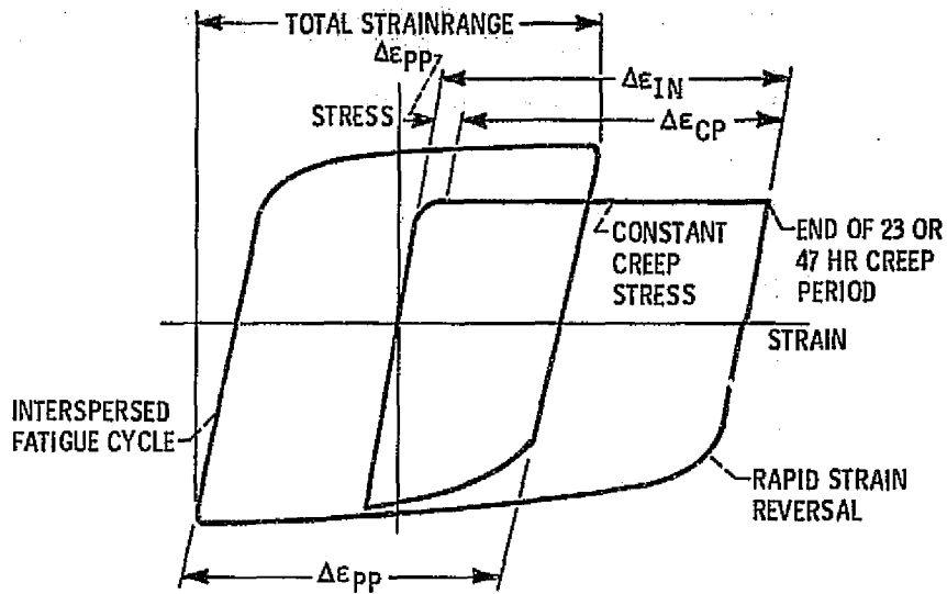
Fig. 1 - Schematic hysteresis loops associated with MPC creep-fatigue interspersed tests (16). Cyclic creep rupture tests involve only creep portion with no interspersed fatigue cycles. Partitioned strainranges indicated on loops.
