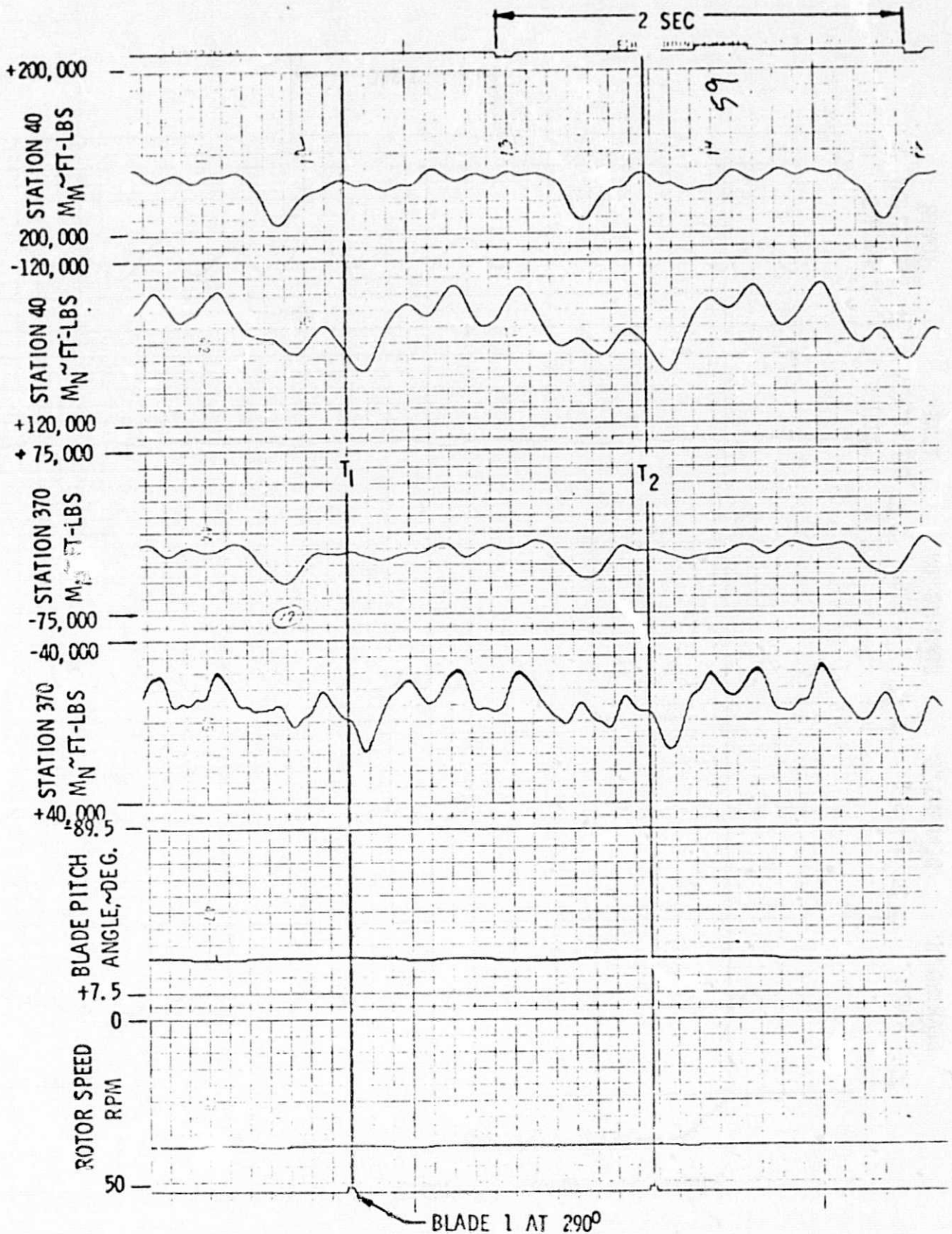
FIGURE 6 40 RPM , 0 POWER
