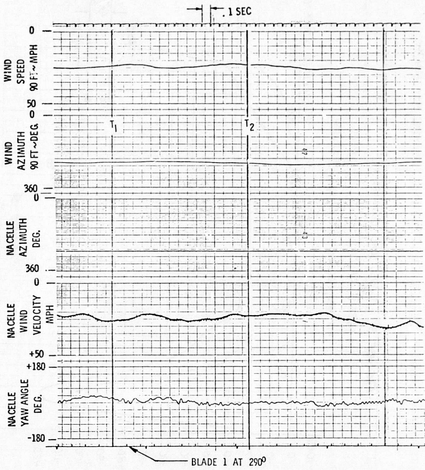
FIGURE 8d GUST RESPONSE (W/SHAFT OSCILLATION)
