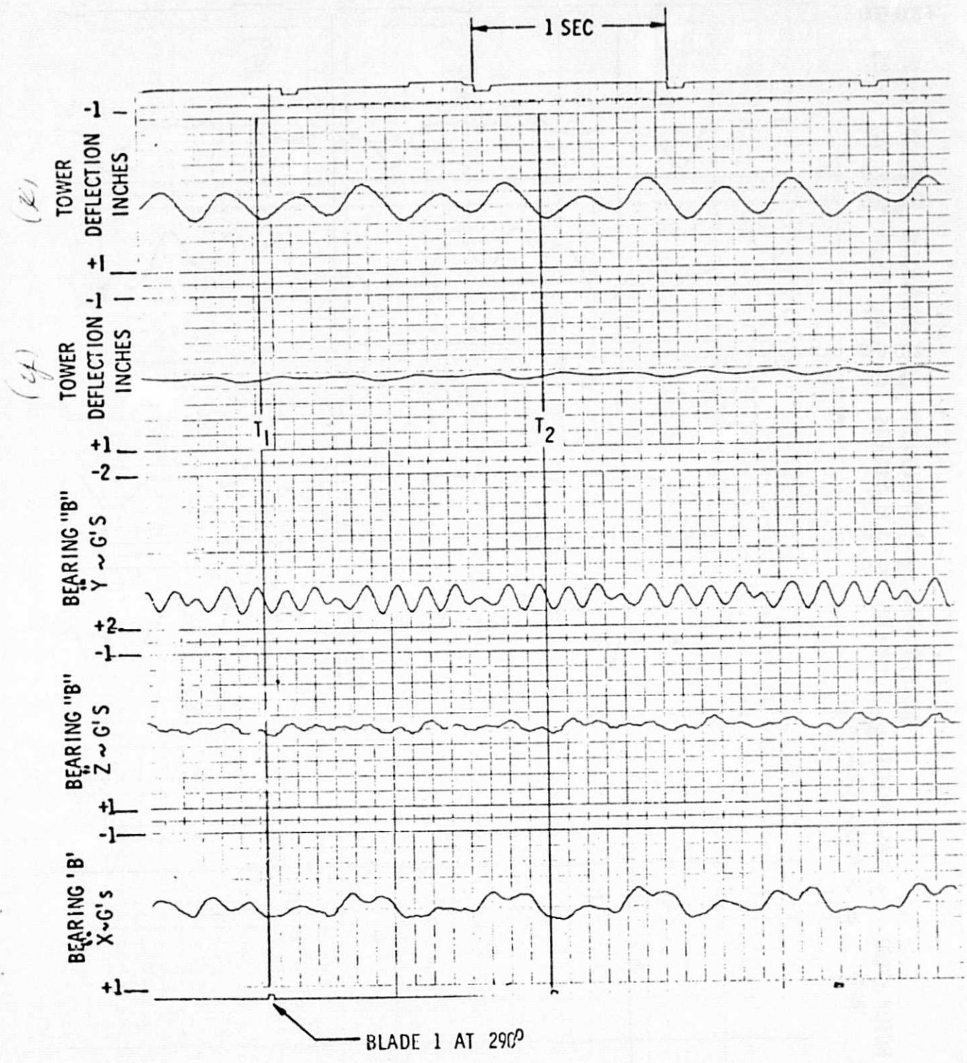
FIGURE 5c 40 RPM , 100 kW
