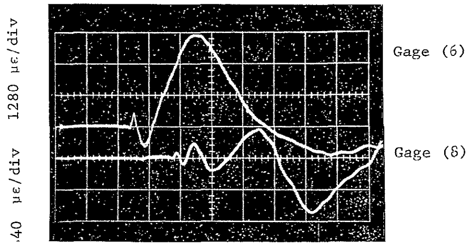
(b) 20μsec/div
