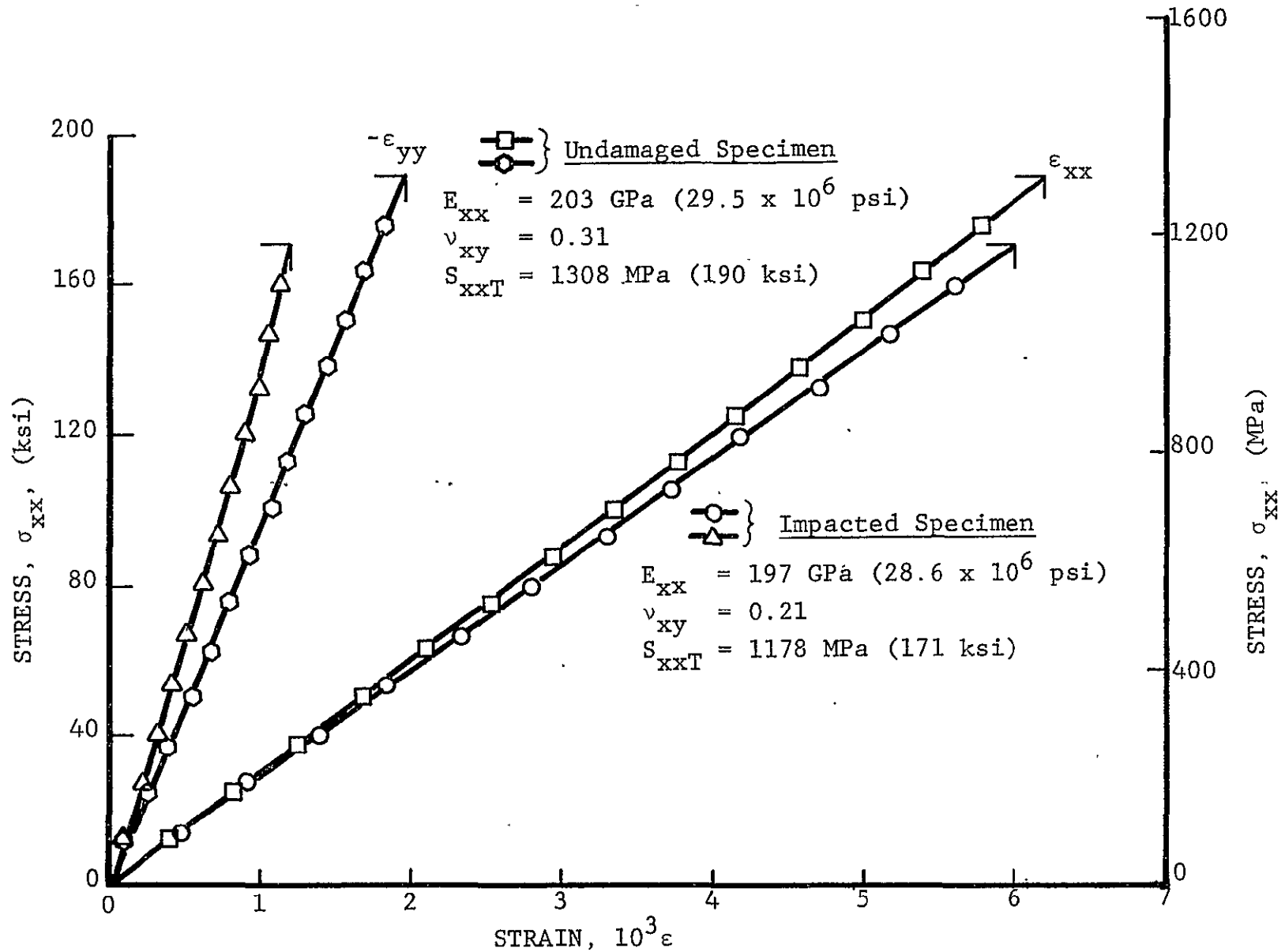
Fig. 46 STRAINS IN [0 16 ] GRAPHITE/EPOXY SPECIMENS UNDER UNIAXIAL TENSION FROM UNDAMAGED AND IMPACTED LAMINATES (Impact Velocity: 192 ms -1 ; 630 ft/sec)
