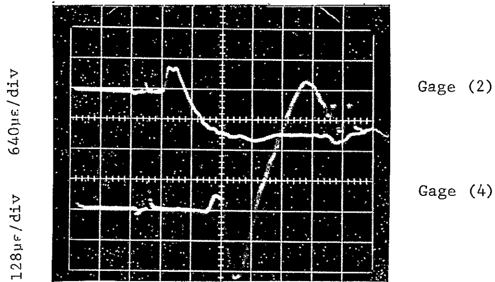
(b) 20\mu\text{sec}/\text{div}
