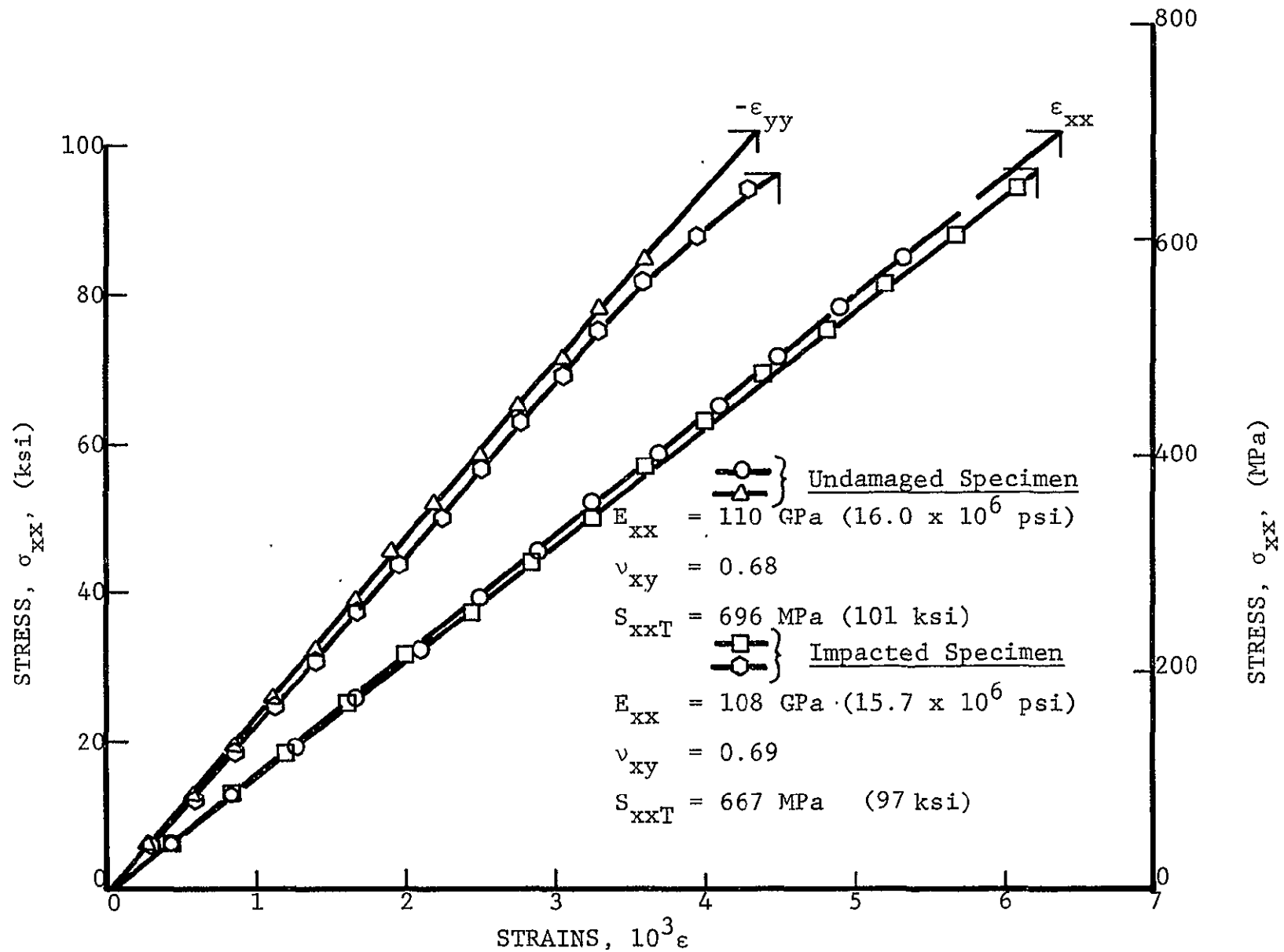
Fig. 48 STRAINS IN [0_2/+45]_2s GRAPHITE/EPOXY SPECIMENS UNDER UNIAXIAL TENSION FROM UNDA MAGED AND IMPACTED LAMINATES (Impact Velocity: 192 \text{ ms}^{-1} ; 630 \text{ ft/sec} )
