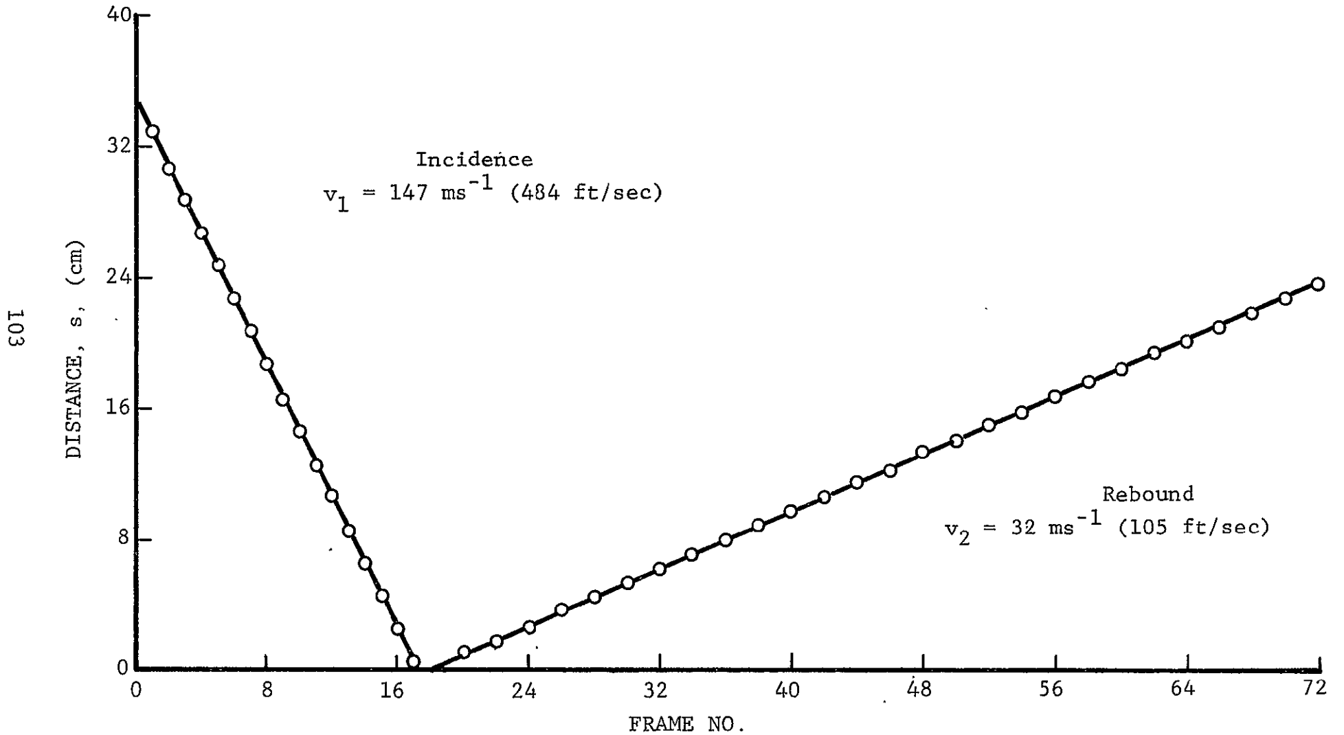
Fig. 56 PROJECTILE DISTANCE FROM IMPACTED PLATE AS A FUNCTION OF FRAME NUMBER (Barrel Pressure: 138 kPa, 20 psi; Plate: [0 16 ] Graphite/Epoxy; 137 \mu\text{s} /frame)
