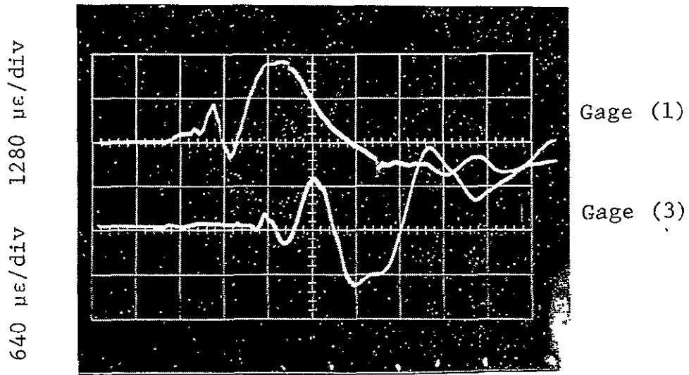
(a) 20 μsec/div
