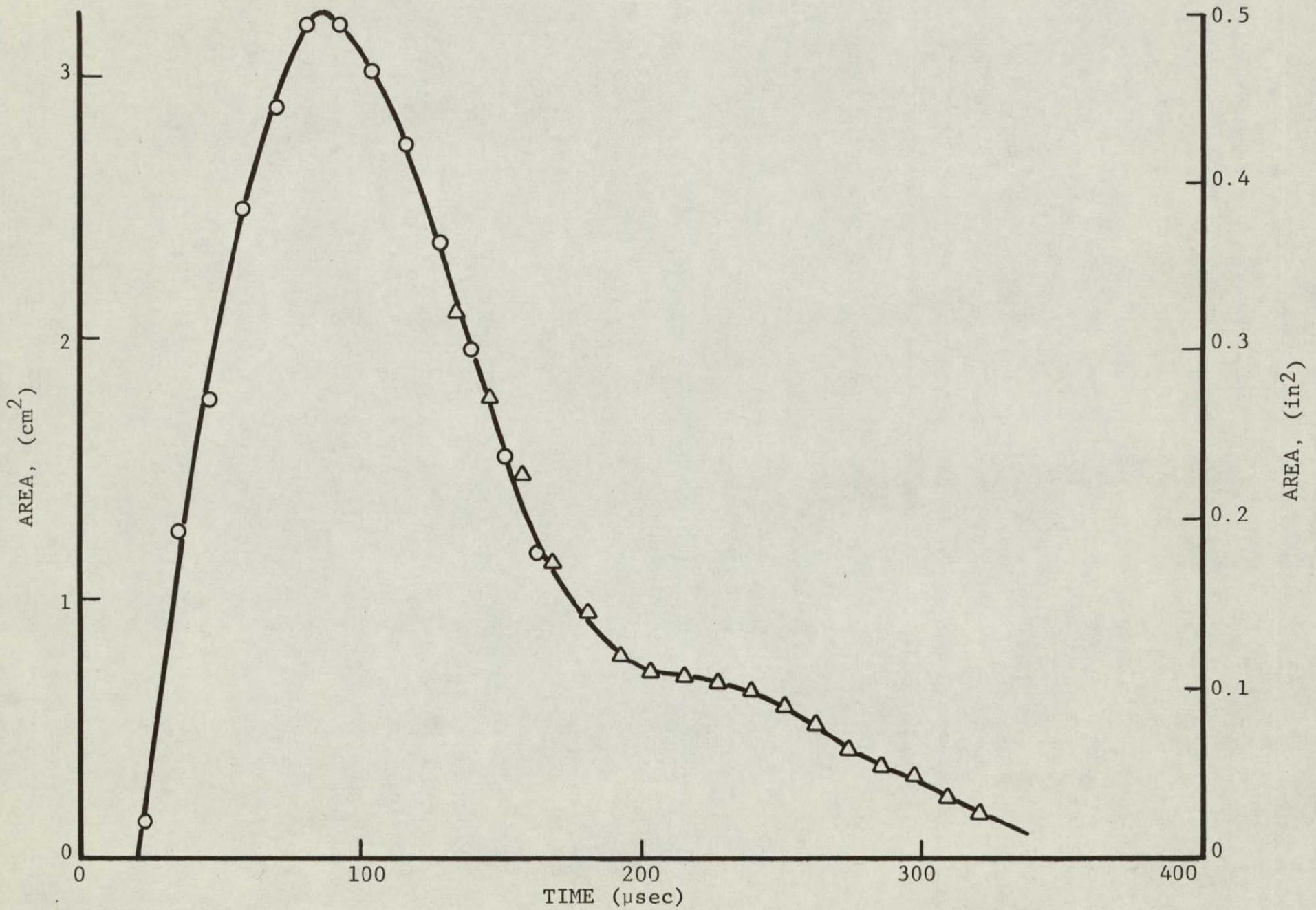
Fig. 63 CONTACT AREA OF PROJECTILE WITH TARGET PLATE AS A FUNCTION OF TIME (7.9 mm diam. Silastic Sphere Impacting at 180 \text{ ms}^{-1} )
