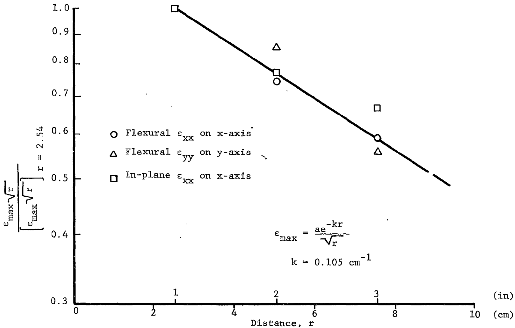
Fig. 24 SEMILOGARITHMIC PLOT FOR SEPARATING MATERIAL AND GEOMETRIC ATTENUATION IN [0_{16}] BORON/EPOXY SPECIMEN IMPACTED NORMALLY WITH A SILASTIC SPHERE
