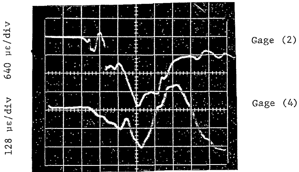
(b) 20 μsec/div
