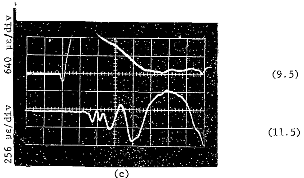
Fig. 16 STRAIN GAGE SIGNALS ALONG 45-DEGREE AXIS OF TRANSVERSELY IMPACTED [016] BORON/EPOXY SPECIMEN (Sweep: 20 \mu s/div) (a) Gages in y-direction 7.62 cm (3 in.) apart (b) Gages in x-direction 7.62 cm (3 in.) apart (c) Gages in 45-degree direction 7.62 cm (3 in.) apart
