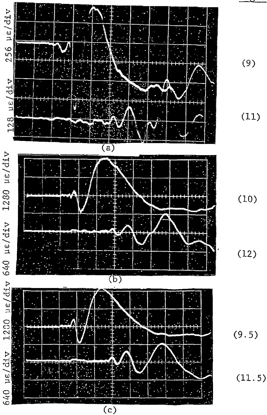
Fig. 30 STRAIN GAGE SIGNALS IN TRANSVERSELY IMPACTED [0_2/\pm 45]_{2s} BORON/EPOXY SPECIMEN 9BA-1 ON 45-DEGREE AXIS (Sweep: 20 \mu\text{sec/div} )
