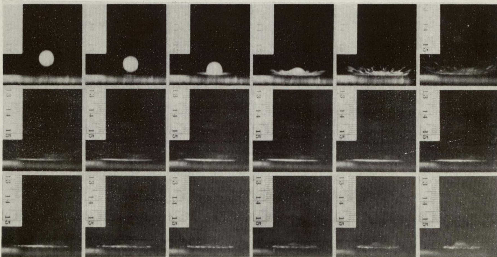
Fig. 64 IMPACT OF 7.9 mm (5/16 in) DIAMETER SILASTIC SPHERE ON [0 2 /+45] 2 s BORON/EPOXY PLATE AT 242 ms -1 (794 ft/sec). (Camera Speed: 85,700 frames/second)
