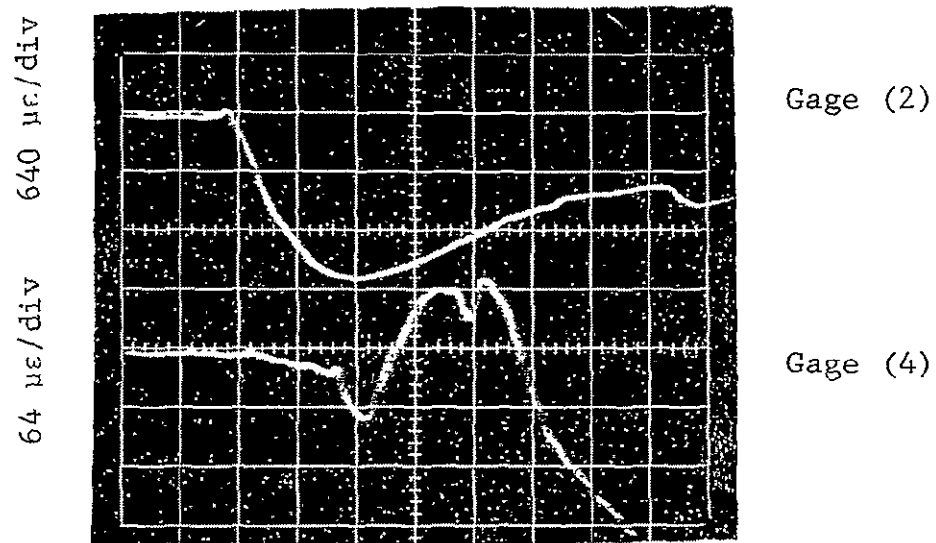
(b) 20 μsec/div
