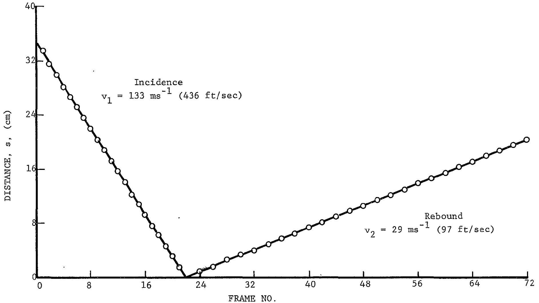
Fig. 55 PROJECTILE DISTANCE FROM IMPACTED PLATE AS A FUNCTION OF FRAME NUMBER (Barrel Pressure: 69 kPa, 10 psi; Plate: [016] Graphite/Epoxy; 138 \mu\text{s}/\text{frame} )
