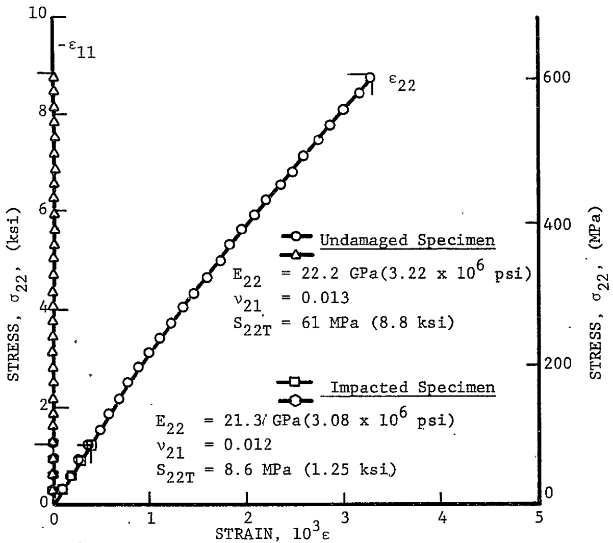
Fig. 43 STRAINS IN [90]_{16} BORON/EPOXY SPECIMENS UNDER UNIAXIAL TENSION FROM UNDAMAGED AND IMPACTED LAMINATES (Impact Velocity: 210 \text{ ms}^{-1} ; 690 \text{ ft/sec} )
