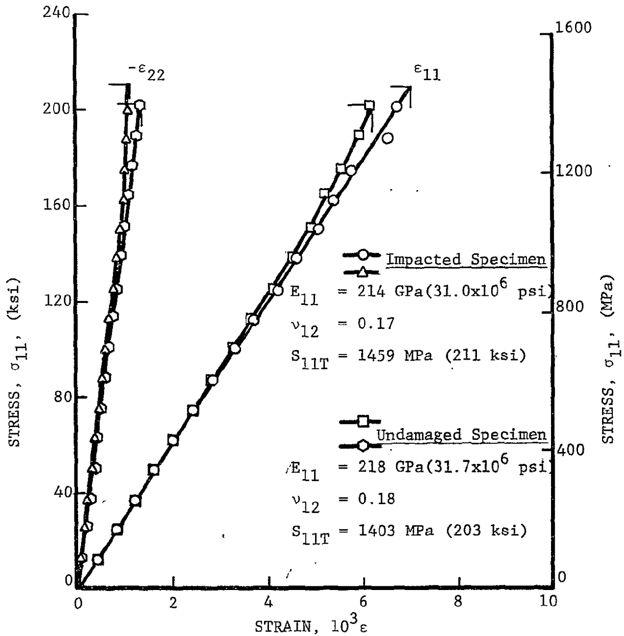
Fig. 42 STRAINS IN [0] 16 BORON/EPOXY SPECIMENS UNDER UNIAXIAL TENSION FROM UNDAMAGED AND IMPACTED LAMINATES (Impact Velocity: 210 ms -1 ; 690 ft/sec)
