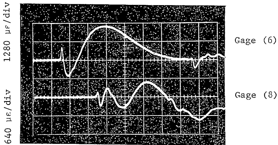
(b) 20 \mu\text{sec}/\text{div}
