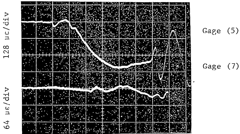
(a) 20 \mu\text{sec}/\text{div}
