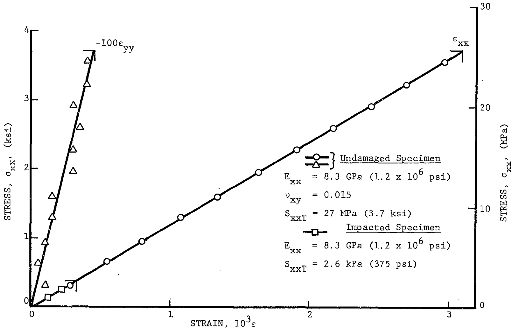
Fig. 47 STRAINS IN [90_{16}] GRAPHITE/EPOXY SPECIMENS UNDER UNIAXIAL TENSION FROM UNDAMAGED AND IMPACTED LAMINATES (Impact Velocity: 192 \text{ ms}^{-1} ; 630 \text{ ft/sec} )
