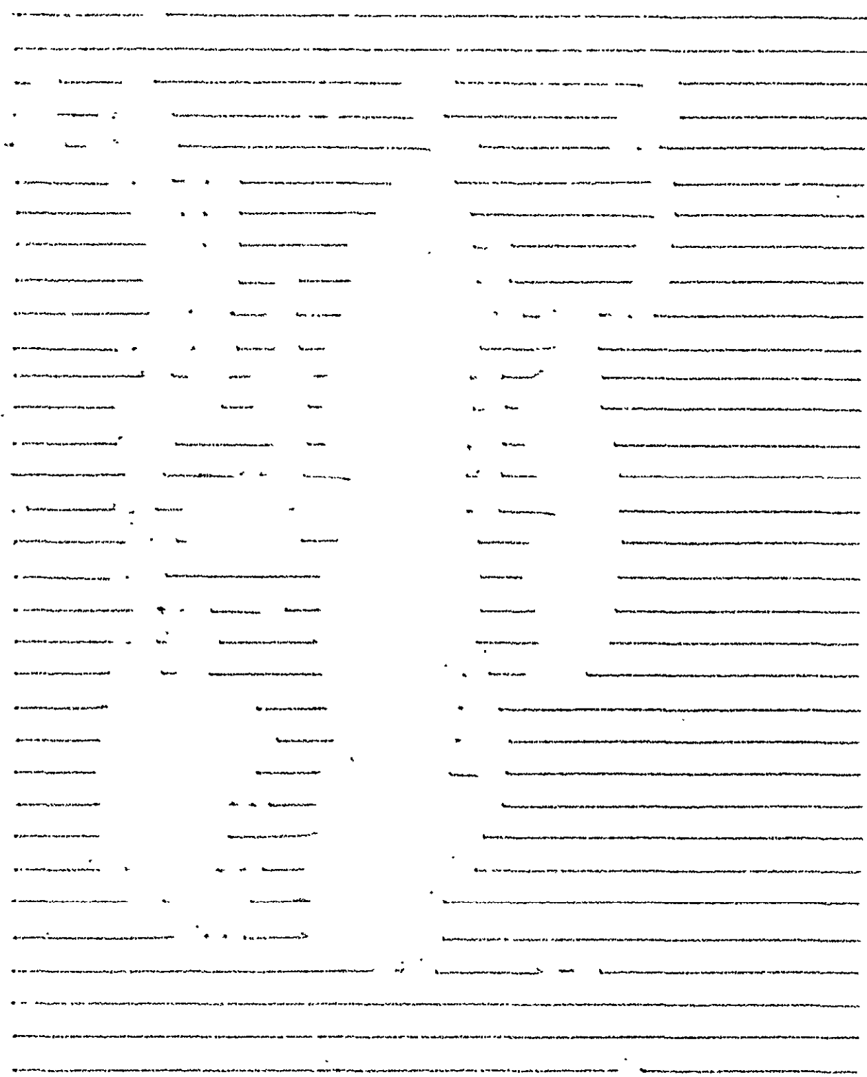
Fig. 17 ULTRASONIC SCAN OF [0_{16}] BORON/EPOXY SPECIMEN AFTER IMPACT TESTING (Specimen 9BU-1)
