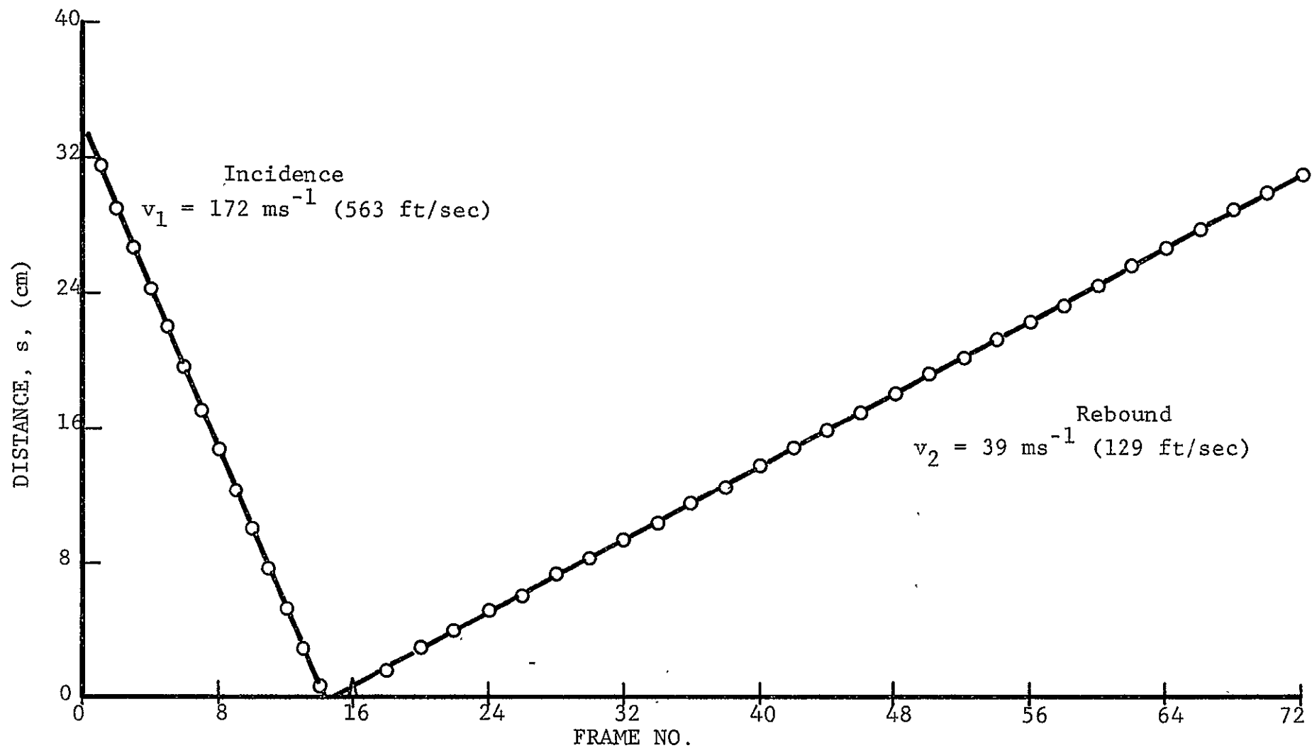
Fig. 59 PROJECTILE DISTANCE FROM IMPACTED PLATE AS A FUNCTION OF FRAME NUMBER (Barrel Pressure: 207 kPa, 30 psi; Plate: [0 2 /+45]2 s Graphite/Epoxy; 137 \mu s/frame)
