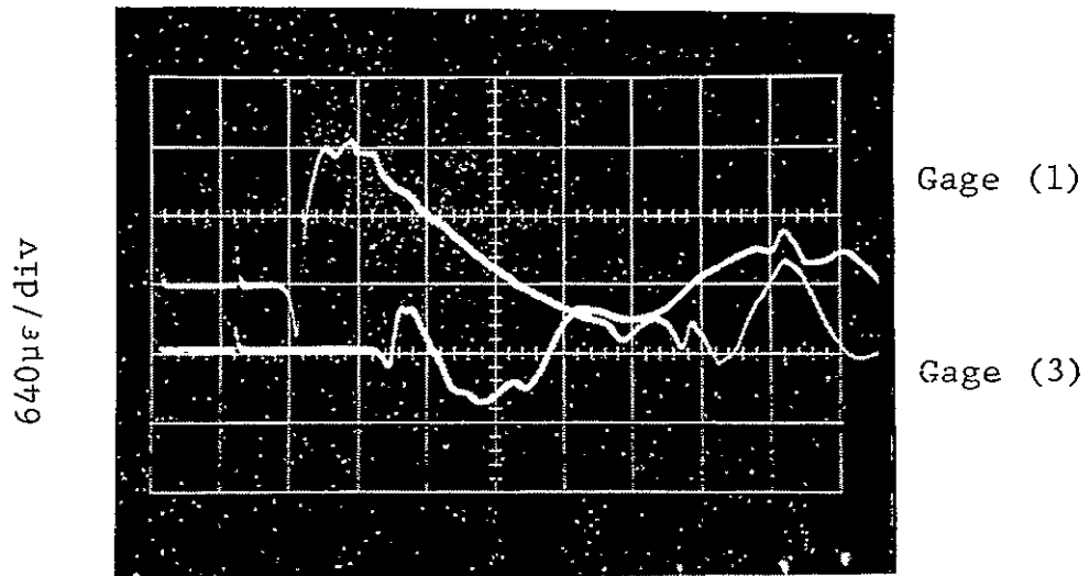
(a) 20\mu\text{sec}/\text{div}
