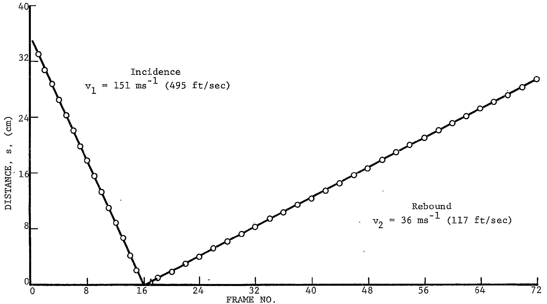
Fig. 58 PROJECTILE DISTANCE FROM IMPACTED PLATE AS A FUNCTION OF FRAME NUMBER (Barrel Pressure: 138 kPa, 20 psi; Plate: [0_2/+45]_2 s Graphite/Epoxy; 146 \mu s/frame)
