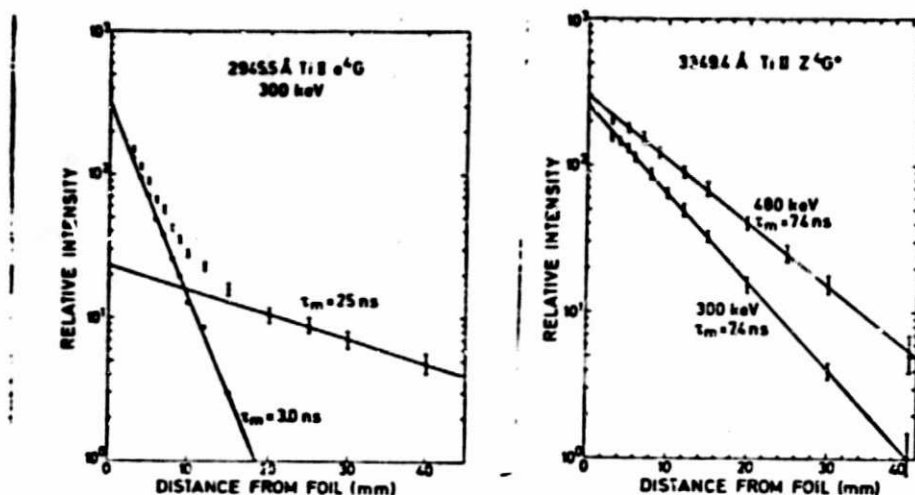
Fig. 7. Beam-foil lifetime data for two different levels in Ti II. After Roberts et al. (Ref. 5).
