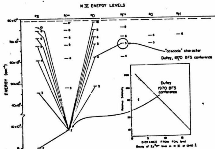
Fig. 11. Beam-foil decay data for a level in N V. After Dufay et al. (Ref. 8).
