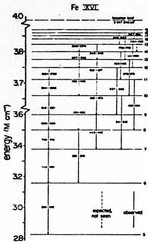
Fig. 2. Transitions in Fe XVI. Observed transitions (solid), expected but unobserved transitions (dashed). Transition wavelengths are indicated.
