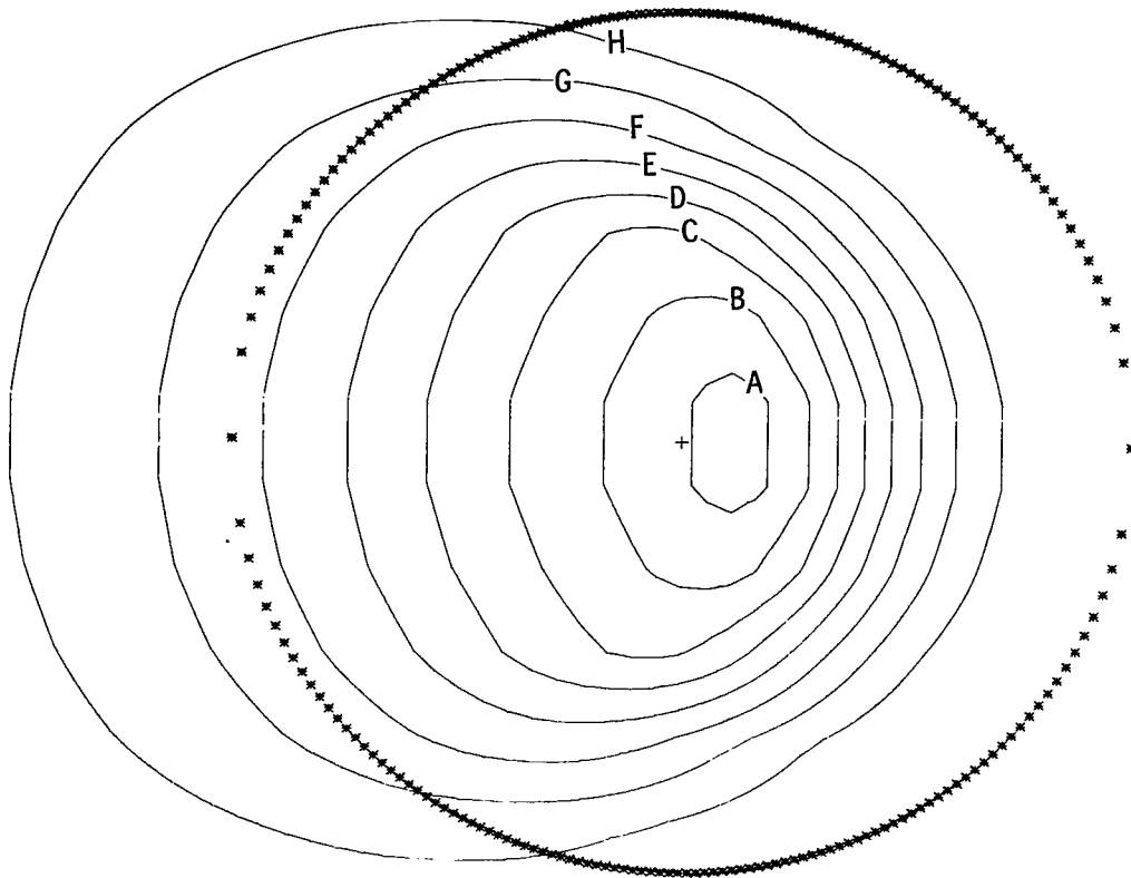
Figure 7. - Contour plots of dimensionless pressure for dimensionless load parameters W of 0.1106 \times 10^{-6} and 0.1290 \times 10^{-5} , respectively. The dimensionless parameters k , U , and G are held constant as defined in equation (18).
