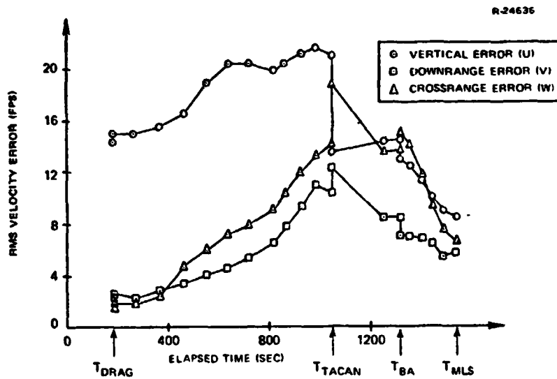
Figure 4.4-1b Overall Performance Down to 20,000 ft: Velocity
