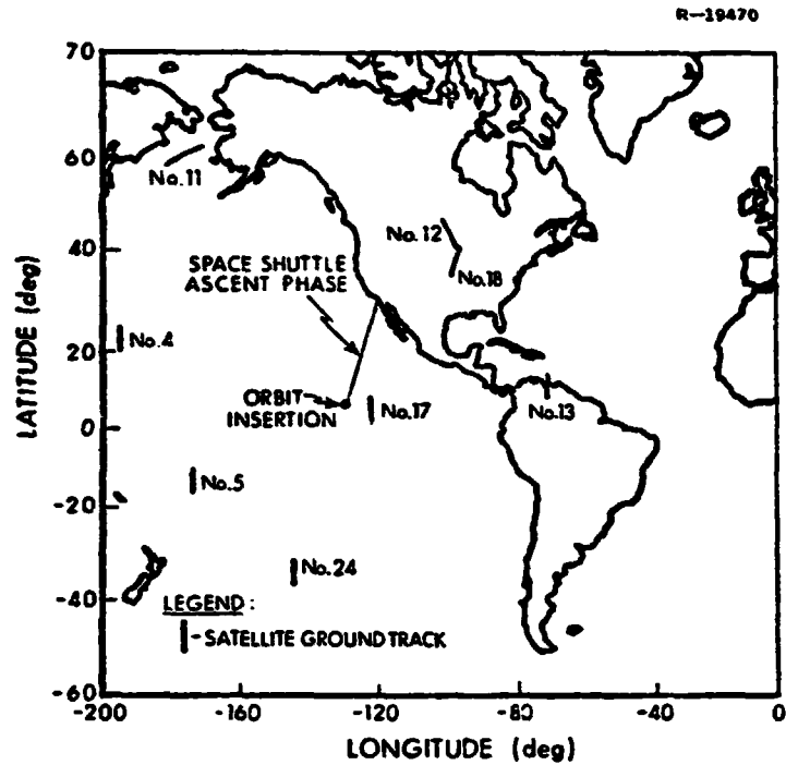
Figure 2.2-1 Baseline GPS Satellite Coverage (Space Shuttle Ascent Phase)
