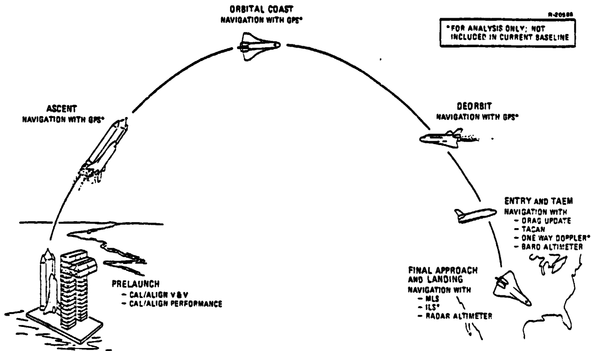
Figure 1-1 Summary of TASC Studies Relative to Space Shuttle Navigation (1973-1976)
