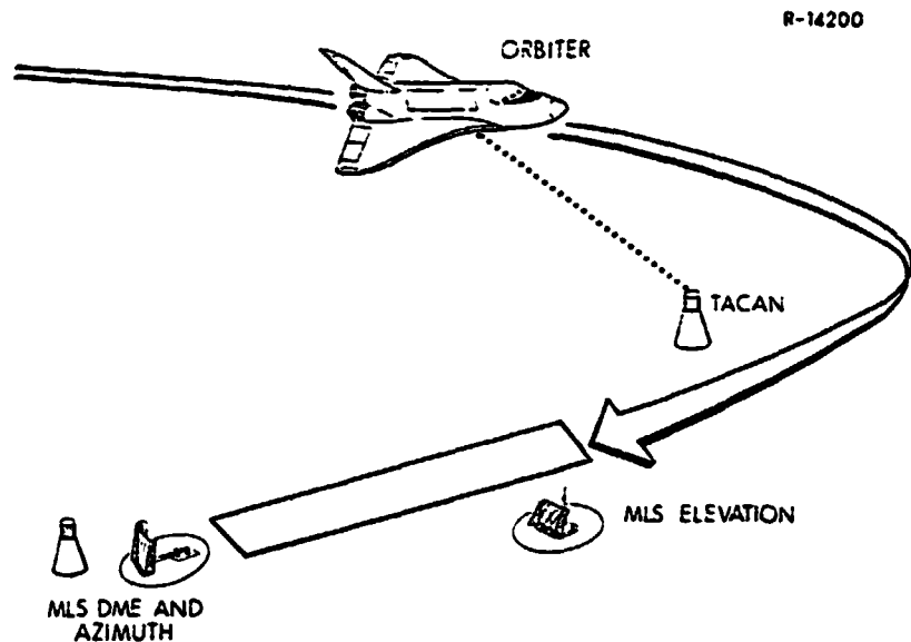
Figure 1.1-2 Baseline Orbiter Radio Navigation Aids
