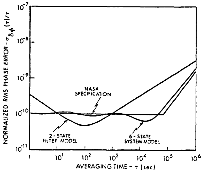
Figure 2.4-1 Normalized RMS Phase Error for Quartz Crystal Clock Model (Assuming Zero Acceleration)
