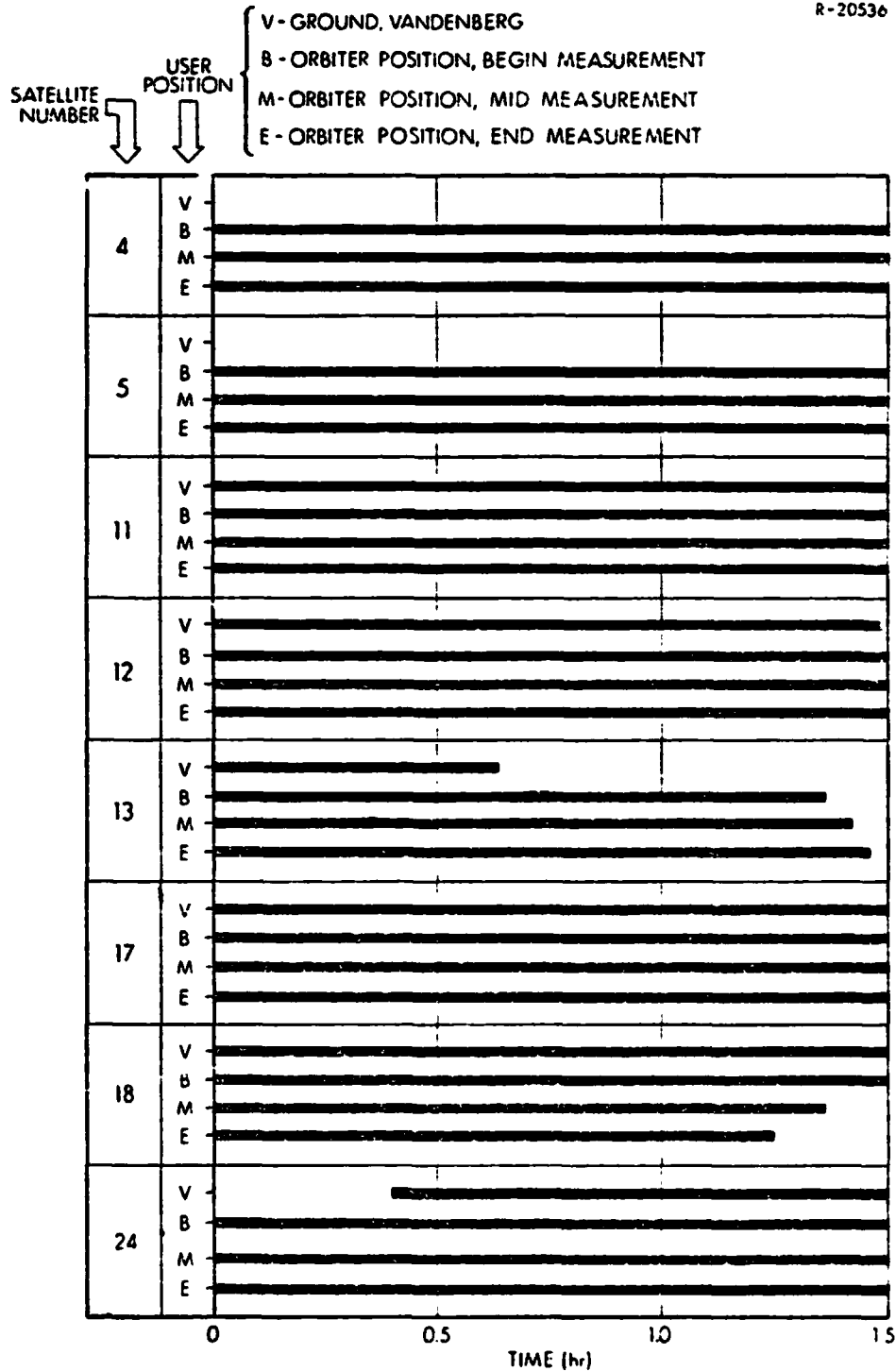
Figure 2.2-3 Satellite Visibility Versus Time from Four User Positions
