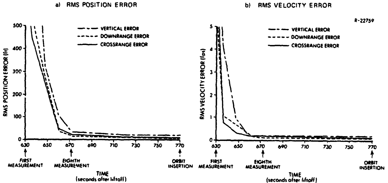
Figure 2.5-1 GPS-Aided Ascent Navigation: Overall Performance
