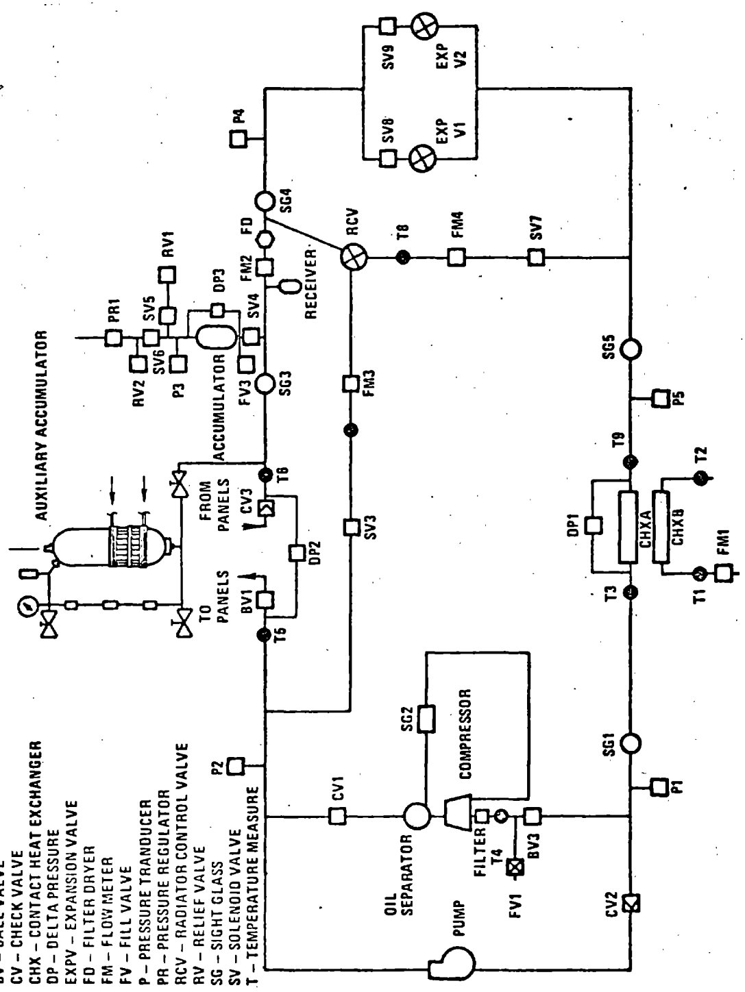
FIGURE 4 PROTOTYPE TEST FLOW MODULE SCHEMATIC AND INSTRUMENTATION
