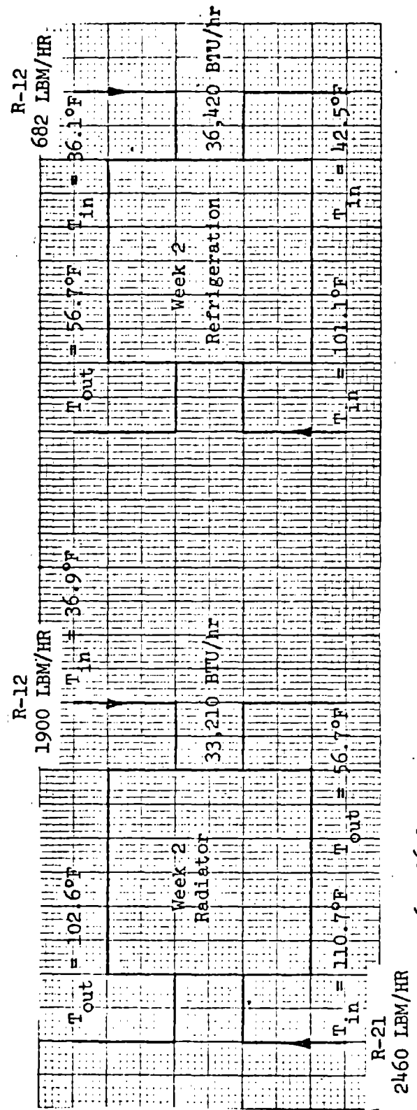
FIGURE 16 CONTACT HEAT EXCHANGER PERFORMANCE
