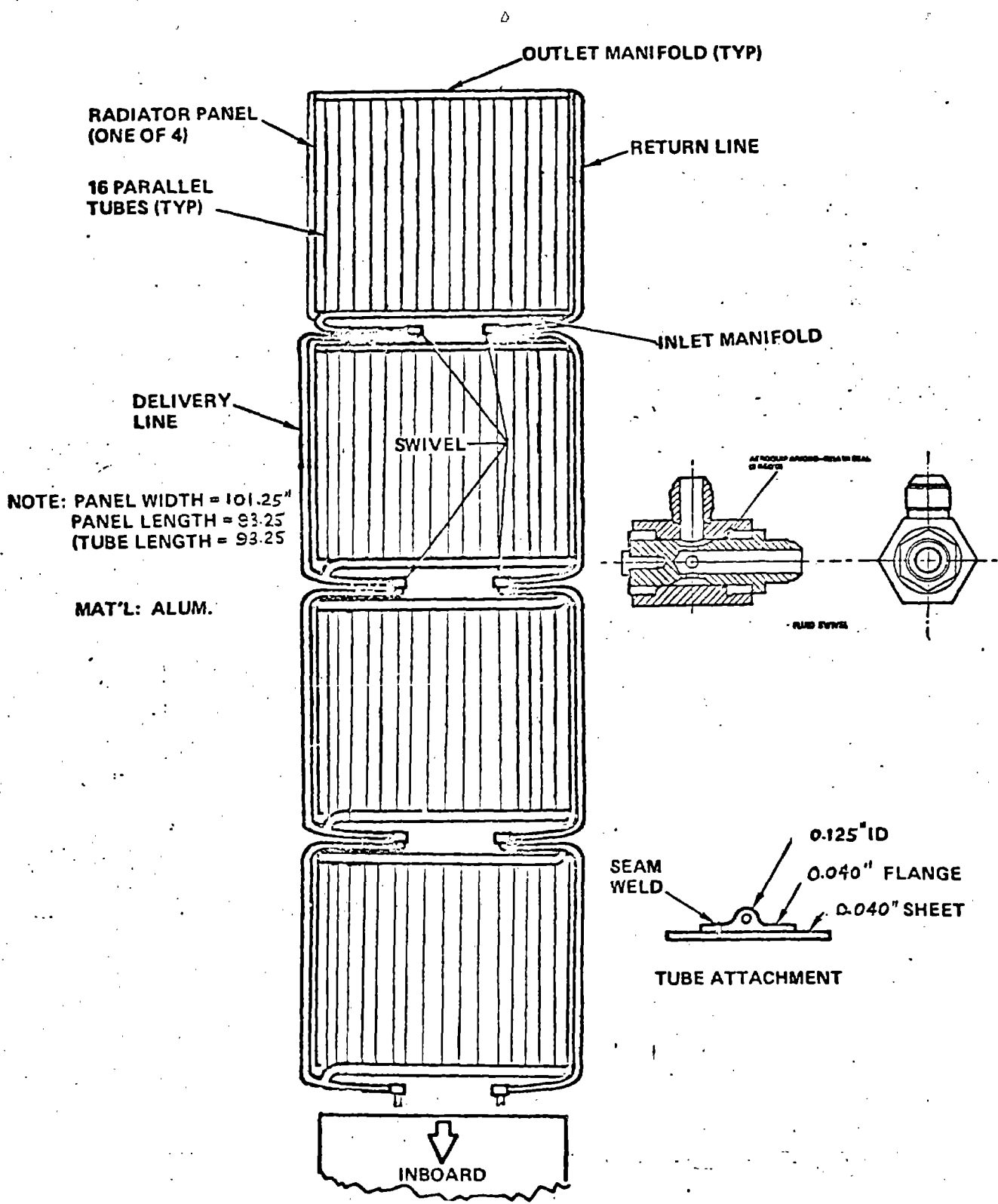
FIGURE 3 SHRM RADIATOR CONFIGURATION
