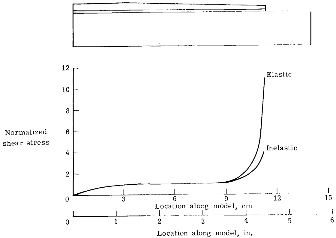
Figure 17.- Comparison of shear stresses in elastic and inelastic adhesive.
