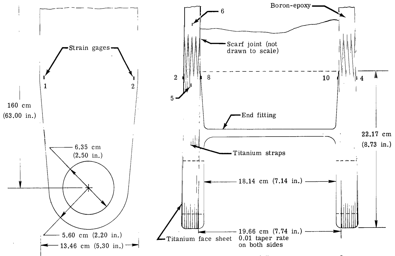
(c) Strain-gage location at boron-epoxy-titanium joints near ends of strut and general arrangement of drag strut ends at section B-B.
