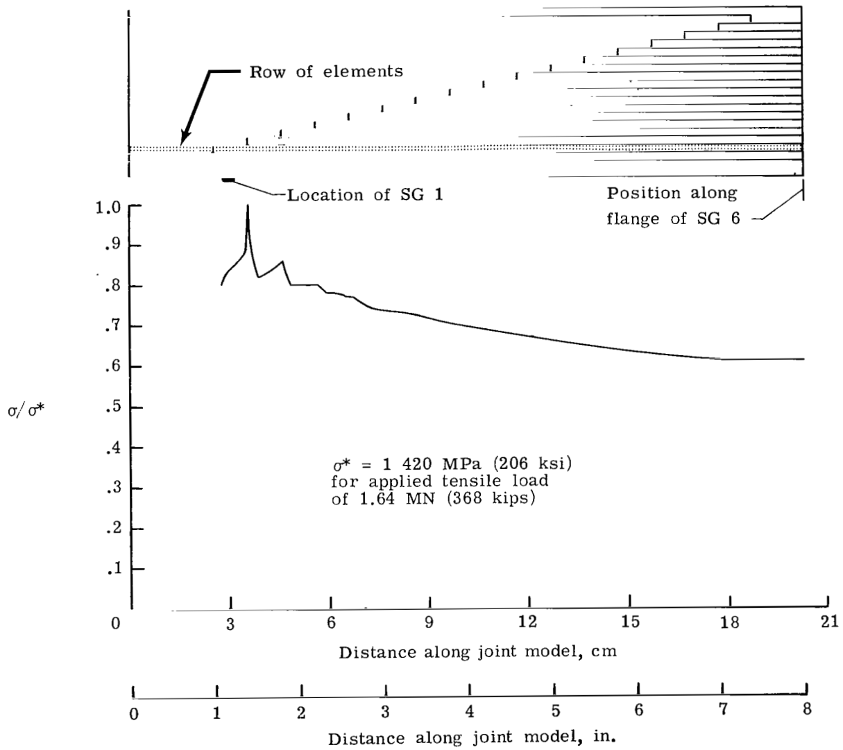
Figure 13.- Axial stress in first ply of boron fibers.
