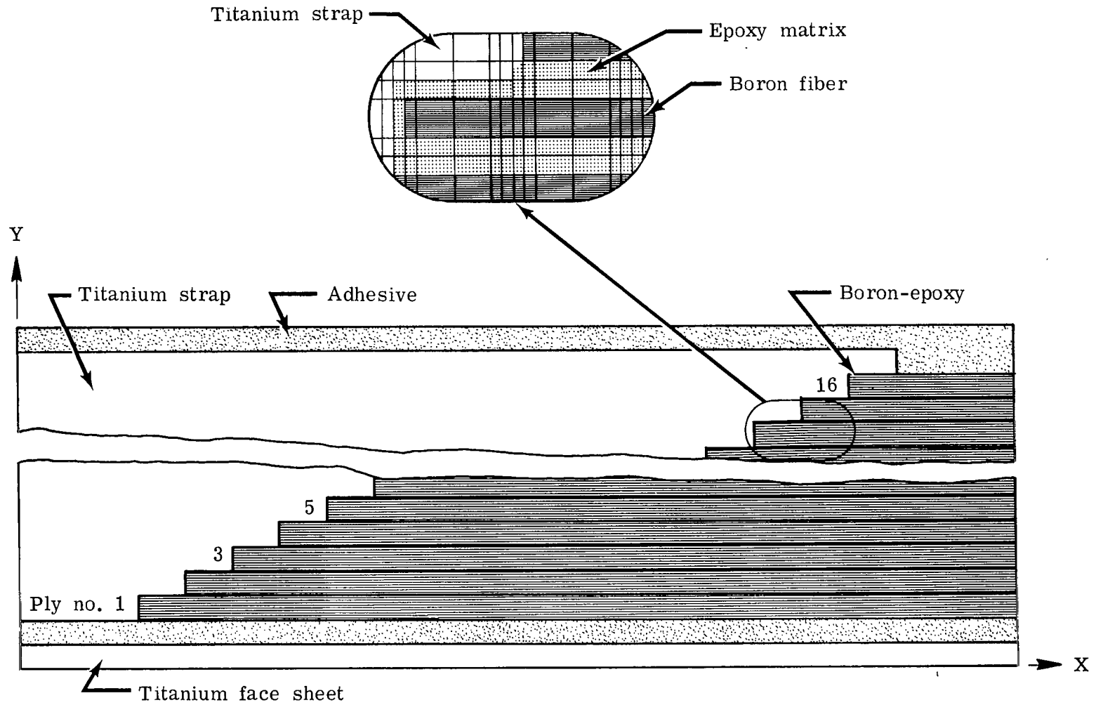
Figure 10.- Structural model used for analytical (NASTRAN®) study.
