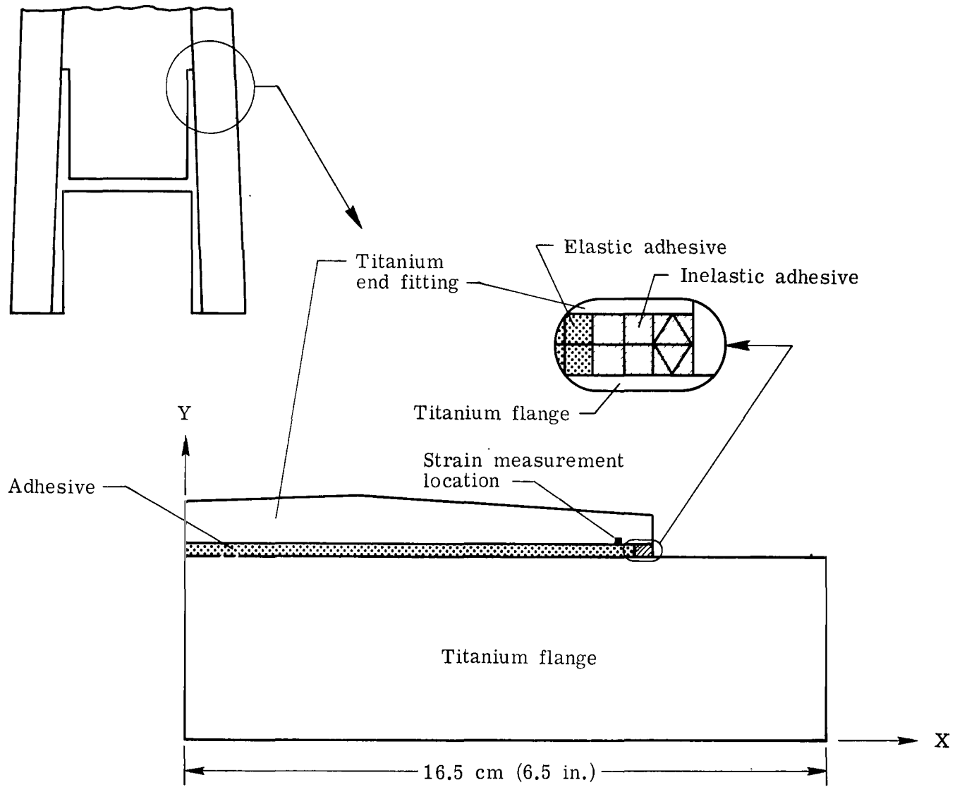
Figure 15.- Model used to evaluate effect of inelastic adhesive on strain of end fitting.
