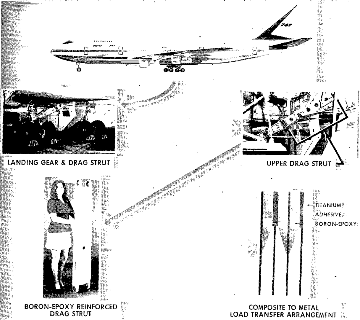
Figure 1.- Composite-reinforced drag strut for Boeing 747 transport.
