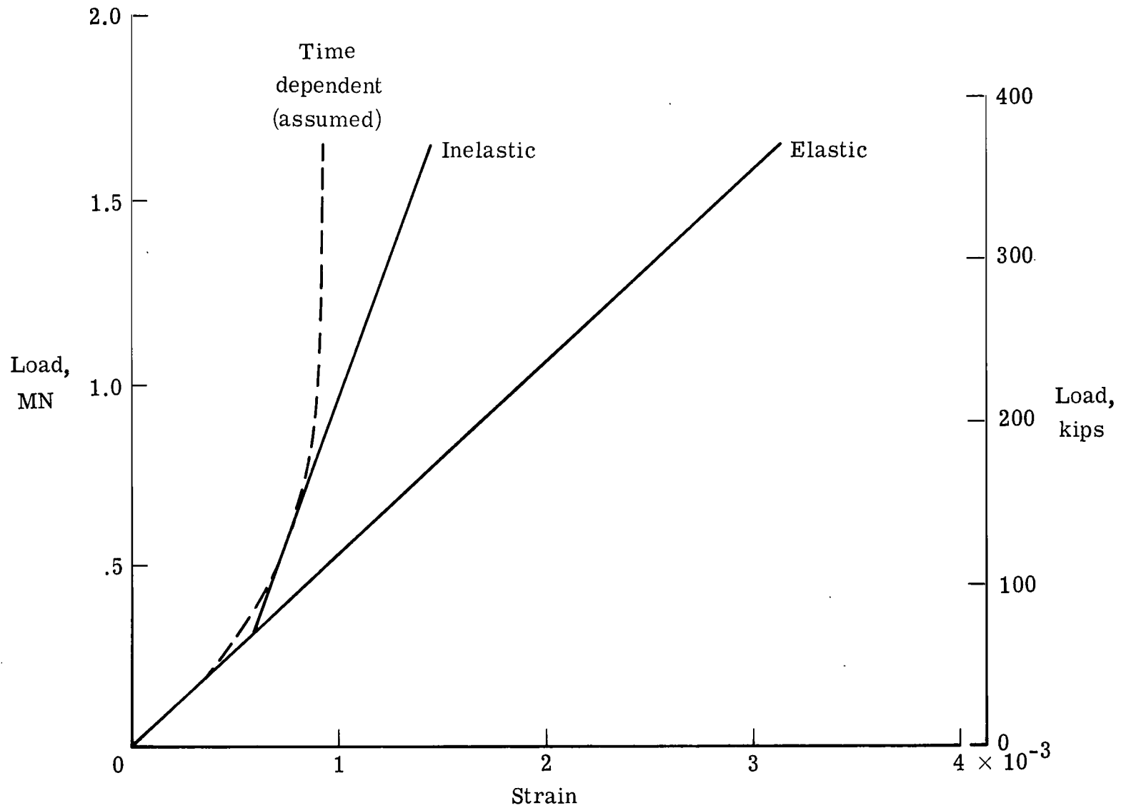
Figure 18.- Decrease in strain in titanium end fitting due to inelastic behavior of adhesive.
