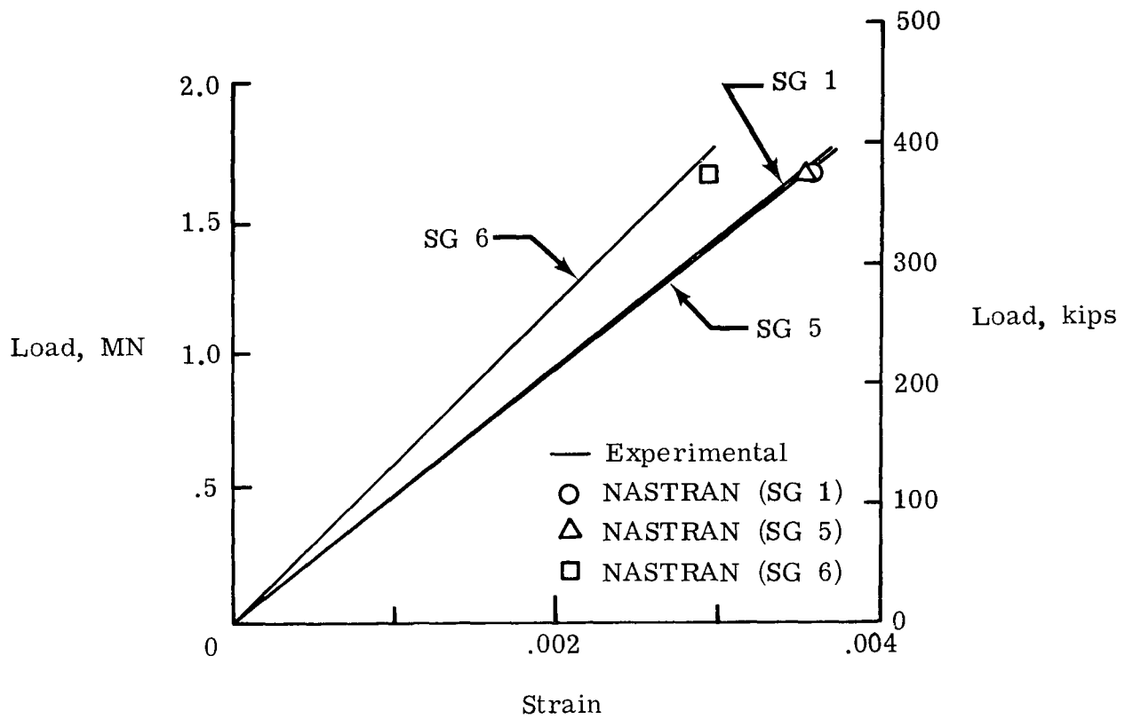
Figure 14.- Comparison of experimentally and analytically (NASTRAN®) determined strains.
