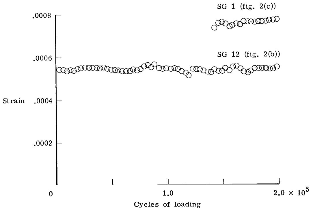
Figure 5.- Strain-gage data from fatigue test. Strains were recorded during a strain survey taken once every 3300 load cycles.
