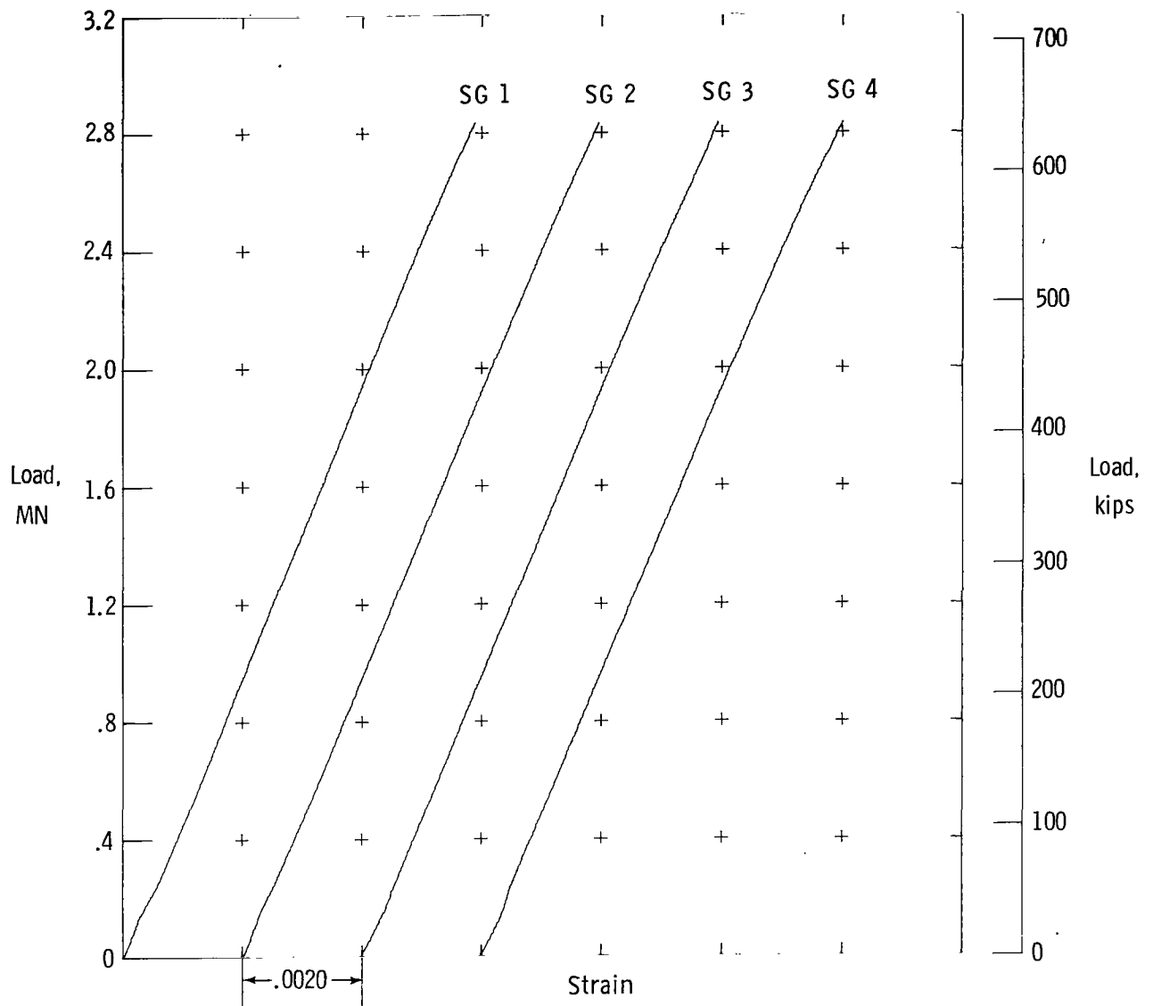
Figure 8.- Strain-gage data for compression design ultimate load (2.83 MN (636 kips)) for strain gages 1 to 4.
