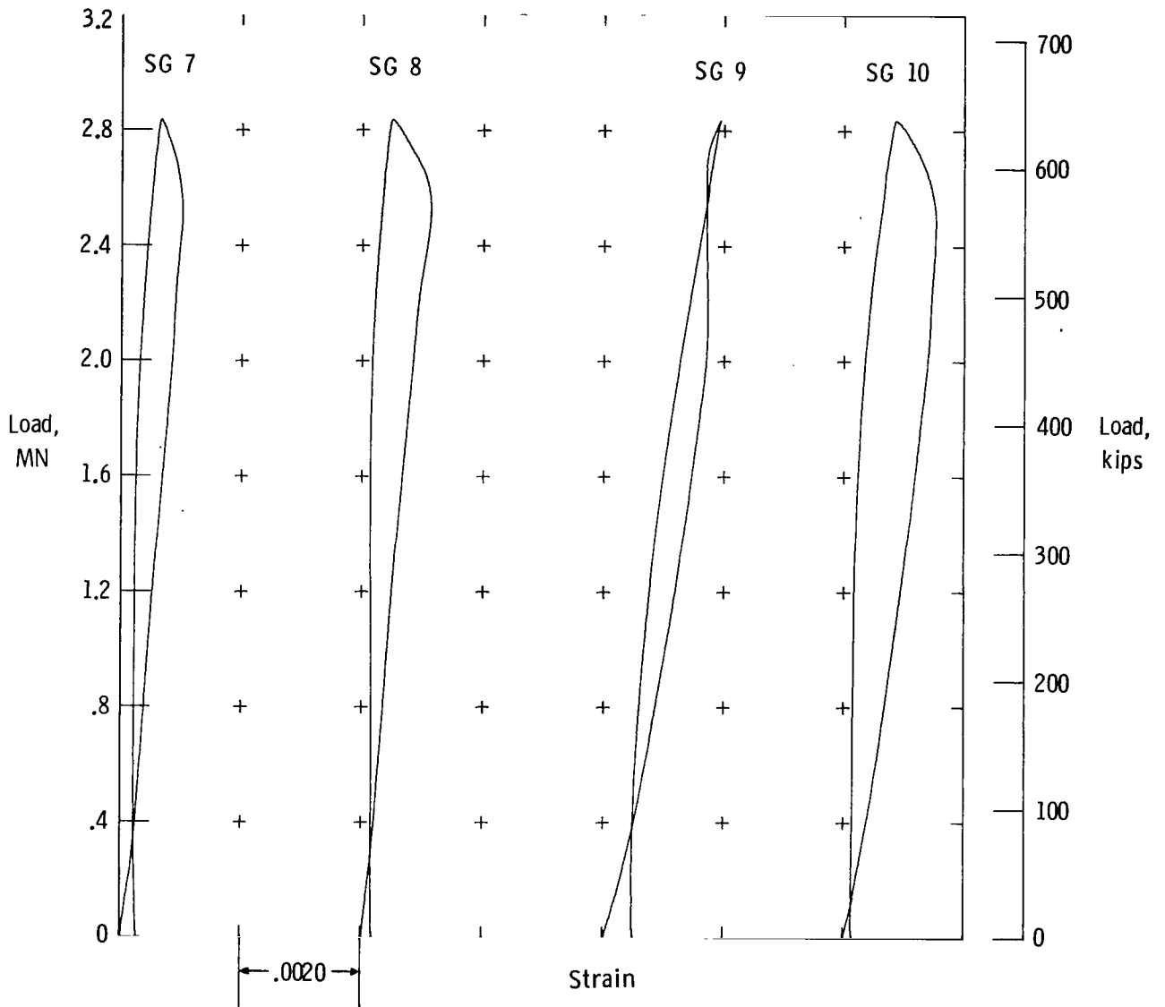
Figure 9.- Strain-gage data for compression design ultimate load (2.83 MN (636 kips)) for strain gages 7 to 10.
