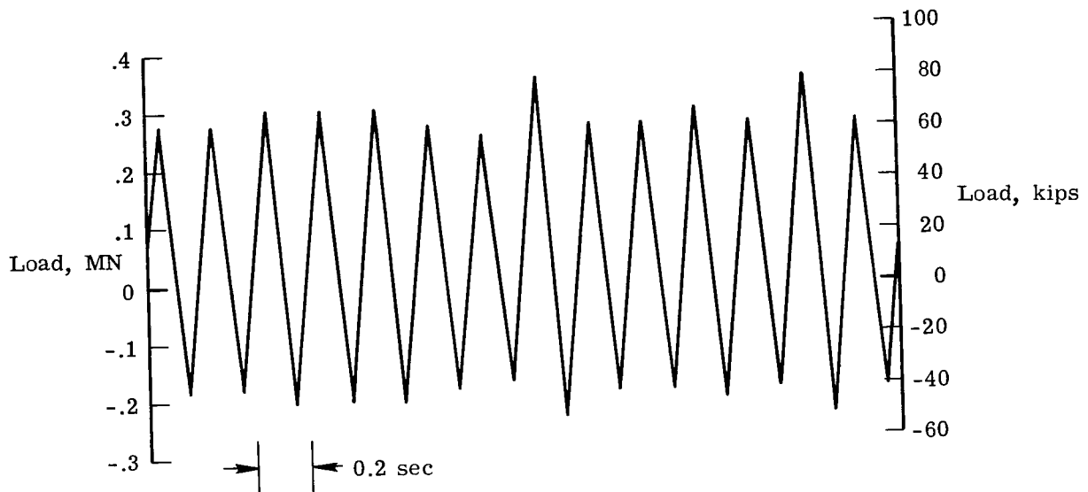
Figure 4.- Sample of fatigue loading.
