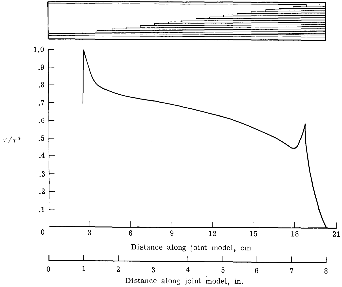
Figure 12.- Peak shear stress distribution along joint.
