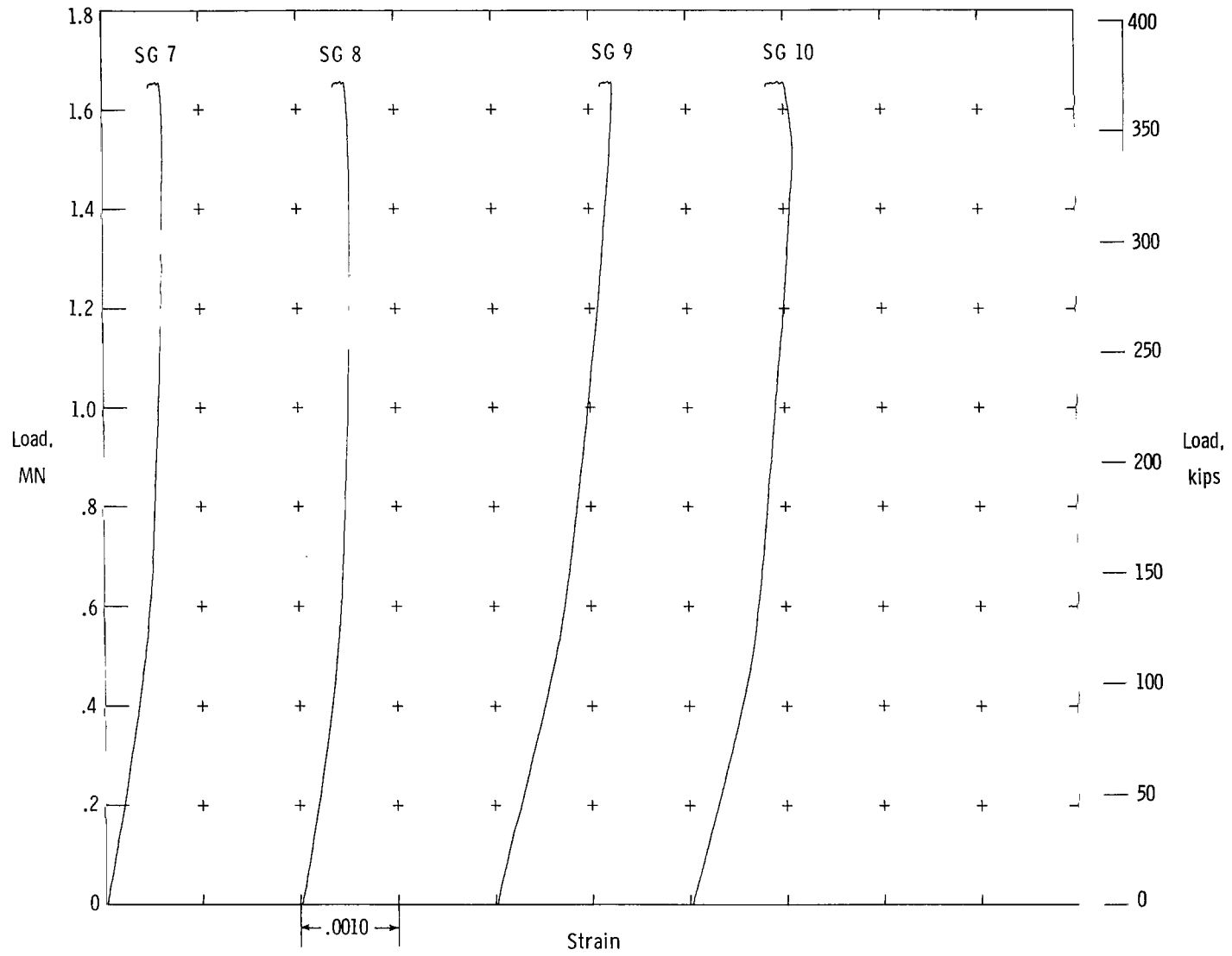
Figure 6.- Strain-gage data for tensile design ultimate load (1.64 MN (368 kips)).
