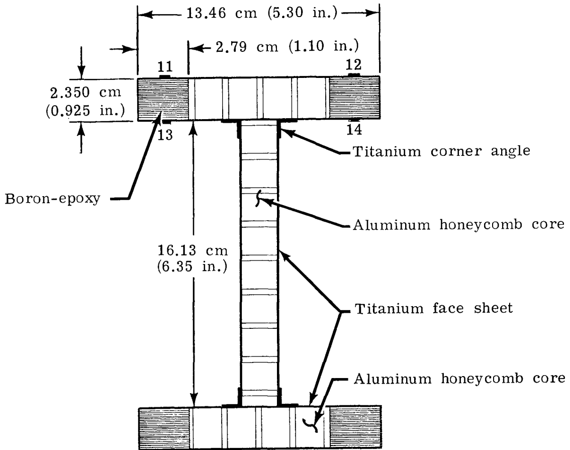
(b) Drag strut cross section at section A-A.
