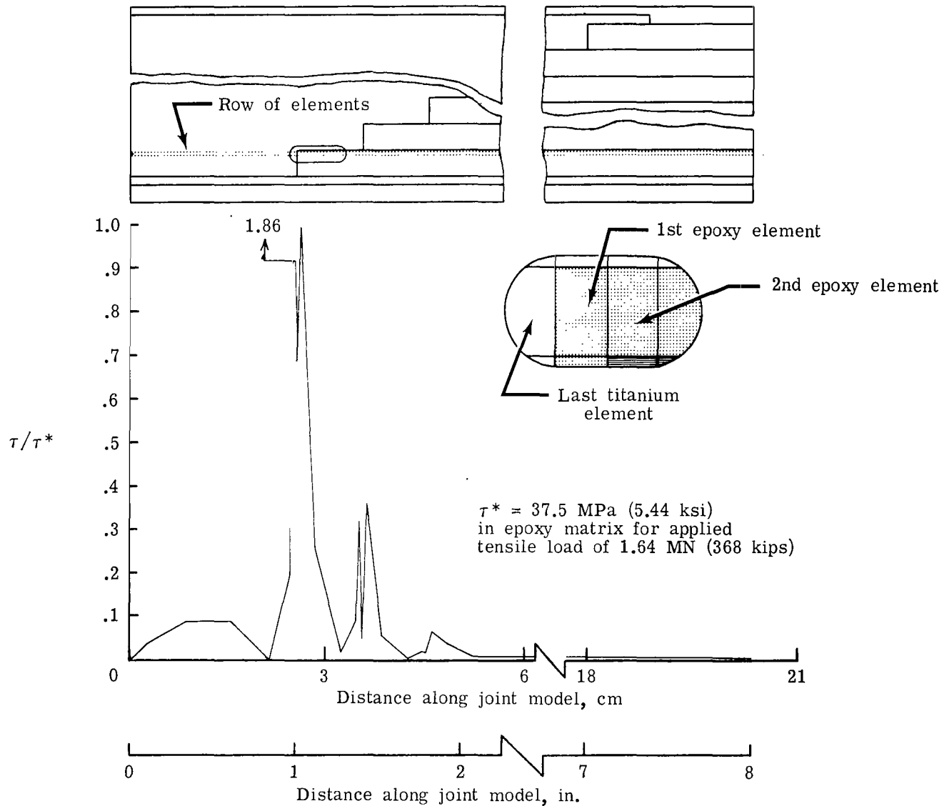
Figure 11.- Shear stress pattern of row of elements containing epoxy matrix of first ply of boron-epoxy.
