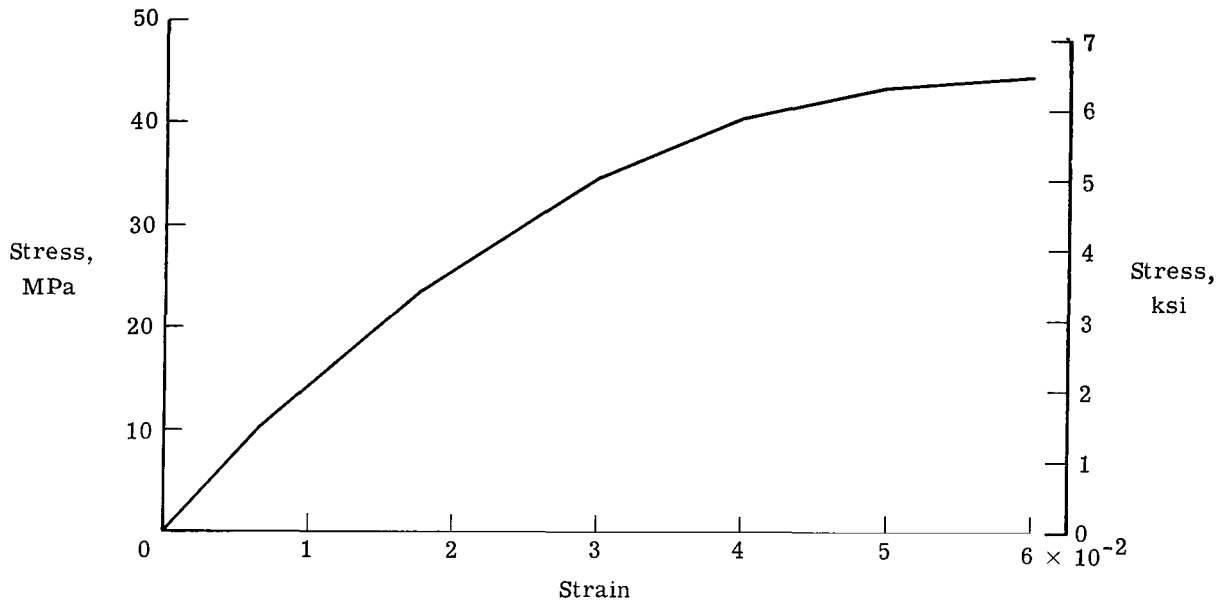
Figure 16.- Assumed stress-strain relationship for inelastic AF-126 adhesive.
