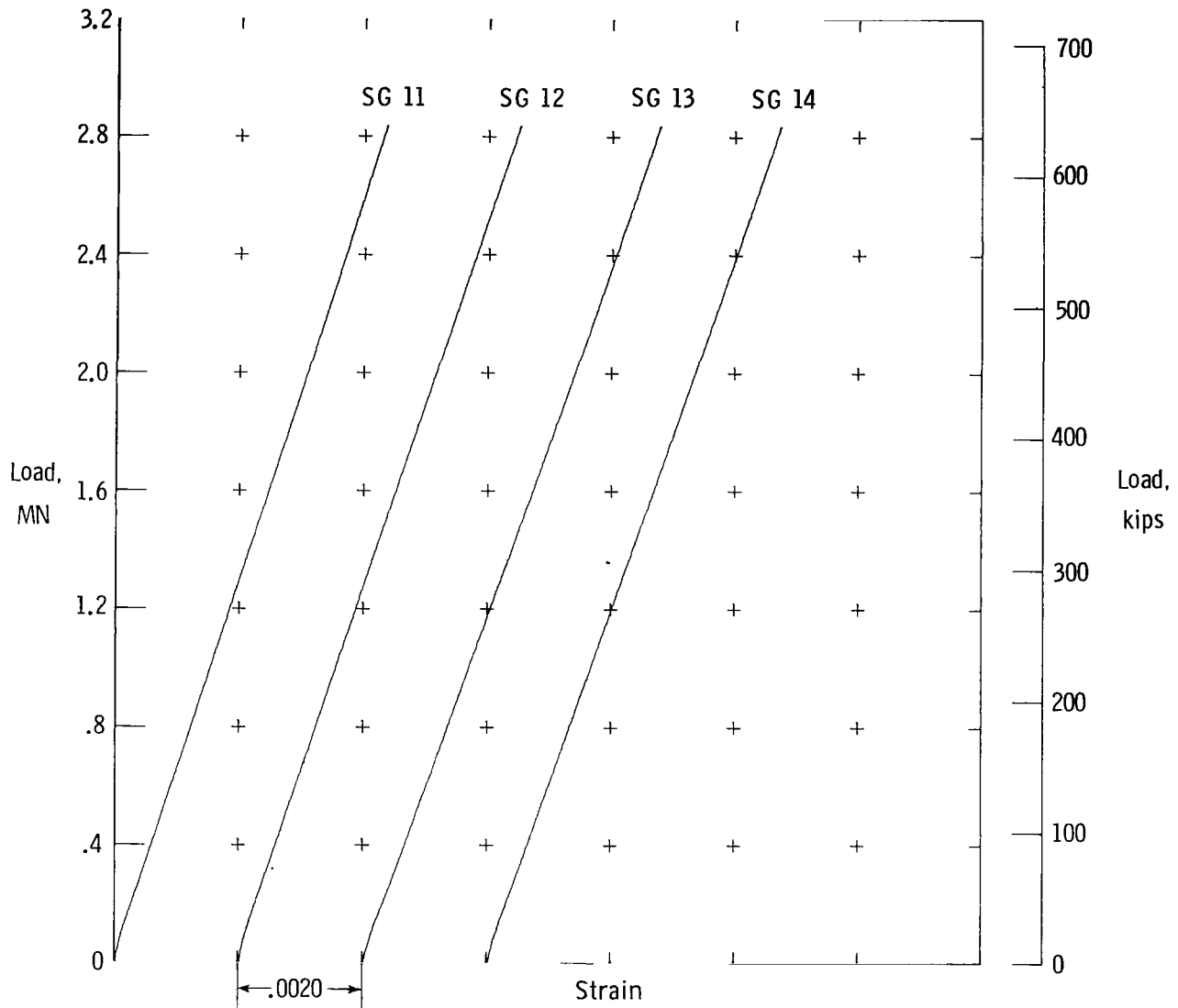
Figure 7.- Strain-gage data for compression design ultimate load (2.83 MN (636 kips)) for strain gages 11 to 14.
