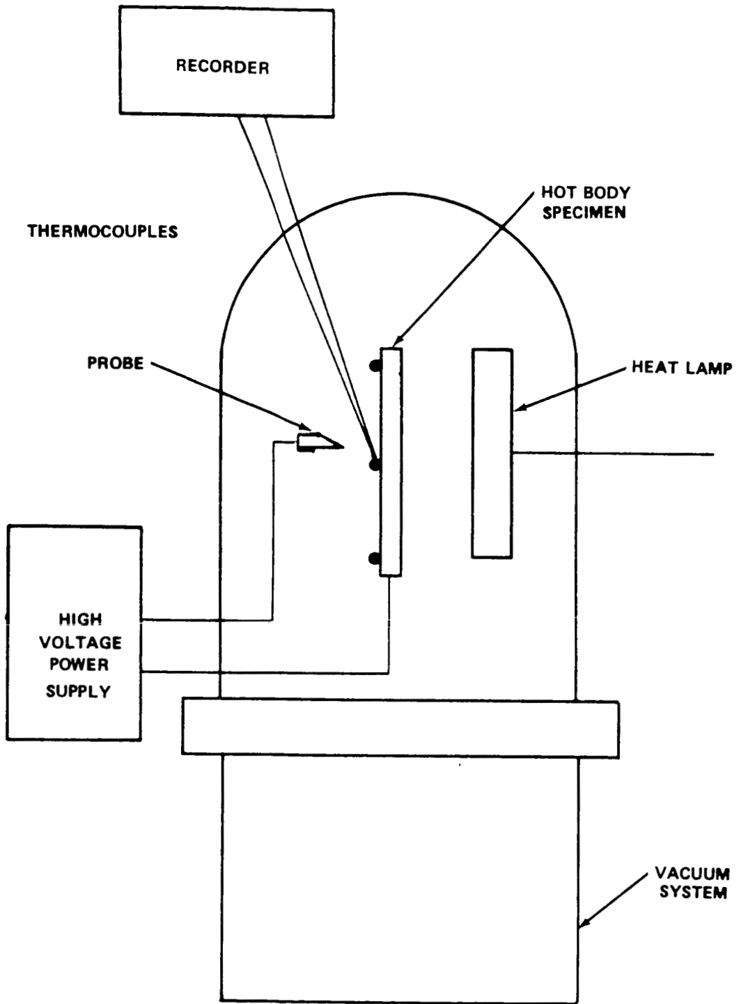
Figure 1. Test configuration.
