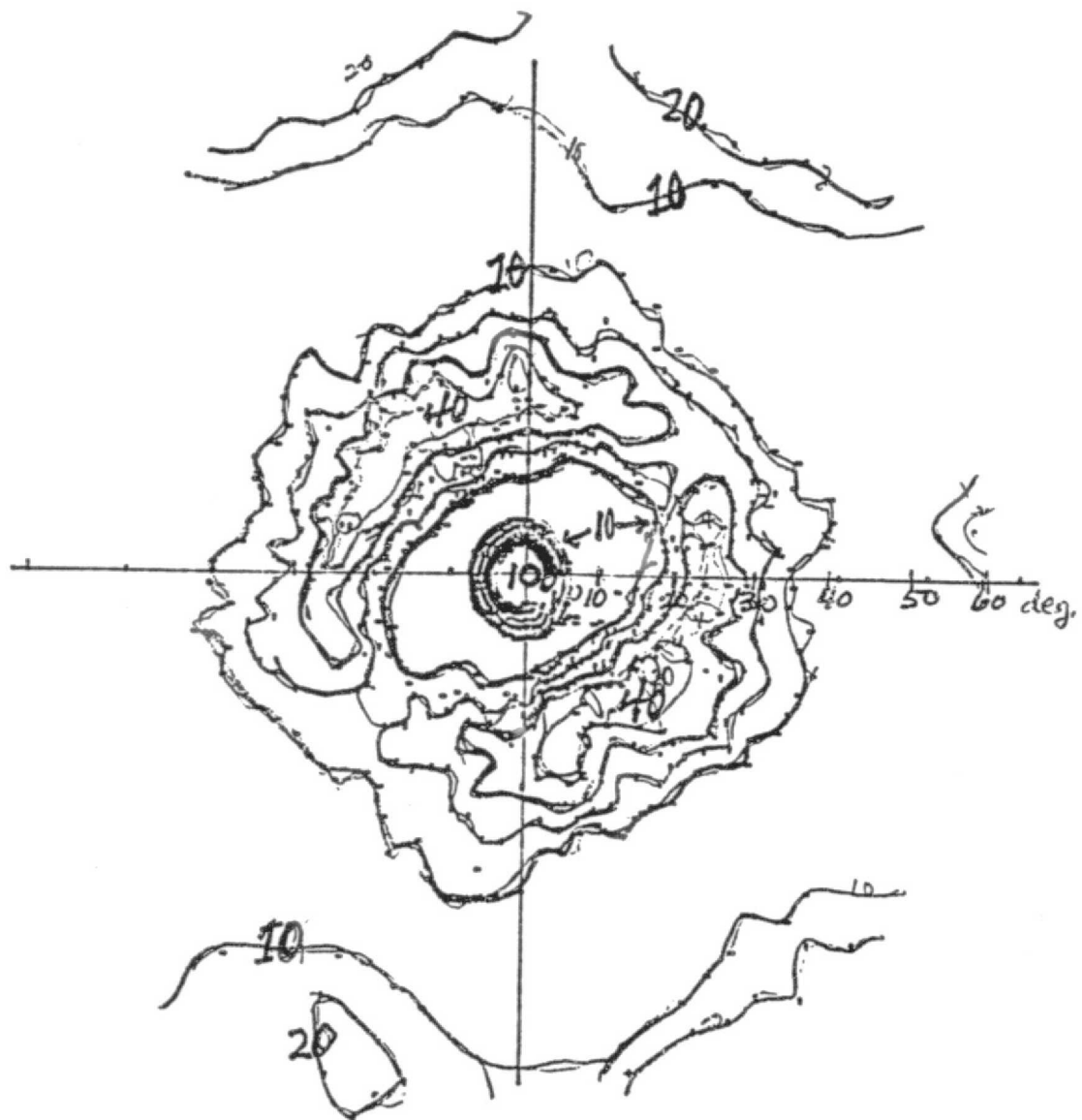
Figure 19 - (200) pole figure for slice from aluminum reference block.
