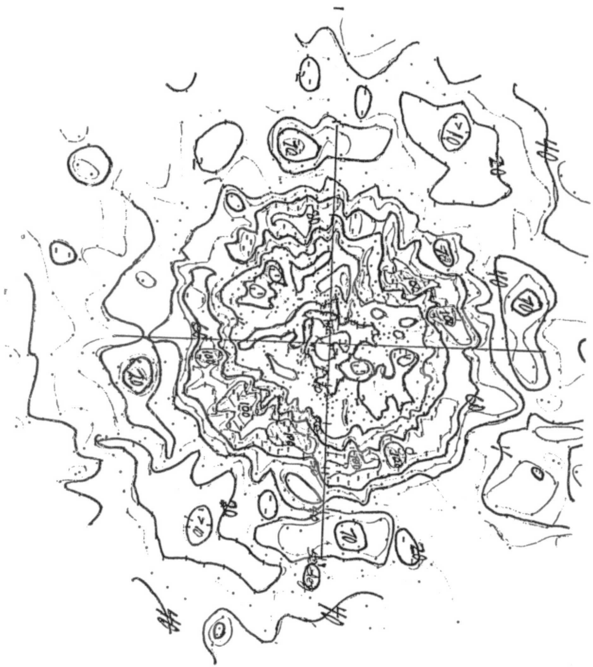
Figure 21 - (220) pole figure for slice from aluminum reference block.
