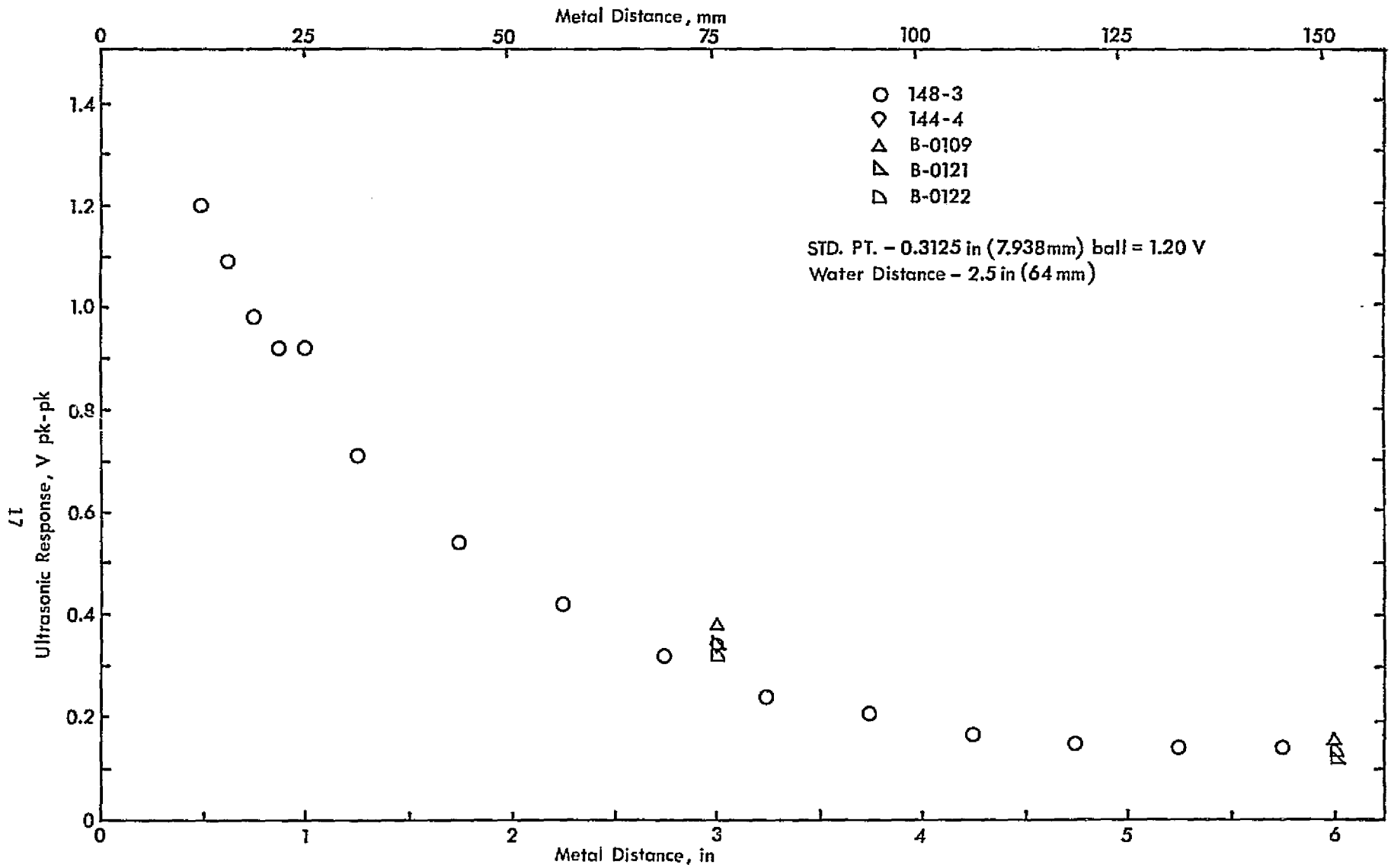
Figure 6 - Distance-amplitude data for No. 8 blocks at 2.25 MHz.
