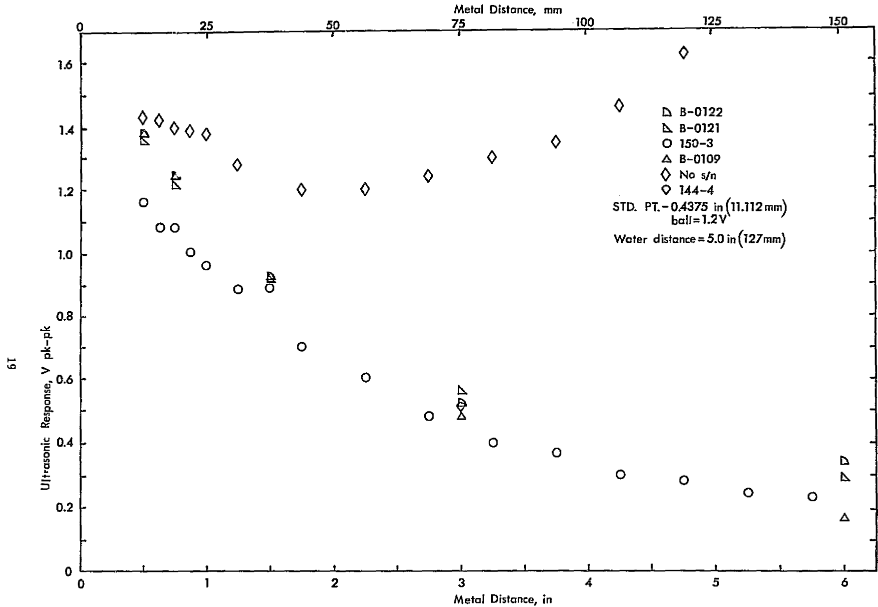
Figure 8 - Distance-amplitude data for No. 5 blocks at 5.0 MHz
