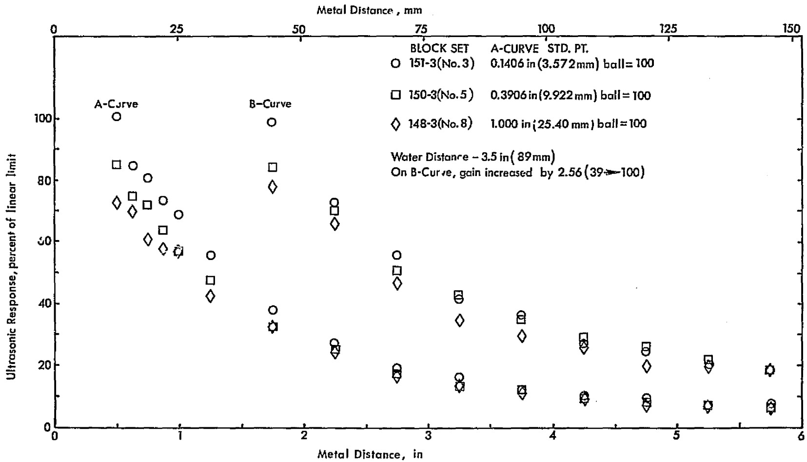
Figure 30- Universal distance-amplitude curves for three sets of aluminum reference blocks.
