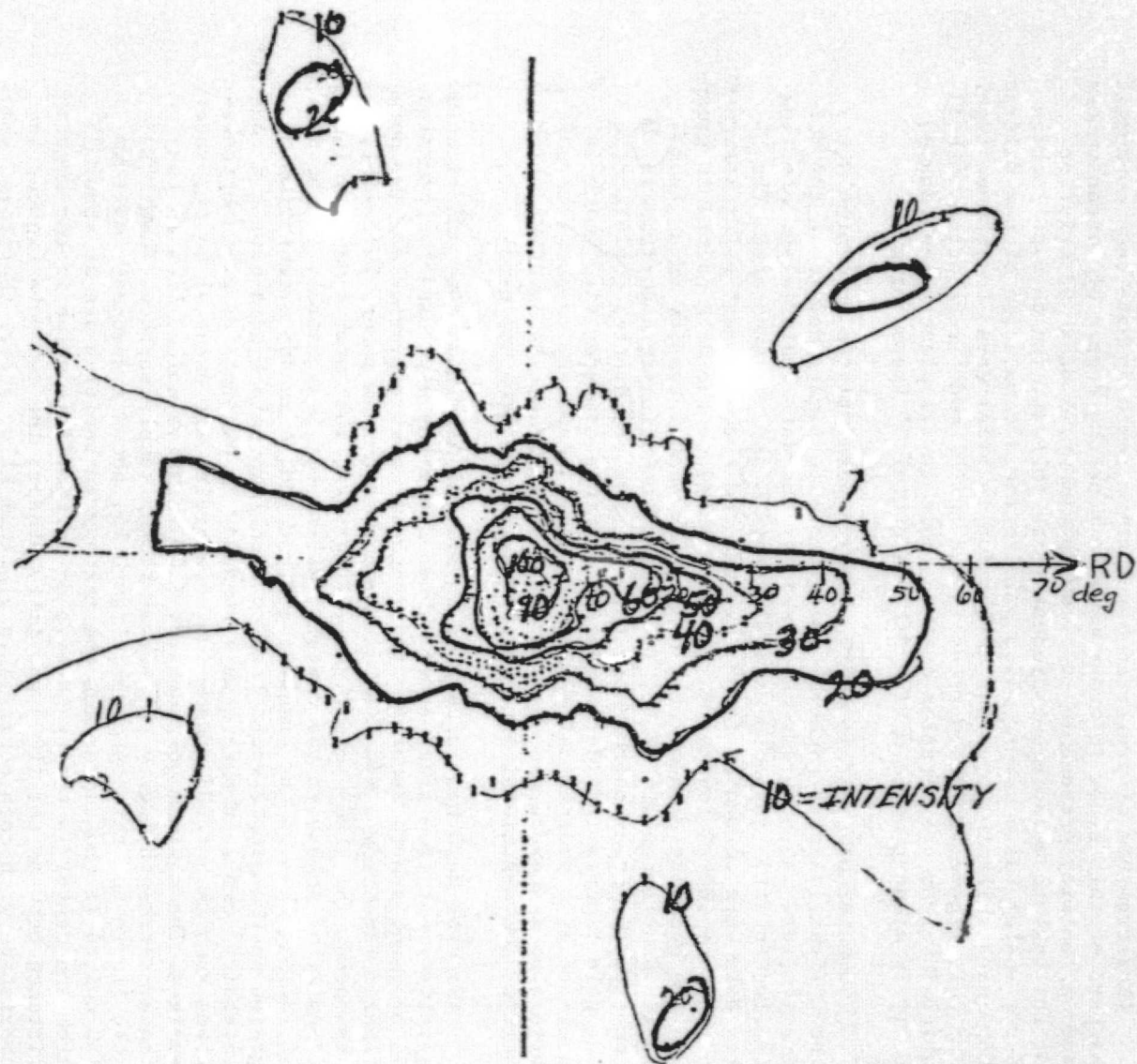
Figure 14 - (200) pole figure for 7075-T631 aluminum.
