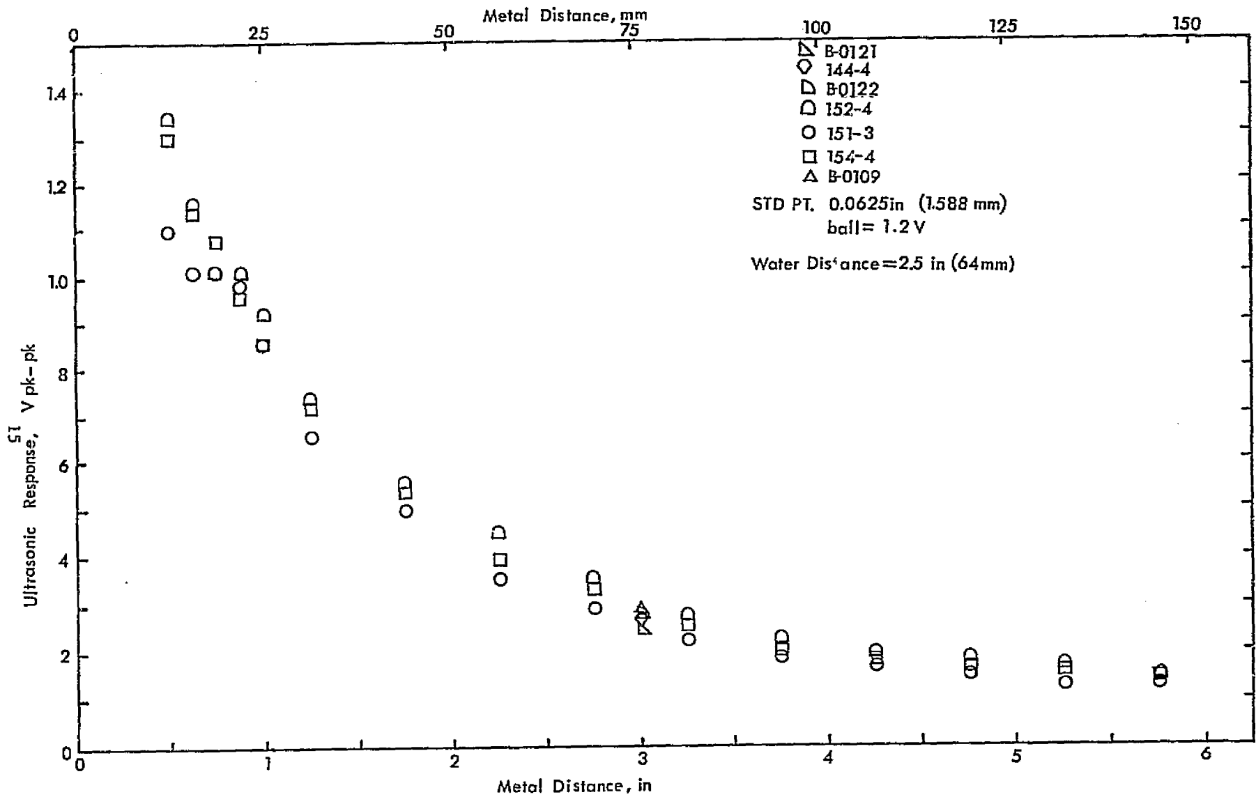
Figure 4 - Distance - amplitude data for No. 3 blocks at 2.25 MHz
