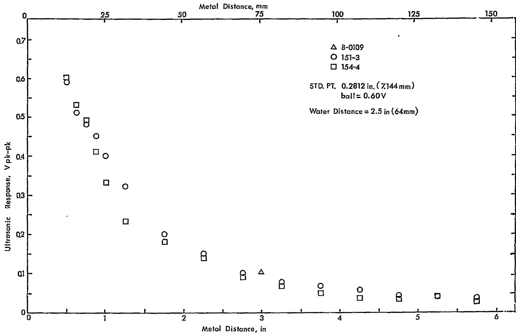
Figure 10 - Distance - amplitude data for No. 3 blocks at 10 MHz.
