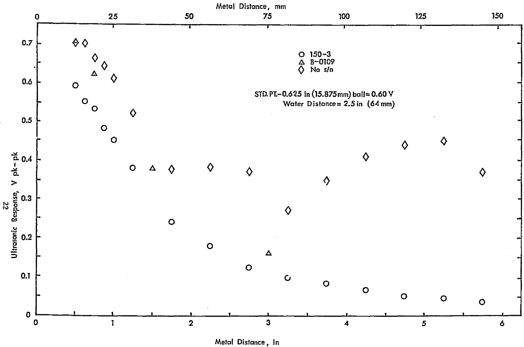
Figure 11 - Distance-amplitude data for No. 5 blocks at 10 MHz.
