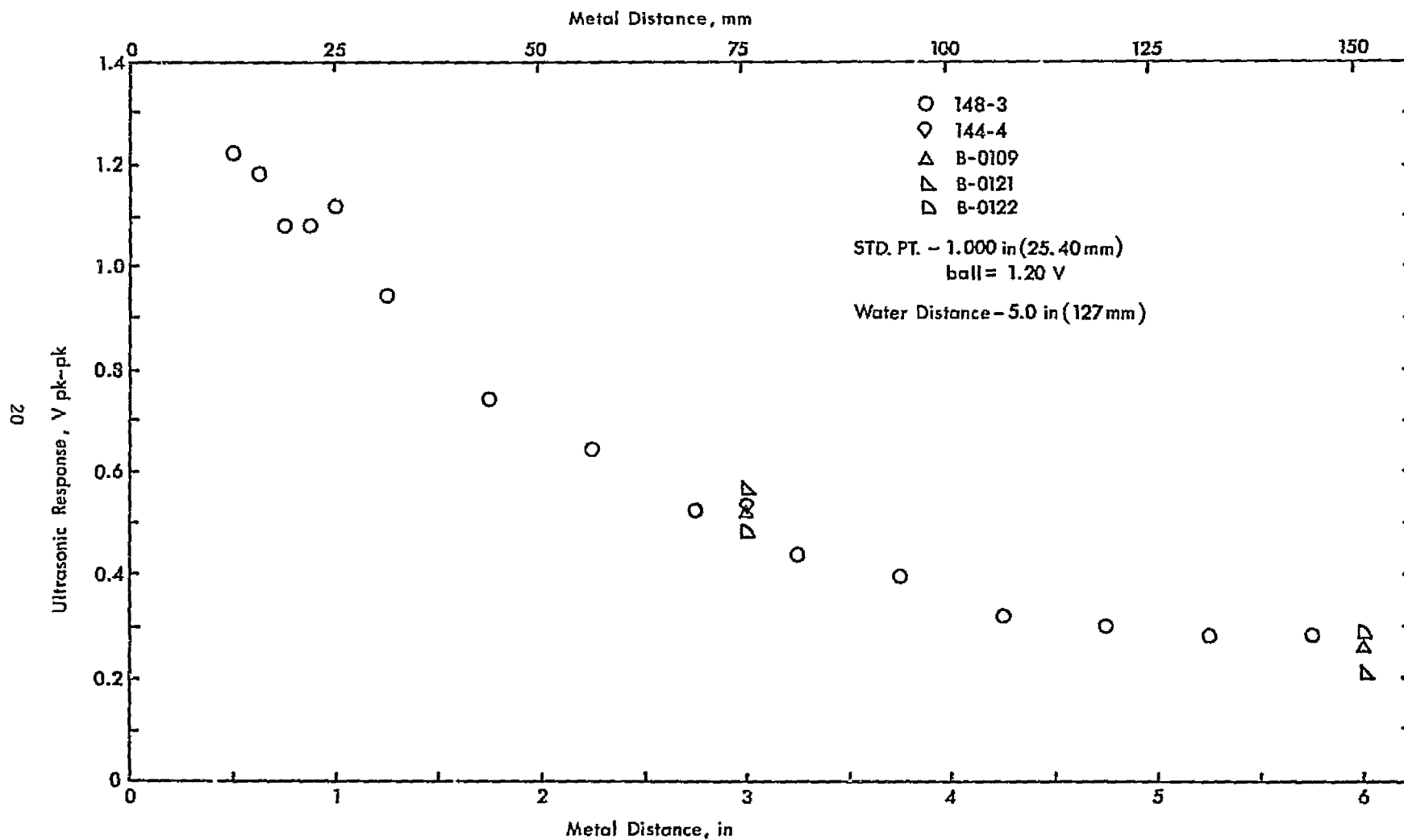
Figure 9 - Distance - amplitude data for No. 8 blocks at 5.0 MHz.
