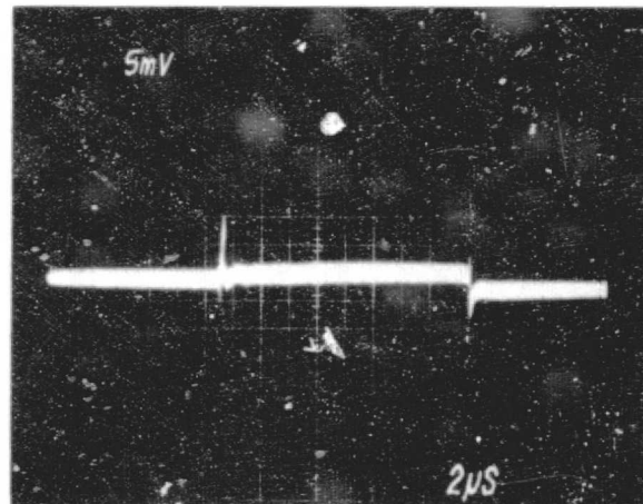
Figure A-2 - Typical "steps" (switching transients) in the gated output.
