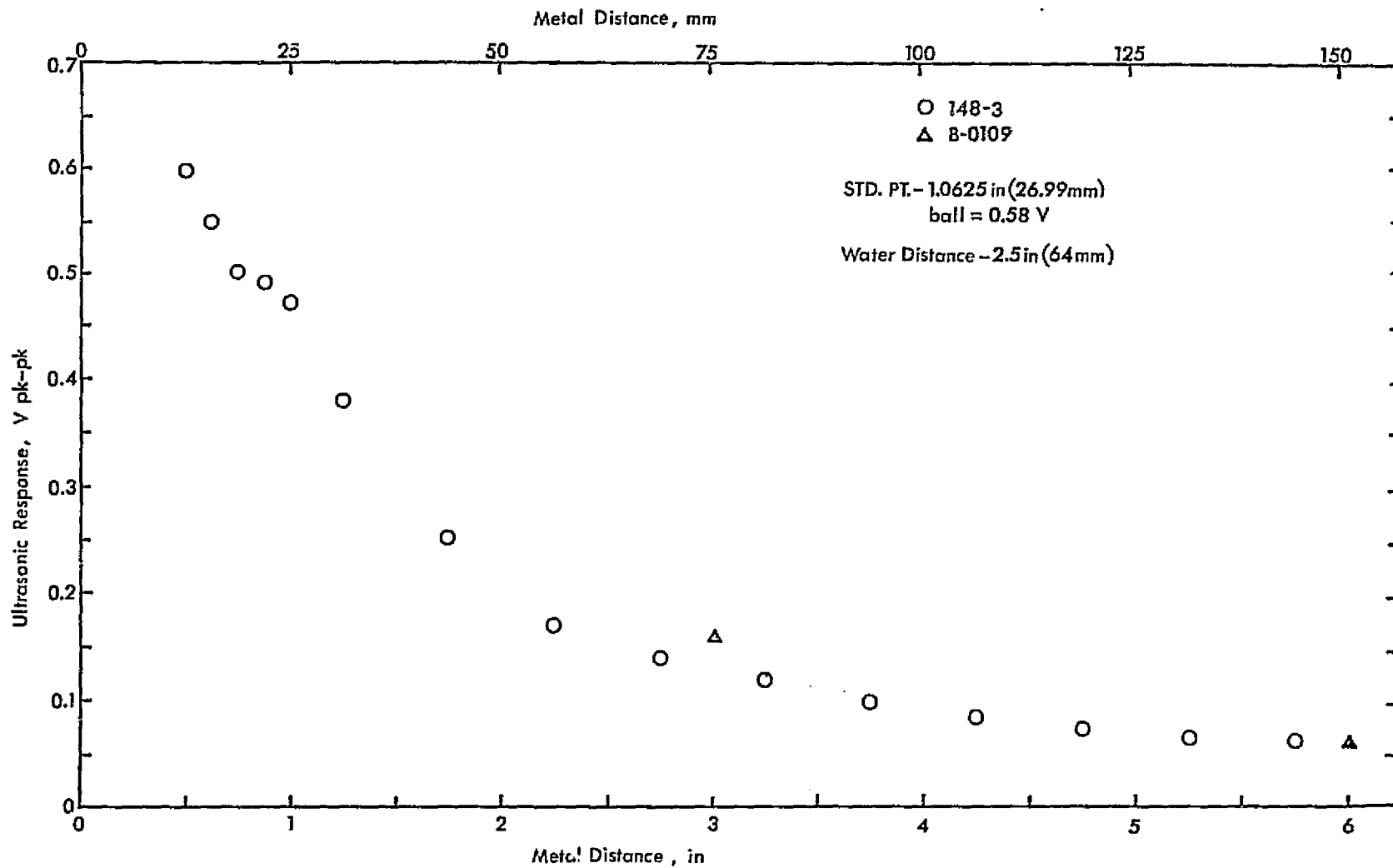
Figure 12 - Distance-amplitude data for No. 8 blocks at 10 MHz.
