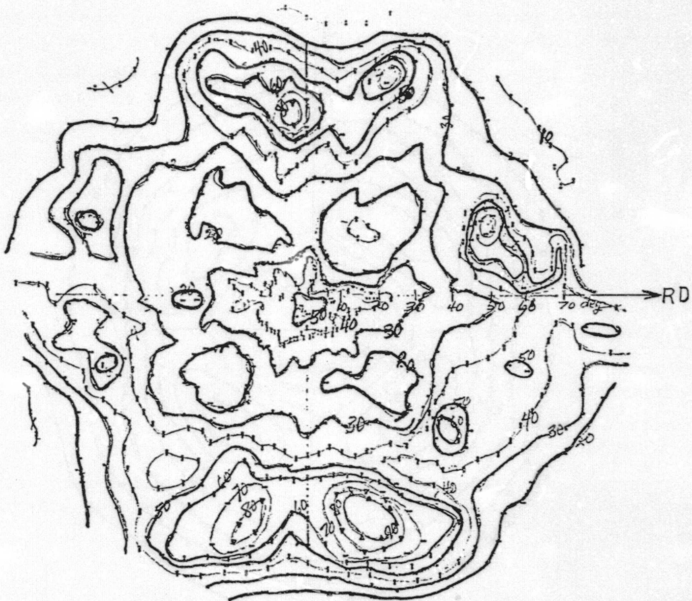
Figure 15 - (111) pole figure for 7075-T631 aluminum
