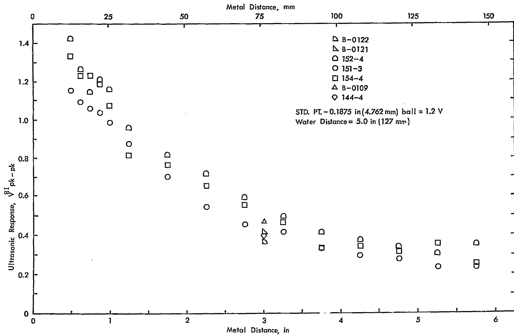
Figure 7 - Distance-amplitude data for No. 3 blocks at 5.0 MHz.
