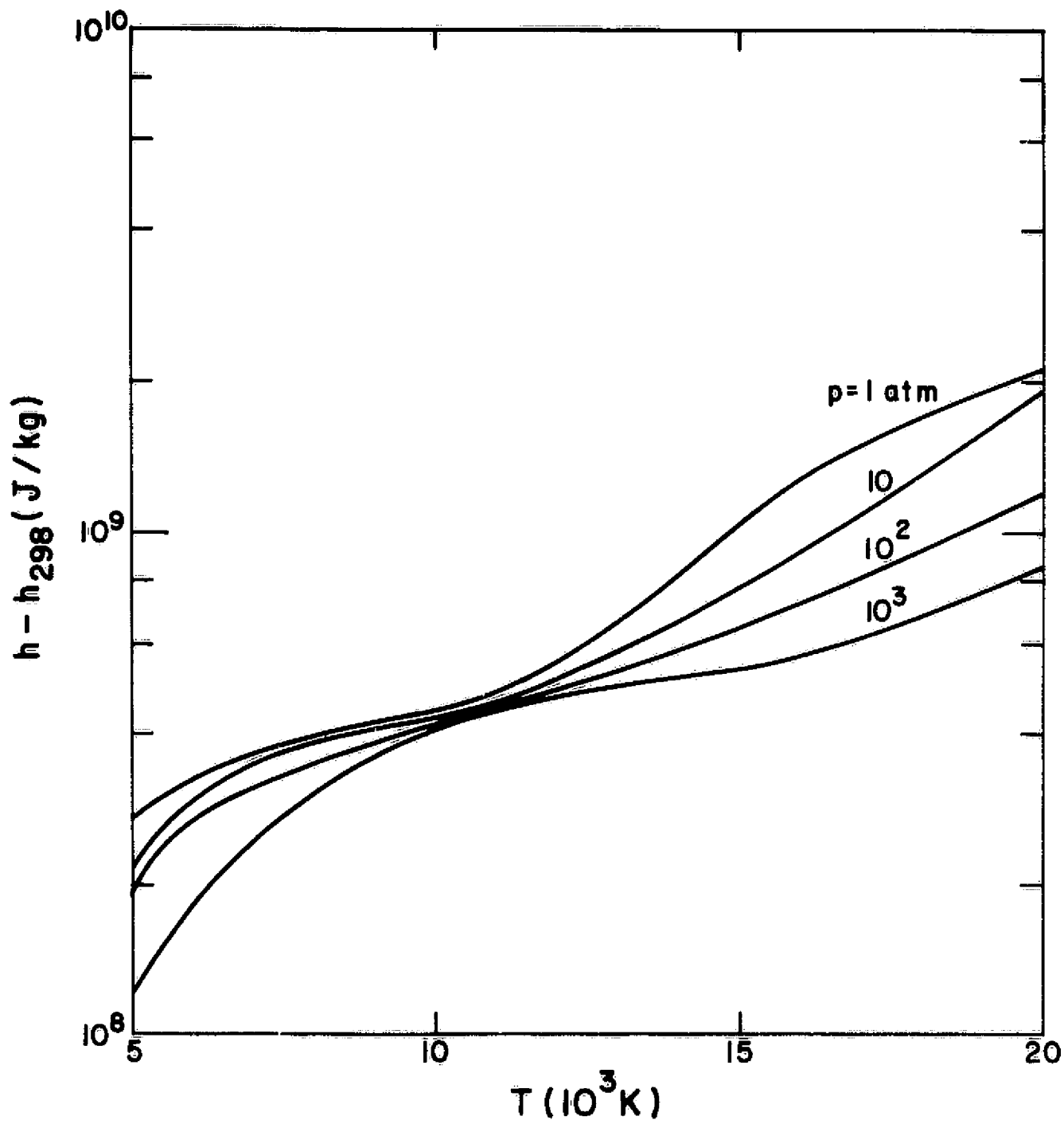
Fig. 2.3 Enthalpy of Hydrogen
