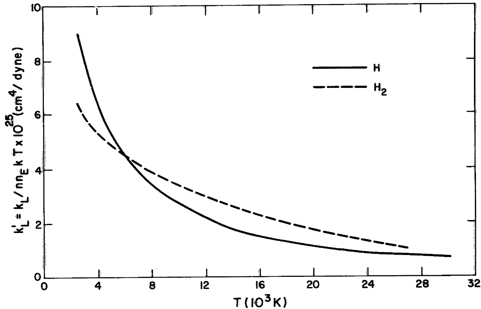
Fig. 2.2 Neutral Inverse Bremsstrahlung Reduced Absorption Coefficient for 10.6 \mu\text{m}
