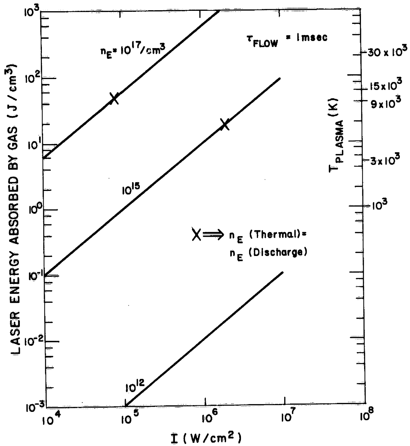
Fig. 2.4 Laser Energy Deposition for Various Discharge Electron Densities (Gas Density 4.9 \times 10^{19} particles/cm 3 )
