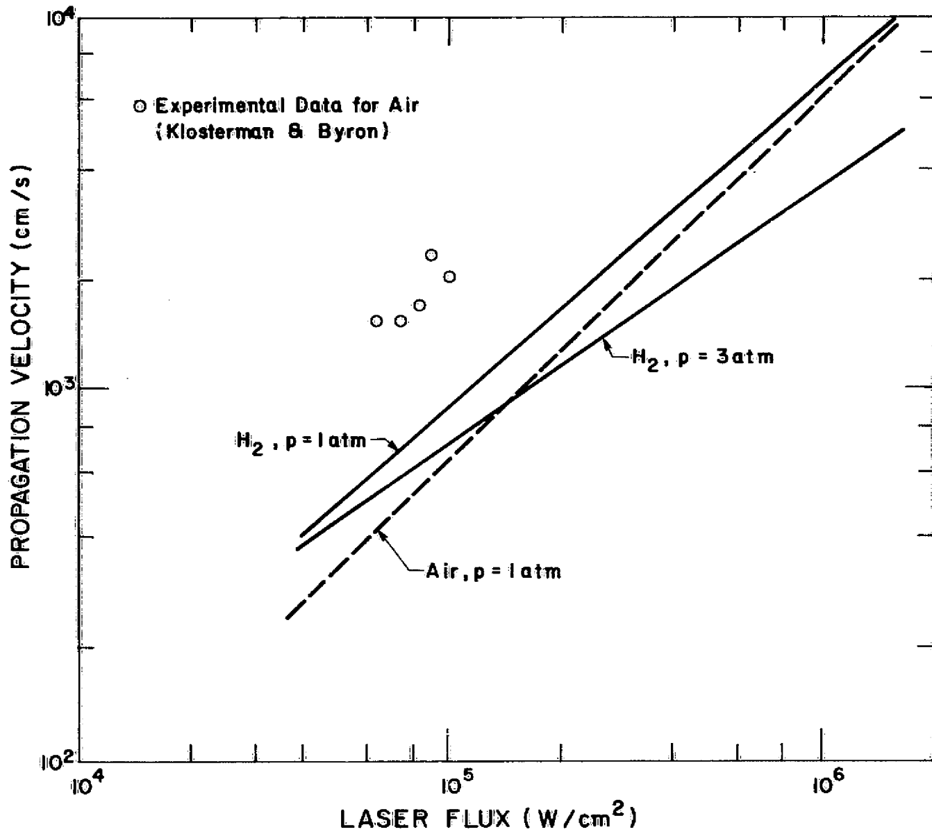
Fig. 6.1 Velocity of Laser Supported Combustion Waves
