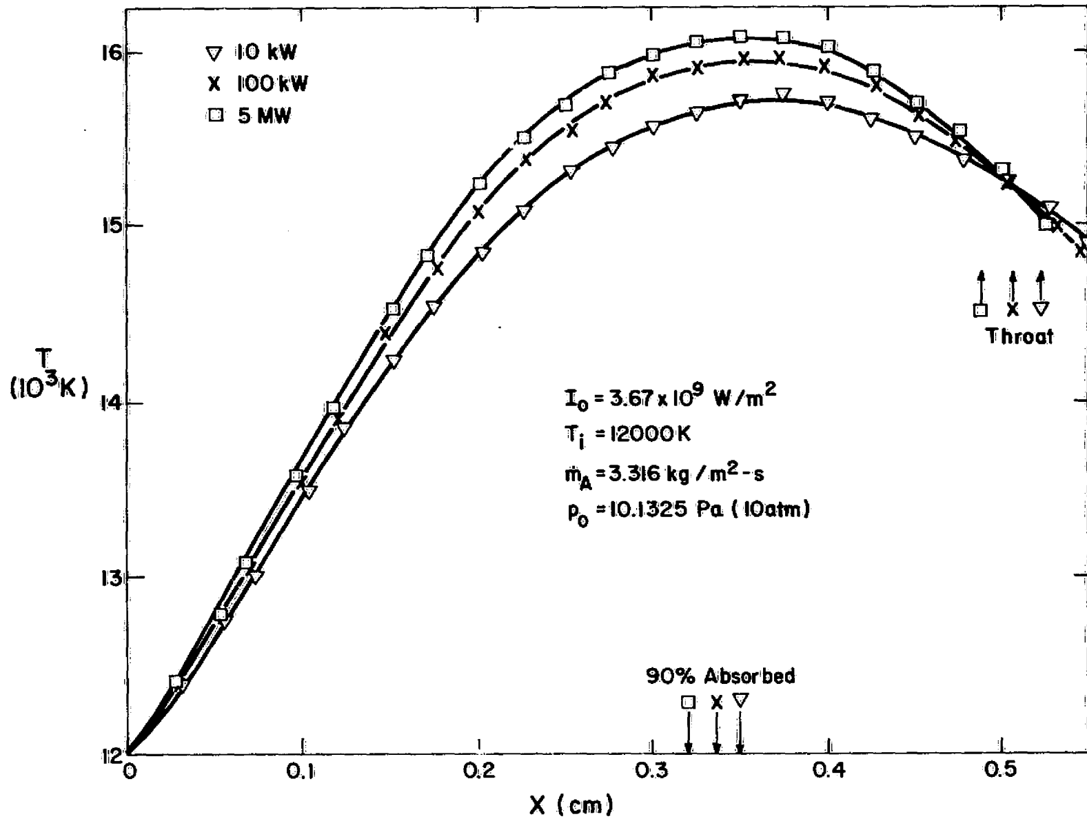
Fig. 7.2b Laser-Heater Streamtube Temperature Distribution for 10 atm Initial Pressure
