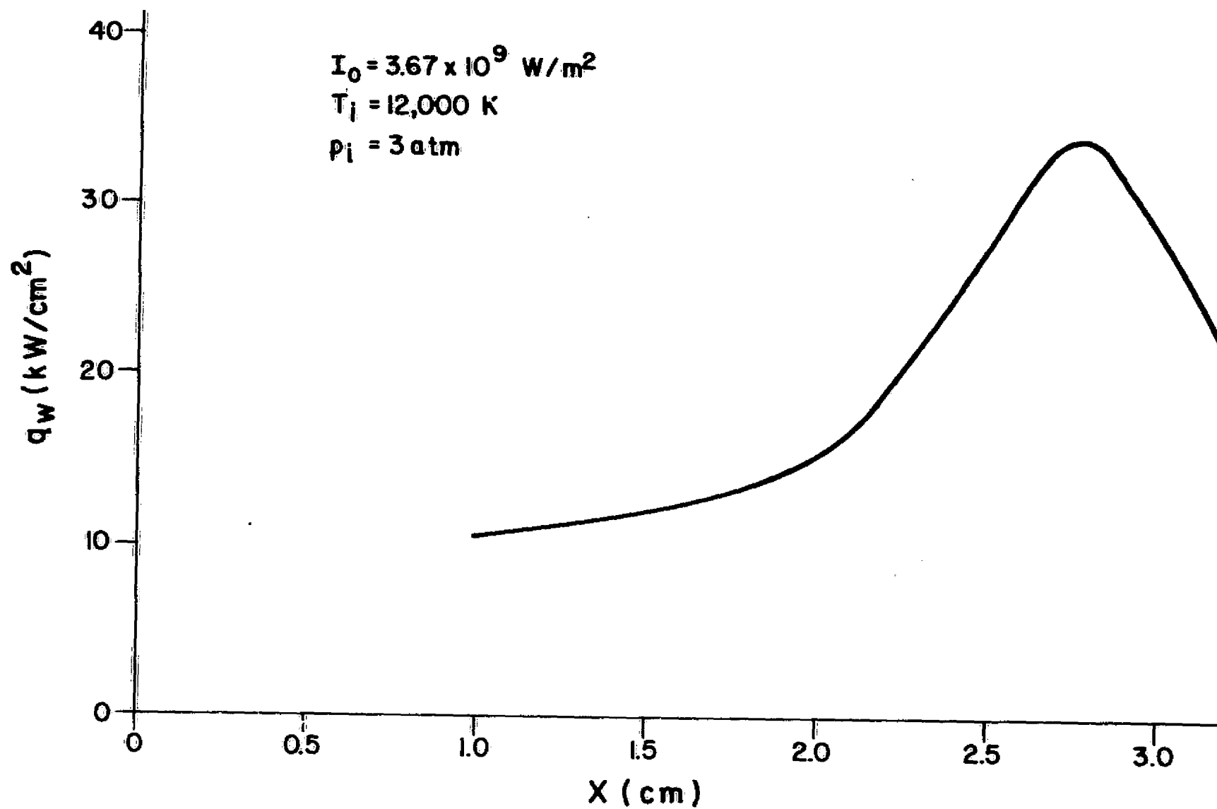
Fig. 8.4 Heat Flux Distribution from Hydrogen Boundary Layer of Laser-Heated Streamtube
