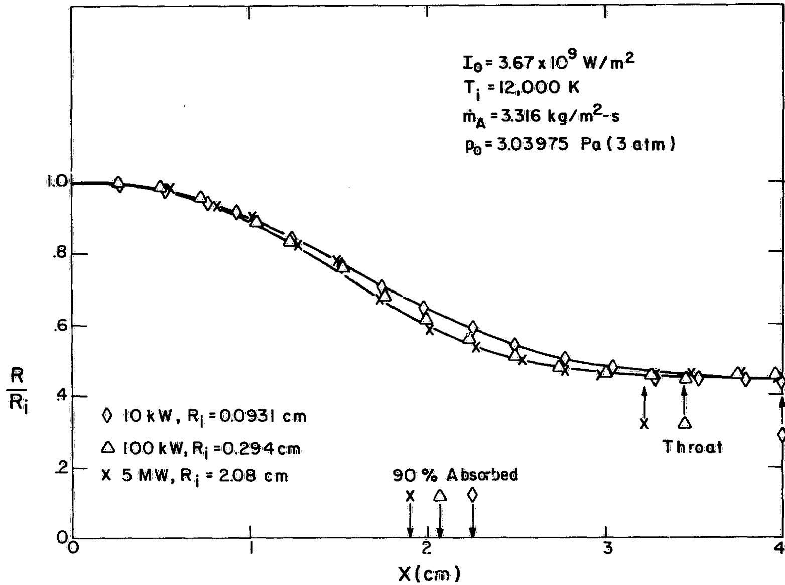
Fig. 7.3a Laser-Heated Streamtube Radius Distribution for 3 atm Initial Pressure
