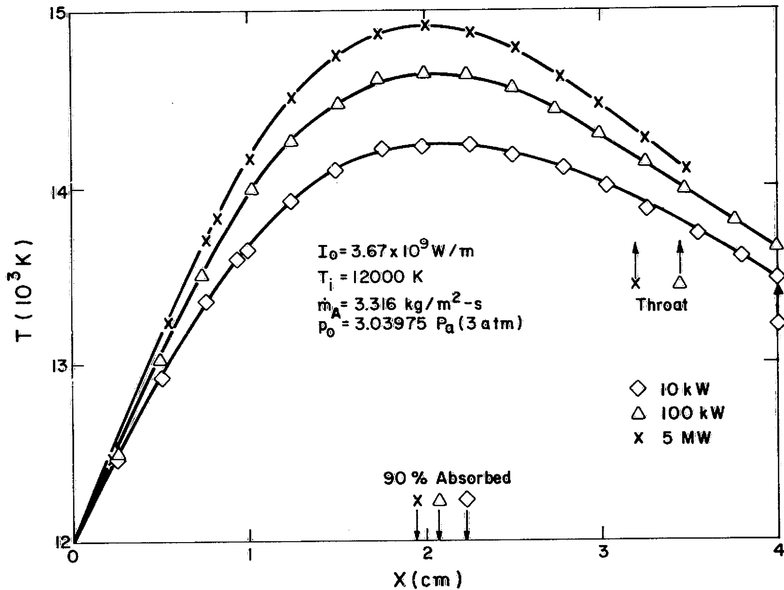
Fig. 7.2a Laser-Heated Streamtube Temperature Distribution for 3 atm Initial Pressure
