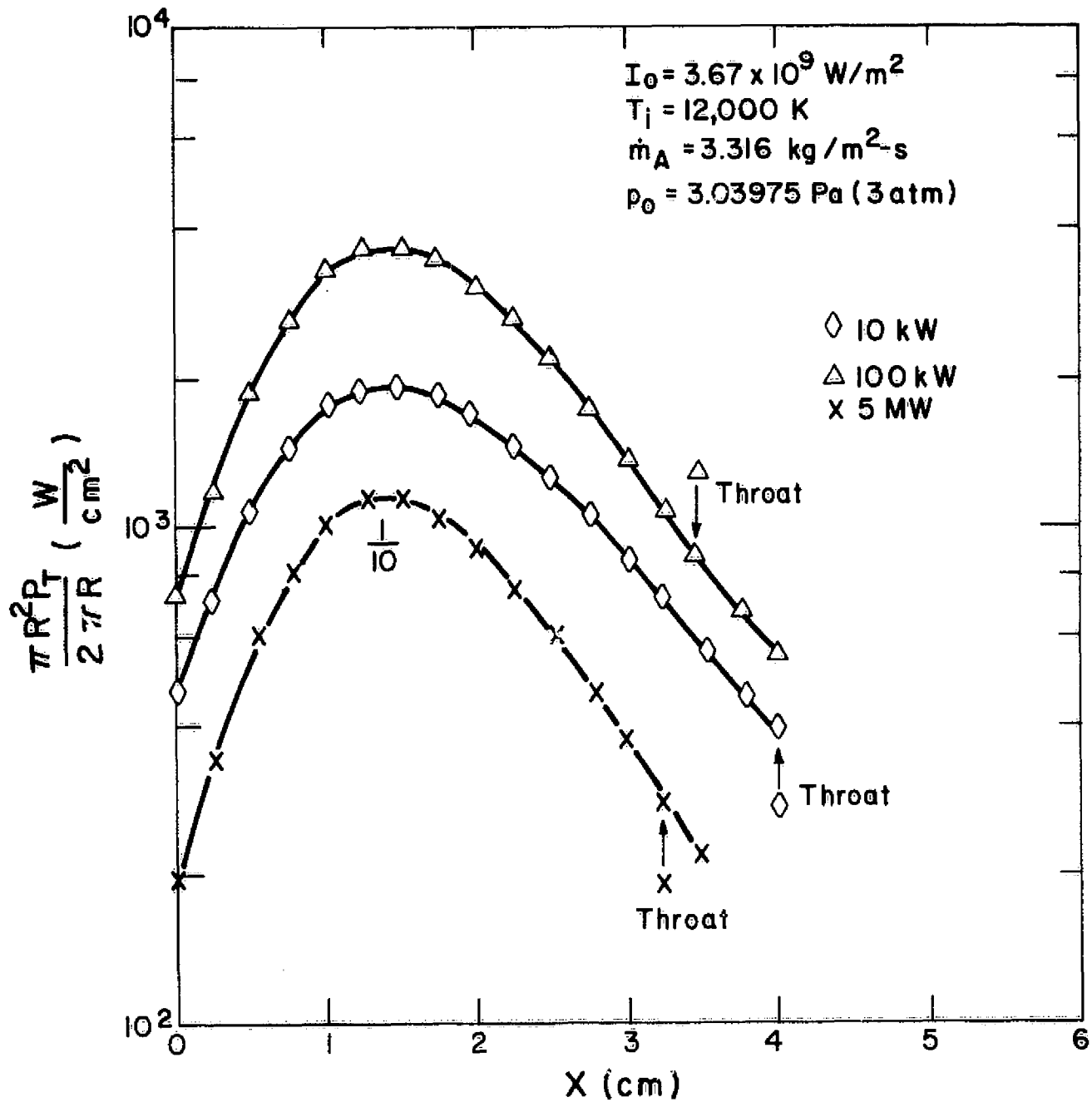
Fig. 8.2a Station Radiant Energy Flux of Laser-Heated Streamtube for 3 atm Initial Pressure
