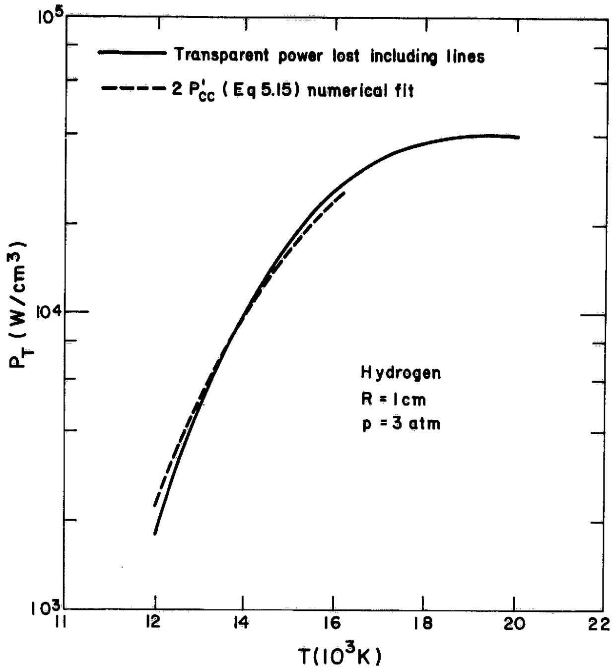
Fig. 5.5 Power Radiated from Hydrogen (3 atm, R = 1 cm) Showing Numerical Results and the Analytic Approximation
