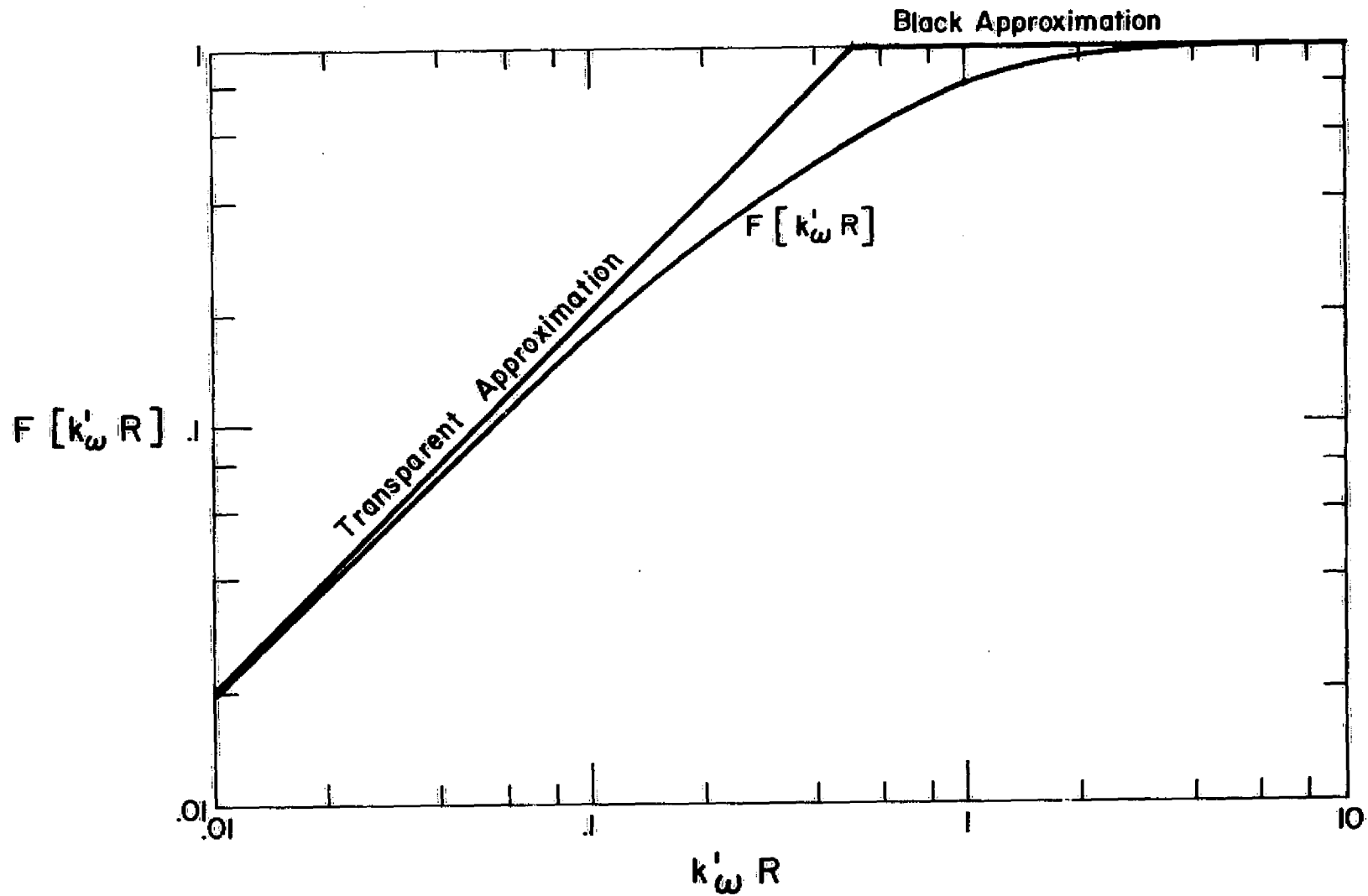
Fig. 5.4 Ratio of Actual Power Lost to Black Body Limit on Power Lost for an Infinite Cylinder. The Transparent and Black Body Approximations Are Also Shown.
