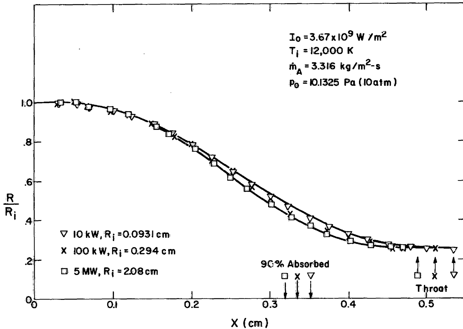
Fig. 7.3b Laser-Heated Streamtube Radius Distribution for 10 atm Initial Pressure
