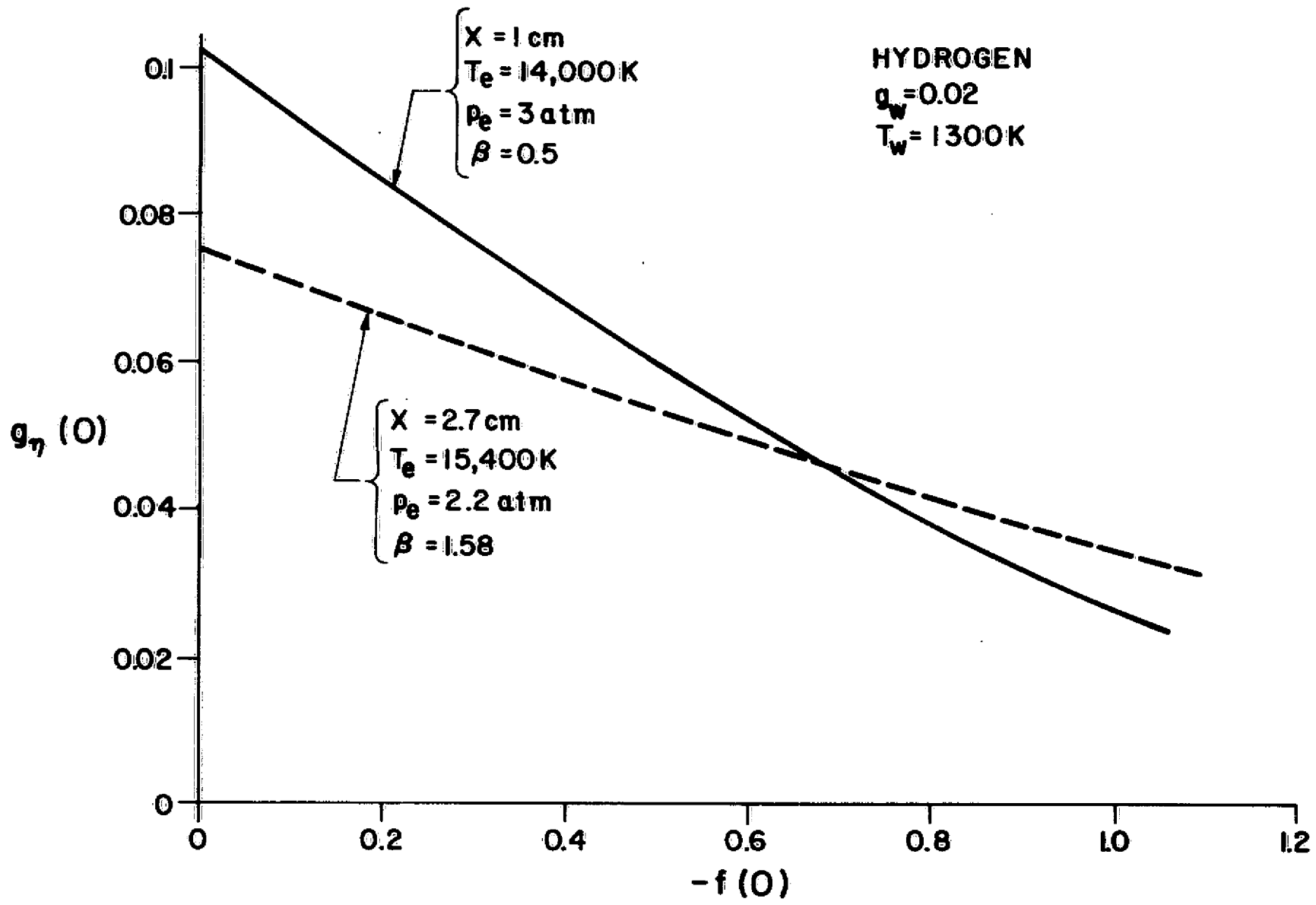
Fig. 8.5 Effect of Normal Hydrogen Injection on Heat Transfer Parameter for Hydrogen Boundary Layer
