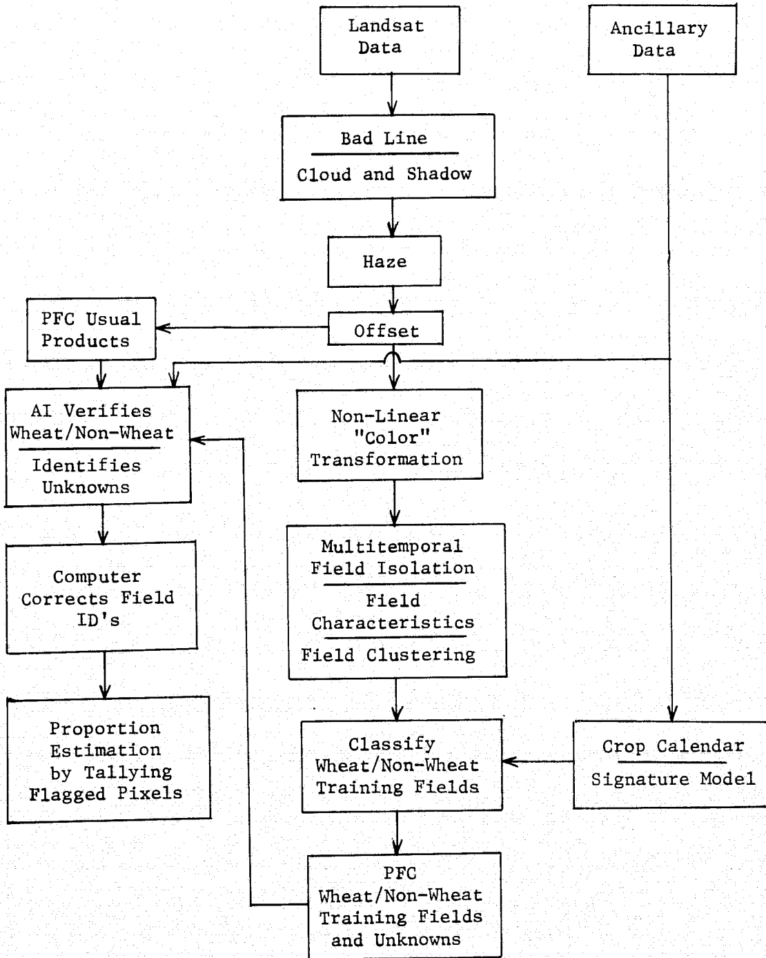
FIGURE 4. OPERATIONS REQUIRED FOR COMPUTER ASSISTED IDENTIFICATION OF WHEAT TRAINING FIELDS
