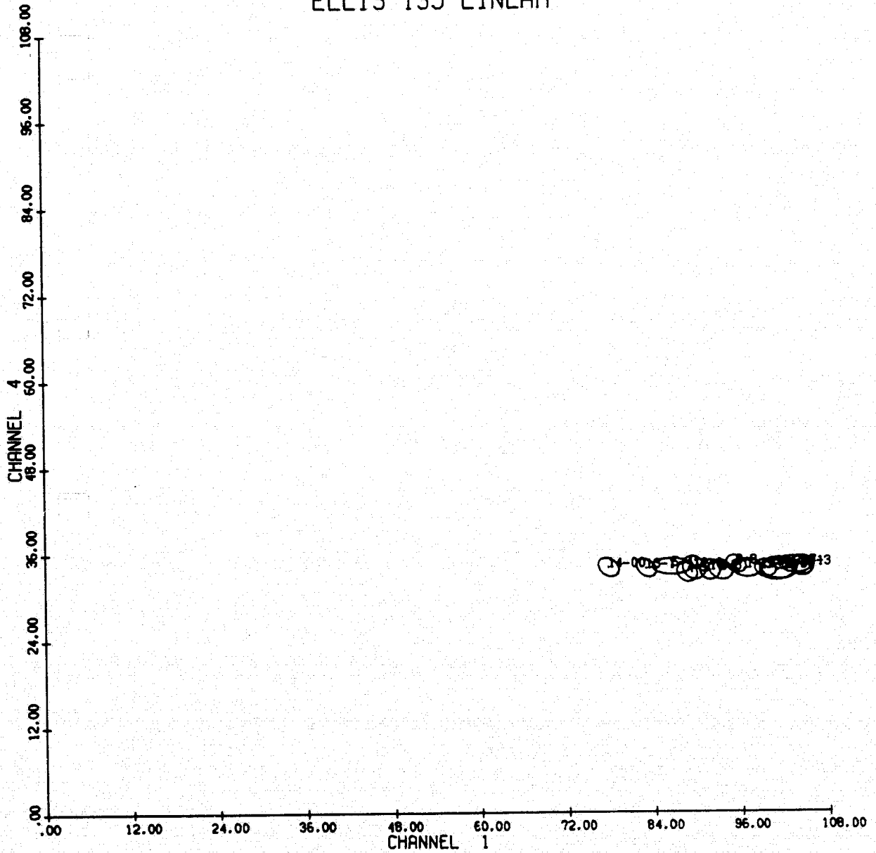
FIGURE 9(c). ELLIS COUNTY, CLUSTER PLOT OF TRANSFORMED DATA, CHANNEL 1 VS 4
