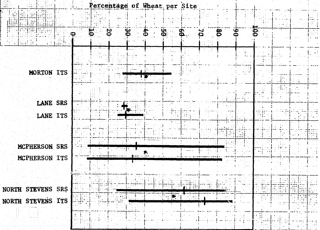
FIGURE 3. COMPARISON OF WHEAT ESTIMATE BOUNDS FOR FOUR SITES
