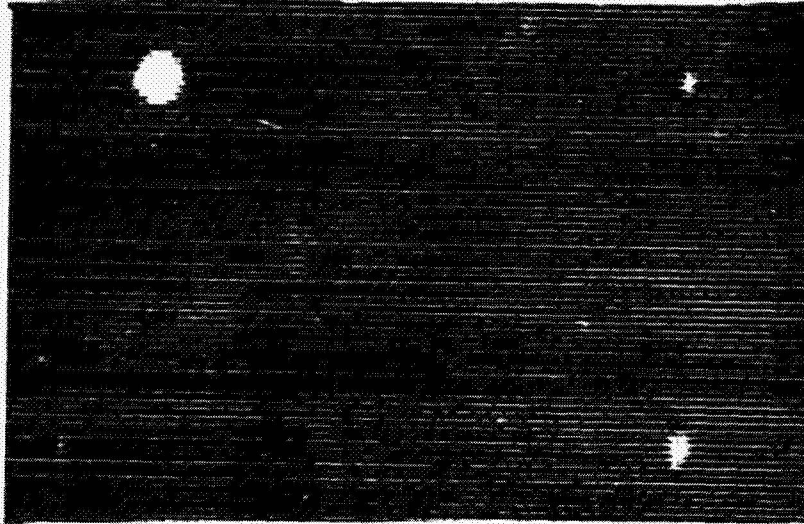
Recording #1: "C" scan presentation of flaws contained in Case 1, Thick, Titanium Reference Panel with flaws at far surface.
