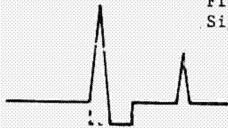
Photo #2 "A" scan presentation of flaw #2 contained in Case 1, Thick, Titanium, Reference Panel when flaw #2 is at far surface from transducer.
