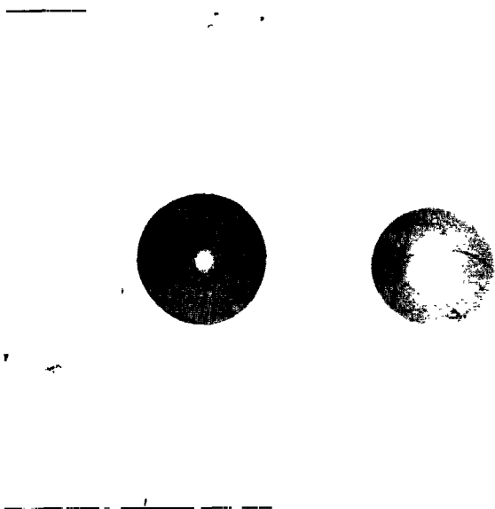
Figure 6. Comparison of P-149 and I-319 Fluorescent Penetrants by the Meniscus Method (P-149 on the Left has Superior Thin Film Sensitivity)
