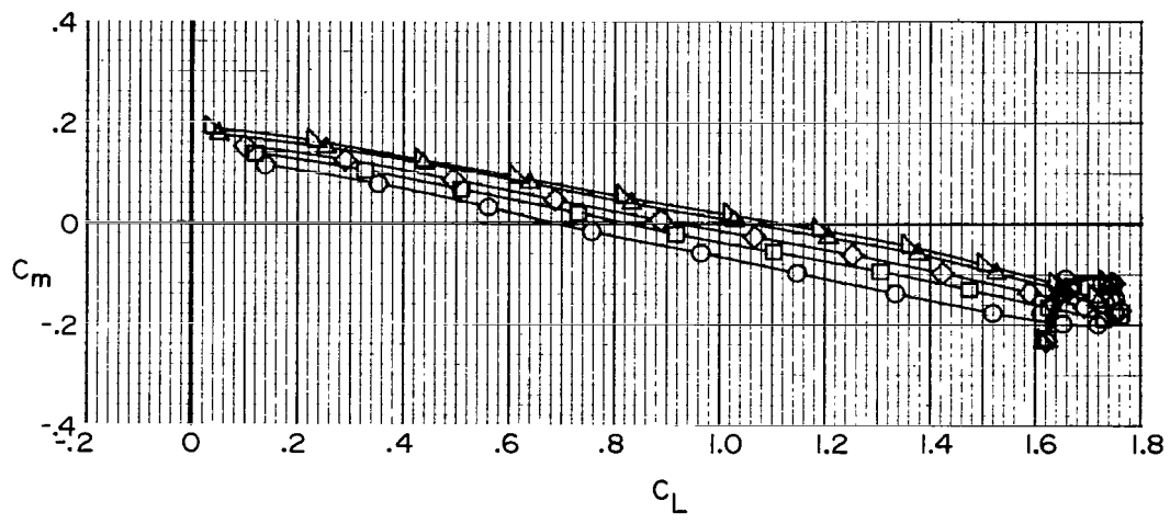
(b) Pitching-moment coefficient.
