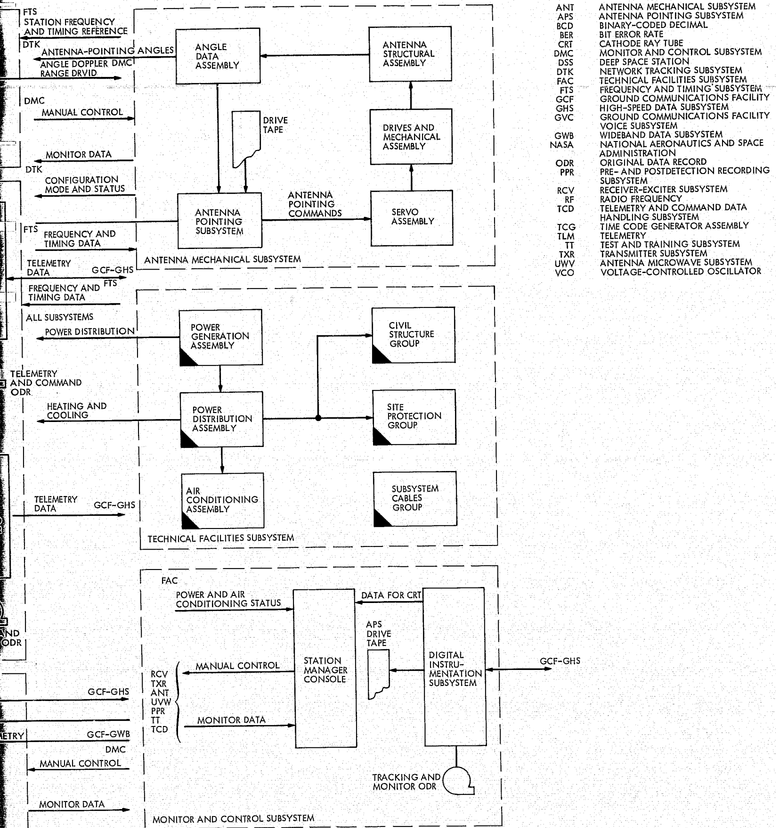
Fig. 40. Deep Space Network Mark III-75 functional network design: 26-meter stations
