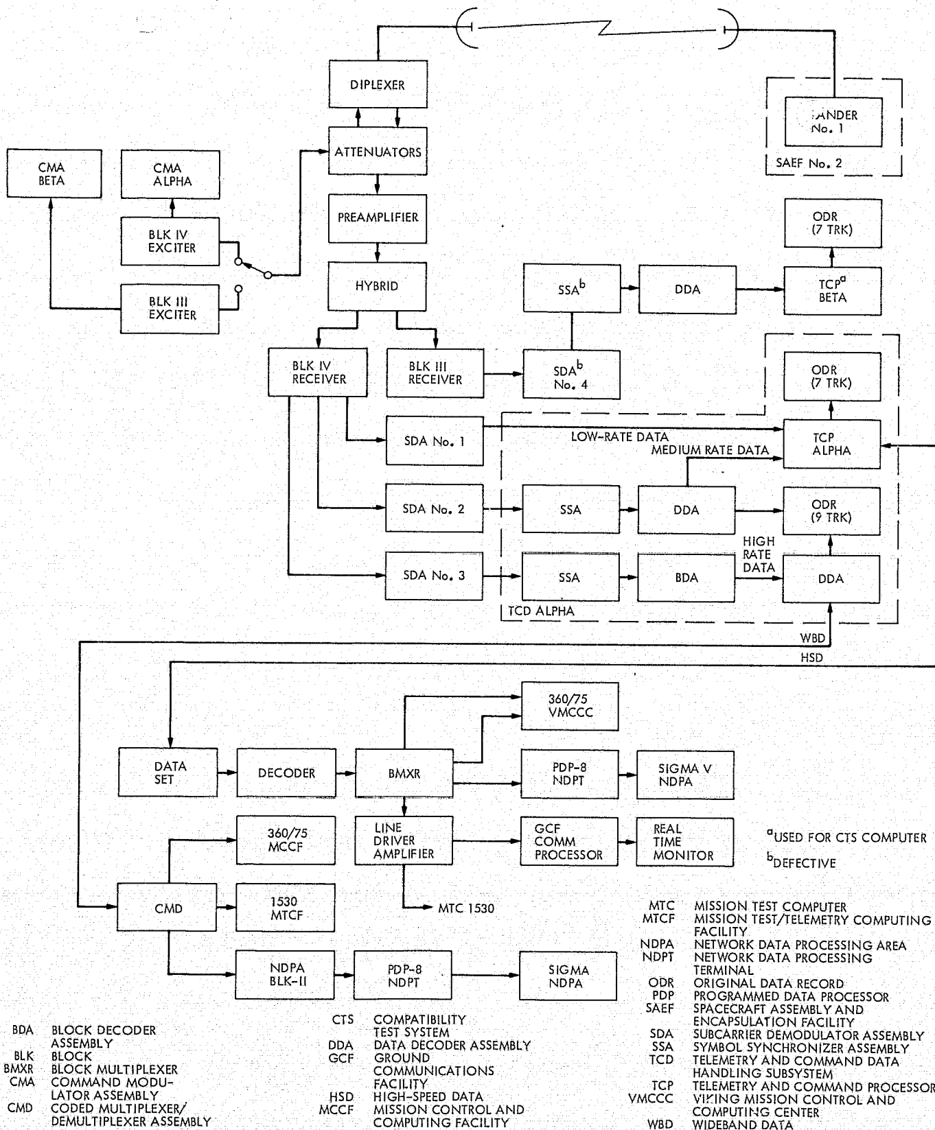
Fig. 50. Telecommunications compatibility test configuration, January 30, 1975
