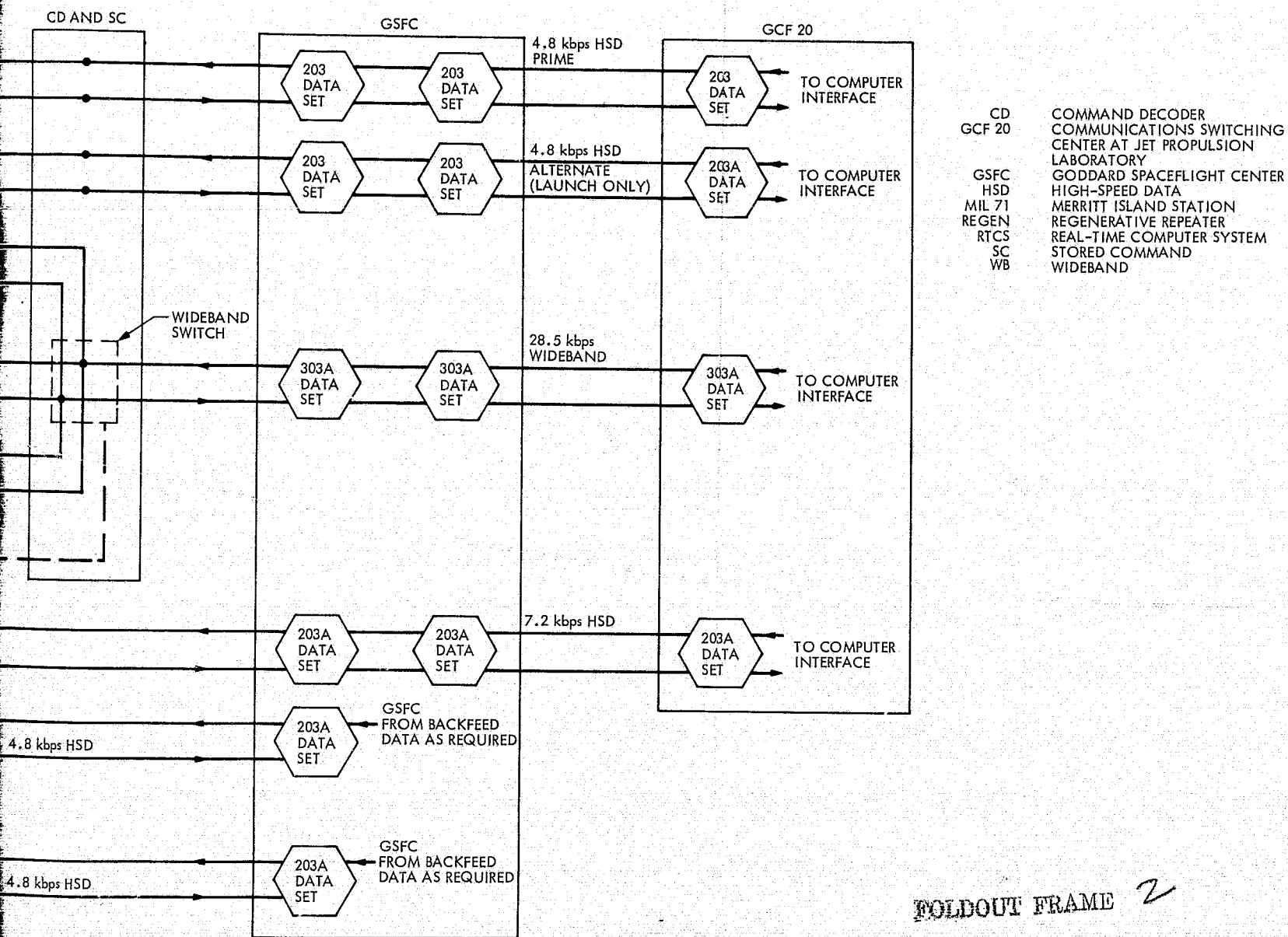
Fig. 34. Viking Project data circuits for near-Earth support
