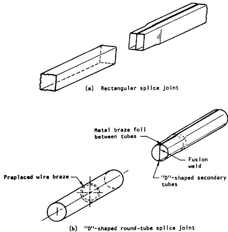
Figure 16. – Two types of coolant-tube splice joints.
