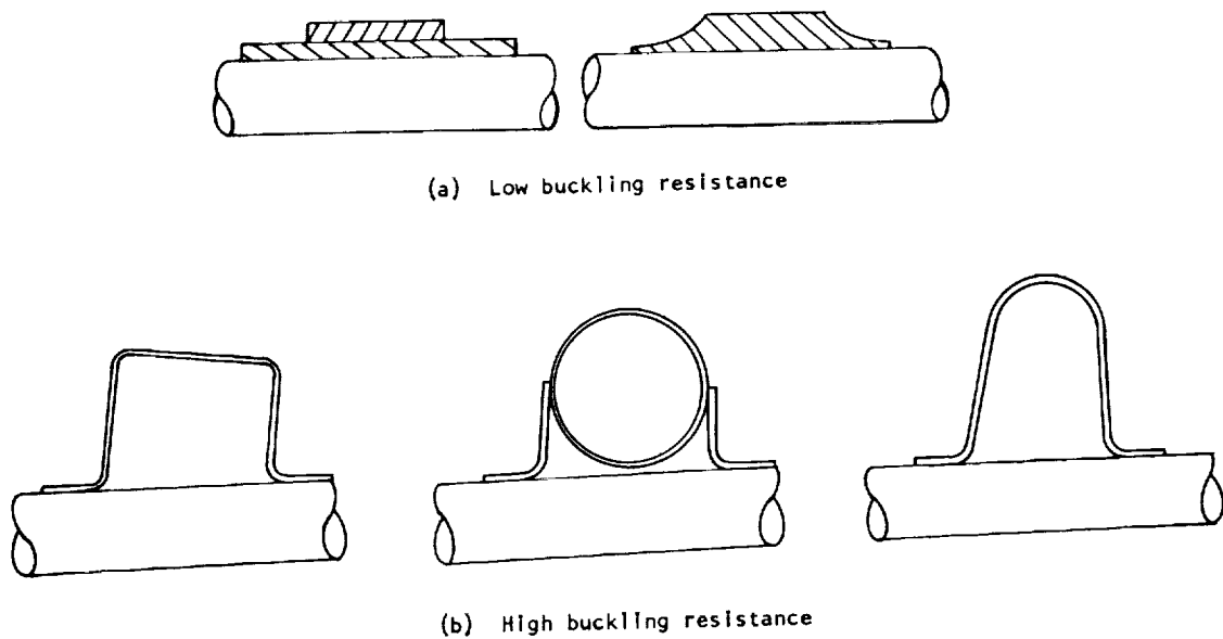
Figure 40. — Recommended designs for retaining bands to provide desired degree of tube-bundle rigidity.
