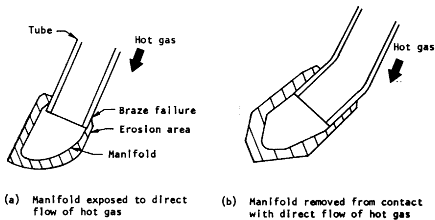
Figure 47. — Method for avoiding failure of manifold from exposure to hot-gas flow.
