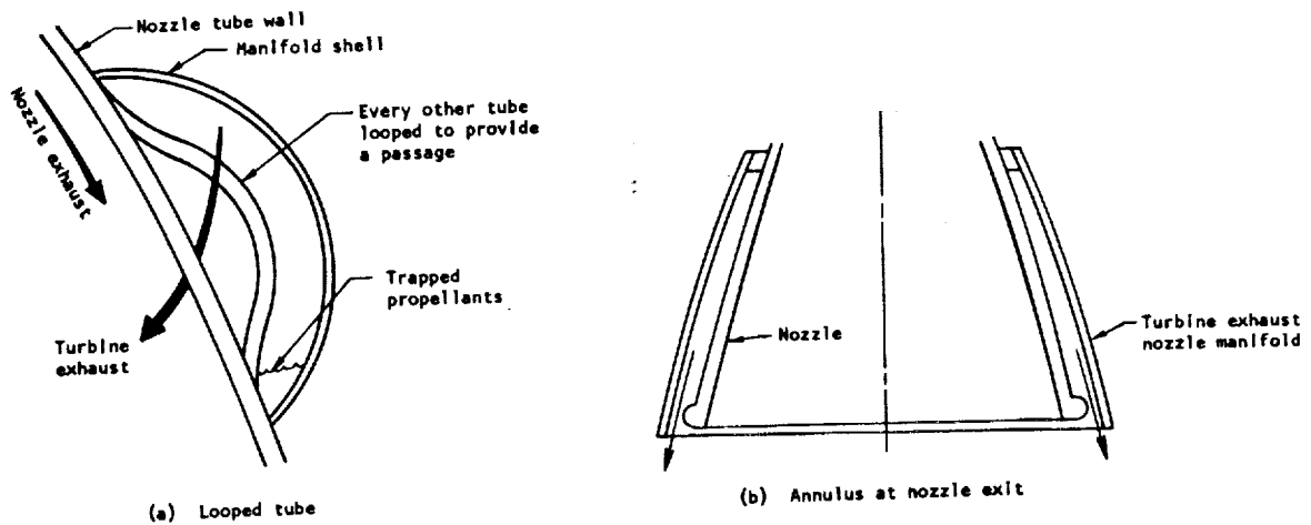
Figure 45. — Two methods recommended for introducing turbine exhaust gas into nozzle.
