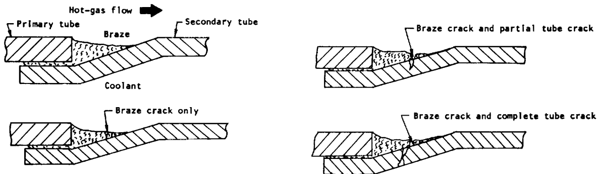
Figure 17. – Types of cracks in brazed joints of coolant tubes (F-1 engine).
