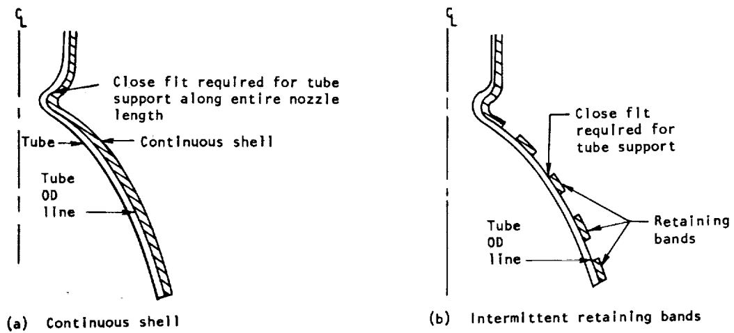
Figure 14. — Two basic methods for supporting coolant tubes.
