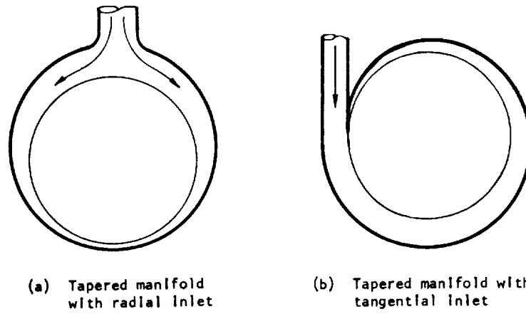
Figure 25. — Two configurations for tapering a manifold to reduce variation of static pressure.
