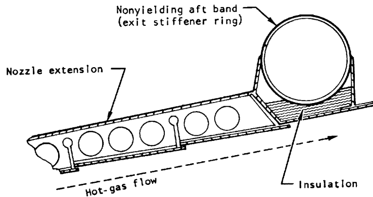
Figure 44. — Recommended construction of a nonyielding aft retaining band.
