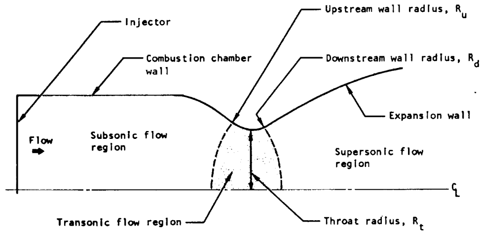
Figure 2. — Sketch illustrating basic nozzle configuration and nomenclature.
