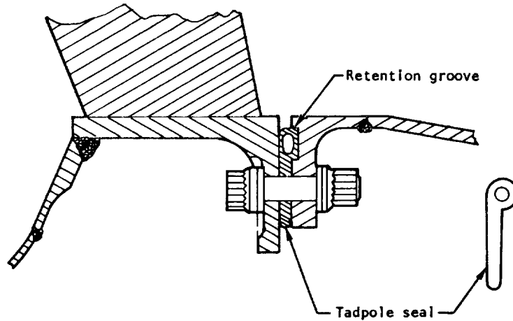
Figure 36. — Flange and seal design for use in high operating temperatures.
