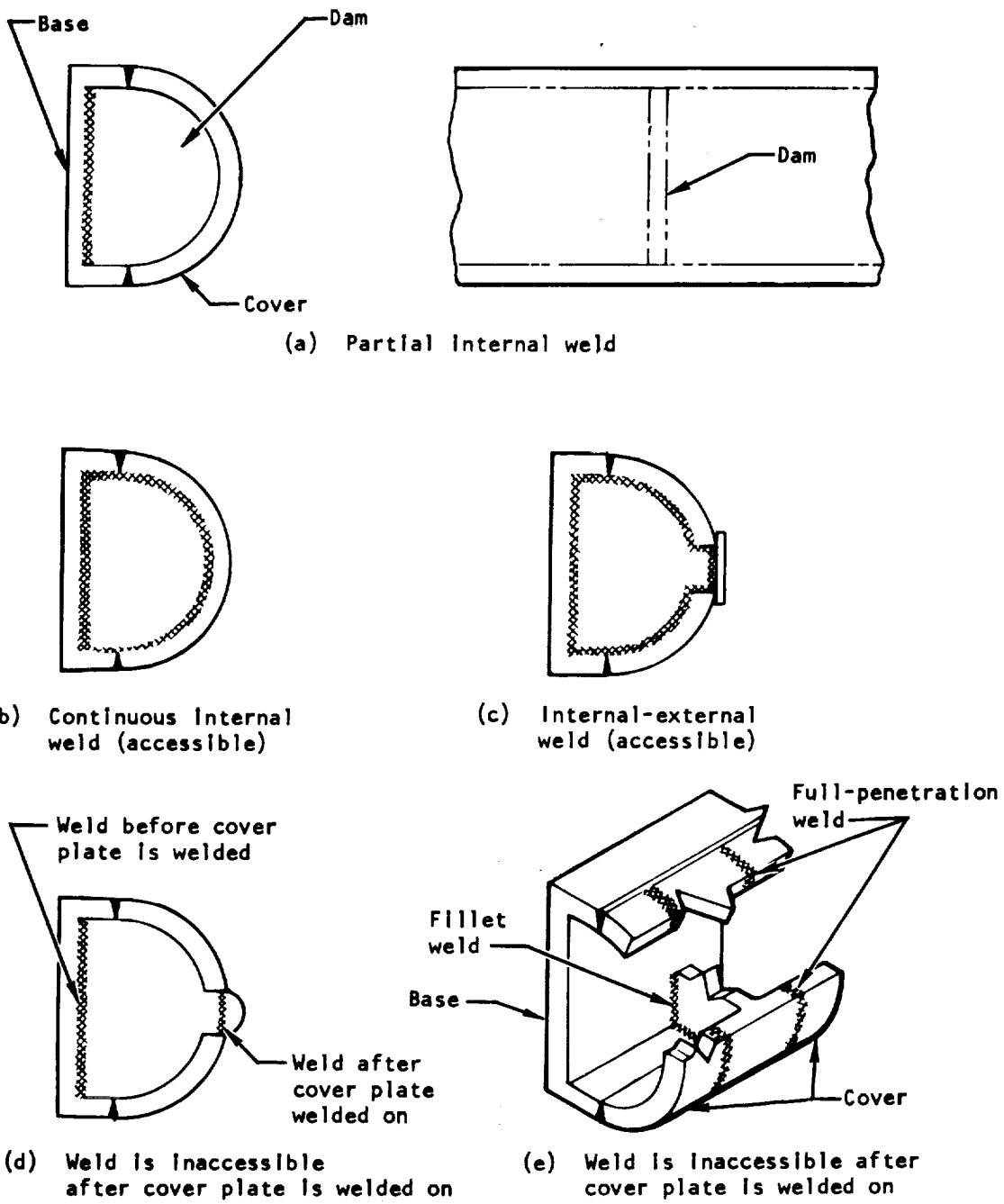
Figure 32. — Methods for welding dams in manifolds.
