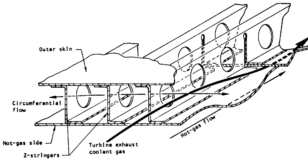
Figure 19. — Provisions for coolant crossflow in F-1 nozzle extension.
