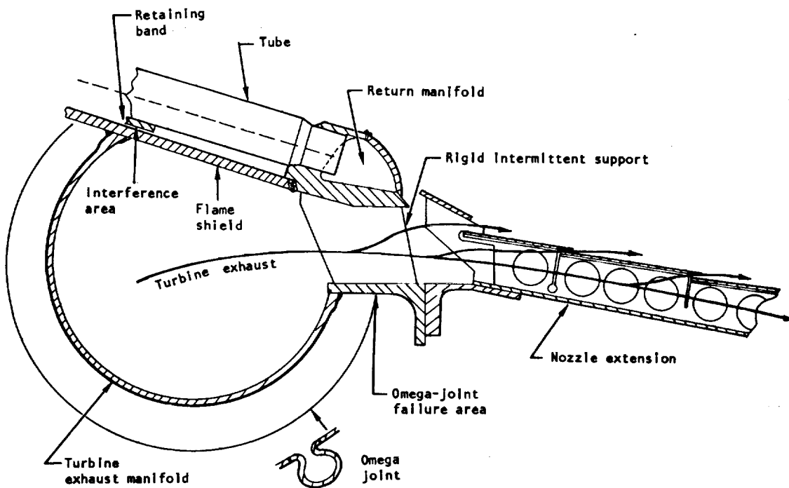
Figure 33. — Construction of junction of turbine exhaust manifold and film-cooled nozzle extension (F-1 engine).
