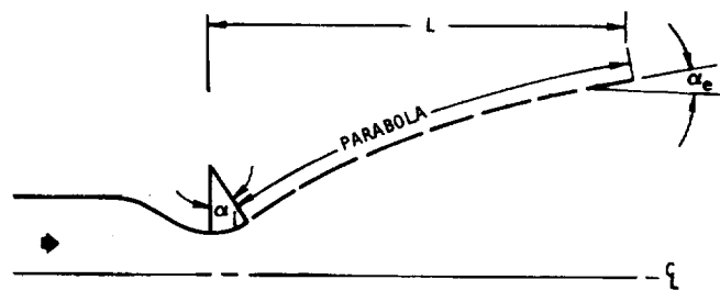
(a) Canted-parabola nozzle contour
