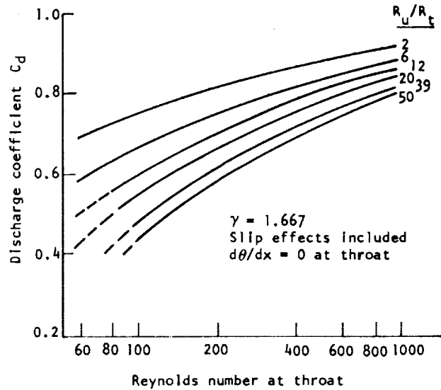
Figure 8. — Nozzle discharge coefficient as a function of Reynolds number at throat for various values of R_u/R_t .
