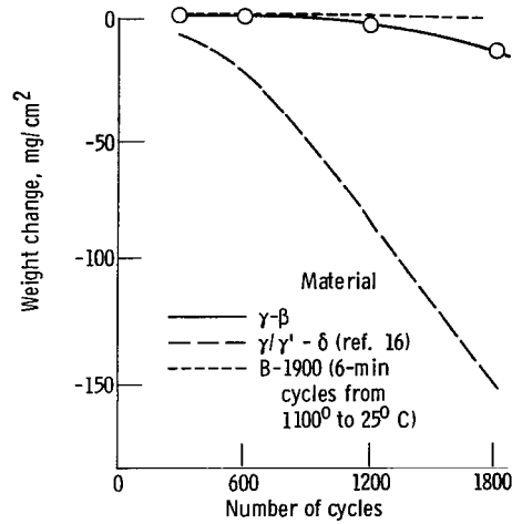
Figure 11. - Specific weight change of directionally solidified \gamma - \beta eutectic alloy due to thermal cycling in Mach 0.3 oxidation-erosion burner rig.
