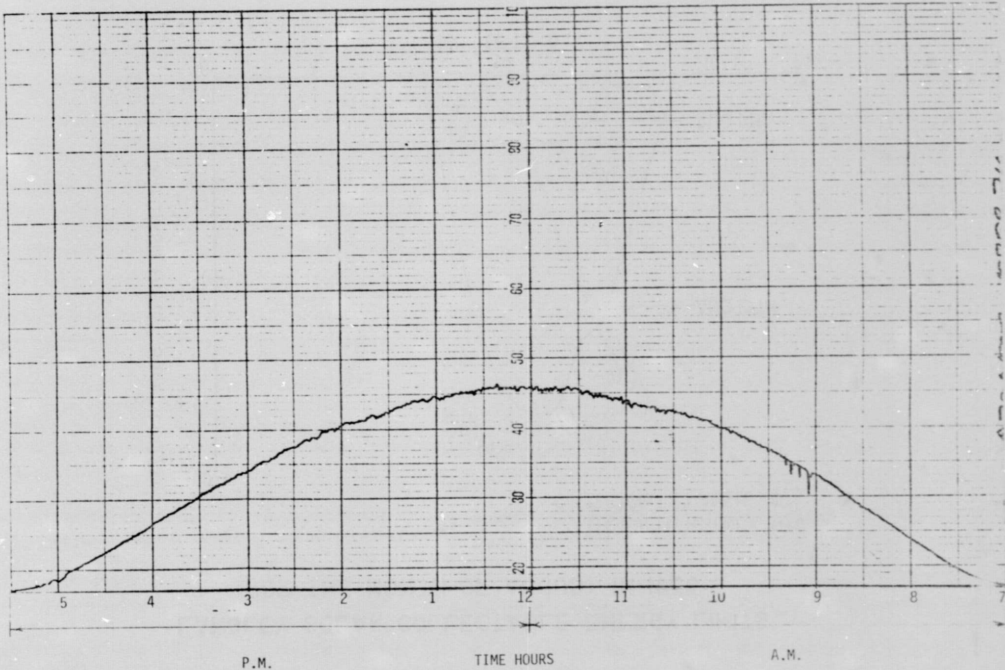
Figure 16 - Solar insolation data recorded at Langley on February 5, 1974. Each ordinate line represents 6.64 BTU/HR - FT 2 (2.09 W/m 2 ). The total area under the curve represents 1,208 BTU/FT 2 - Day. ( 1.4 \times 10^7 J/m 2 - Day)
