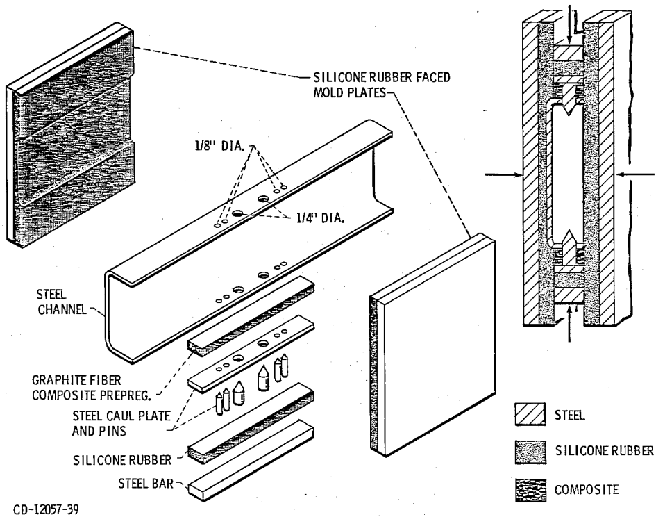
Figure 5. - Mold schematic.
