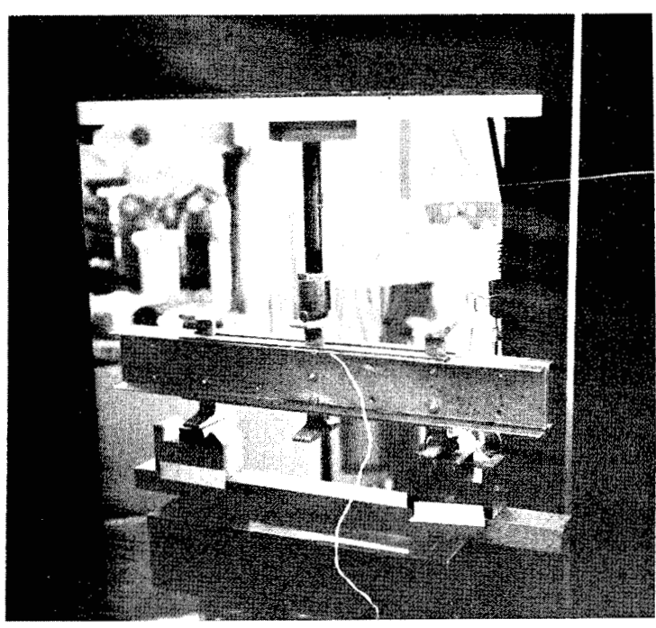
Figure 8. - Rail test assembly in testing machine.
