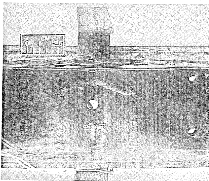
Figure 13. - Buckled flange after ultimate load failure.
