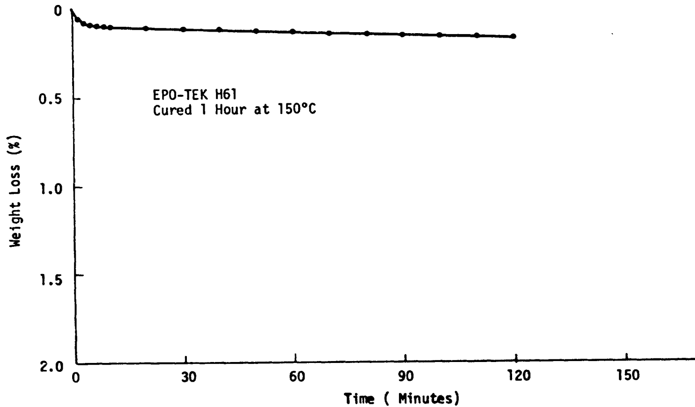
Figure 4. Weight Loss of Epo-Tek H61 at Constant Temperature (150°C) After Cure - As Measured on TGA Apparatus
