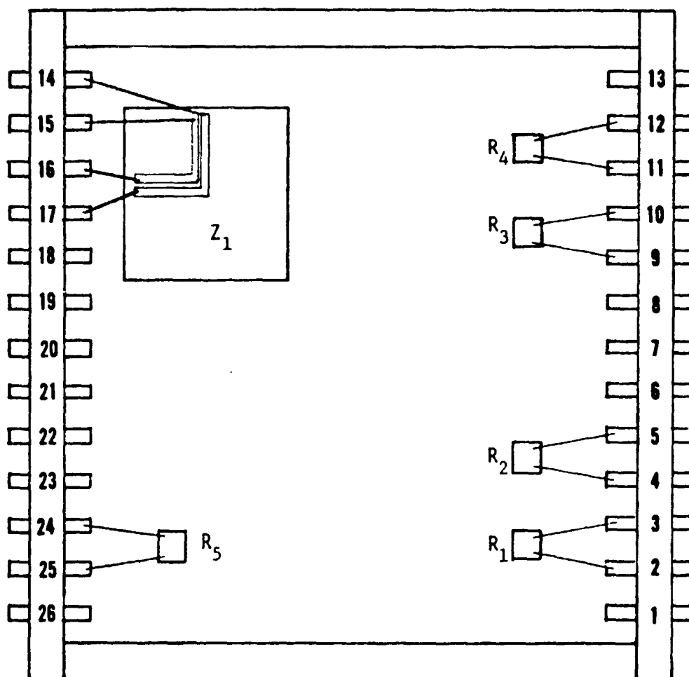
Figure 56. Layout of Thin Film Chip Resistor Test Specimens Containing Only Amount of Adhesive Required to Mount Chips. R_1 through R_4 are Glass Passivated Thin Film Nichrome Chip Resistors. R_5 is an Unpassivated Thin Film Nichrome Chip Resistor. Z_1 is a Chip Containing an Aluminum Conductor Pattern (Shown in Detail in Figure 58.)
