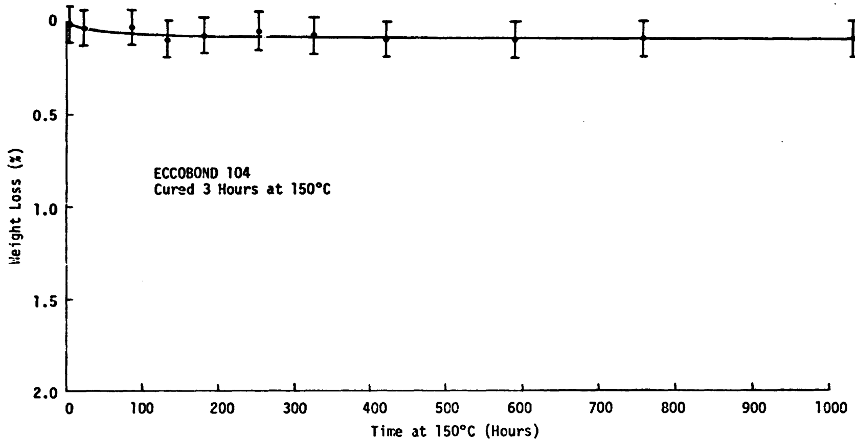
Figure 12. Weight Loss of Eccobond 104 at Constant Temperature (150°C) After Cure - As Measured on Analytical Balance
