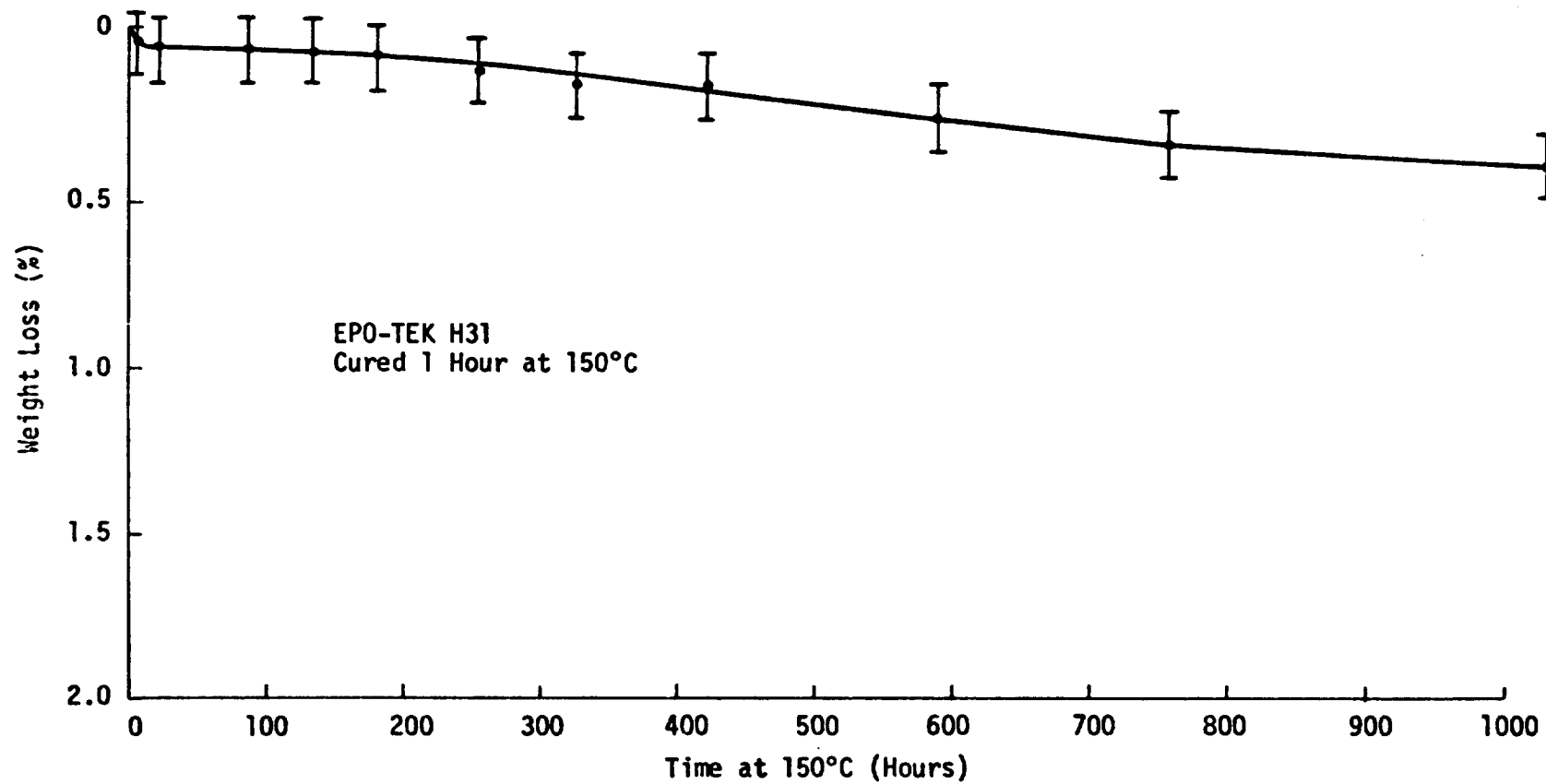
Figure 16. Weight Loss of Epo-Tek H31 at Constant Temperature (150°C) After Cure - As Measured on Analytical Balance
