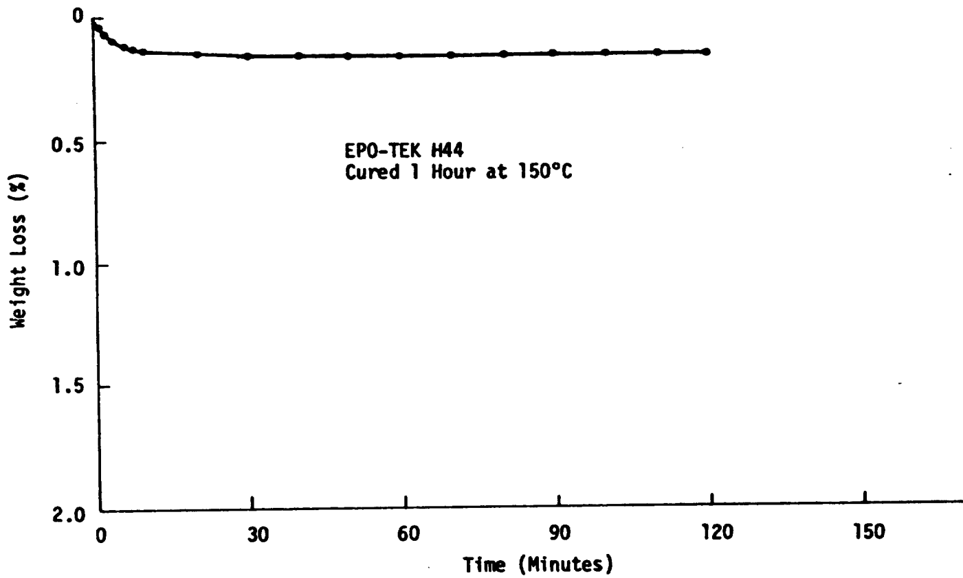
Figure 9. Weight Loss of Epo-Tek H44 at Constant Temperature (150°C) After Cure - As Measured on TGA Apparatus
