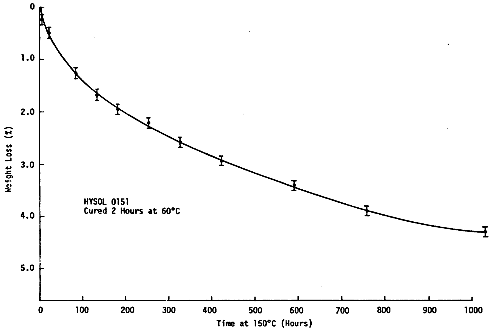
Figure 10. Weight Loss of Hysol 0151 at Constant Temperature (150°C) After Cure - As Measured on Analytical Balance
