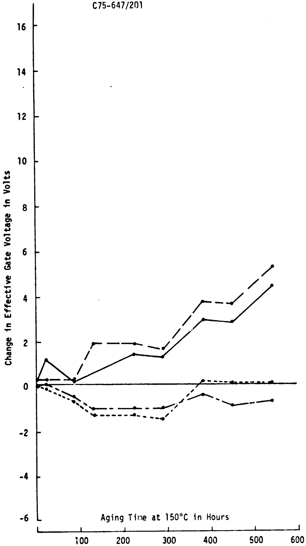
Figure 43. FET Test Specimen Containing 5.4 mg of Epo-Tek H74
