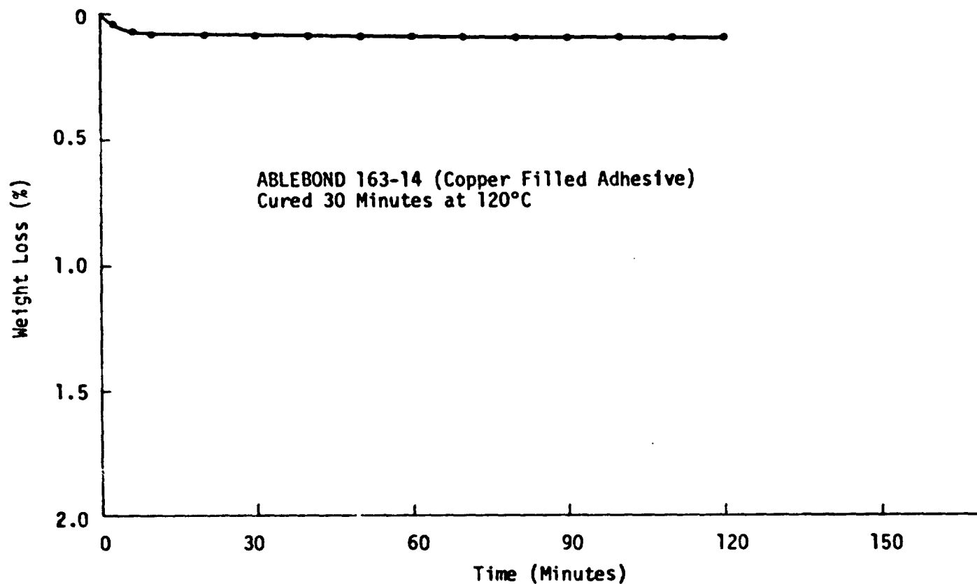
Figure 22. Weight Loss of Ablebond 163-14 at Constant Temperature (150°C) After Cure - As Measured on TGA Apparatus
