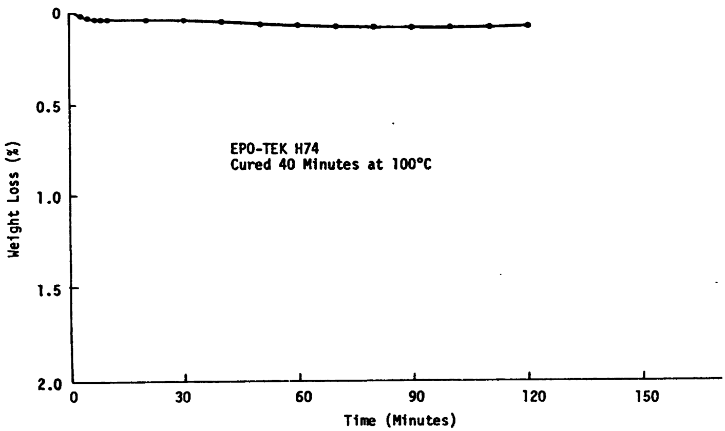
Figure 5. Weight Loss of Epo-Tek H74 at Constant Temperature (150°C) After Cure - As Measured on TGA Apparatus
