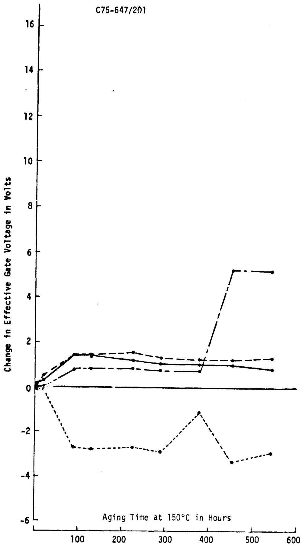
Figure 53. FET Test Specimen Containing 10.5 mg of Ablebond 58-1
