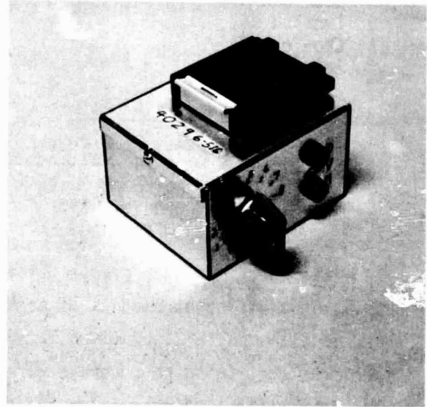
FIGURE 24. Test Adapter for Thin Film Chip Resistor Test Specimens
