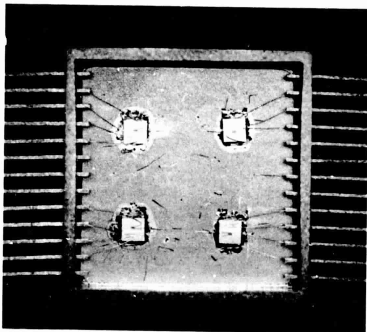
FIGURE 30. FET Device Test Specimen
