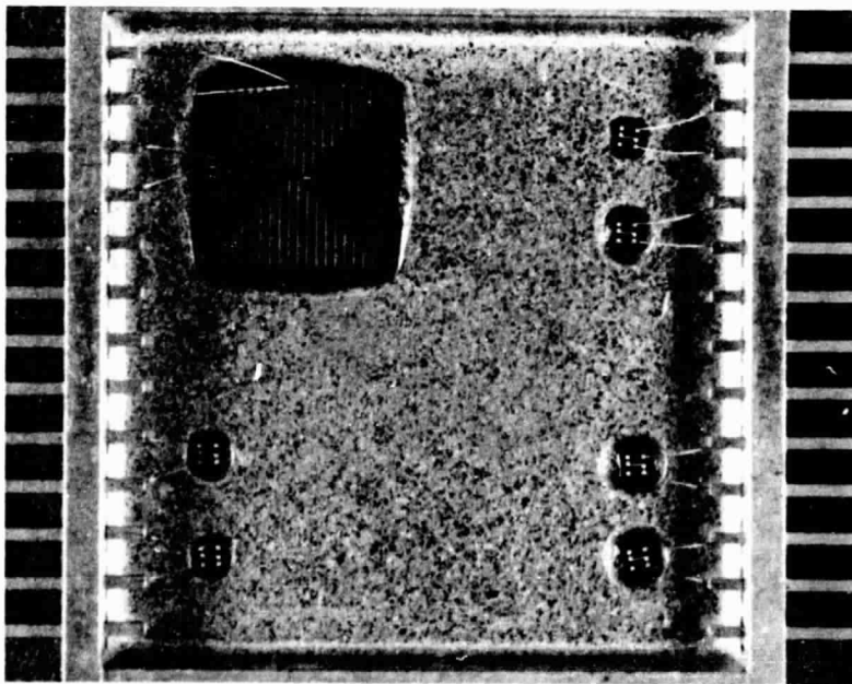
Figure 59. Thin Film Chip Resistor Test Specimens
