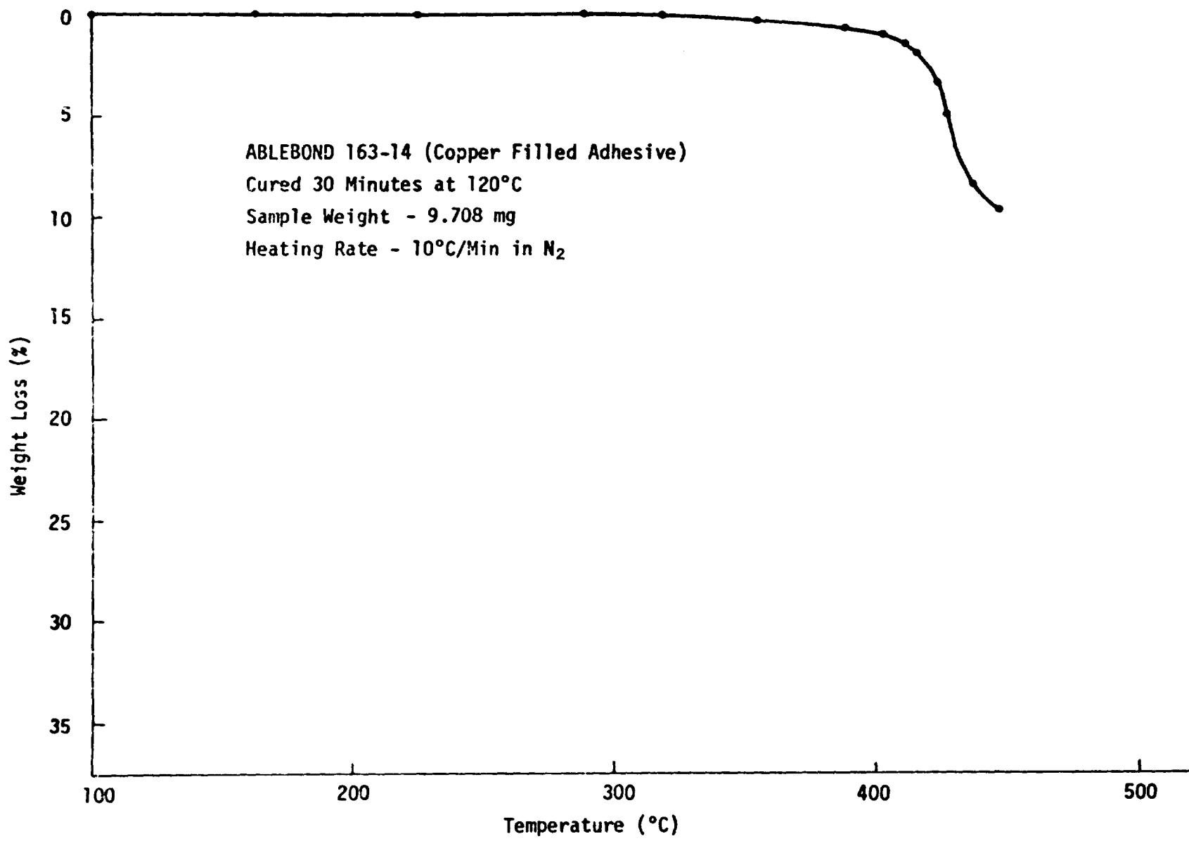
Figure 21. TGA Curve - Ablebond 163-14
