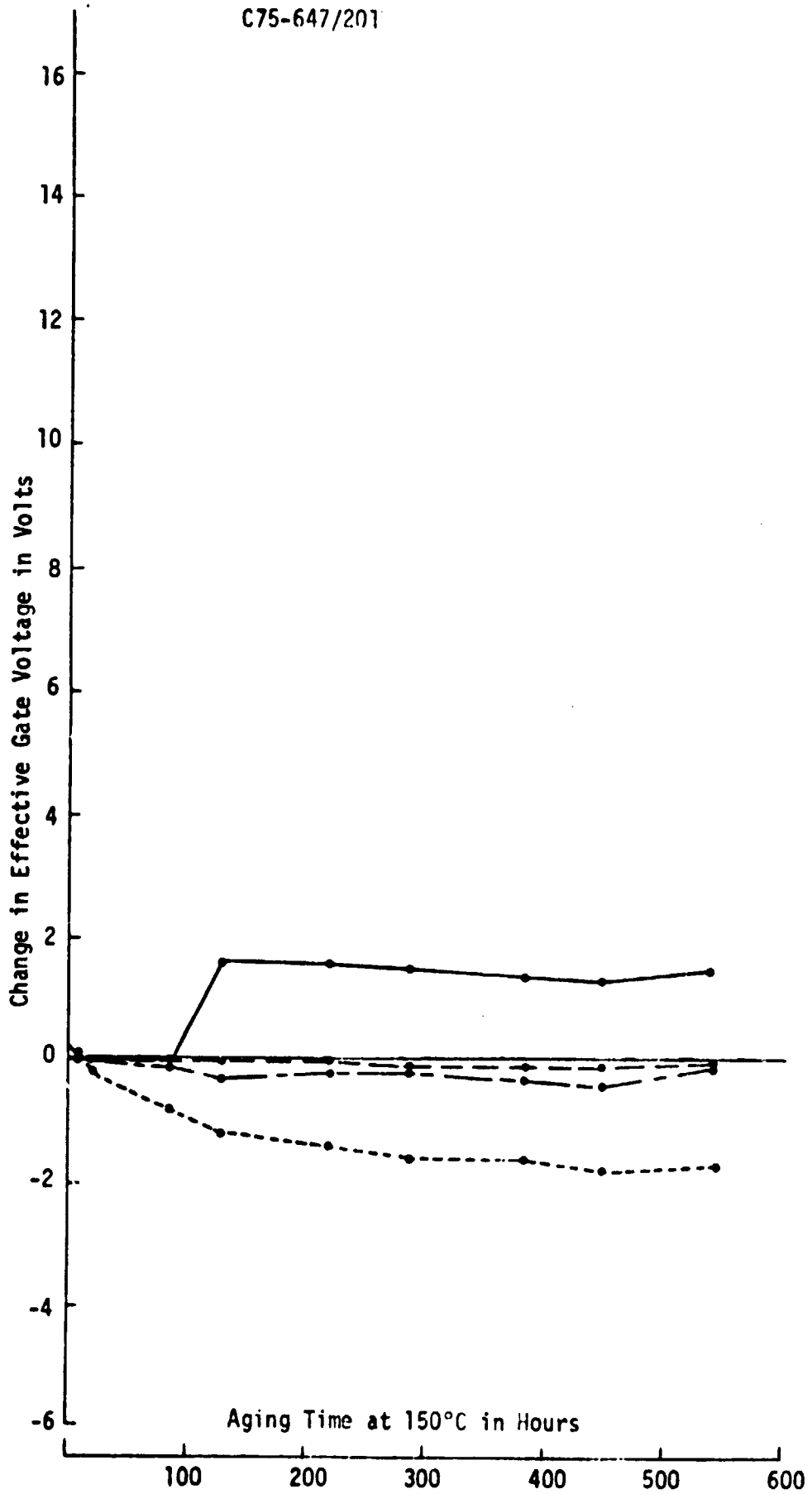
Figure 41. FET Test Specimen Containing 5.0 mg of Epo-Tek H61
