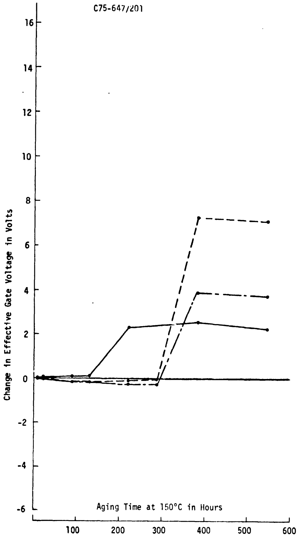
Figure 51. FET Test Specimen Containing 5.2 mg of DuPont 5504
