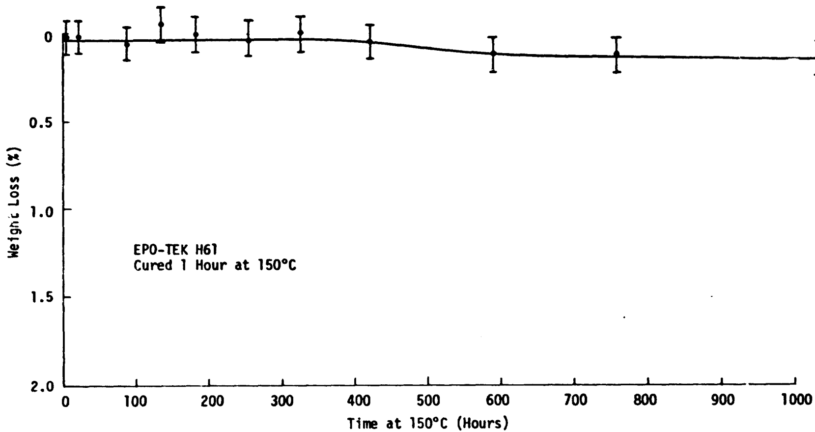
Figure 13. Weight Loss of Epo-Tek H61 at Constant Temperature (150°C) After Cure - As Measured on Analytical Balance
