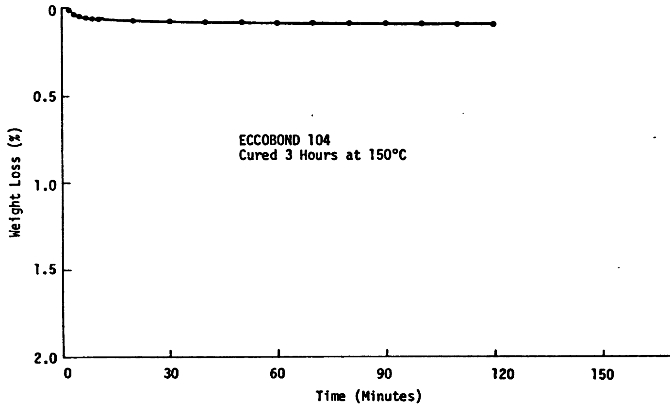
Figure 3. Weight Loss of Eccobond 104 at Constant Temperature (150°C) After Cure - As Measured on TGA Apparatus
