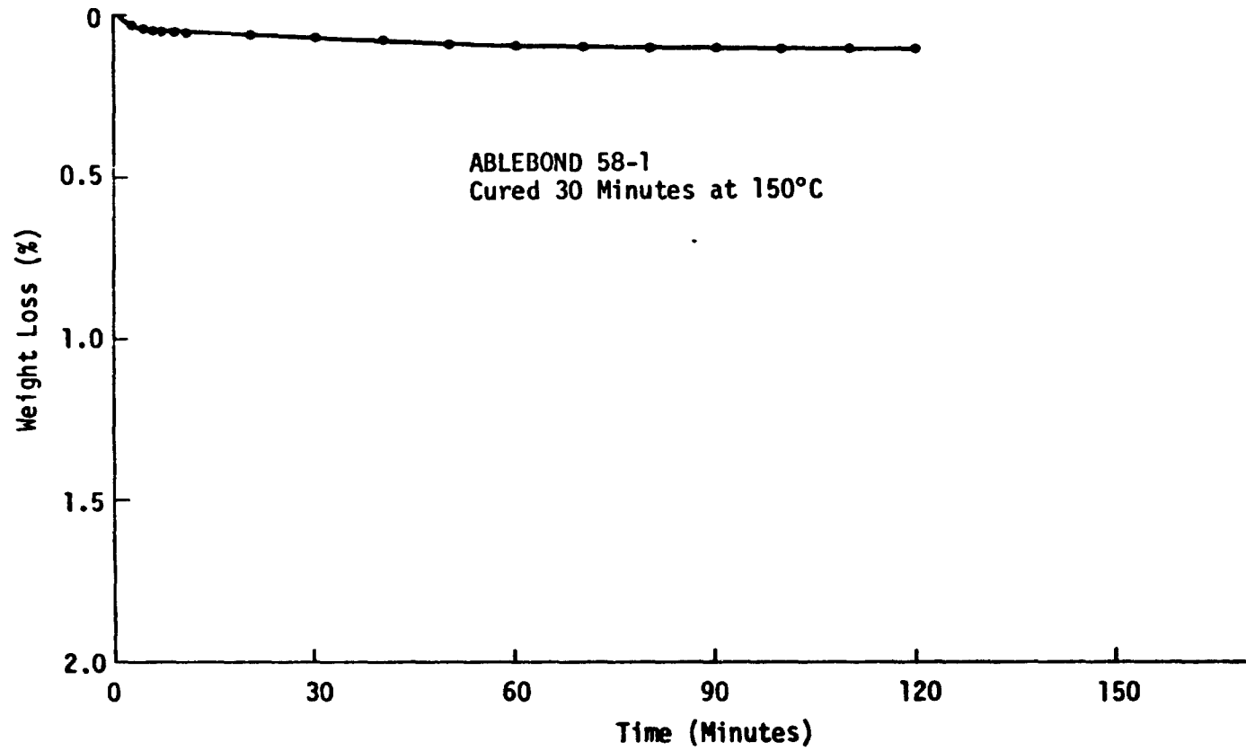
Figure 8. Weight Loss of Ablebond 58-1 at Constant Temperature (150°C) After Cure - As Measured on TGA Apparatus
