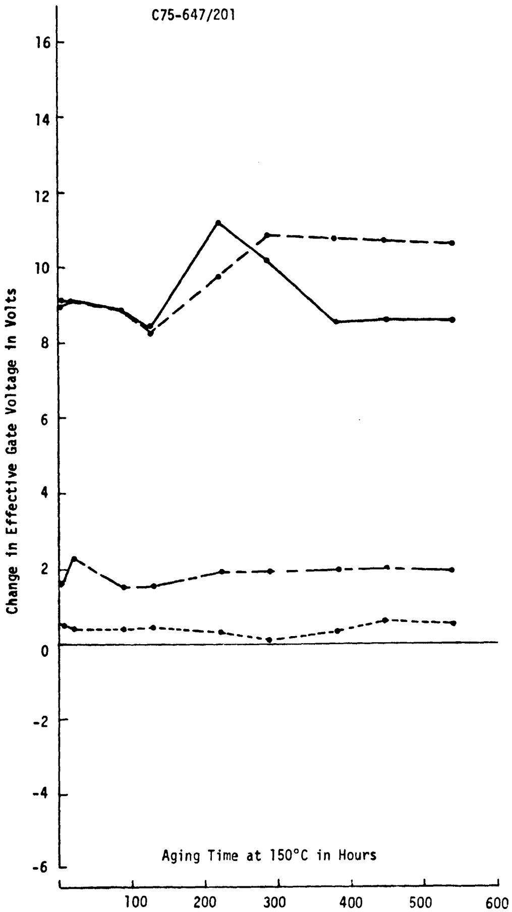
Figure 49. FET Test Specimen Containing 4.7 mg of EpoTek H31
