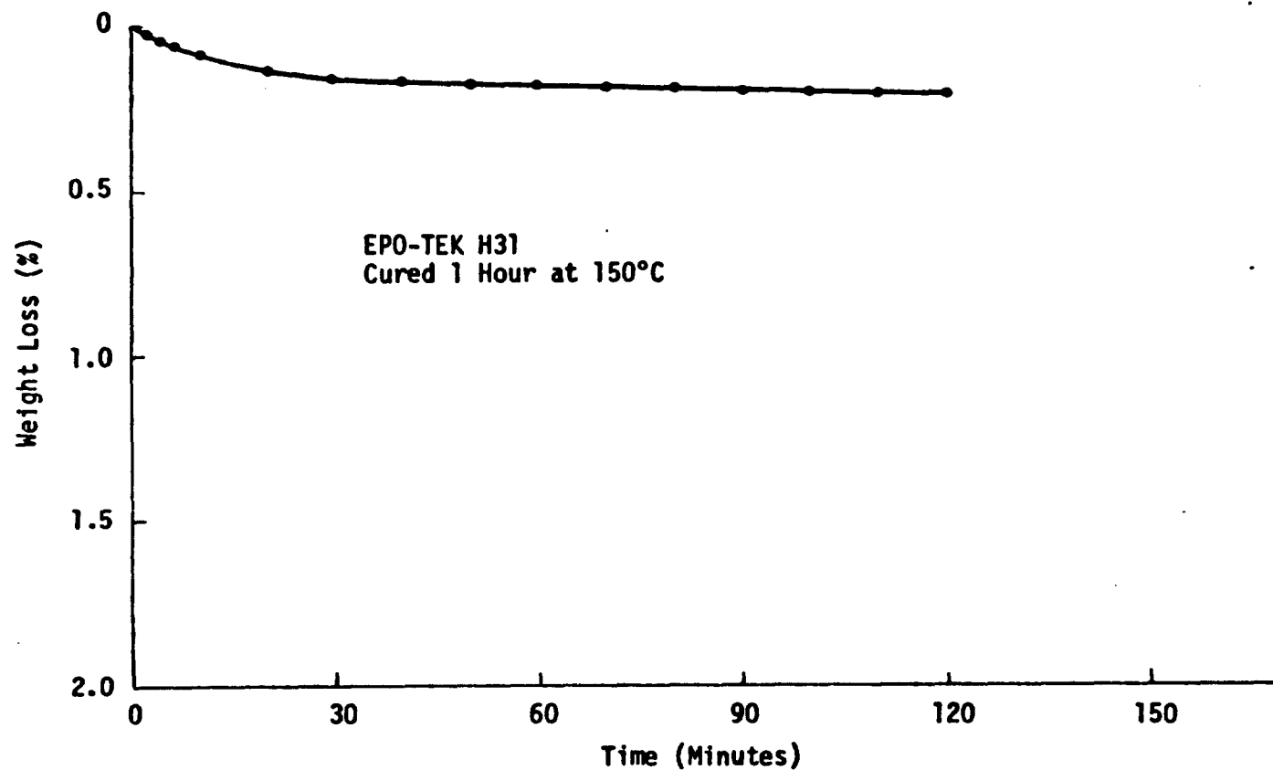
Figure 7. Weight Loss of Epo-Tek H31 at Constant Temperature (150°C) After Cure - As Measured on TGA Apparatus
