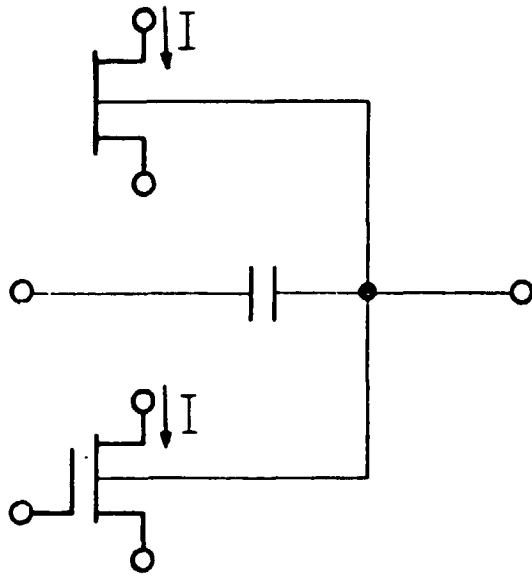
Figure 27. Schematic Circuit Diagram of FET Test Devices
