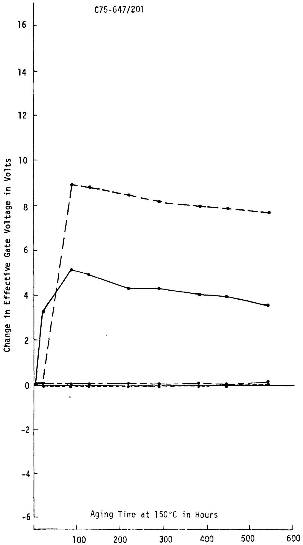
Figure 46. FET Test Specimen Containing 47.2 mg of Ablebond 36-2
