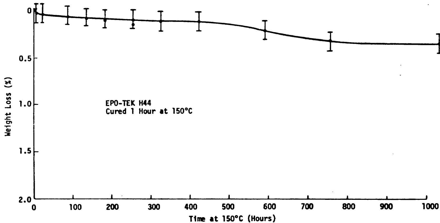
Figure 18. Weight Loss of Epo-Tek H44 at Constant Temperature (150°C) After Cure - As Measured on Analytical Balance
