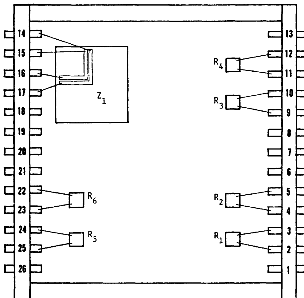
Figure 57. Layout of Thin Film Chip Resistor Test Specimens Containing Ten Times Amount of Adhesive Required to Mount Chips. R_1 through R_4 are Glass Passivated Thin Film Nichrome Chip Resistors. R_5 and R_6 are Unpassivated Thin Film Nichrome Chip Resistors. Z_1 is a Chip Containing an Aluminum Conductor Pattern (Shown in Detail in Figure 58.)
