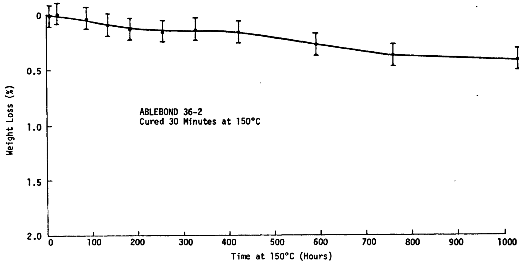
Figure 15. Weight Loss of Ablebond 36-2 at Constant Temperature (150°C) After Cure - As Measured on Analytical Balance
