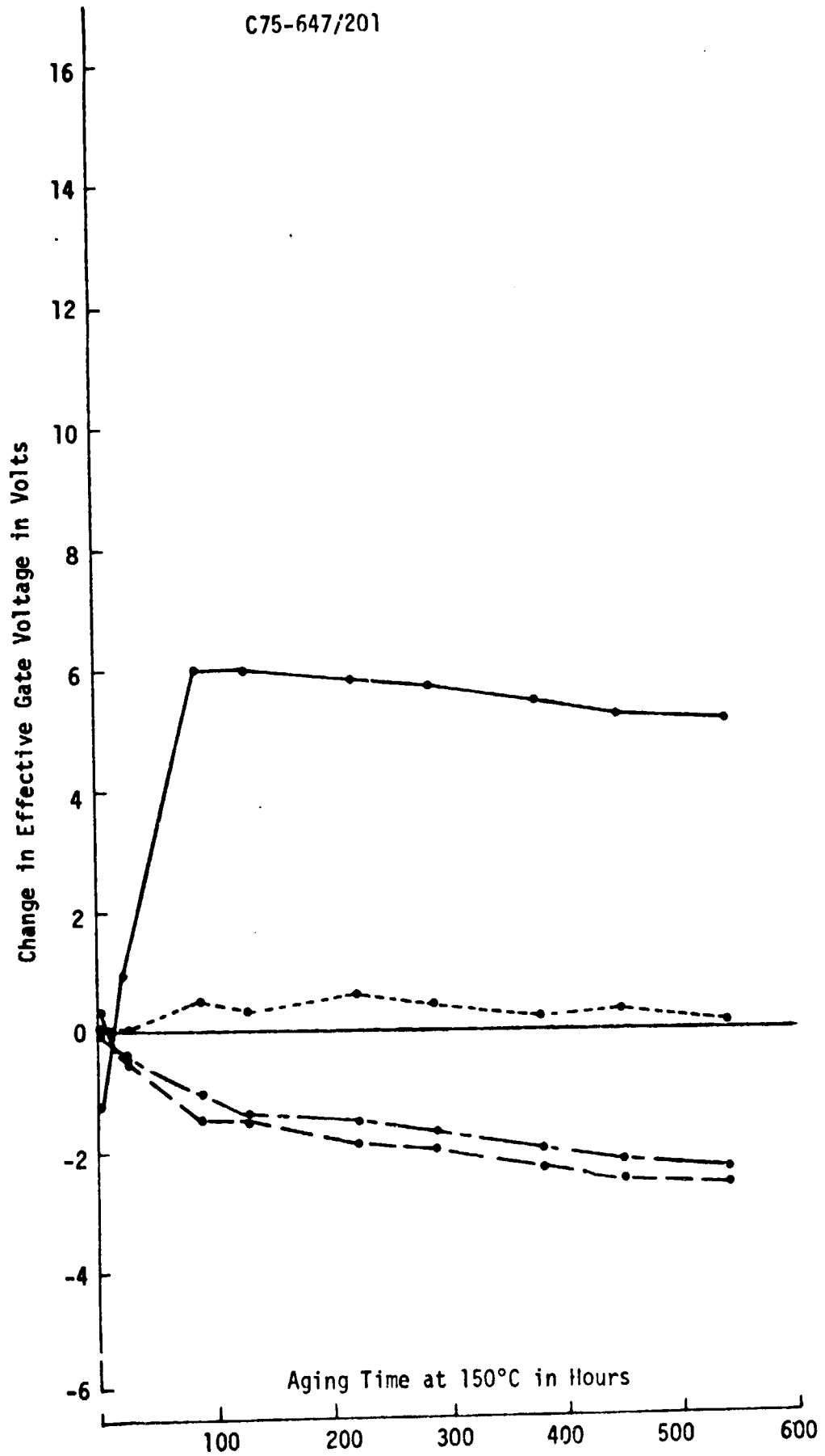
Figure 47. FET Test Specimen Containing 4.8 mg of Ablebond 36-2
