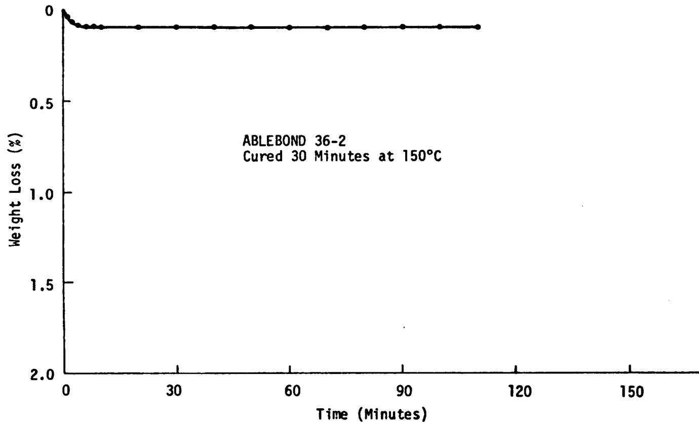
Figure 6. Weight Loss of Ablebond 36-2 at Constant Temperature (150°C) After Cure - As Measured on TGA Apparatus
