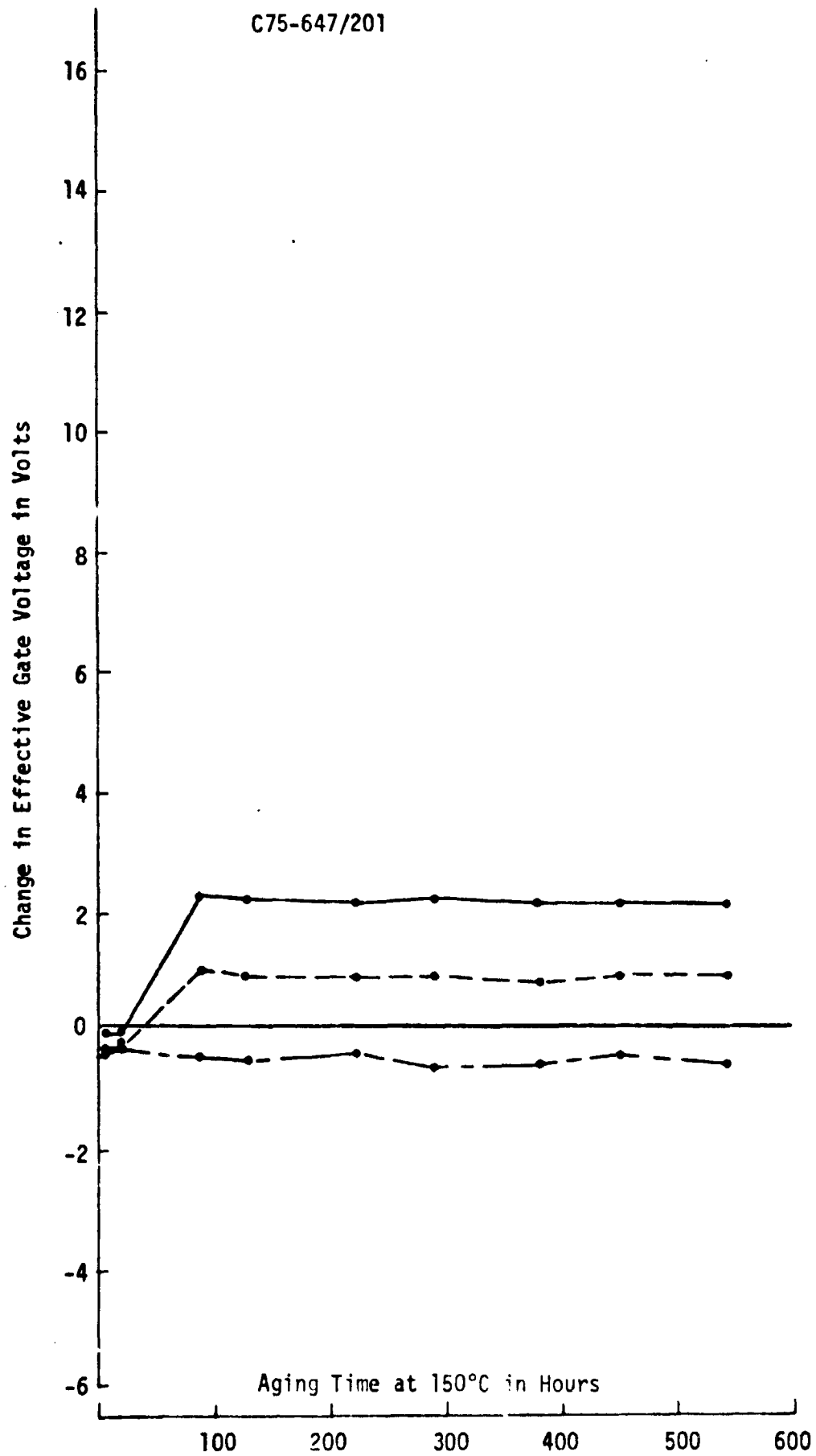
Figure 45. FET Test Specimen Containing 4.4 mg of Ablefilm 529
