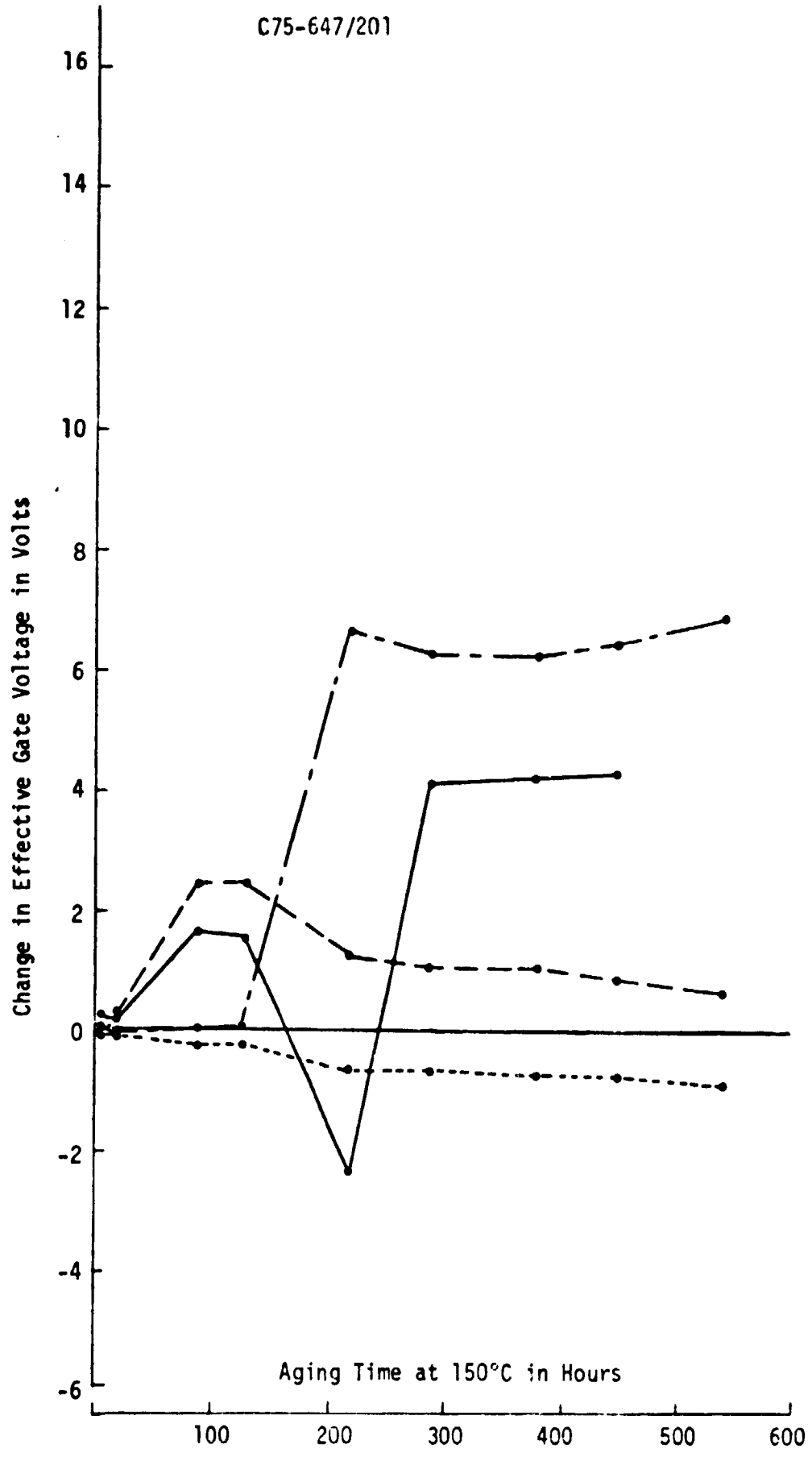
Figure 55. FET Test Specimen Containing 12.3 mg of Epo-Tek H44
