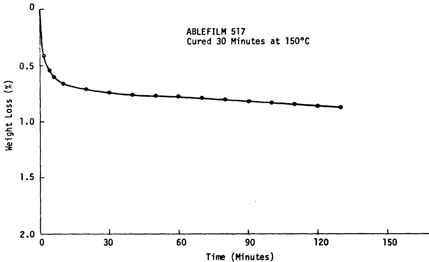
Figure 2. Weight Loss of Ablefilm 517 at Constant Temperature (150°C) After Cure - As Measured on TGA Apparatus
