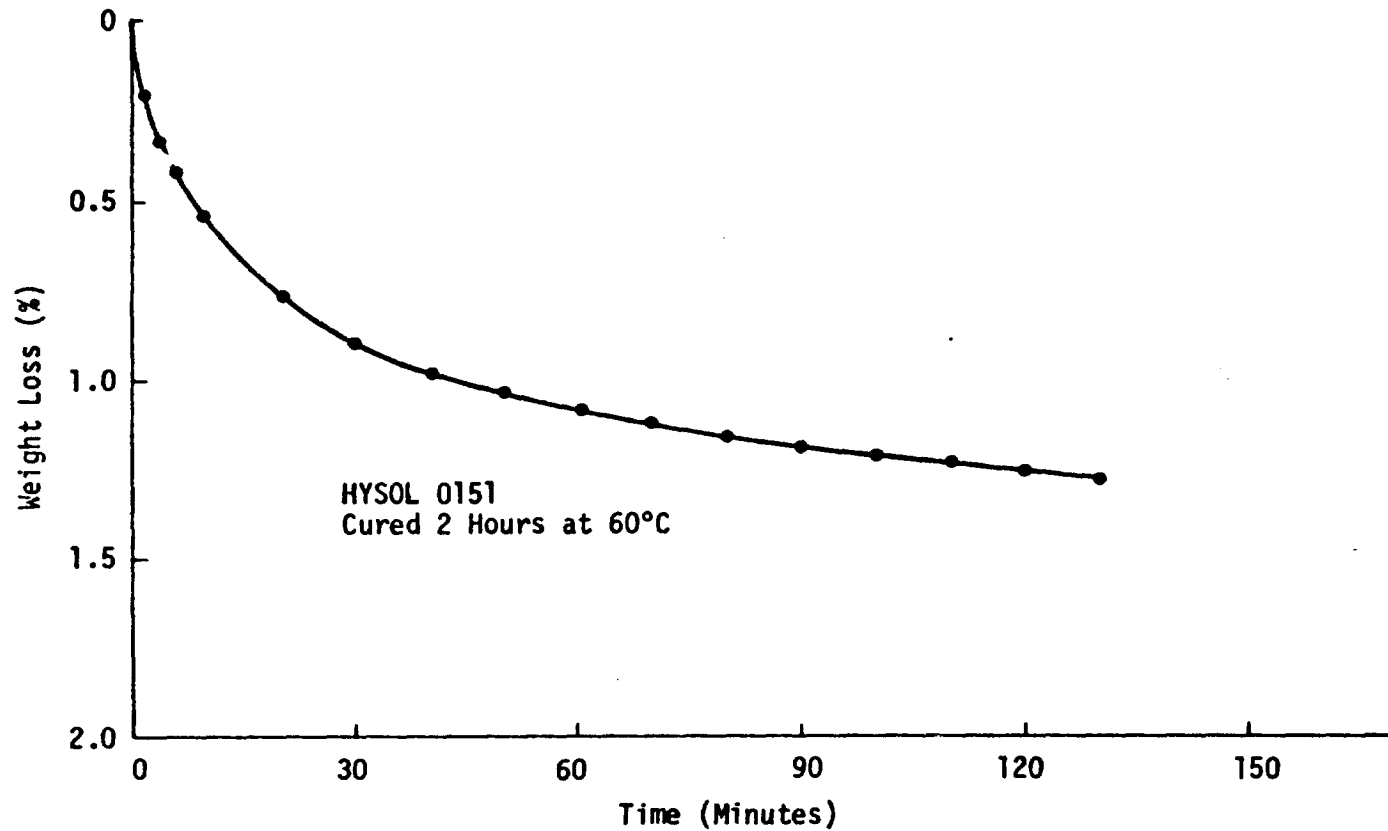
Figure 1. Weight Loss of Hysol 0151 at Constant Temperature (150°C) After Cure - As measured on TGA Apparatus
