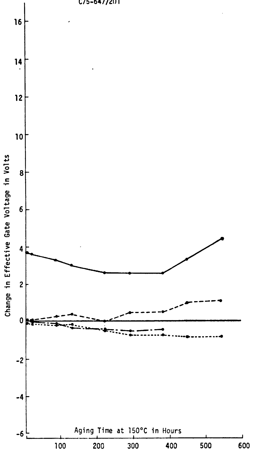
Figure 34. FET Test Specimen Containing 22.7 mg of Hysol 0151
