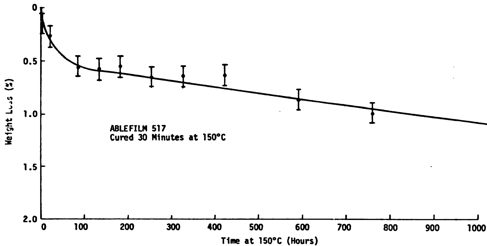
Figure 11. Weight Loss of Ablefilm 517 at Constant Temperature (150°C) After Cure - As Measured on Analytical Balance
