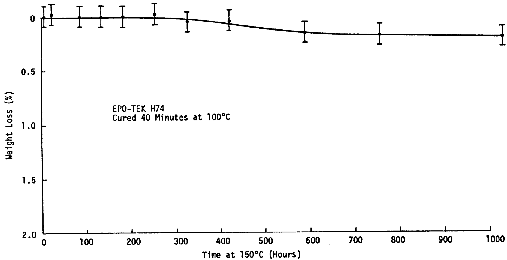
Figure 14. Weight Loss of Epo-Tek H74 at Constant Temperature (150°C) After Cure - As Measured on Analytical Balance
