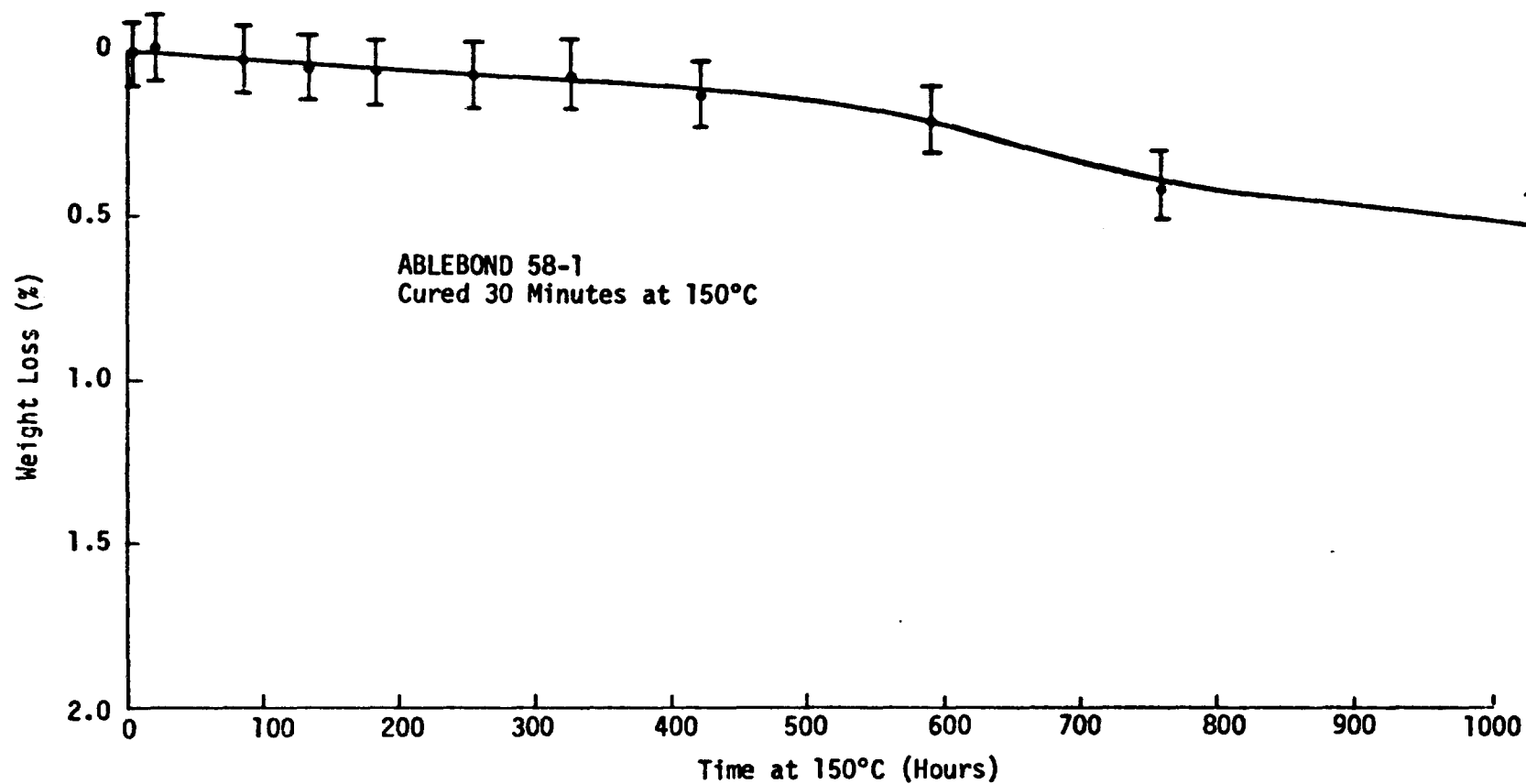
Figure 17. Weight Loss of Ablebond 58-1 at Constant Temperature (150°C) After Cure - As Measured on Analytical Balance
