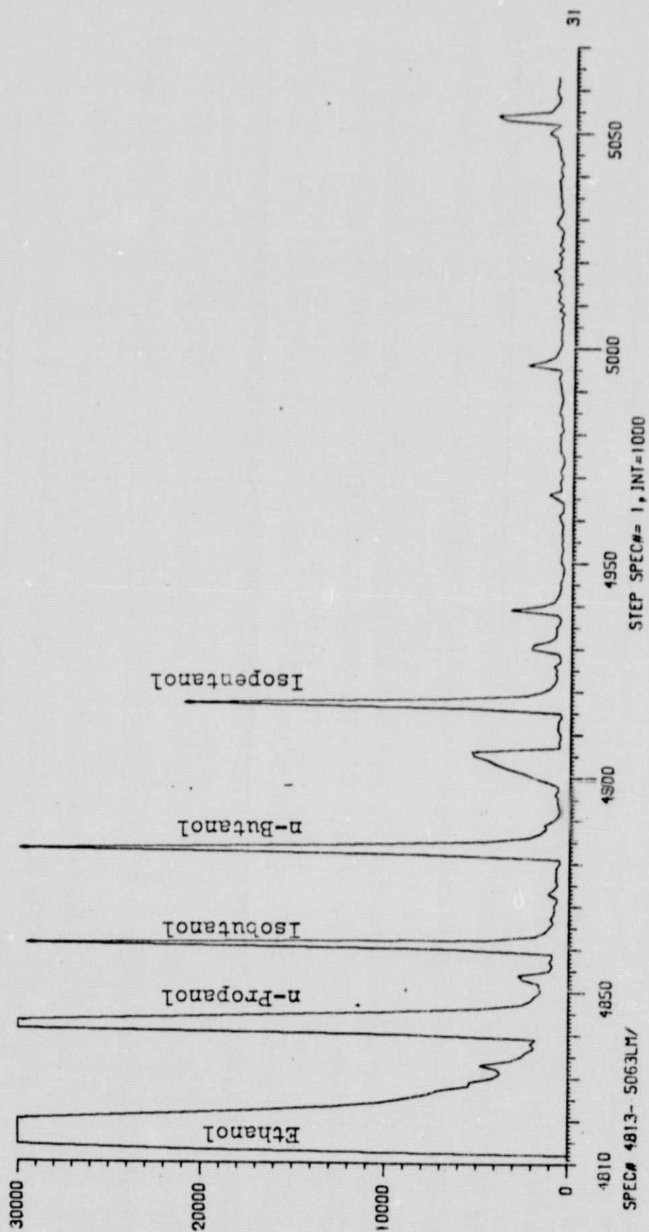
Figure 2 Mass Fragmentogram of Primary Alcohols, M/E 31 (diabetic urine) - patient shown in Figure 1.
