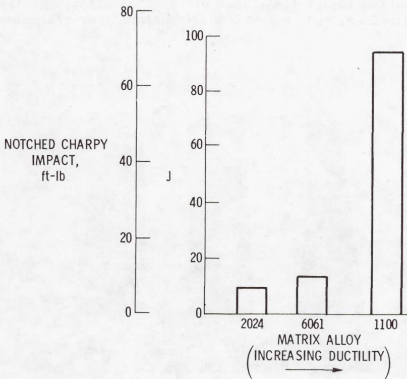
Figure 6.- Effect of matrix ductility on impact strength of boron/aluminum composites. Boron fiber content, 50 vol %; fiber diameter, 0.02 cm.
