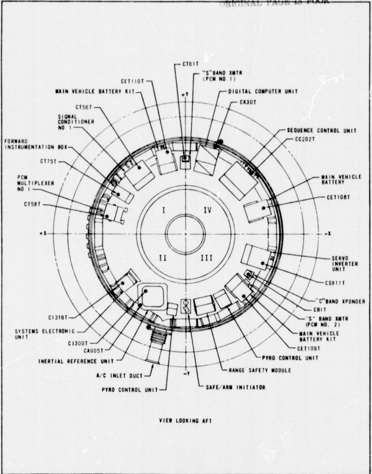
Figure 2B CENTAUR Forward Equipment Module
