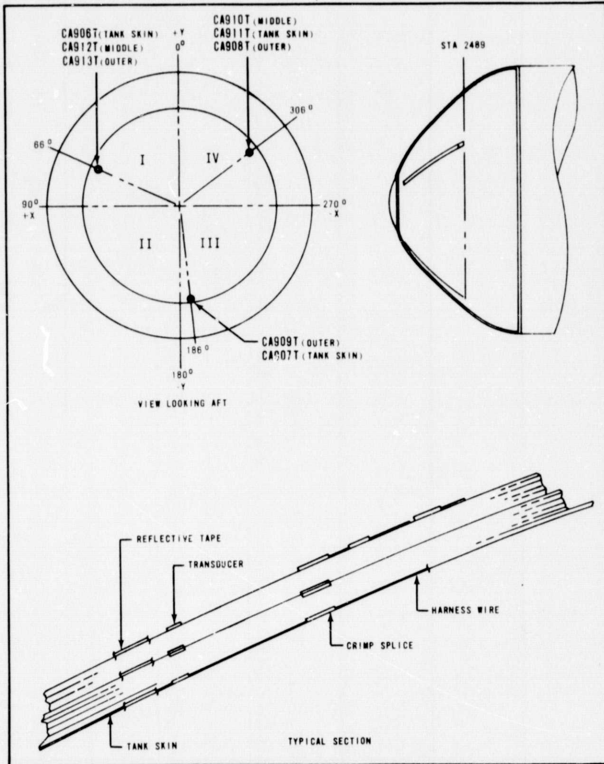
Figure 2A CENTAUR Forward Bulkhead Temperatures
