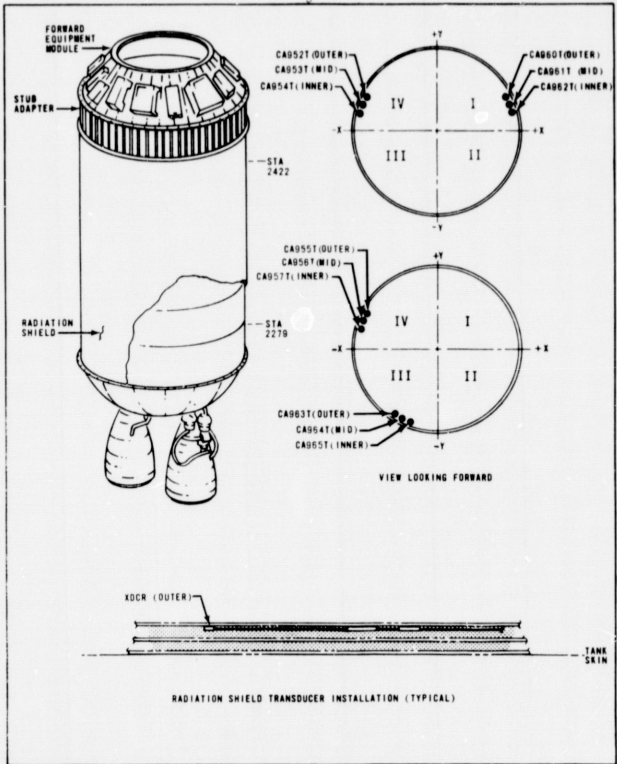
Figure 2C CENTAUR Tank Radiation Shield Temperature
