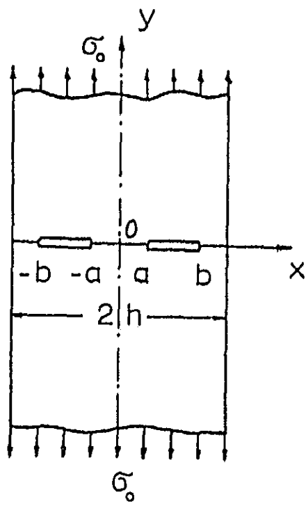
Figure 1. Infinite strip with two internal cracks.
