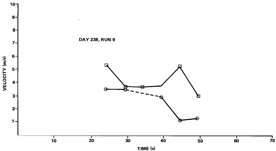
Figure 31. Velocity time history dust devil no. 1.
