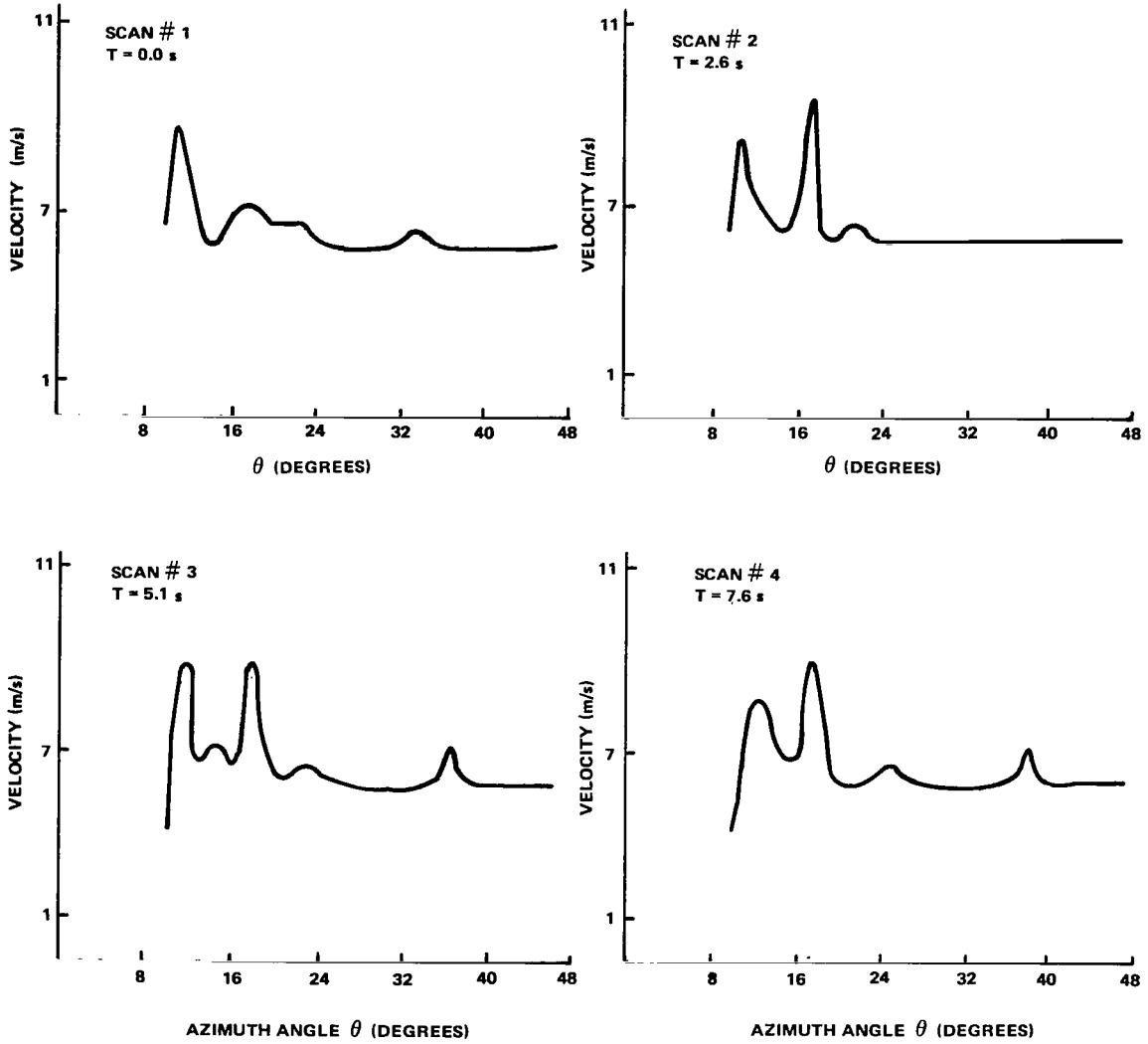
DAY 235 RUN 5 ELEVATION = 5° Figure 21. Velocity versus azimuth.
