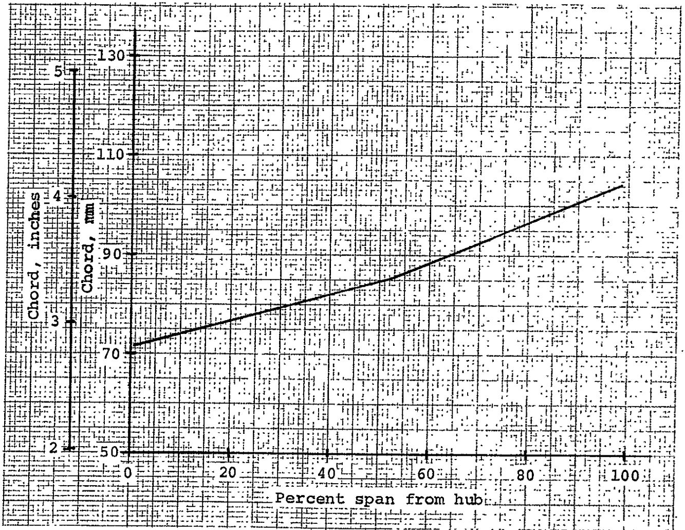
Figure 17. Rotor chord
