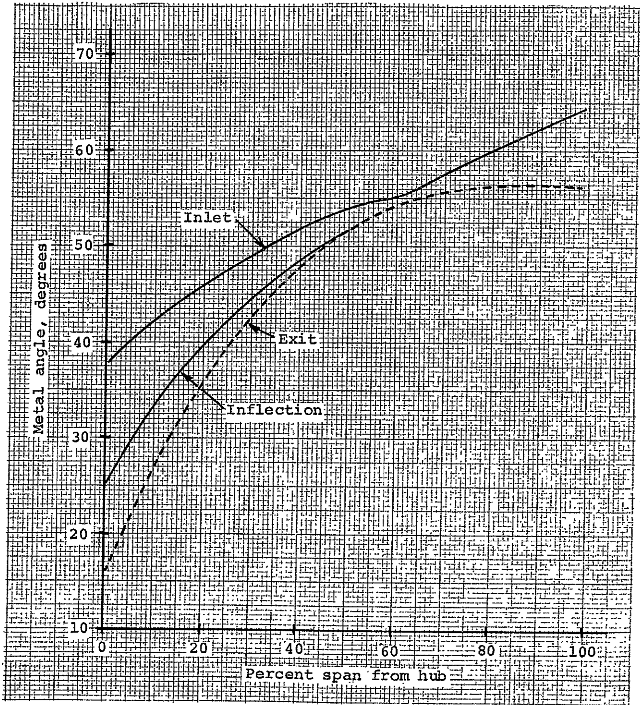
Figure 21. Rotor metal angles
