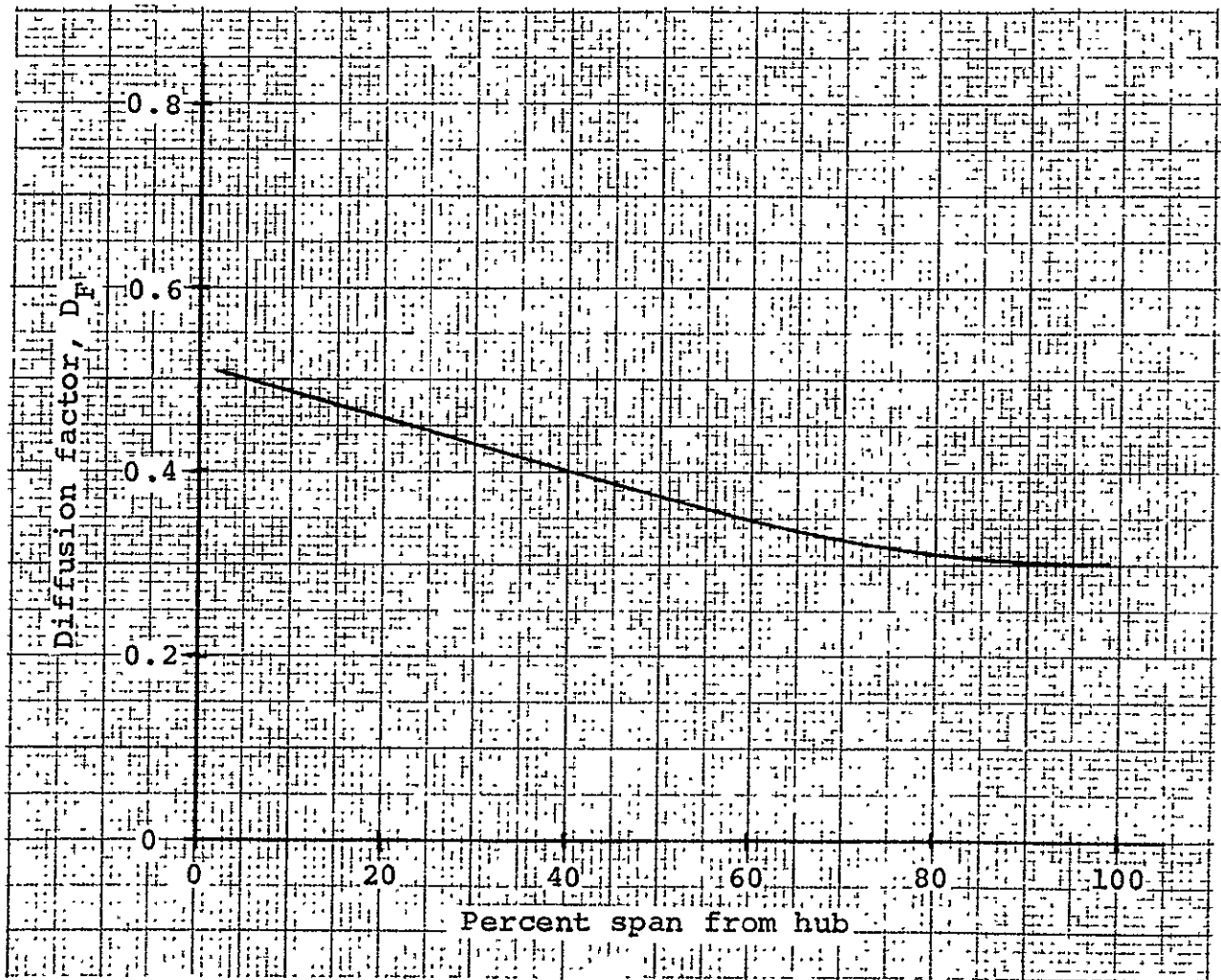
Figure 5. Rotor diffusion factor
