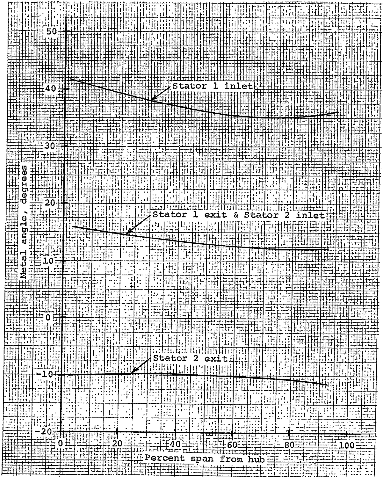
Figure 25. Radial metal angle distribution for the stators
