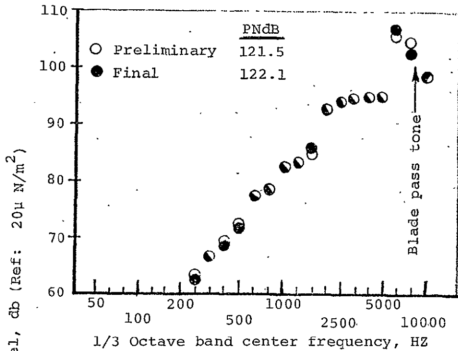
29a. Inlet noise at 50° from axis
