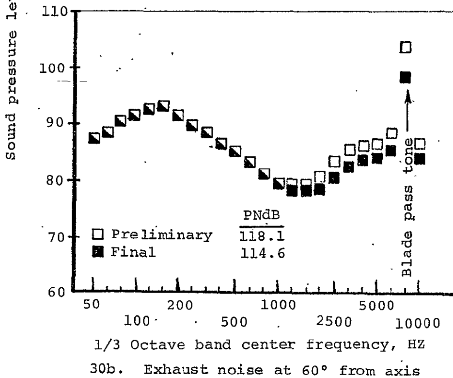
Figure 30. Comparison of rig test noise levels estimated for QHF fan preliminary and final designs - approach condition at 5m (16.4 ft) radius
