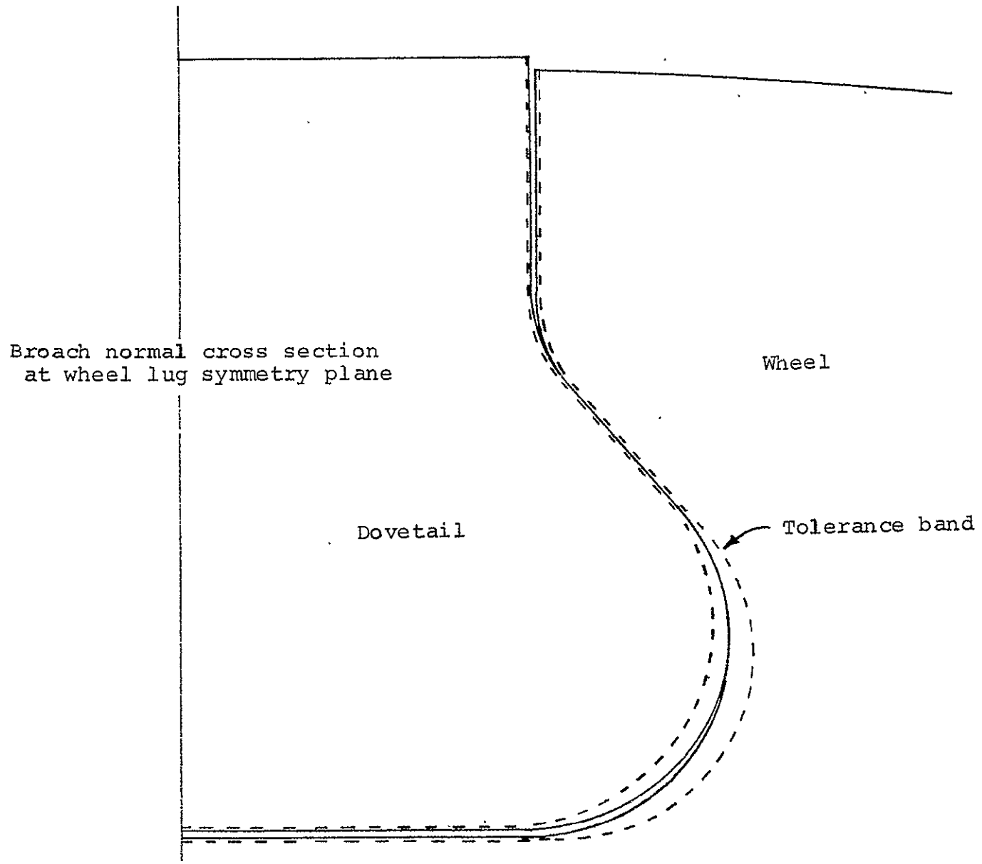
Figure 41. Dovetail attachment
