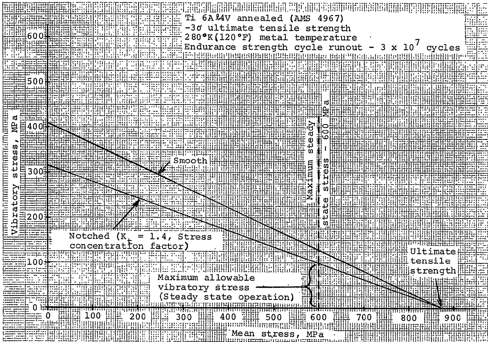
Figure 38. Modified Goodman diagram - blade fillet region
