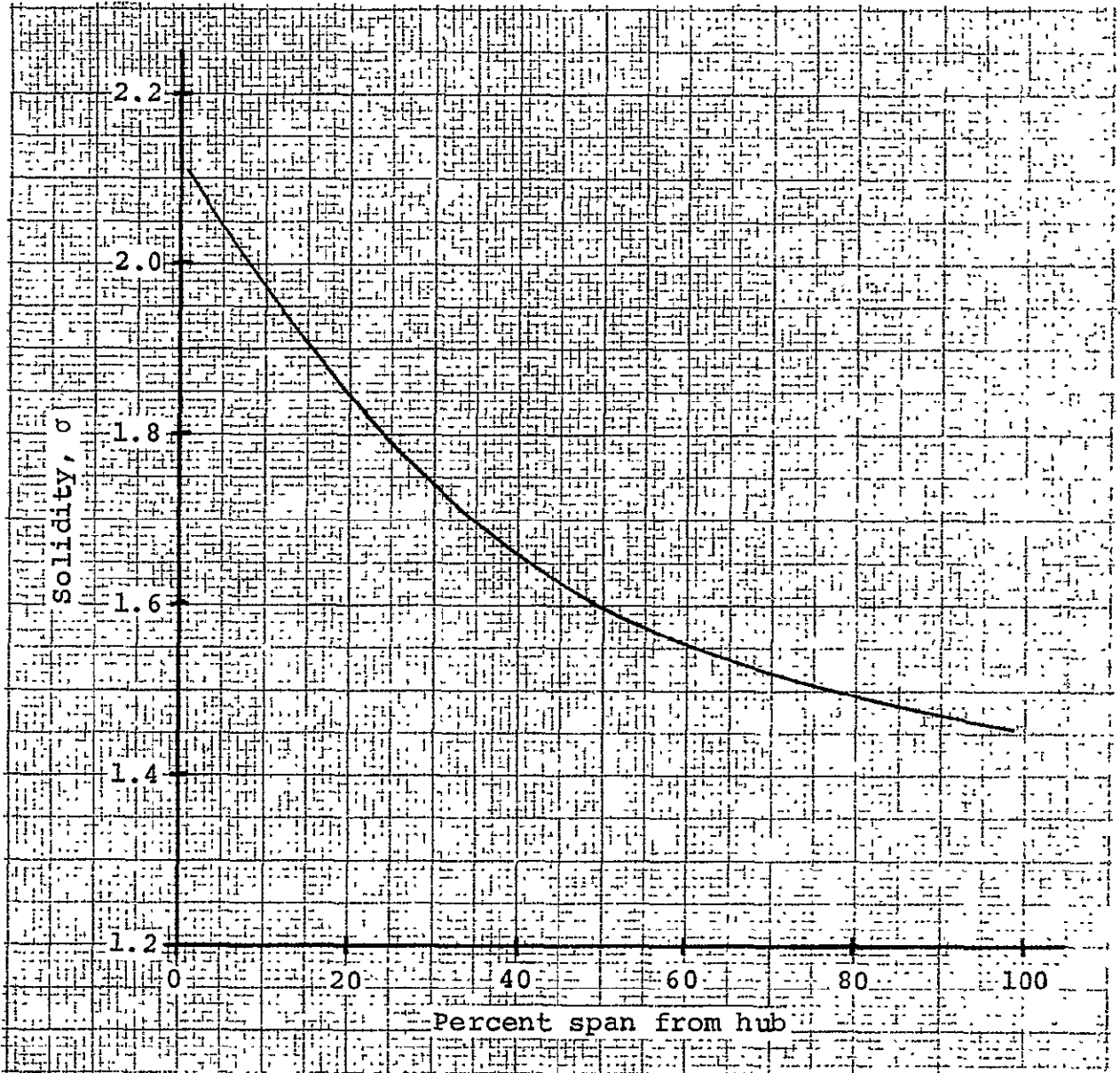
Figure 16. Rotor solidity
