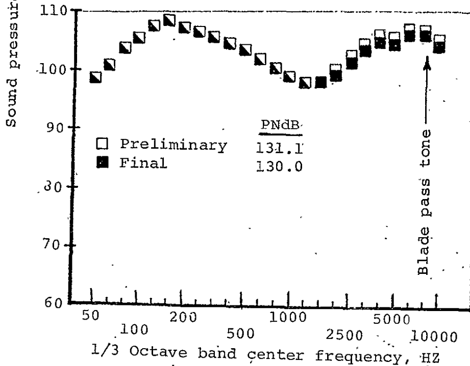
29b. Exhaust noise at 60° from axis
