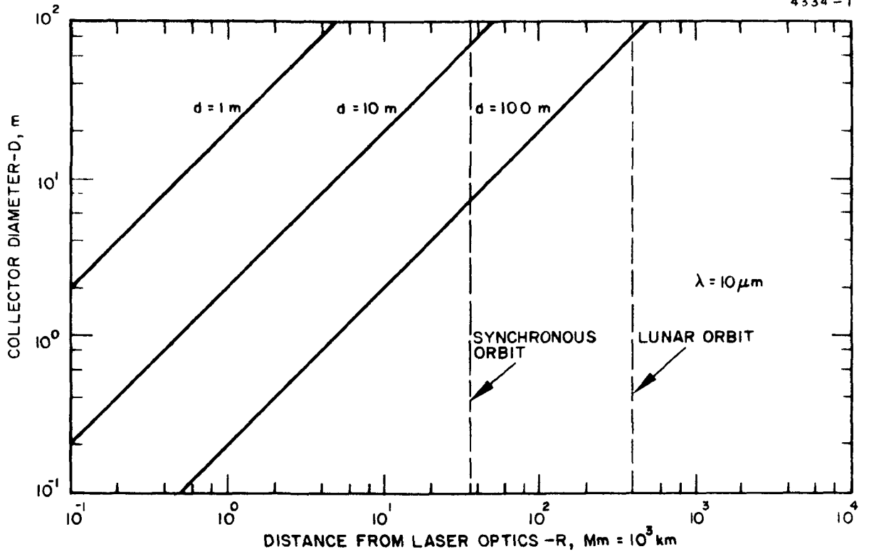
Fig. B-2. Range/optical diameter relations for 10 μm laser radiation.
