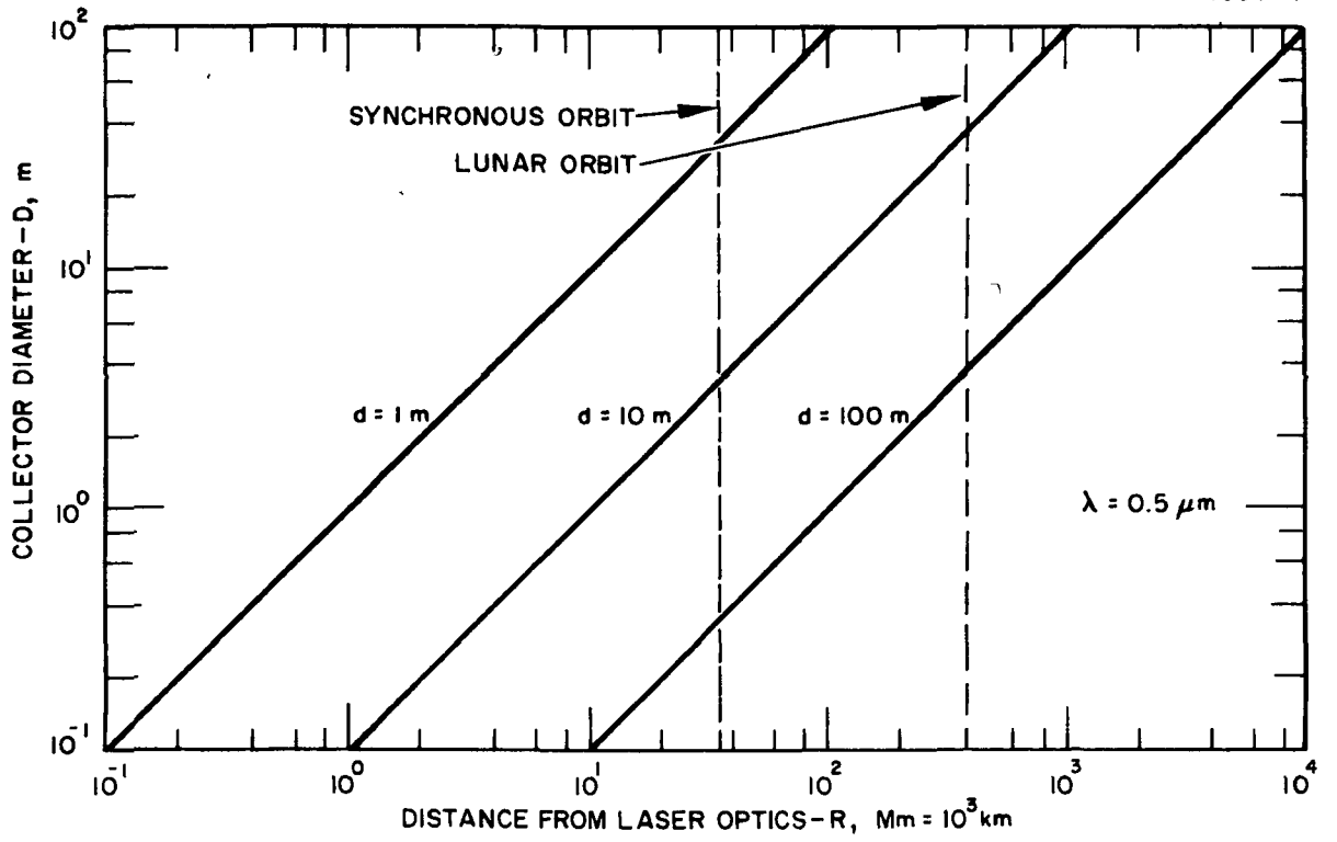
Fig. B-4. Range/optical diameter relations for 0.5 μm laser radiation.
