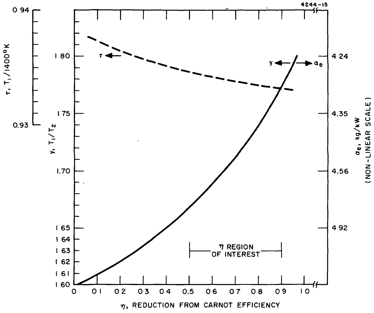
Fig. G-2. Optimization of SEP Thermal Cycle System with Ehrlicke Sphere.
