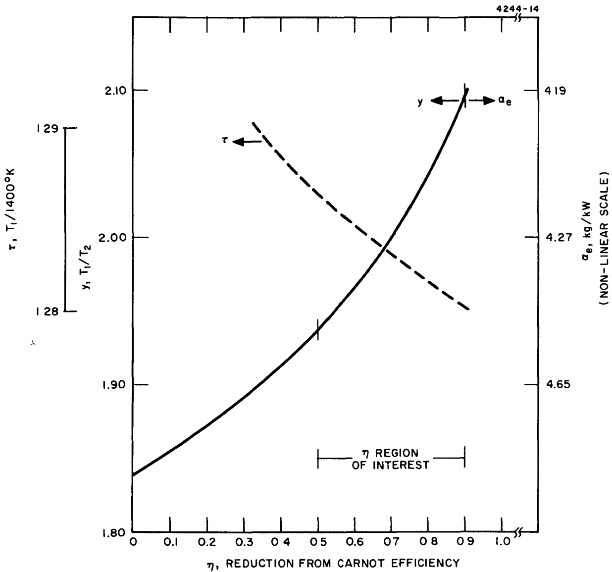
Fig. G-3. Optimization of LEP thermal cycle system with Ehrlicke Sphere.
