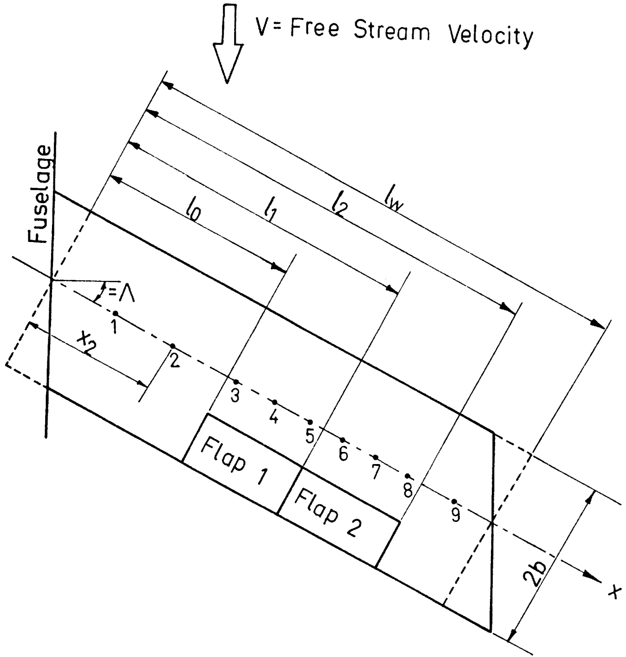
Fig. 1. Swept wing with two flaps and nine node points.
