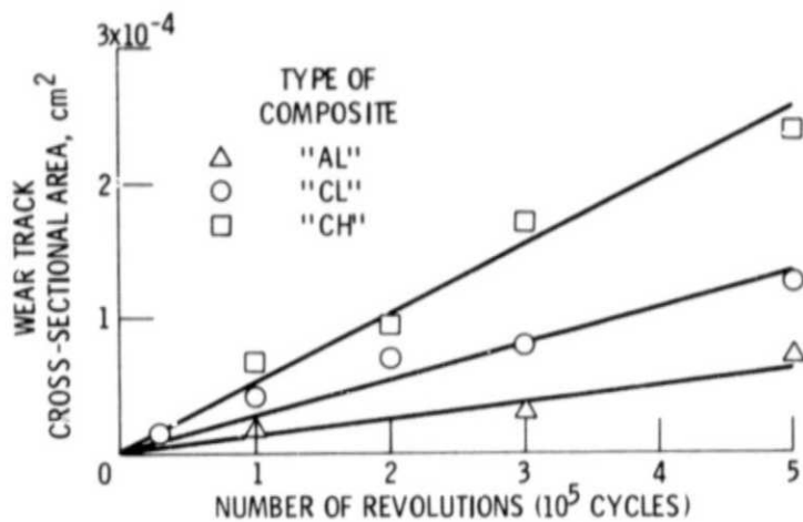
Figure 4. - Composite film wear at 25^\circ\text{C} in a moist air atmosphere ( 10\,000\text{ ppm H}_2\text{O} ) as a function of the number of sliding revolutions.
