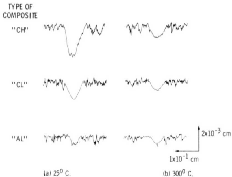
Figure 5. - Surface profiles of composite wear tracks taken after 300 000 cycles of sliding in a moist air atmosphere ( 10\,000\text{ ppm H}_2\text{O} ).
