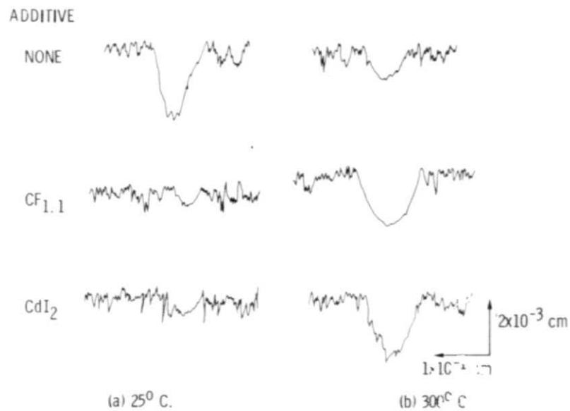
Figure 8. - Effect of additives on the wear of type "CH" composites after sliding in a moist air atmosphere (10 000 ppm H 2 O) for 300 000 cycles.
