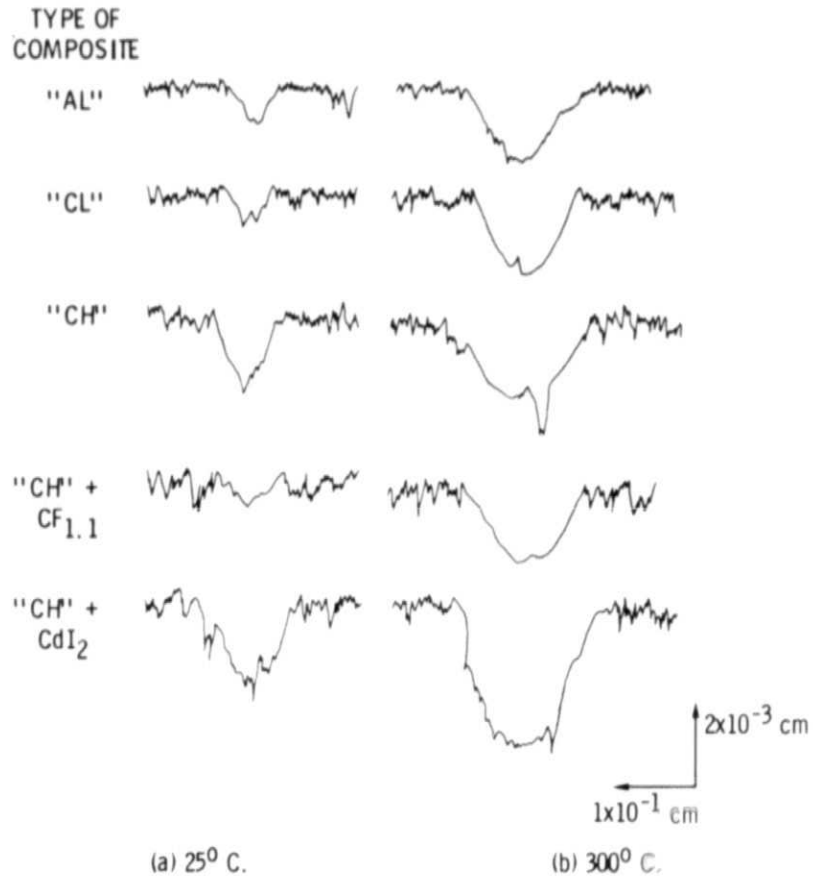
Figure 10. - Effect of a dry air atmosphere ( < 20 ppm H_2O ) on the wear of polyimide composites after 300 000 cycles of sliding at (a) 25 0 C and (b) 300 0 C.
