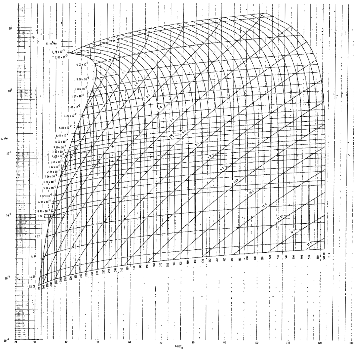
Figure 1.- Pressure enthalpy diagram for \text{CBrF}_3 with lines of constant entropy, volume, and temperature.
