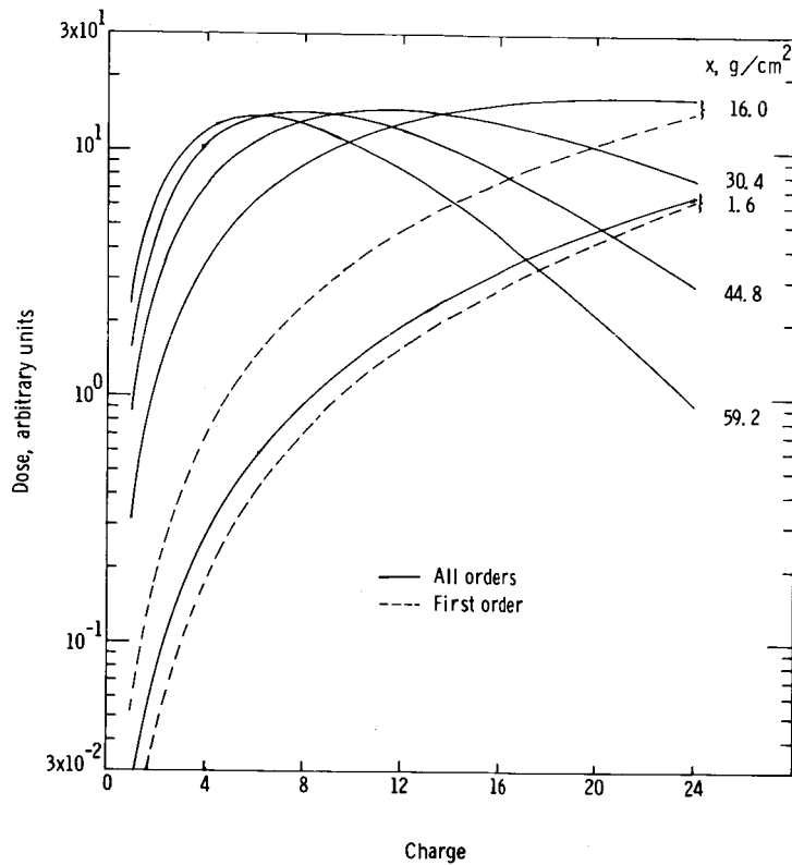
Figure 5.- Dose contribution from various ion types in Earth's atmosphere due to normally incident high-energy iron group ion integrated flux ( 1/\text{cm}^2 ).
