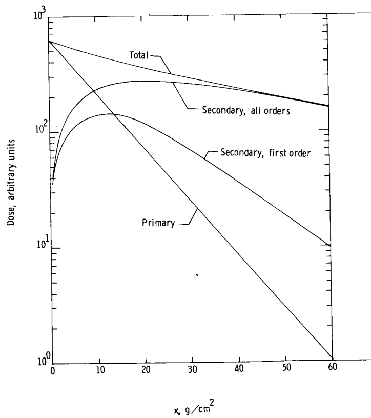
Figure 4.- Dose in Earth's atmosphere due to normally incident iron group integrated flux (1/cm 2 ) of high energy.
