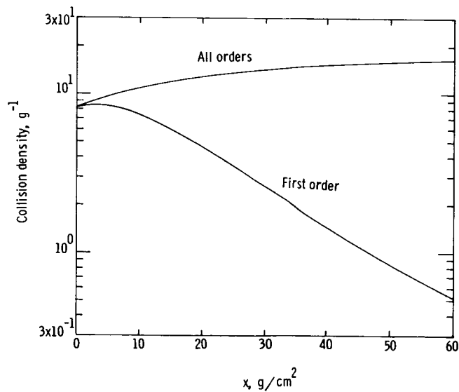
Figure 6.- Density of nuclear reactions with air nuclei produced by normally incident iron group ion integrated flux ( 1/\text{cm}^2 ) and all secondary fragments.
