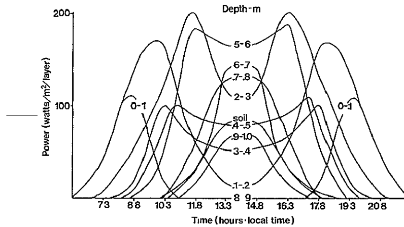
Figure 10. Solar flux, ABik, intercepted by foliage (or soil) in each layer of the wheat canopy for 30 July 1975.
