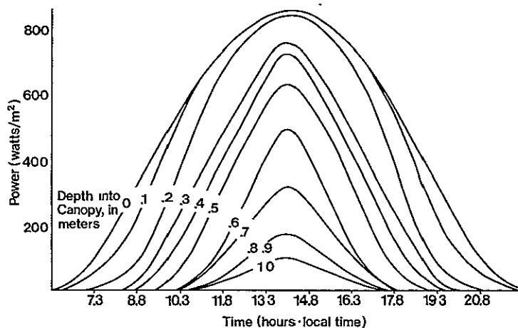
Figure 9. Solar flux, AF_{ik} , for 30 July 1975.
