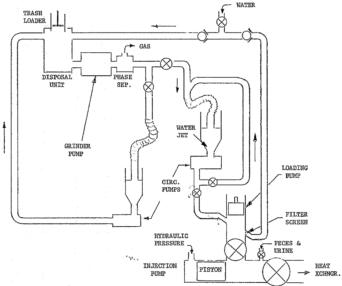
Fig. 17 TRASH LOADING CONCEPT B
