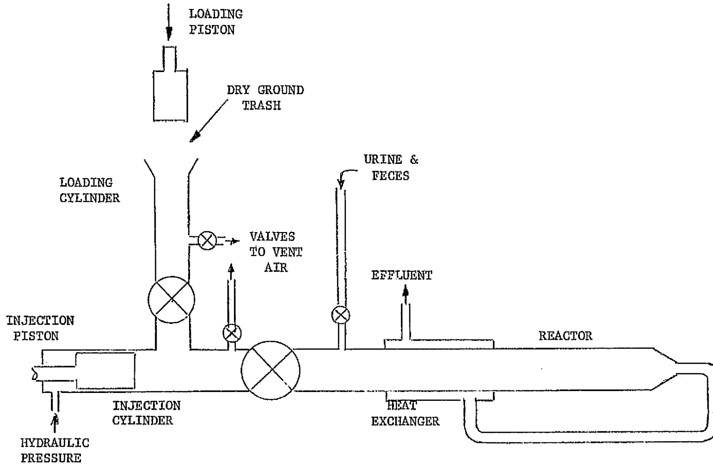
Fig. 18 Trash Loading Concept C
