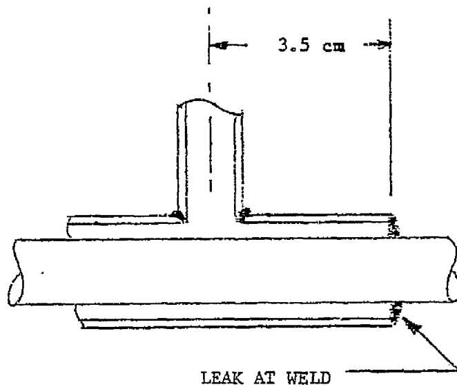
ORIGINAL HEAT EXCHANGER DETAIL
