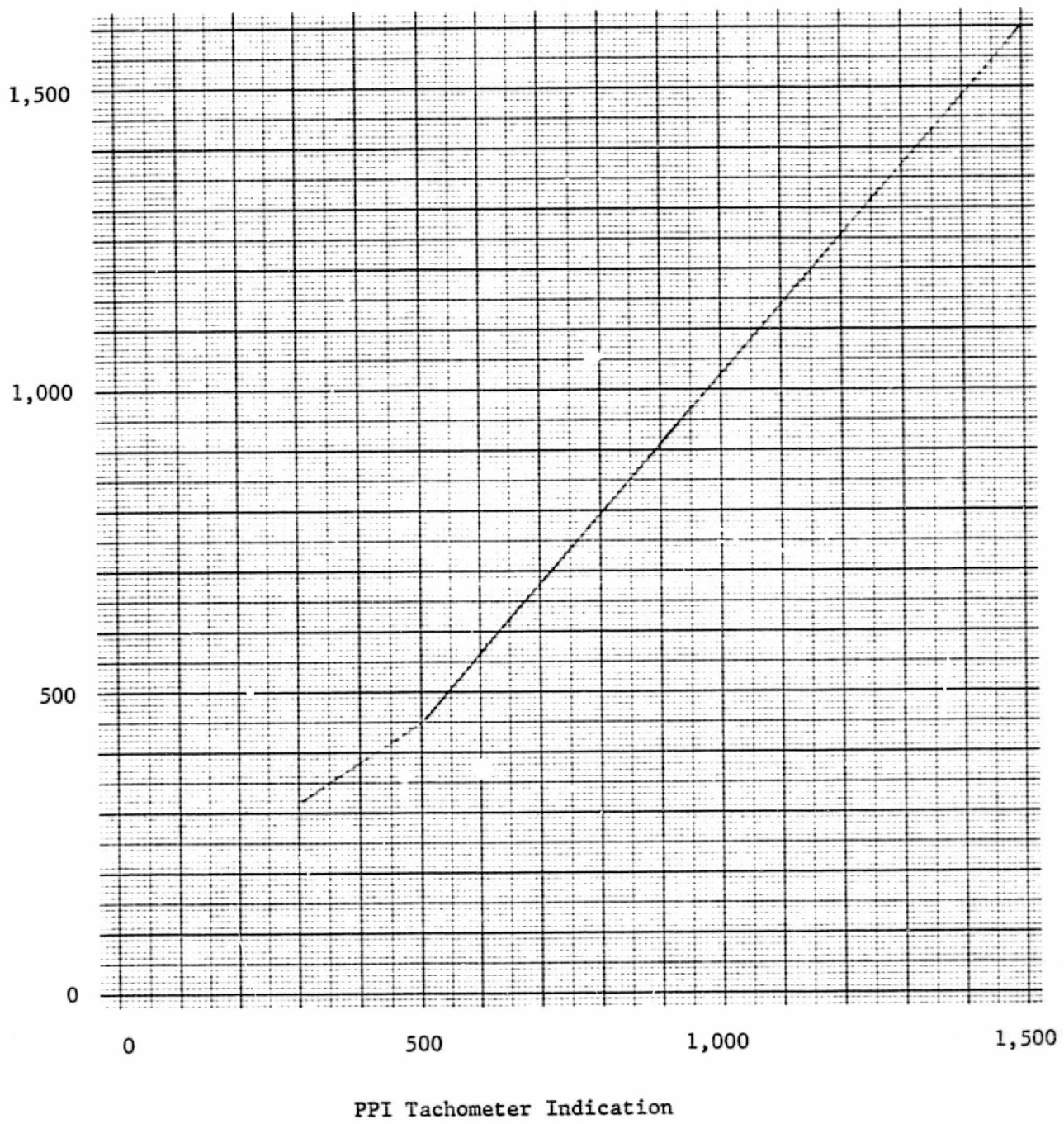
Fig. 7 Reactor Stirring Rate Calibration
