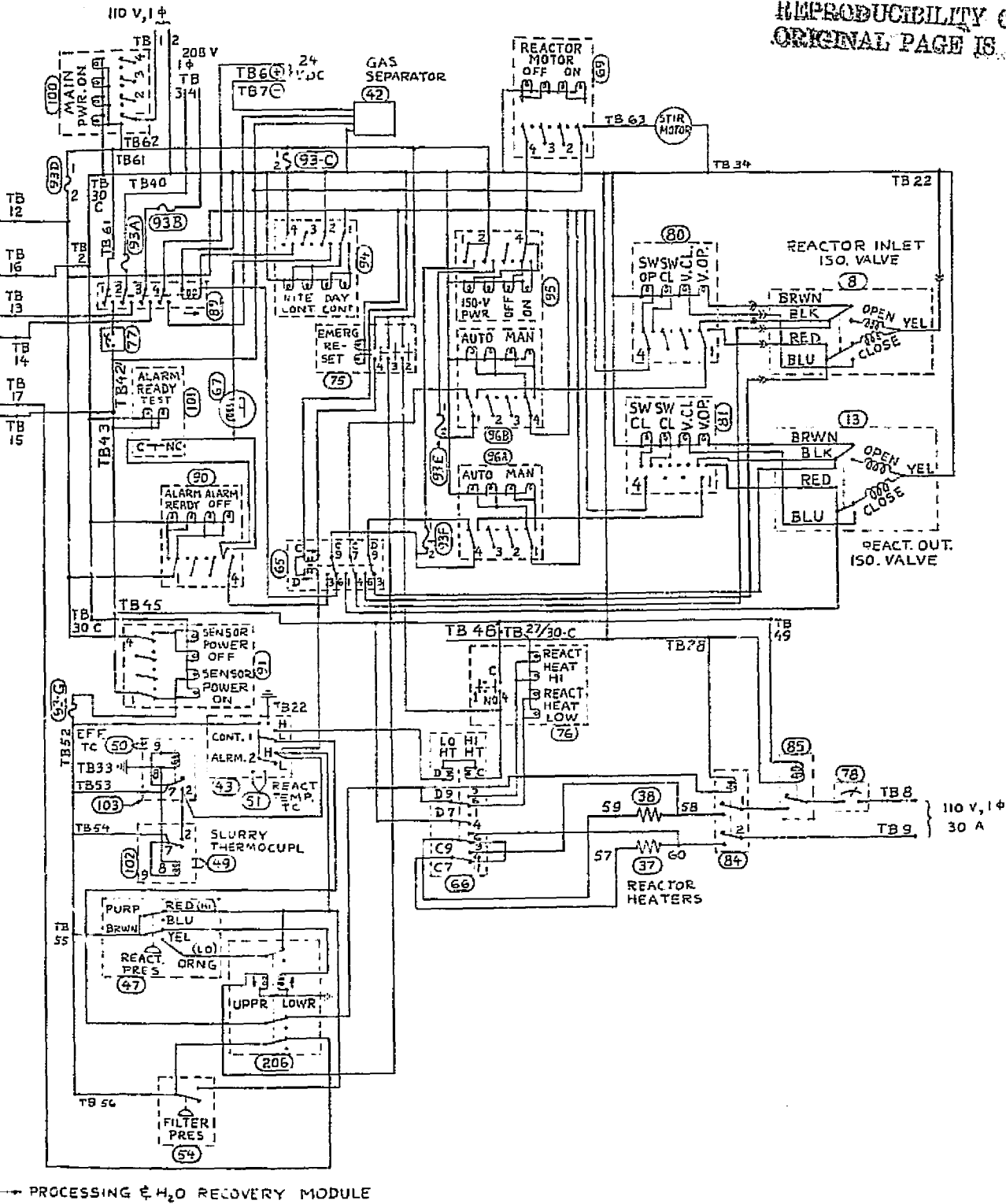
Figure 5 Electrical Schematic Diagram
