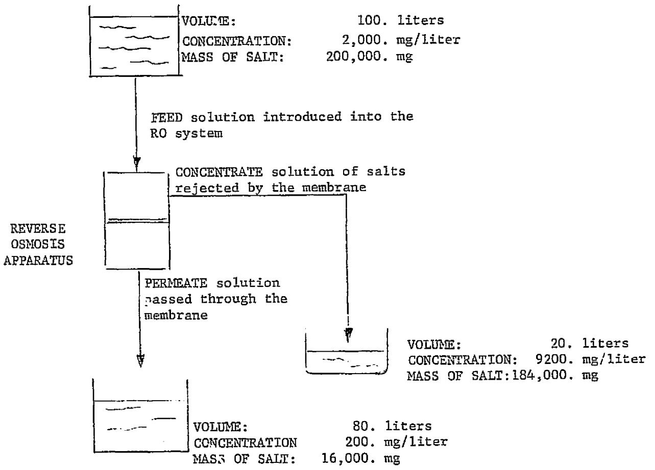
Fig. 13 Reverse Osmosis System as Separator and Concentrator
