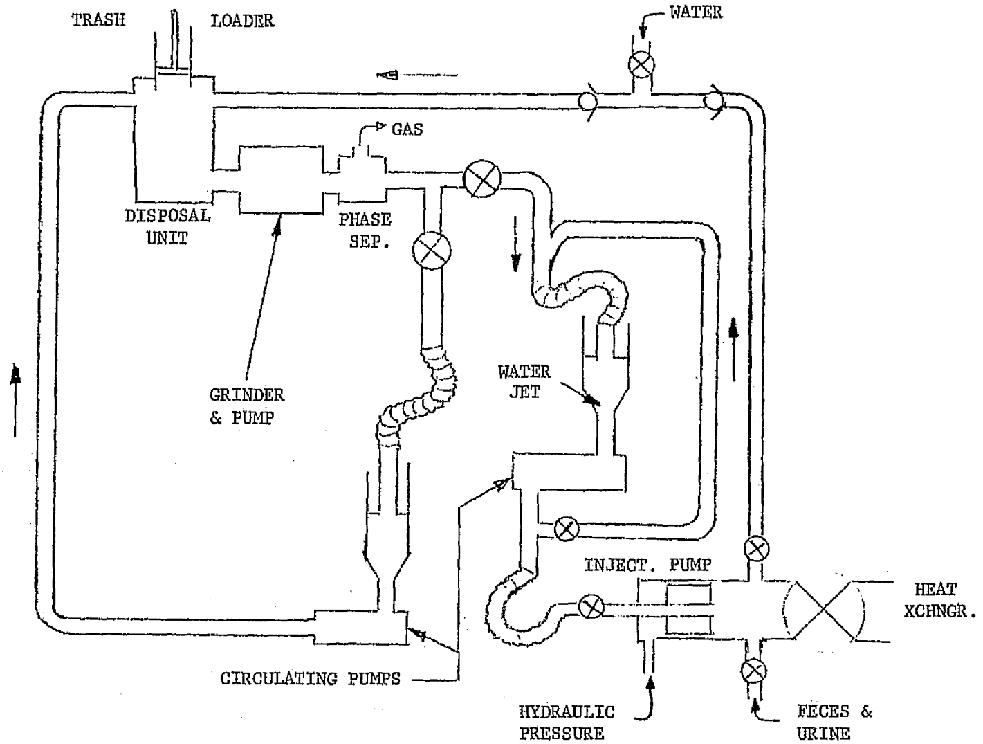
Fig. 16 TRASH LOADING CONCEPT A
