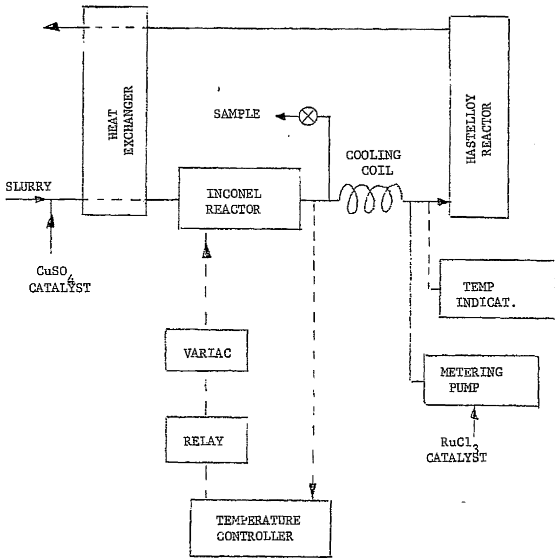
Figure 15 ADDITION OF FIRST STAGE REACTOR & AUXILIARIES TO WET OXIDATION SYSTEM
