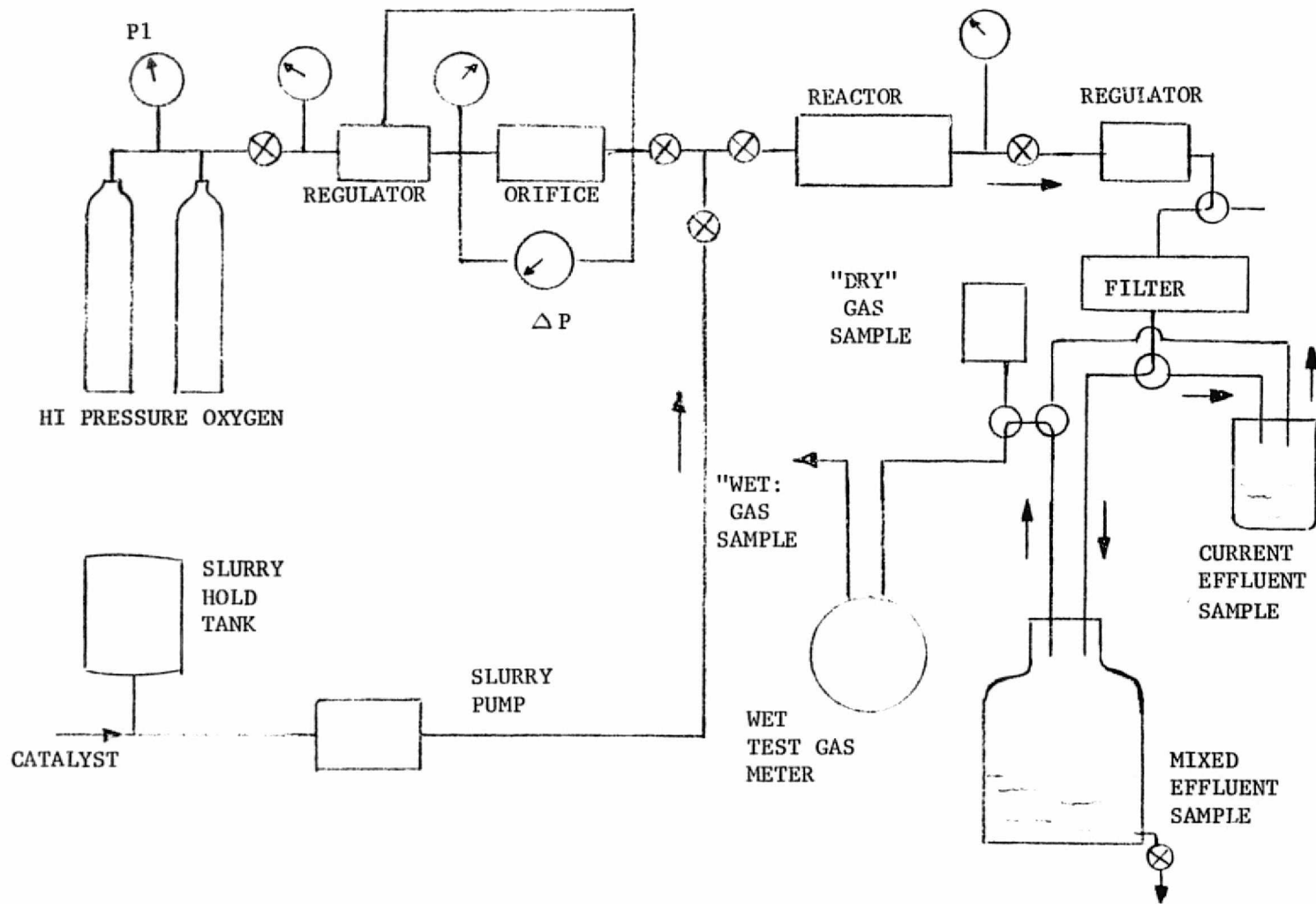
FIGURE 14 SCHEMATIC FOR MATERIAL BALANCE TEST
