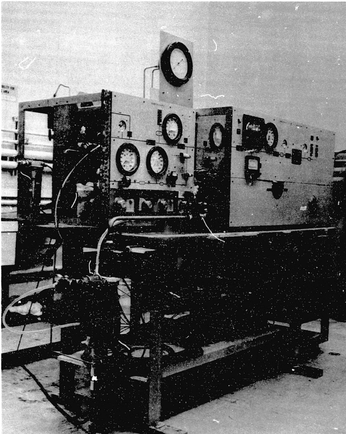
Fig. 6 Photo of Wed Oxidation Modules
