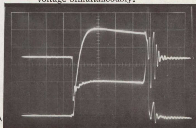
Figure 53. Driver output, Design I, showing load current and switching transistor saturation voltage simultaneously.
