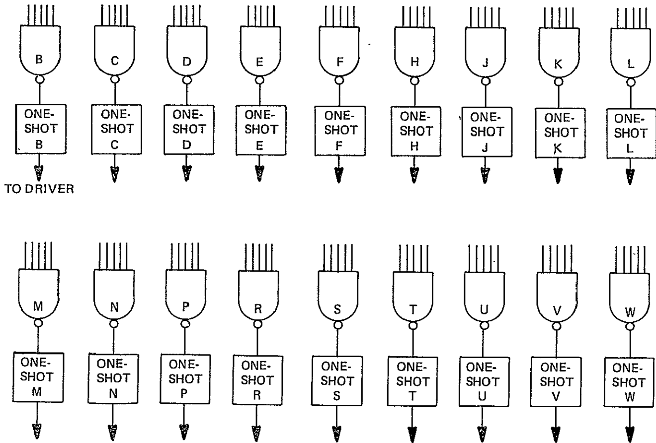
Figure 60. Block diagram of ripple-fired logic system.
