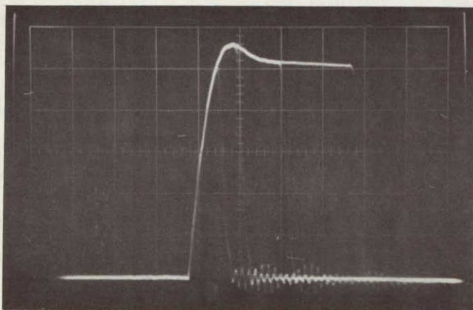
Figure 52. Driver output, Design I, multiexposure showing minimum to maximum pulse width.
