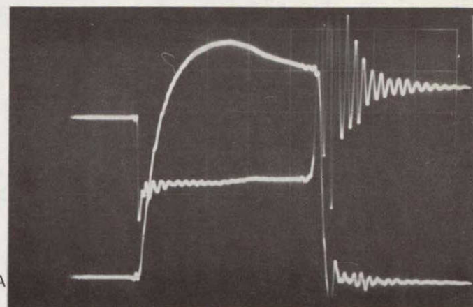
Figure 53. Driver output, Design I, showing load current and switching transistor saturation voltage simultaneously.
