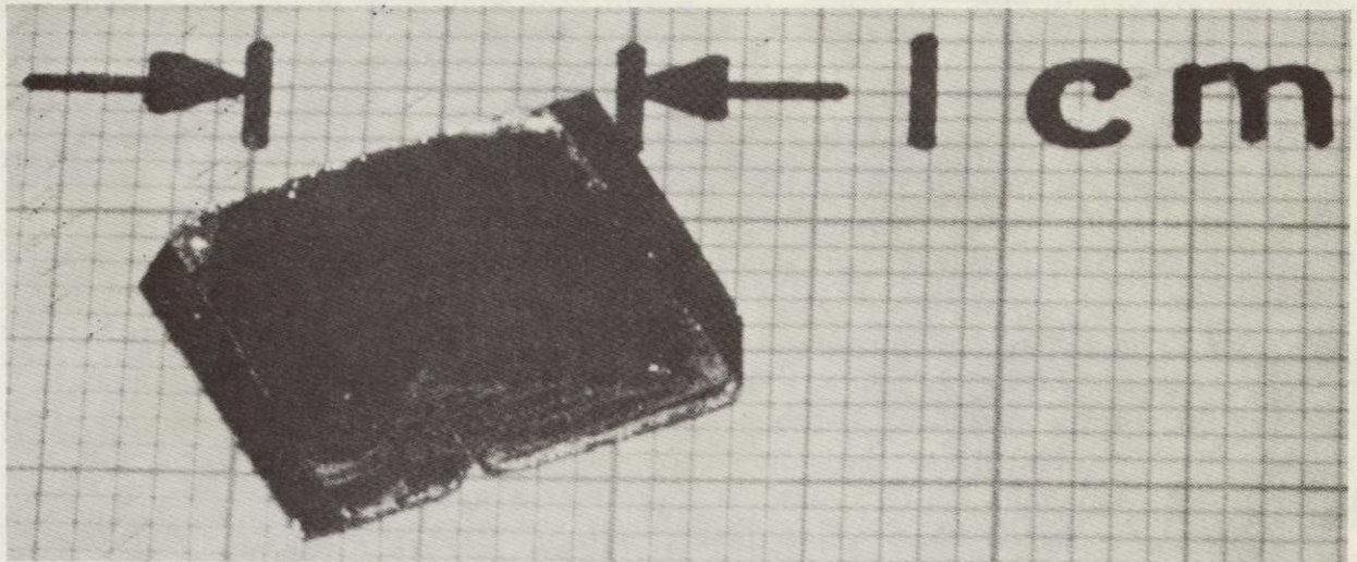
Figure 36. As-grown wafer showing solution adhering to edges and a network of defects along the leading edge. (The crystal has been cleaved through the defective region.)
