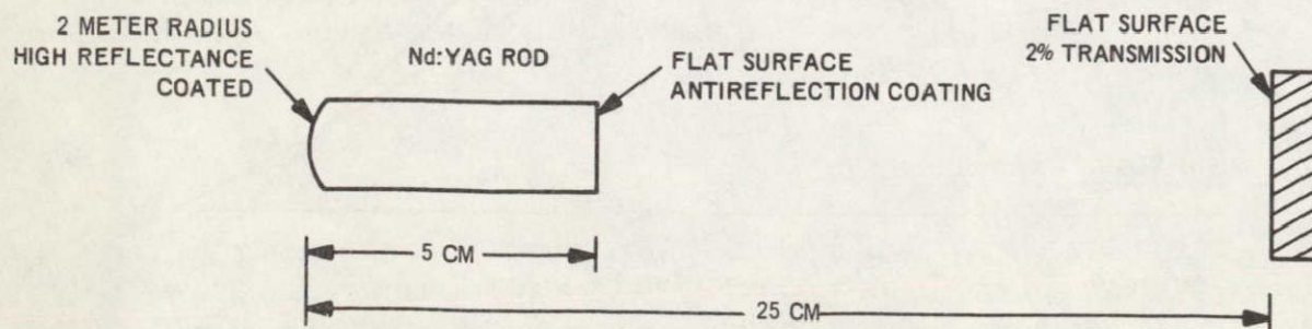
Figure 12. Cavity configuration.
