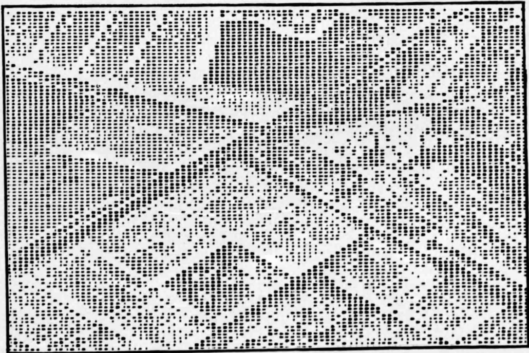
Fig. 4 - Sharpening
