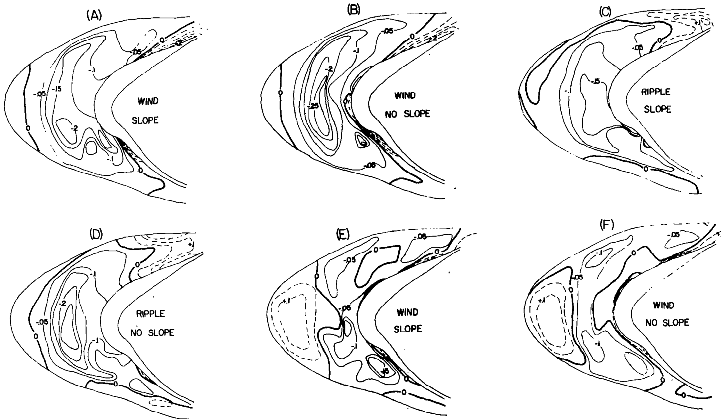
Figure 10.- Simulated erosion and deposition rates (scaled): (A-D), Simulations for nominal conditions except as indicated: Wind = transport following wind streamlines; Ripple = transport along ripple streamlines; Slope = slope effects upon transport included; No Slope = slope effects discounted; (E and F), Differences between simulated erosion rates and rates predicted by assumption of equilibrium.
