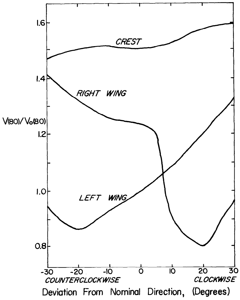
Figure 13.- 0. Effect of variation in direction of oncoming wind upon velocities ( v(80)/v_0(80) ) measured at three brinkline locations on the model dune (see Fig. 5).
