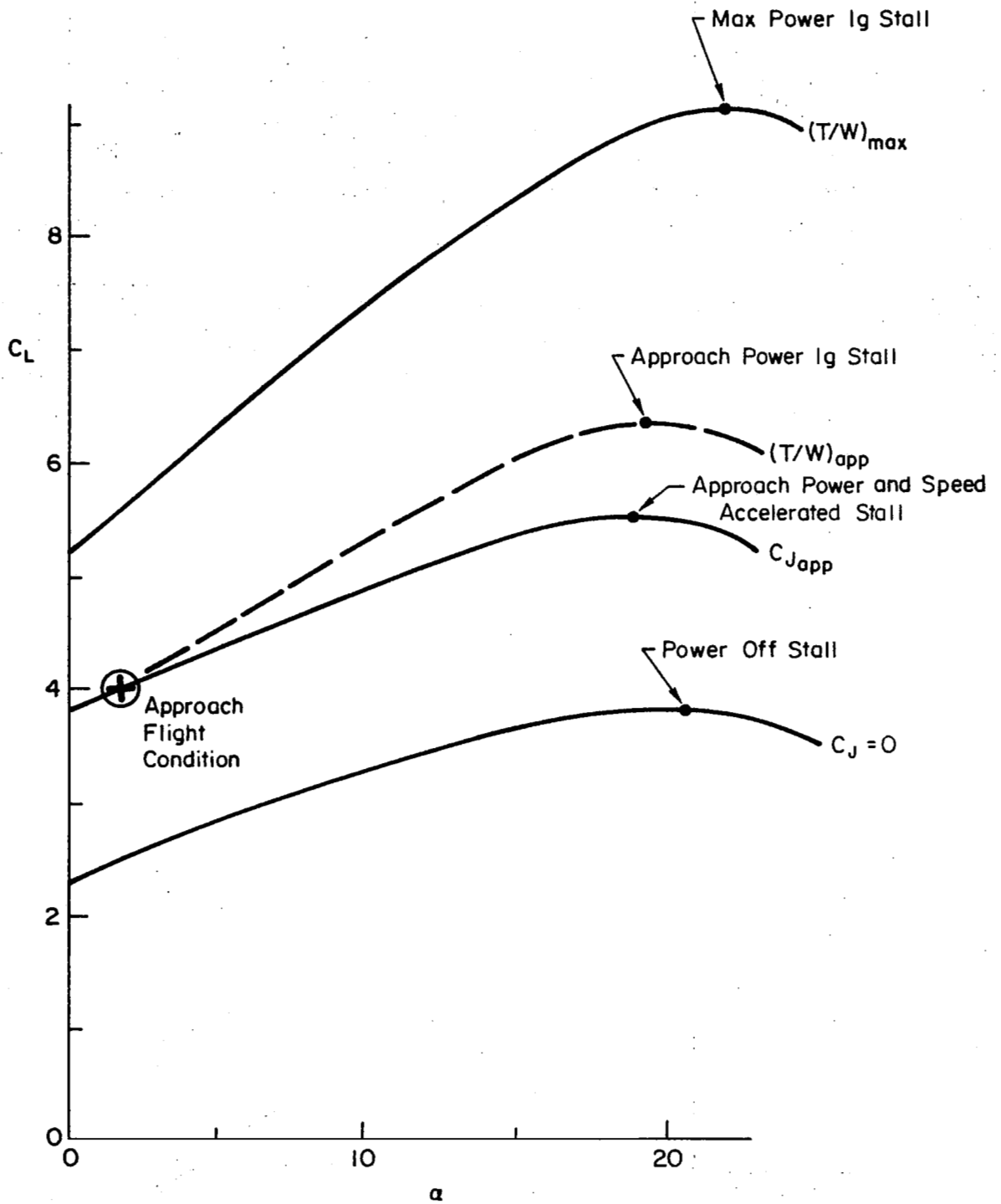
Figure 3-2: Variety of Stall Types for Powered-Lift Aircraft
