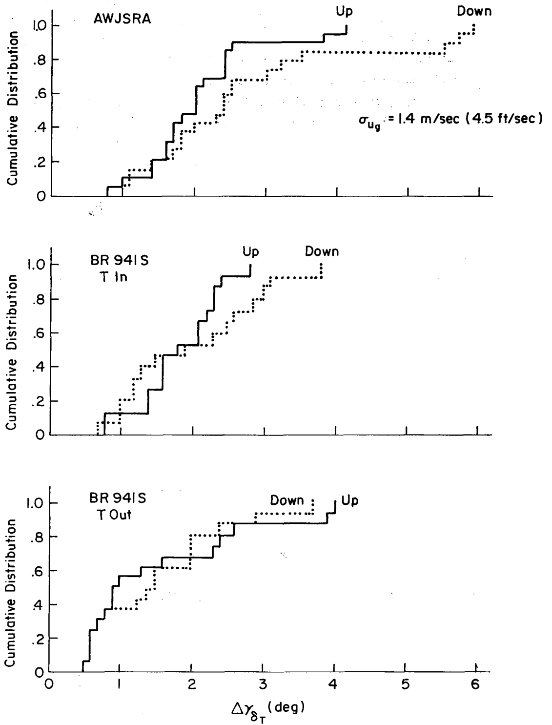
Figure 5-9: Cumulative Distribution of Maximum Flight Path Corrections
