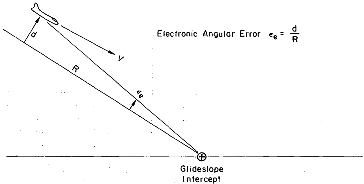
Figure 5-5: Two Examples of Perceived Flight Path Error (Visual and ILS)
