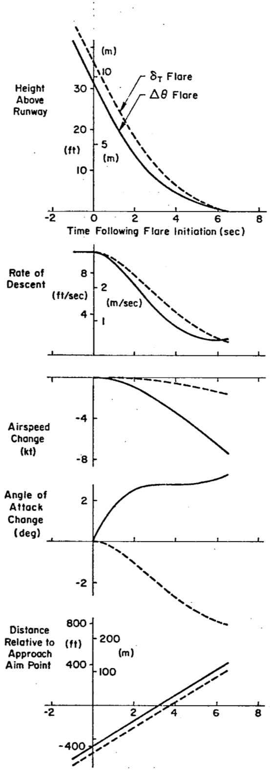
Figure 6-5: Comparison of Flare Technique
