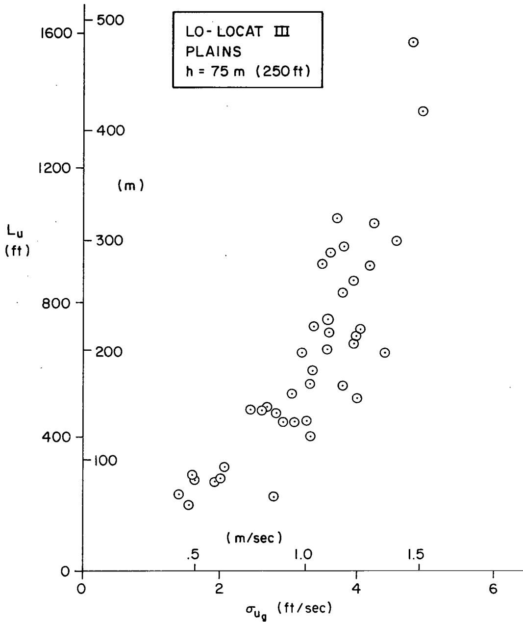
Figure B-9: Measured Values of Scale Length Versus RMS u_g
