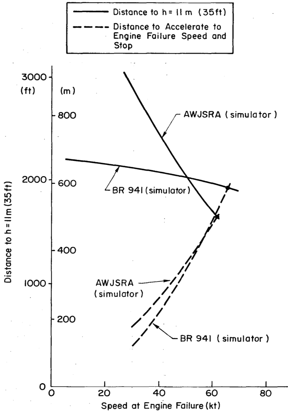
Figure 11-1: Effect of Engine Failure on Takeoff and Stopping Distance
