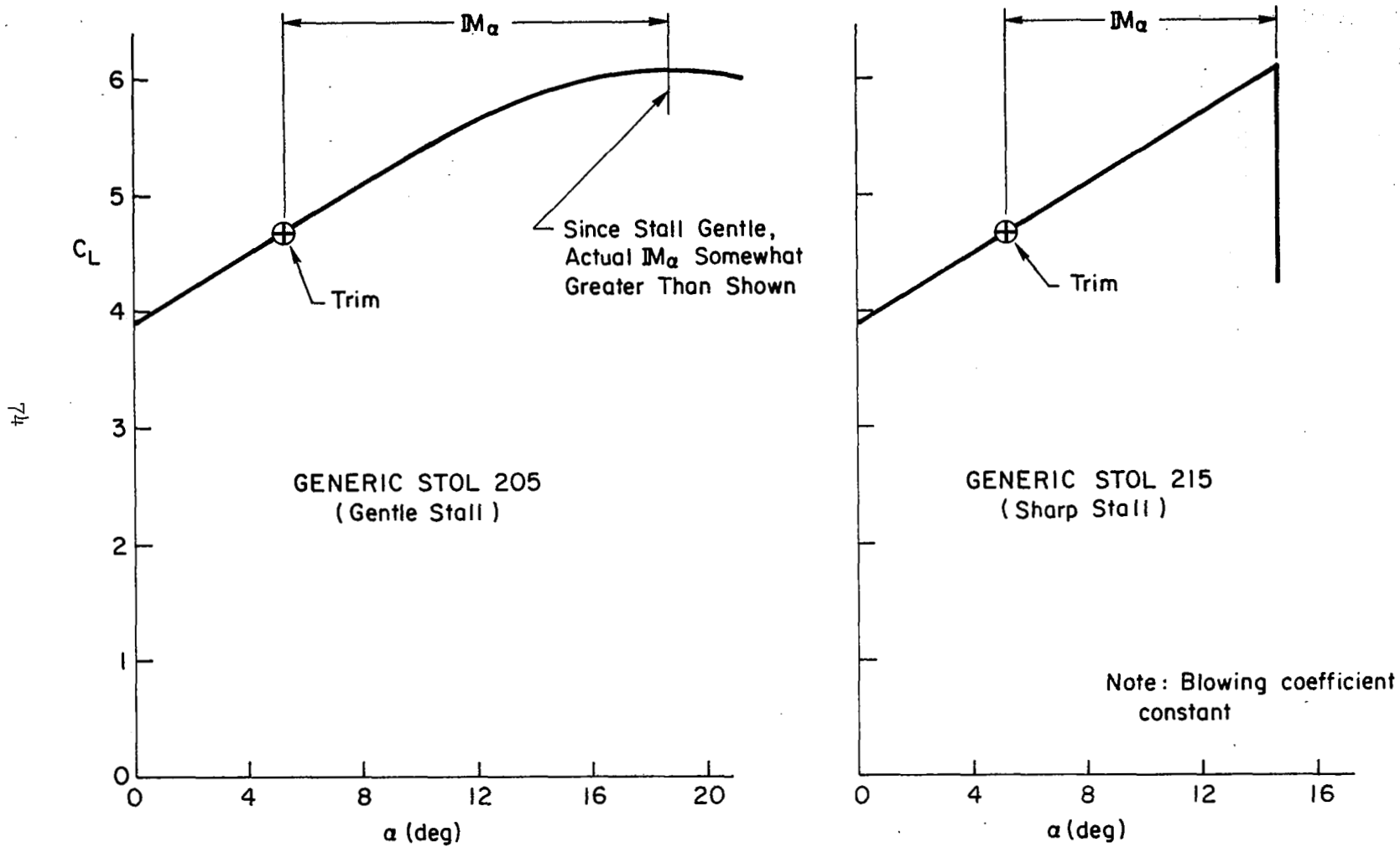
Figure 4-16: Lift versus Angle of Attack (Cases used to show need for angle of attack margin)
