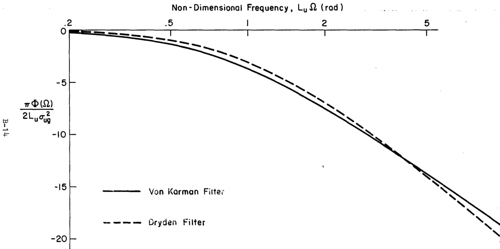
Figure B-5: Comparison of Normalized Horizontal Gust Power Spectral Density for Von Karman and Dryden Spectral Forms
