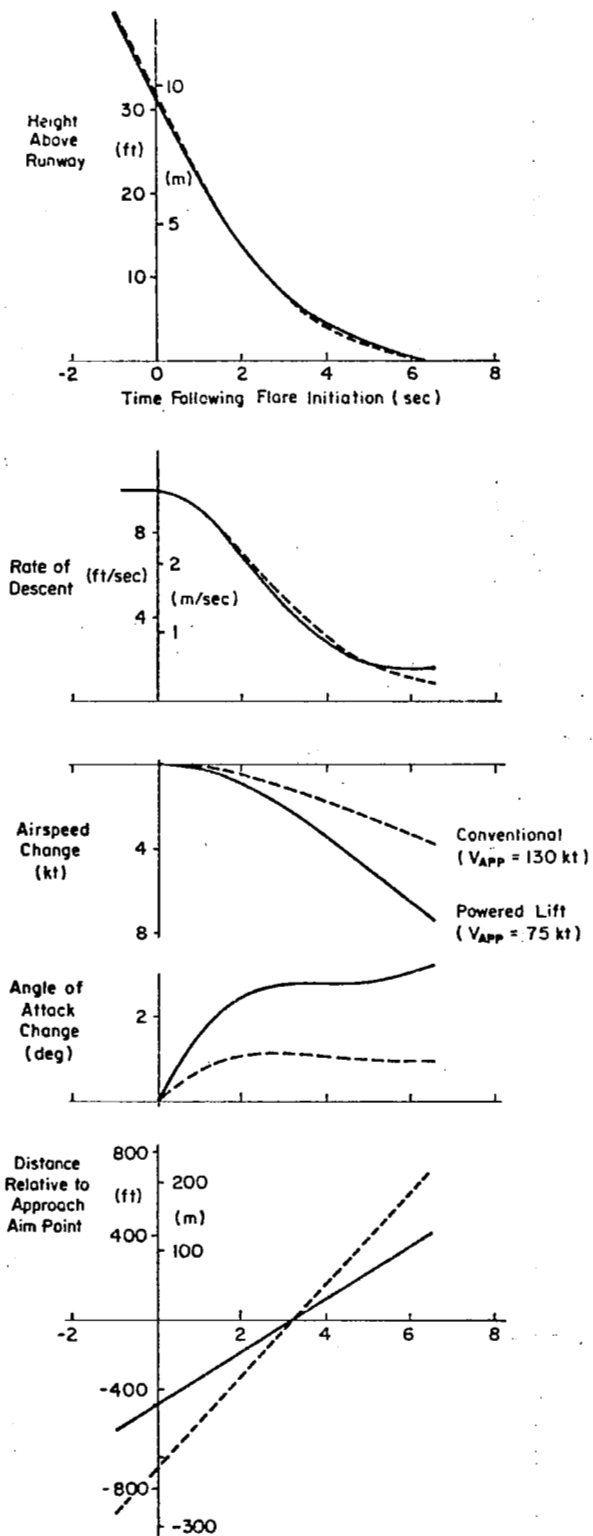
Figure 6-3: Comparison of Aircraft Categories with Regard to Flare
