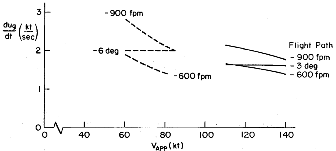
Figure 5-10: Comparative Ability to Counter Horizontal Shears in the Long Term
