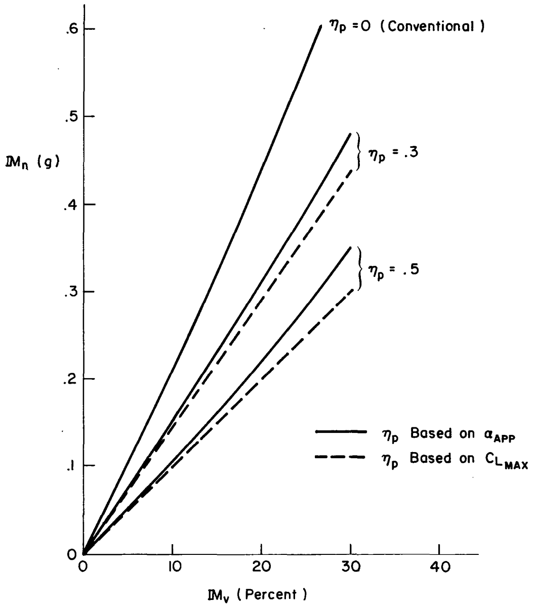
Figure 4-9: Lift Margin Implied by Relative Speed Margin (Powered-Lift Aircraft)
