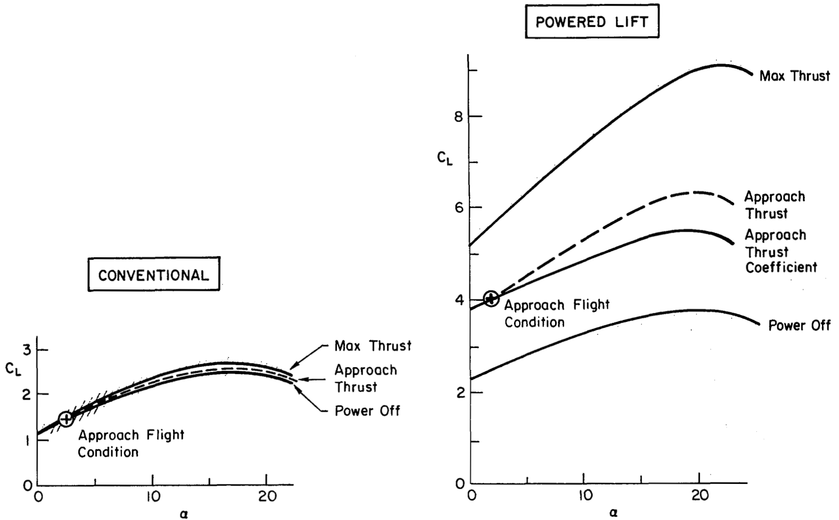
Figure 3-1: Typical Plots of Lift Coefficient versus Angle of Attack and Thrust
