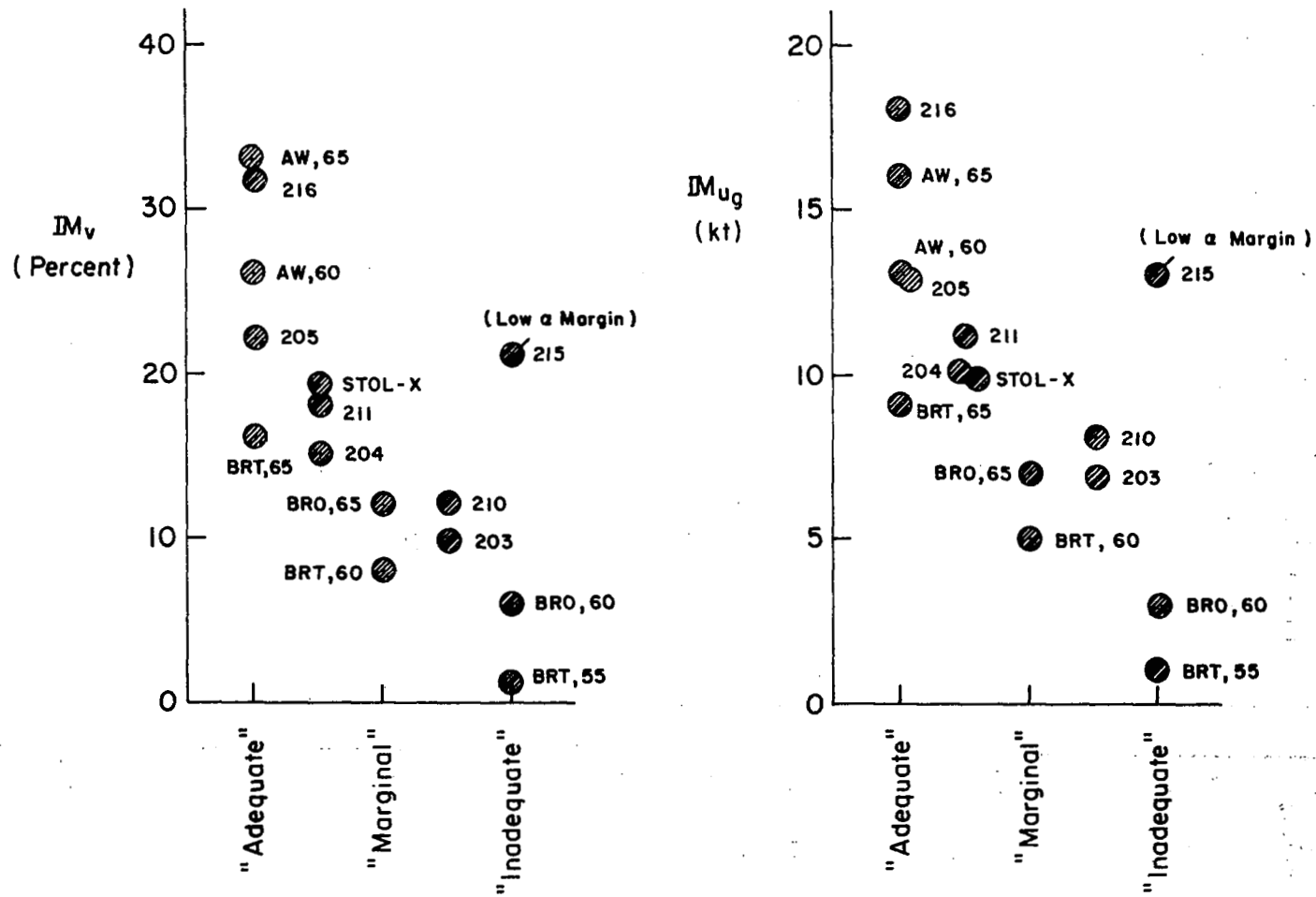
Figure 4-14: Speed Margin Trends
