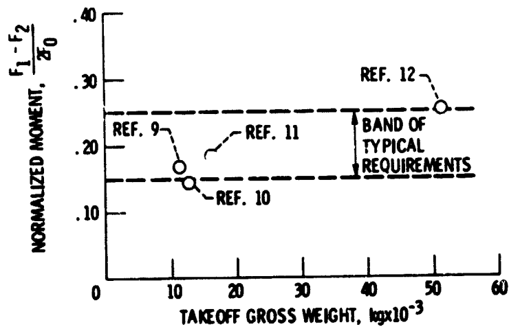
Figure 4. - V/STOL aircraft differential thrust requirements for roll control.
