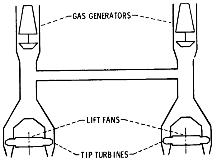
Figure 1. - Gas-coupled lift fan system.
