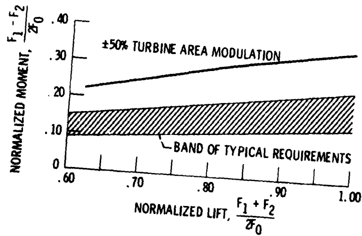
Figure 7. - Available control moment versus available lift for the gas-coupled system with variable-area turbines.
