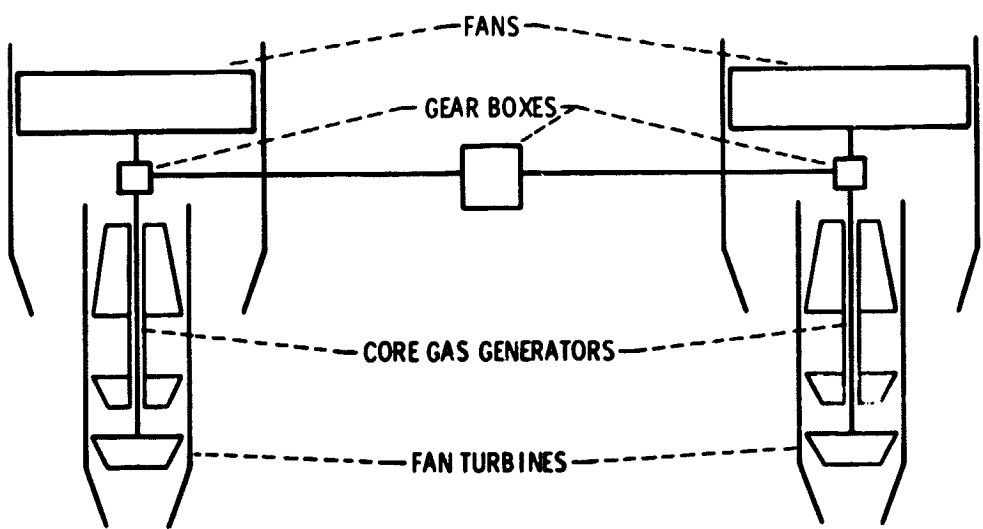
Figure 2. - Shaft-coupled lift fan system.
