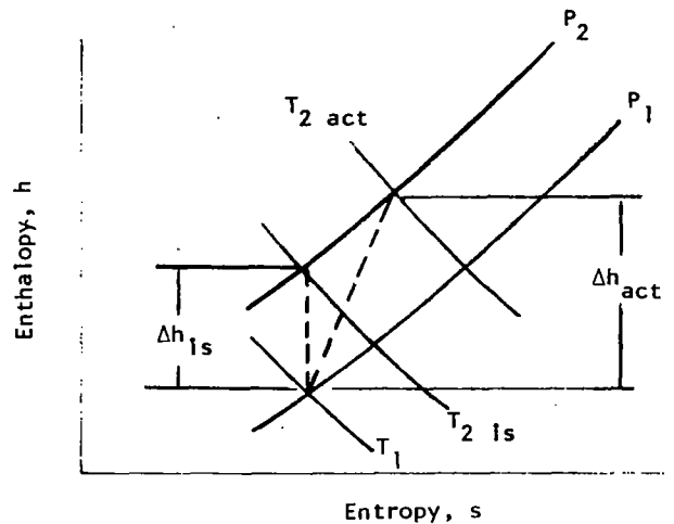
Figure 20. Mollier Diagram
