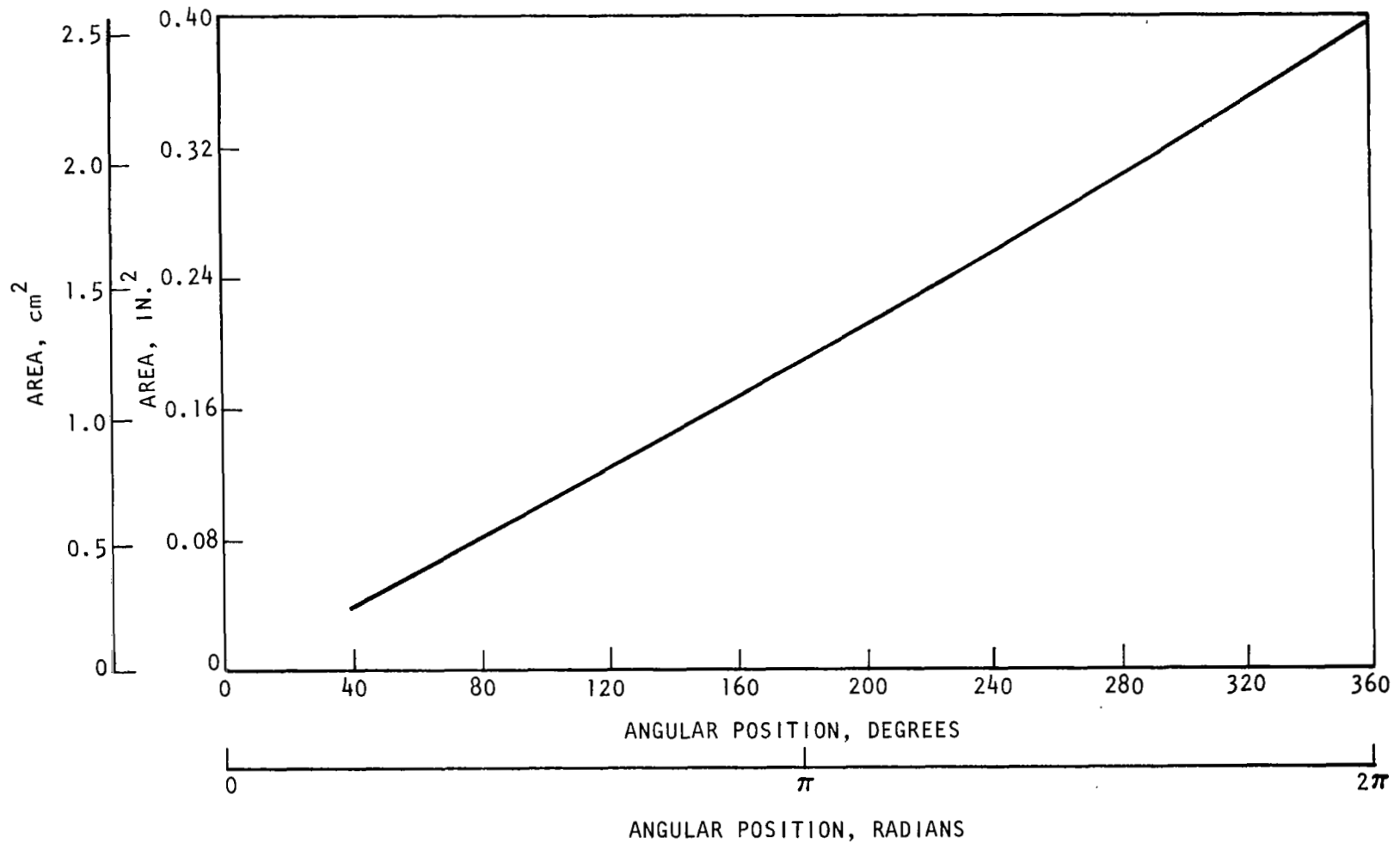
Figure 19. Mark 48-F Pump Volute Area Distribution
