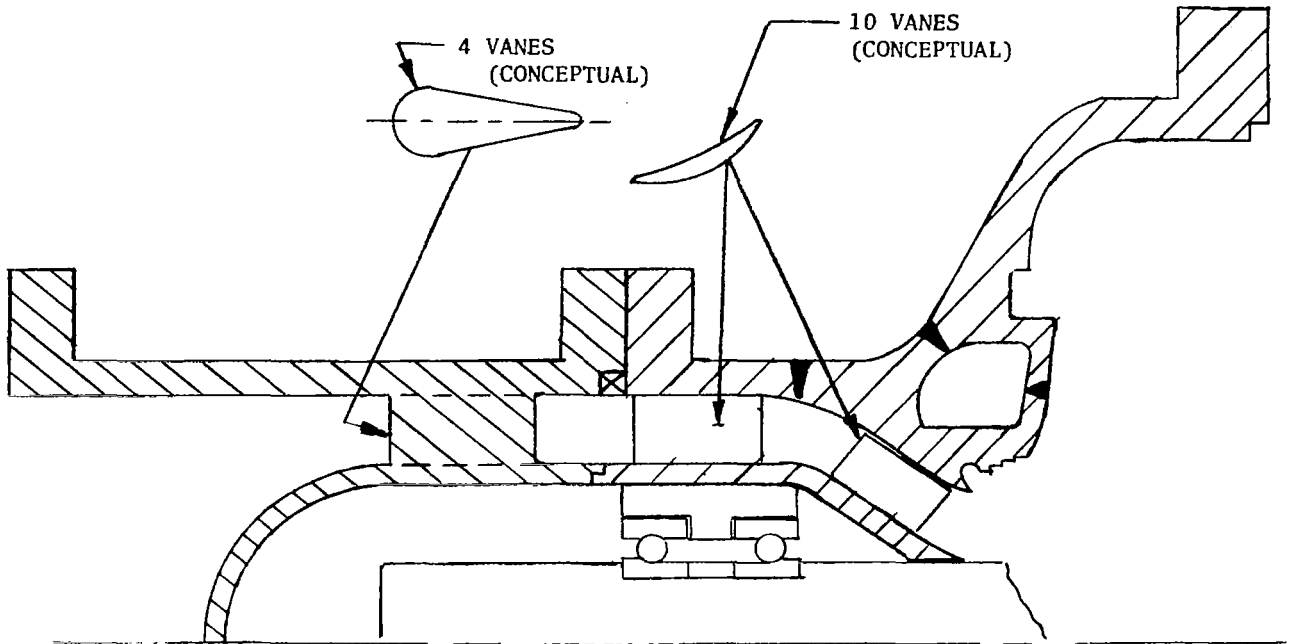
Figure 91. Mark 48-F Turbopump Axial Entry Pump Inlet
