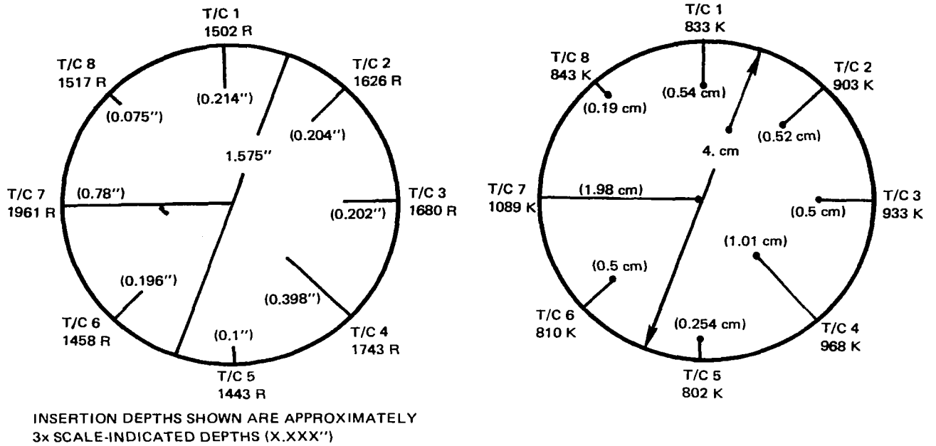
Figure 120. Thermocouple Rake Installation and Typical Temperature Measurements
