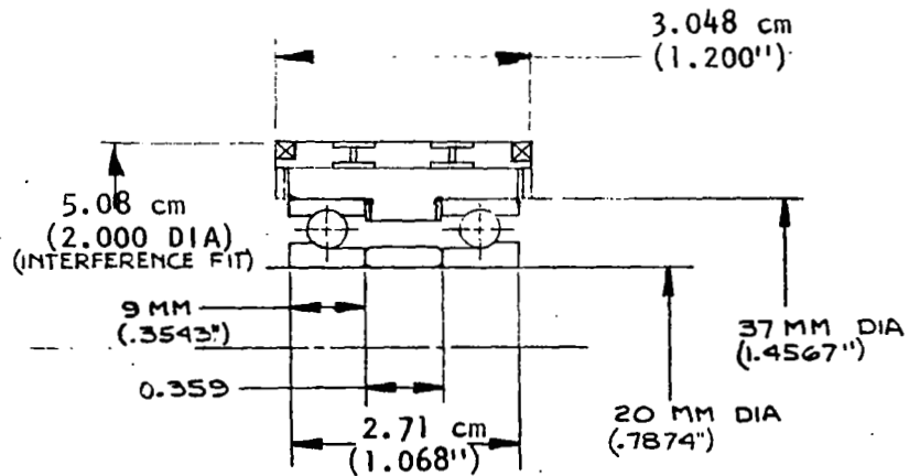
Figure 48. Mark 48-F Turbopump Hybrid Bearing Installation
