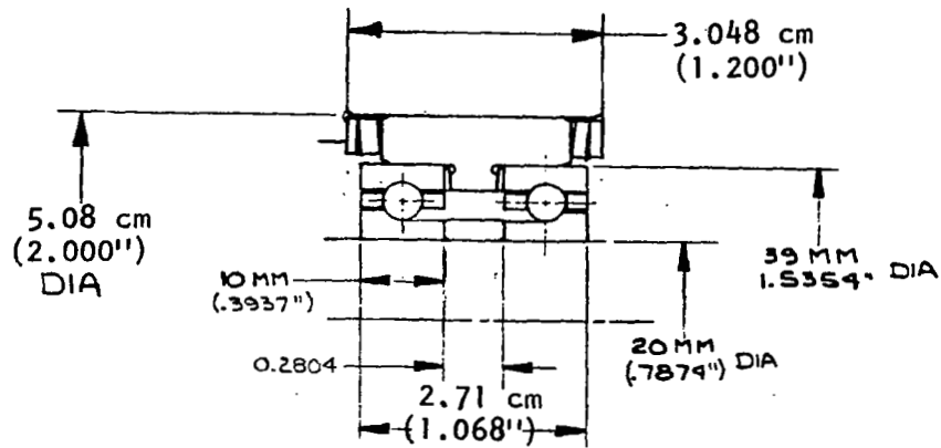
Figure 46. Mark 48-F Turbopump Rocketdyne Bearing Installation
