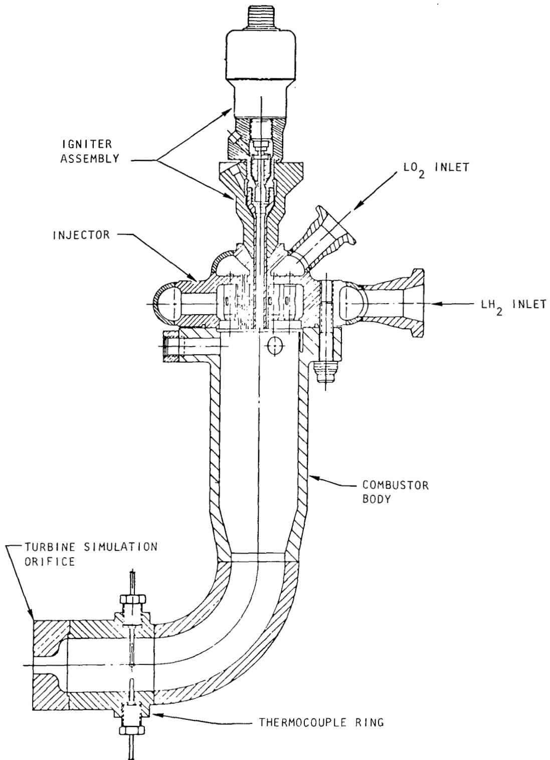
Figure 80. LH 2 Turbopump Gas Generator
