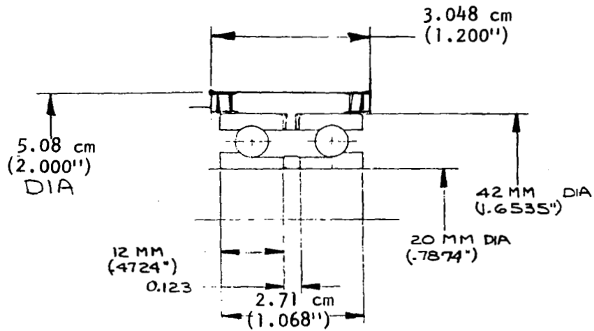
Figure 47. Mark 48-F Turbopump MTI Ball Bearing Installation
