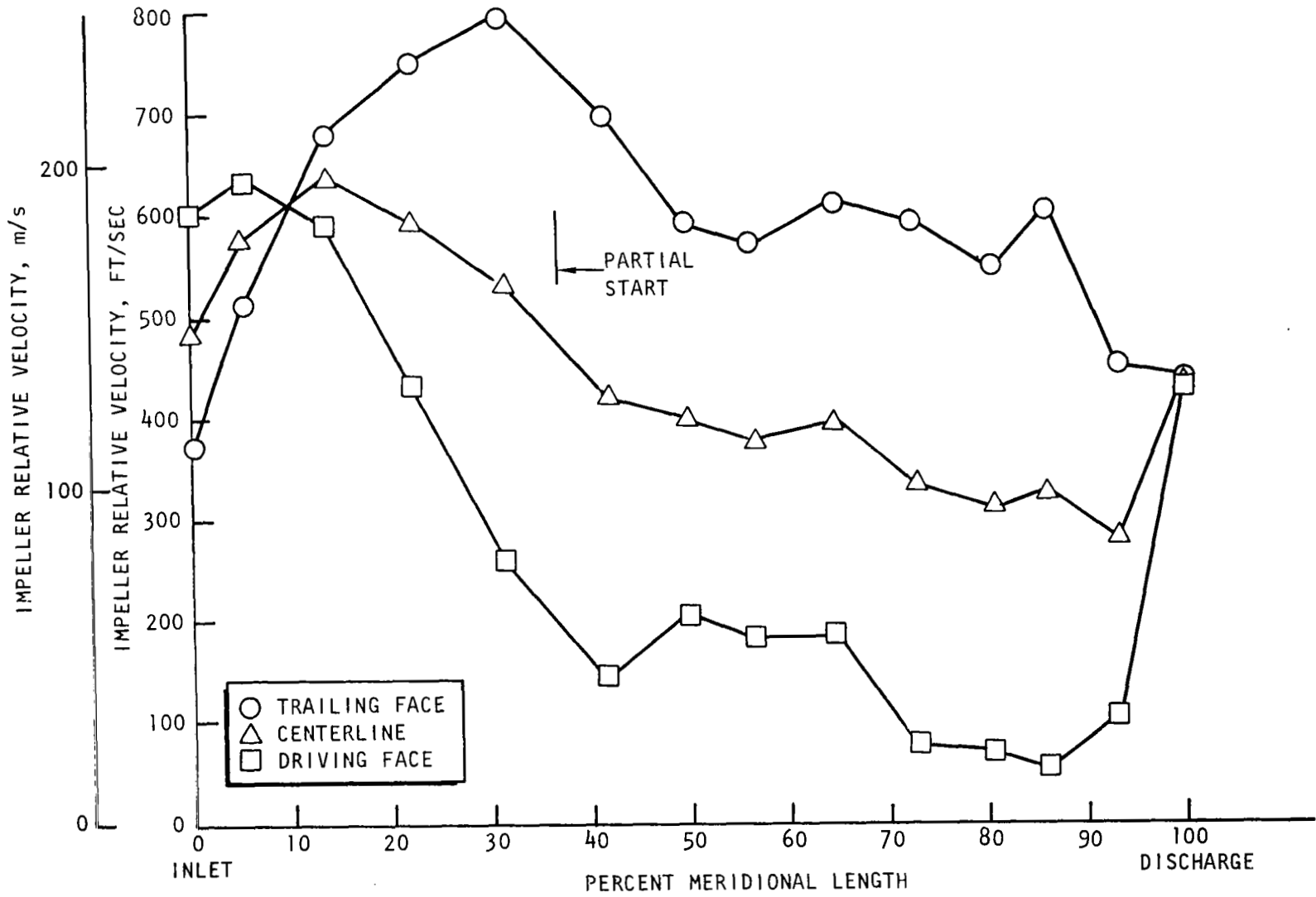
Figure 10. Fuel Impeller Relative Velocities, Inner Streamtube
