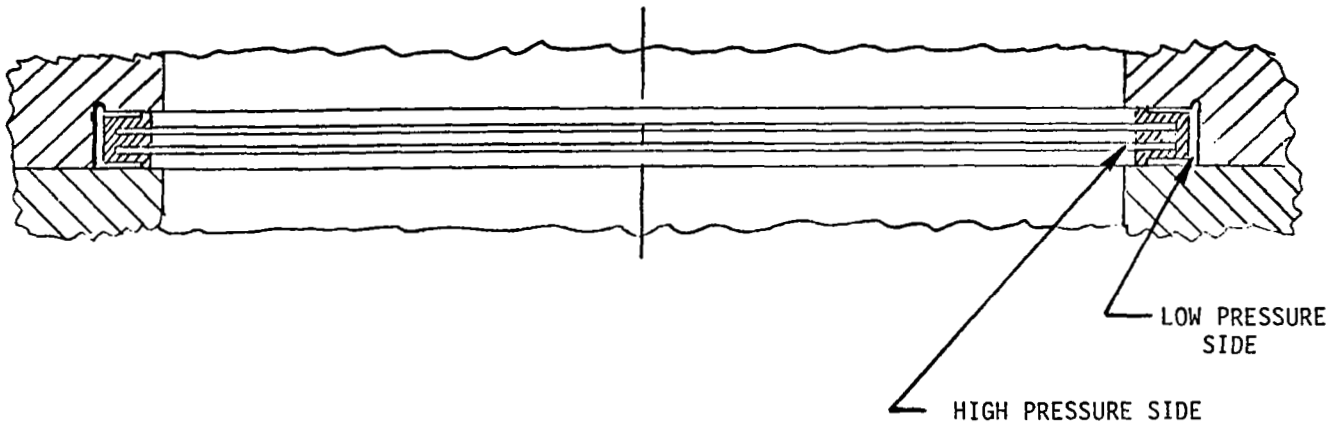
Figure 52. Typical Static Flange Seal Configuration
