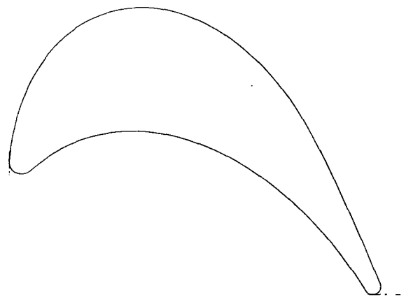
Figure 33. Mark 48-F Turbine Second-Stage Rotor Blade Shape
