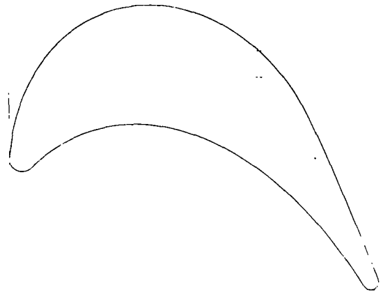
Figure 31. Mark 48-F Turbine First-Stage Rotor Blade Shape
