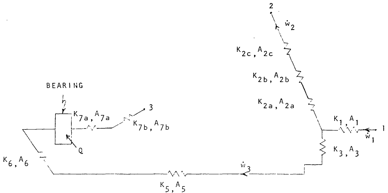
Figure 153. Front Bearing Coolant Resistances
