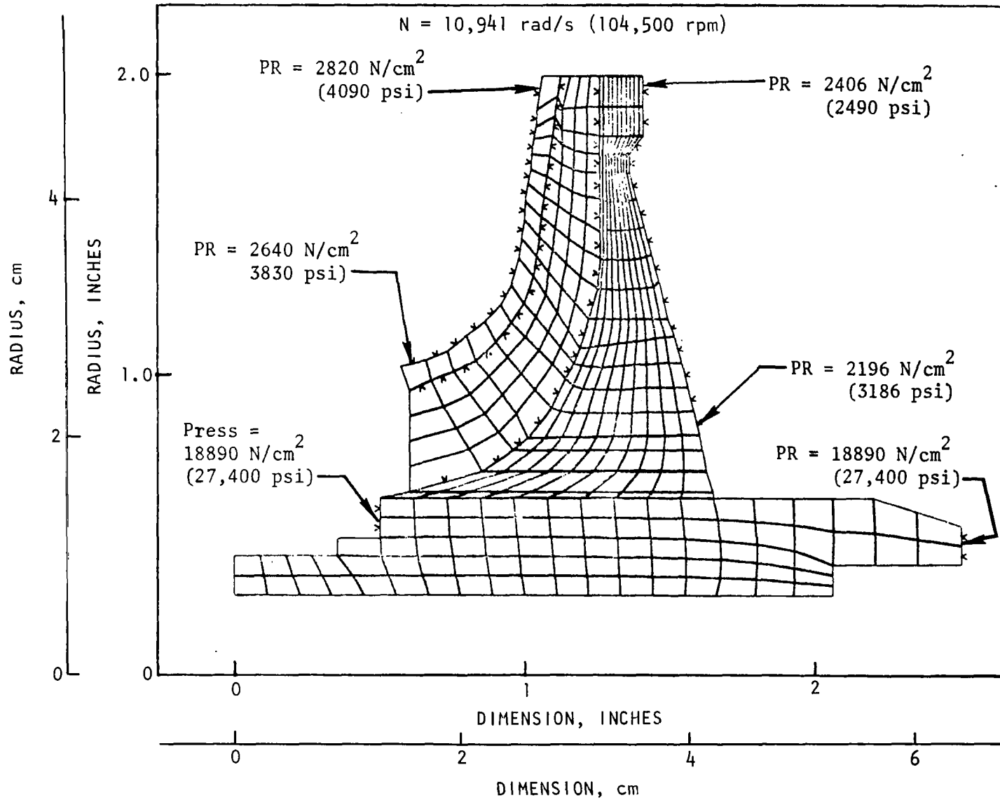
Figure 67. Mark 48-F Third-Stage Impeller Finite-Element Model
