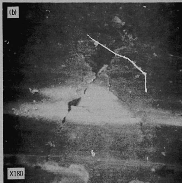
Figure 9. - 33 Percent dense NiCrAlY fibermetal after interaction with a knife-edge at 305 m/sec rotational speed, 25.4 \times 10^{-6} m/sec incursion rate, 1116 o K. (a) Microsection of the rub groove; (b) SEM photograph of the rub surface.
