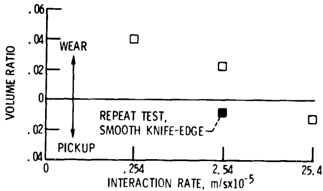
Figure 6. - Volume wear ratio versus incursion rate for 33 percent dense fibermetal. Surface speed was 305 m/sec and temperature was 1366^{\circ} K.
