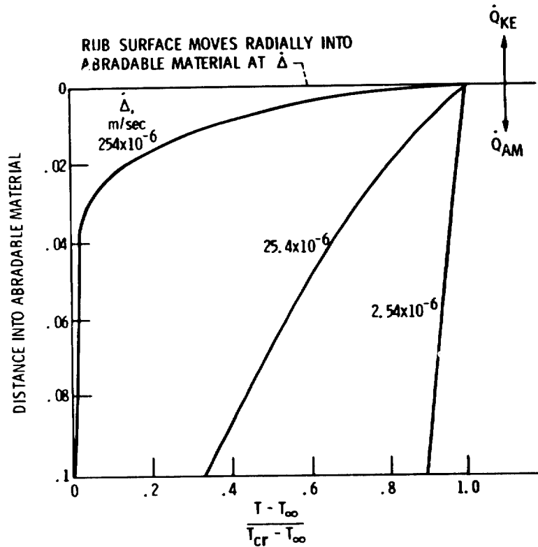
Figure 11. - Schematic representation of temperature profile beneath the sub surface, in the abradable material.
