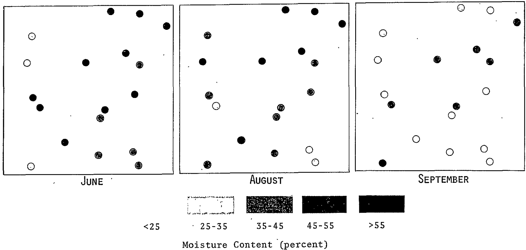
Figure 4-22. Moisture content of the herbaceous vegetation measured at the ETSA primary sites.
