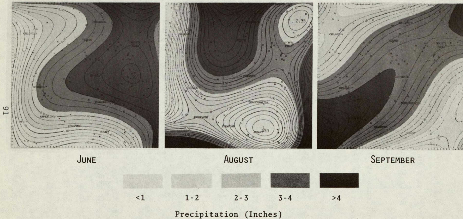
Figure 4-9. Accumulated precipitation from 61 weather stations for the 18-day period prior to Landsat overpasses in the ETSA corresponding with the June, August and September sampling periods in 1975.
