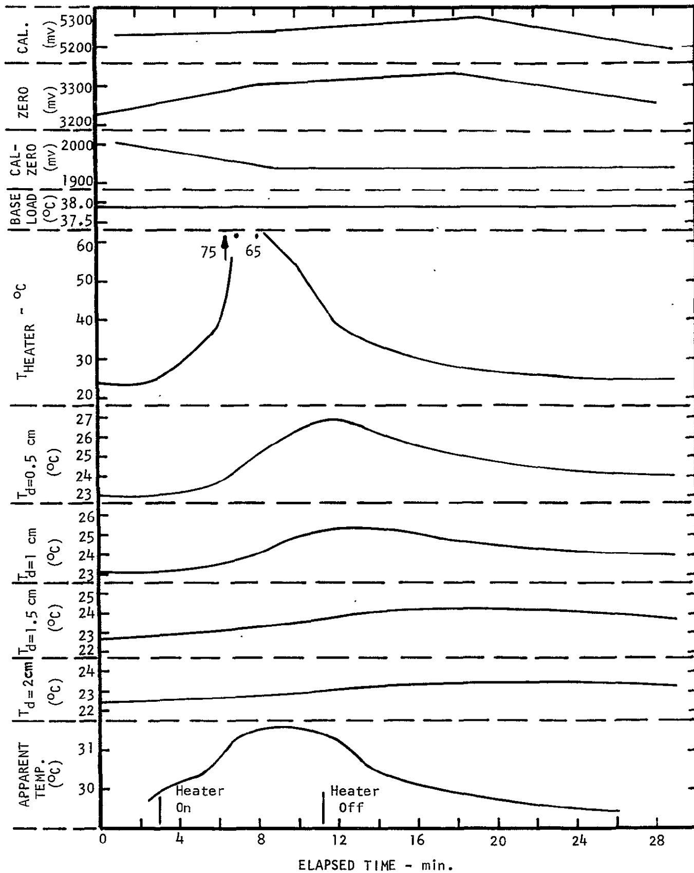
Figure 3-2 - Phantom Measurement No. 1 - Beefsteak Layer Thickness = 5 mm
